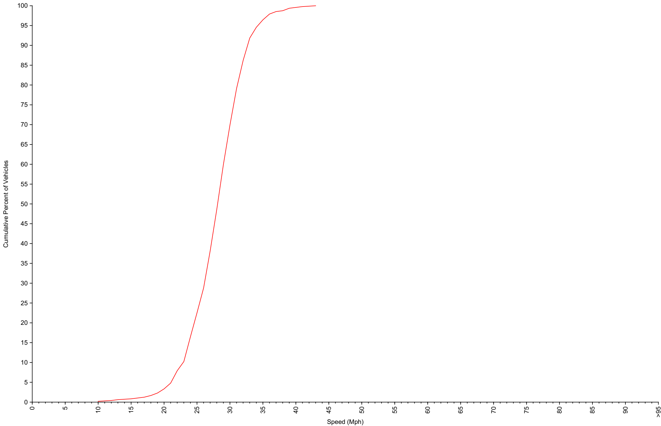
Cumulative Speed Distribution Curve Daily Overview for Thu Jul 17 2025
