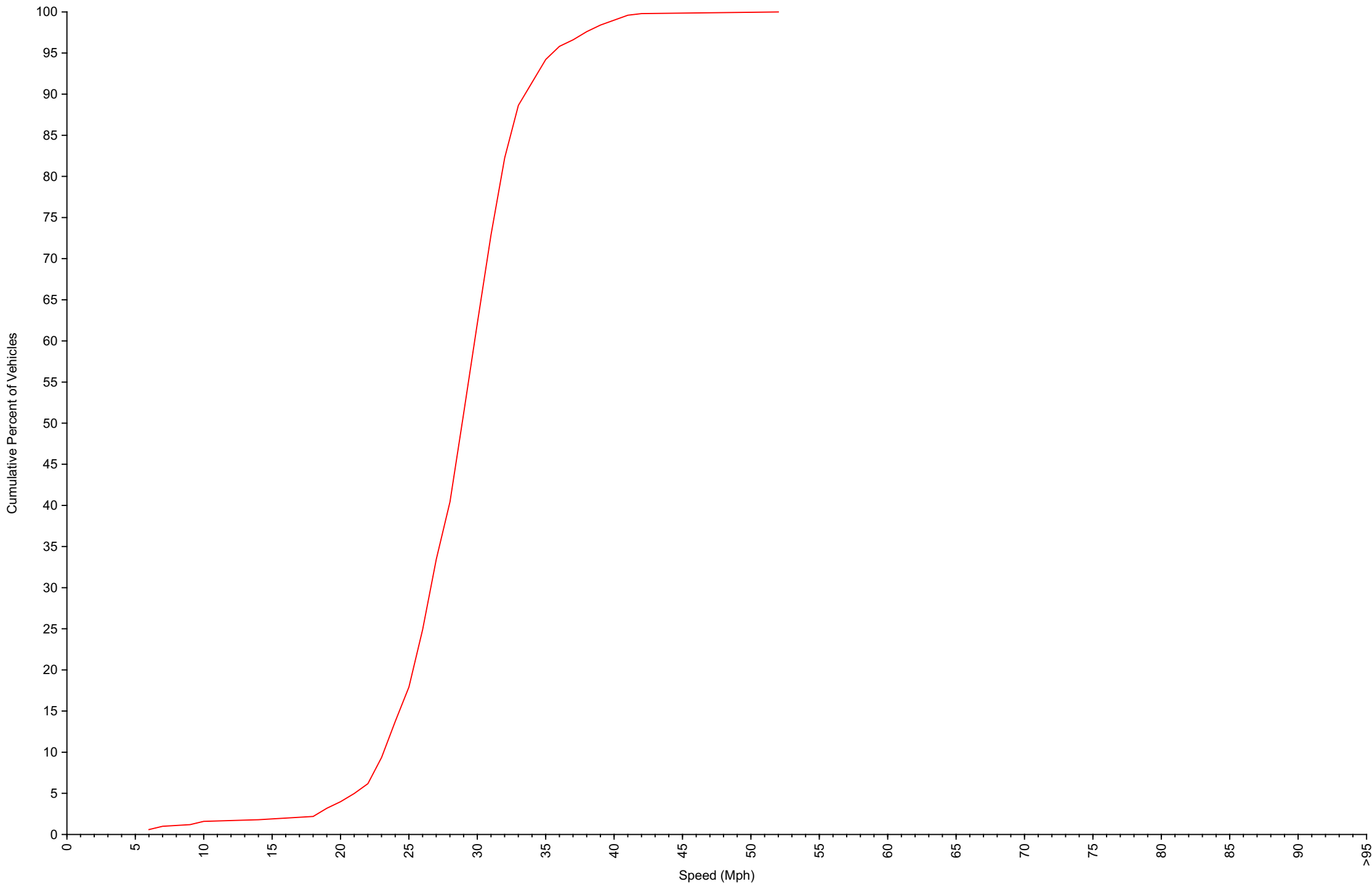
Cumulative Speed Distribution Curve Daily Overview for Fri Aug 23 2024
