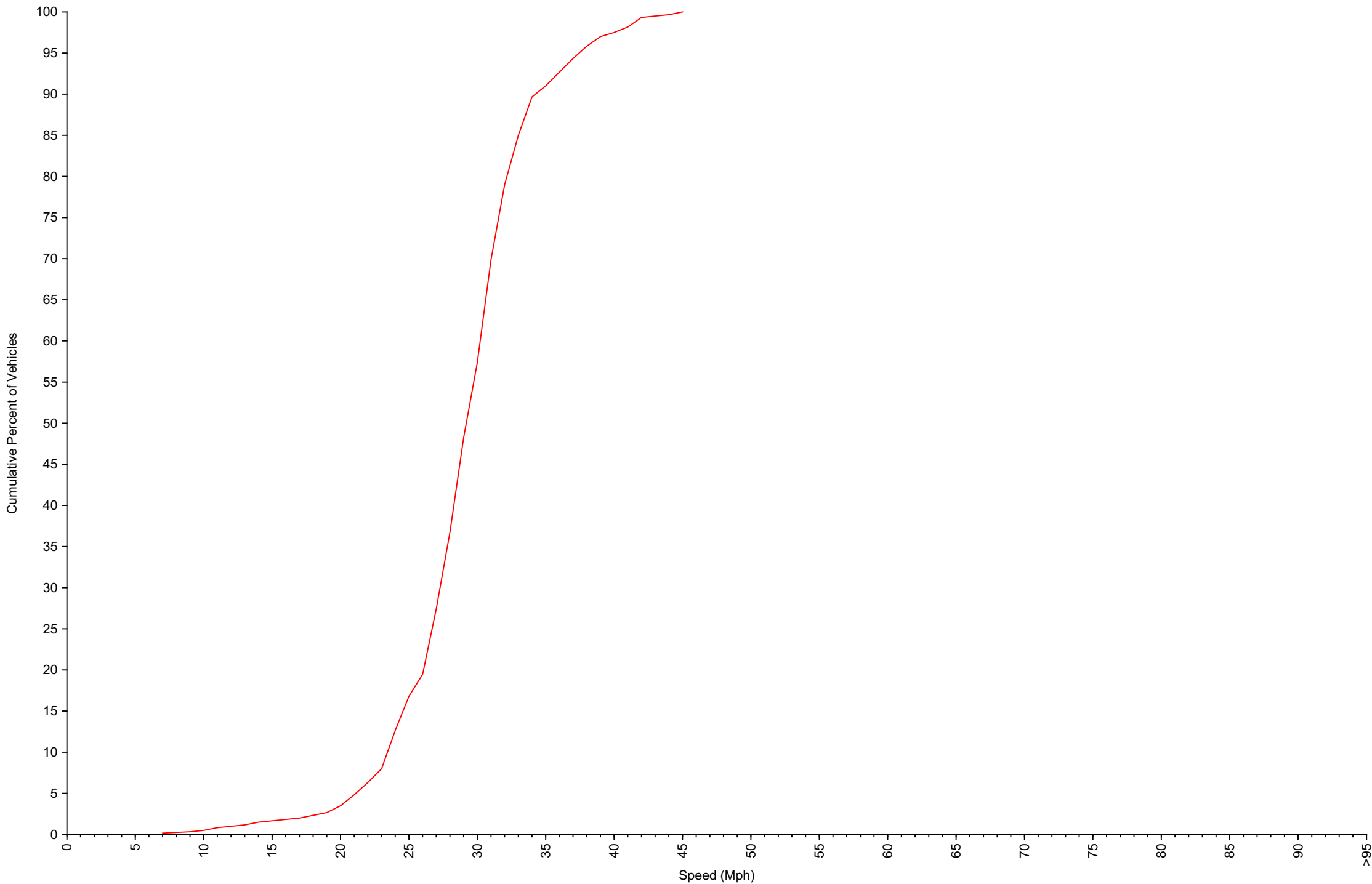
Cumulative Speed Distribution Curve Daily Overview for Mon Aug 5 2024
