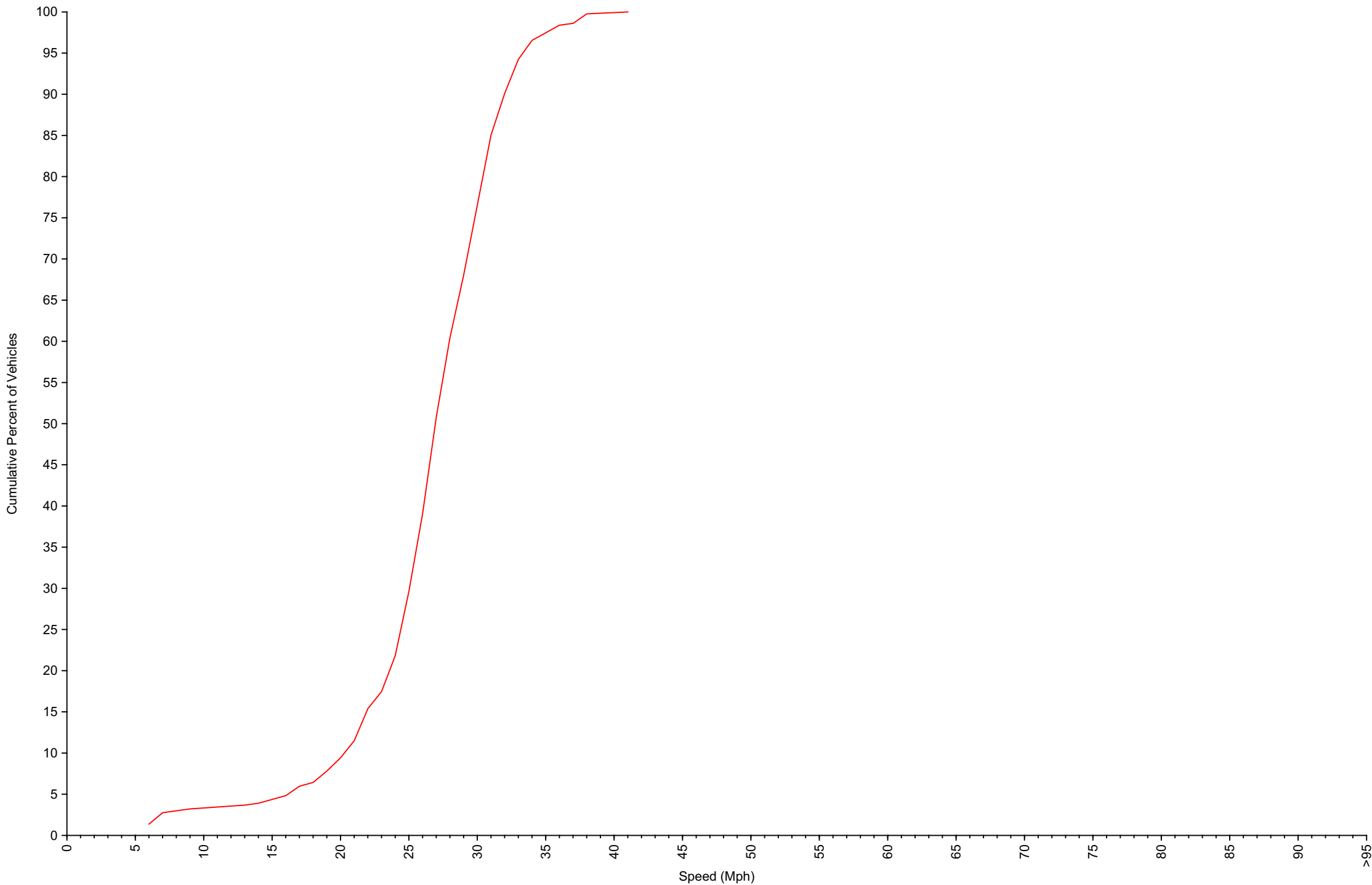
Cumulative Speed Distribution Curve Daily Overview for Thu Aug 22 2024
