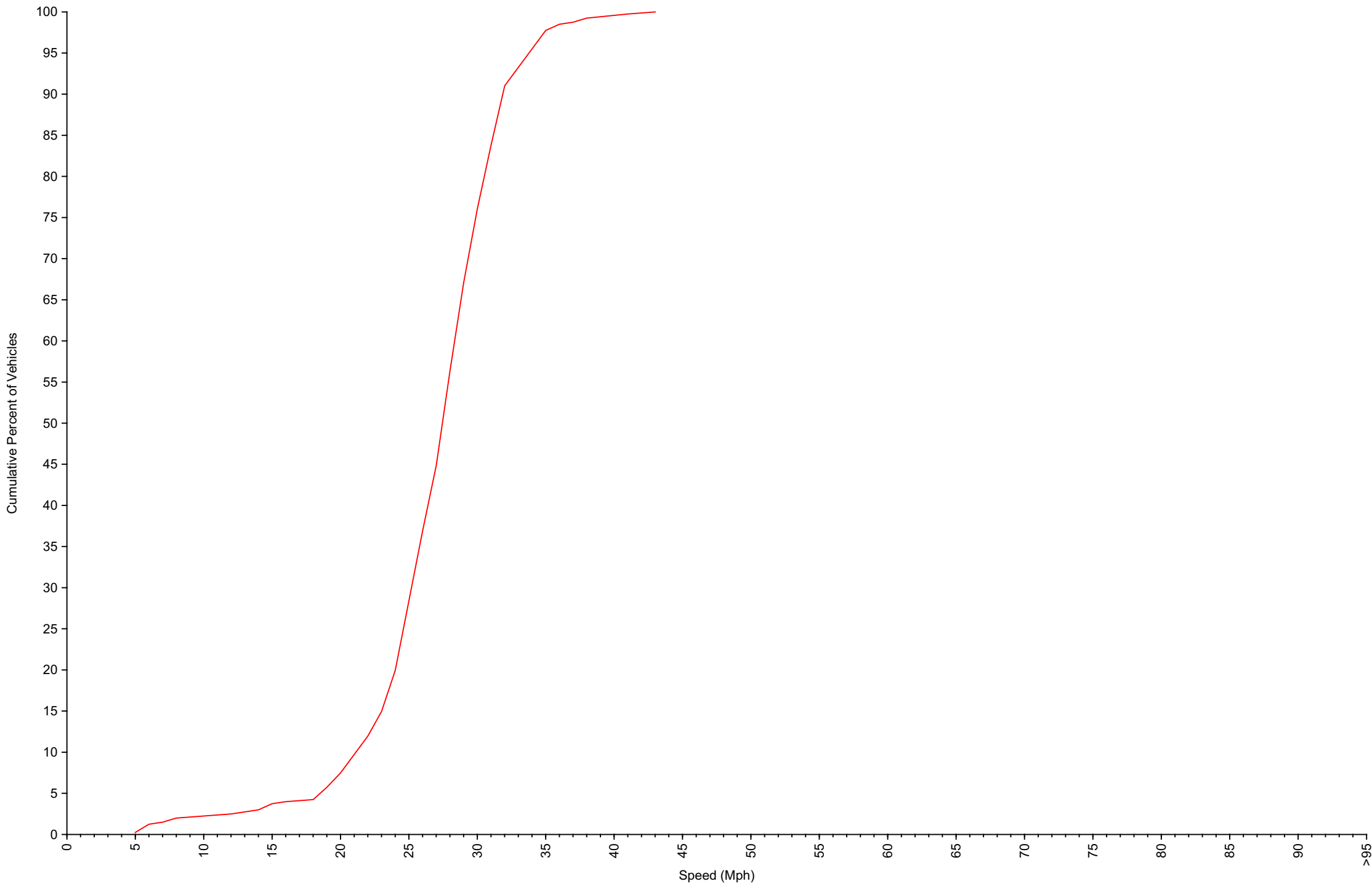
Cumulative Speed Distribution Curve Daily Overview for Thu Aug 8 2024
