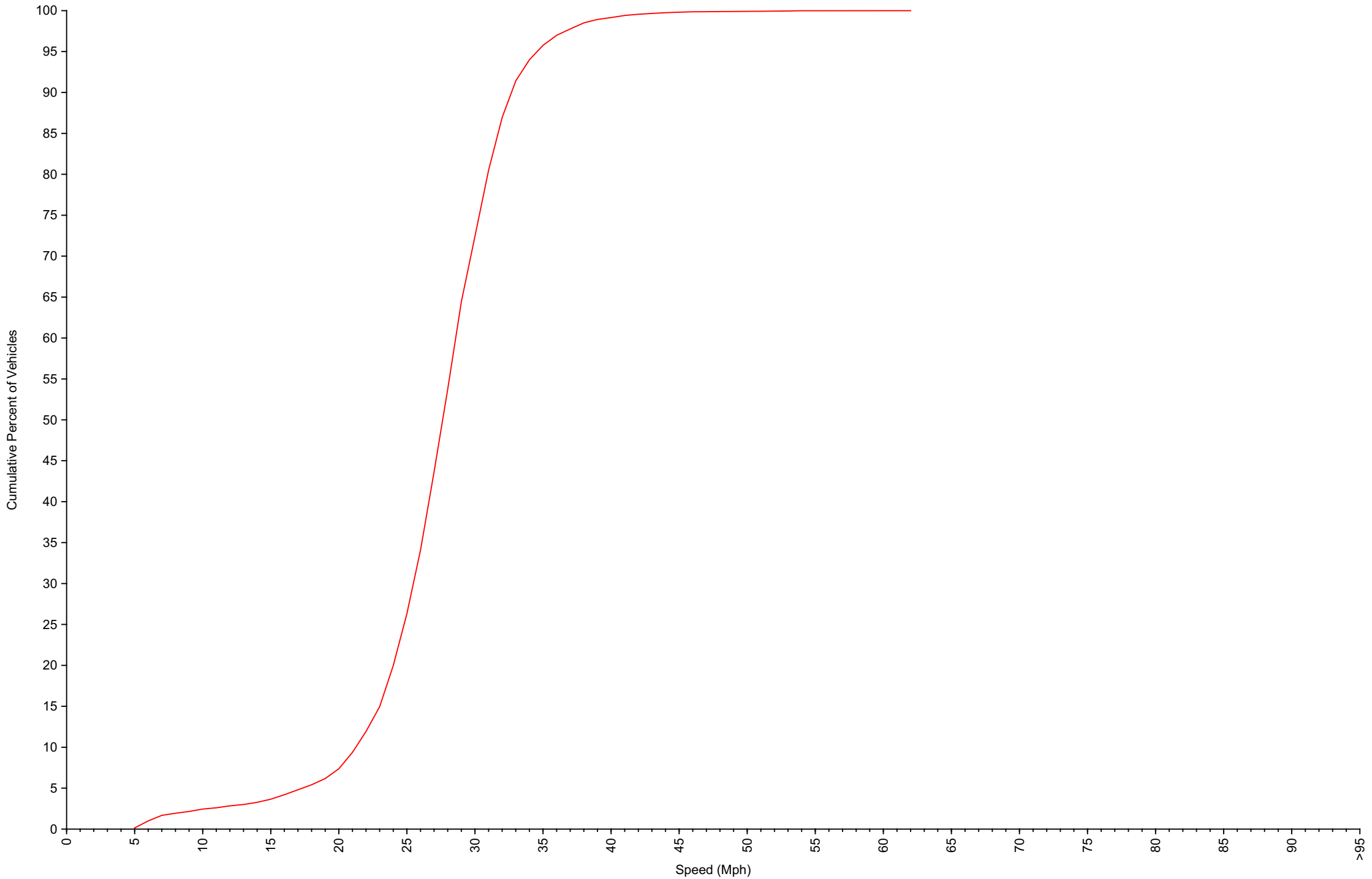
Cumulative Speed Distribution Curve Traffic Overview from Mon Aug 5 2024 to Sat Aug 31 2024
