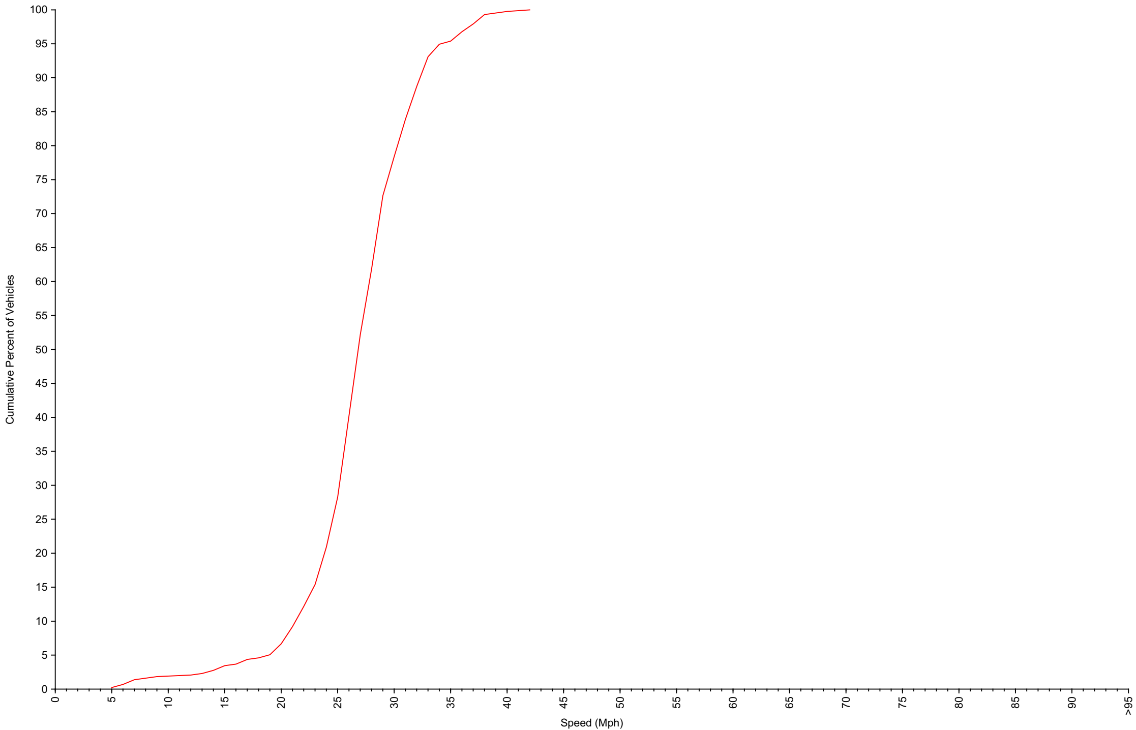
Cumulative Speed Distribution Curve Daily Overview for Wed Aug 21 2024
