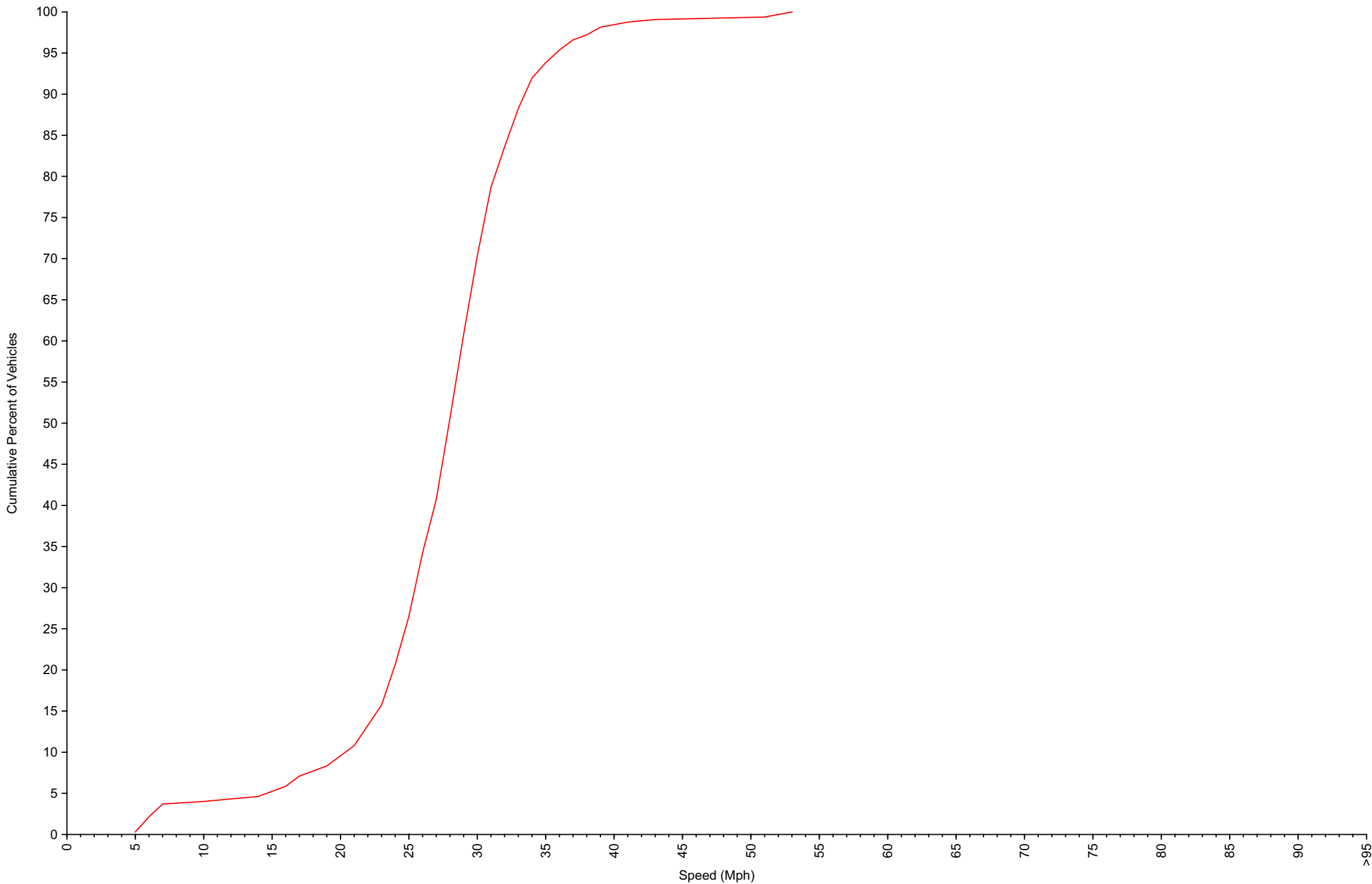
Cumulative Speed Distribution Curve Daily Overview for Mon Aug 26 2024
