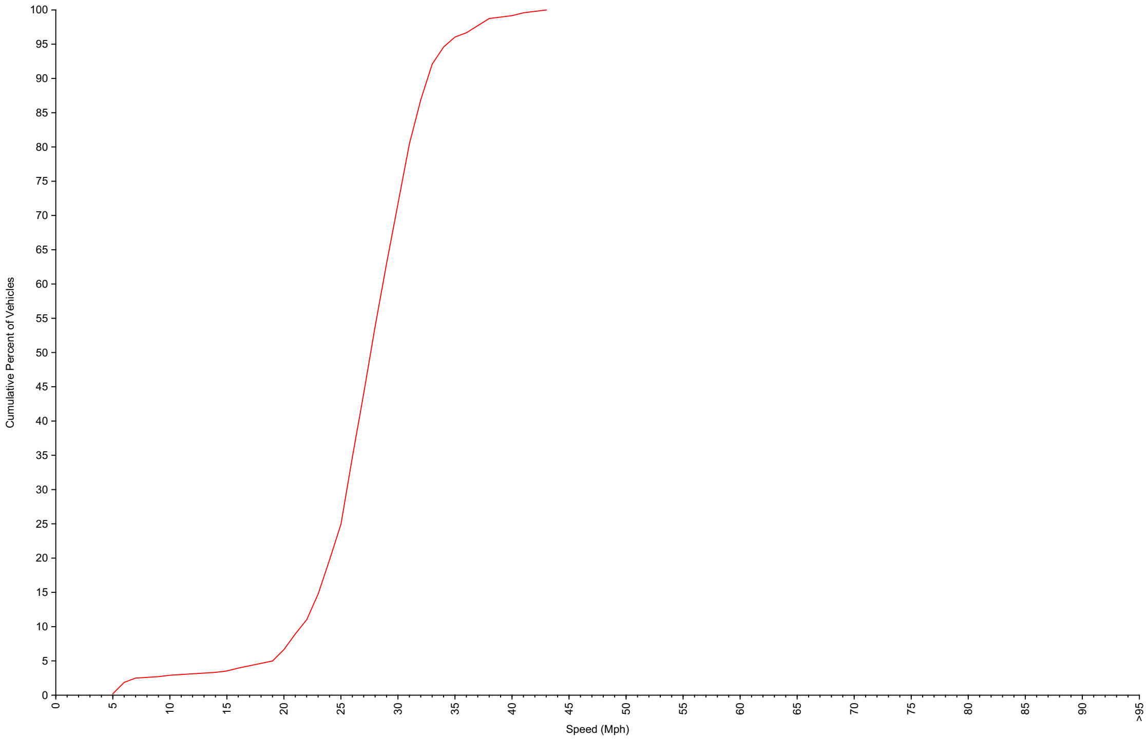
Cumulative Speed Distribution Curve Daily Overview for Thu Aug 29 2024
