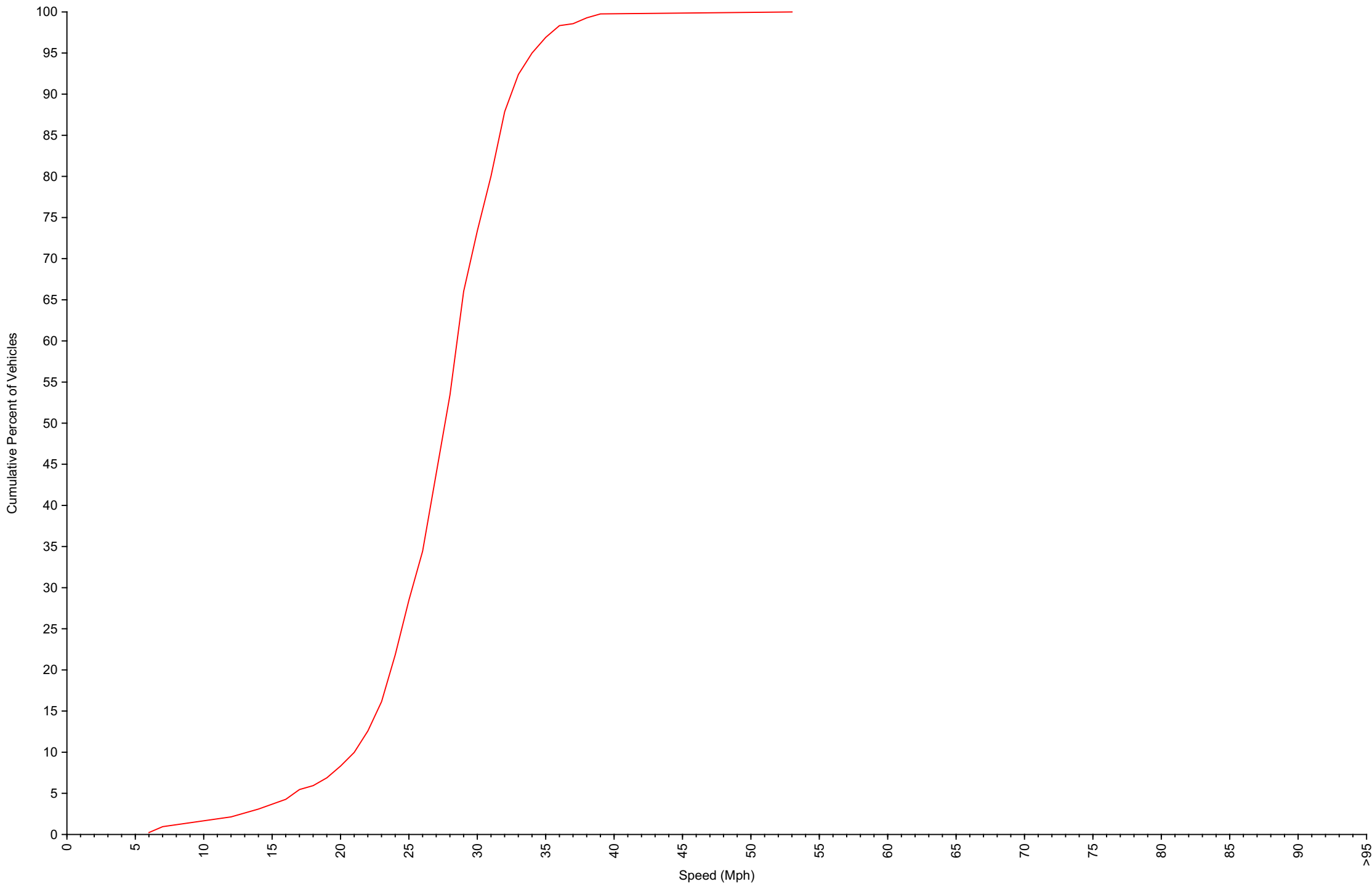
Cumulative Speed Distribution Curve Daily Overview for Mon Aug 19 2024
