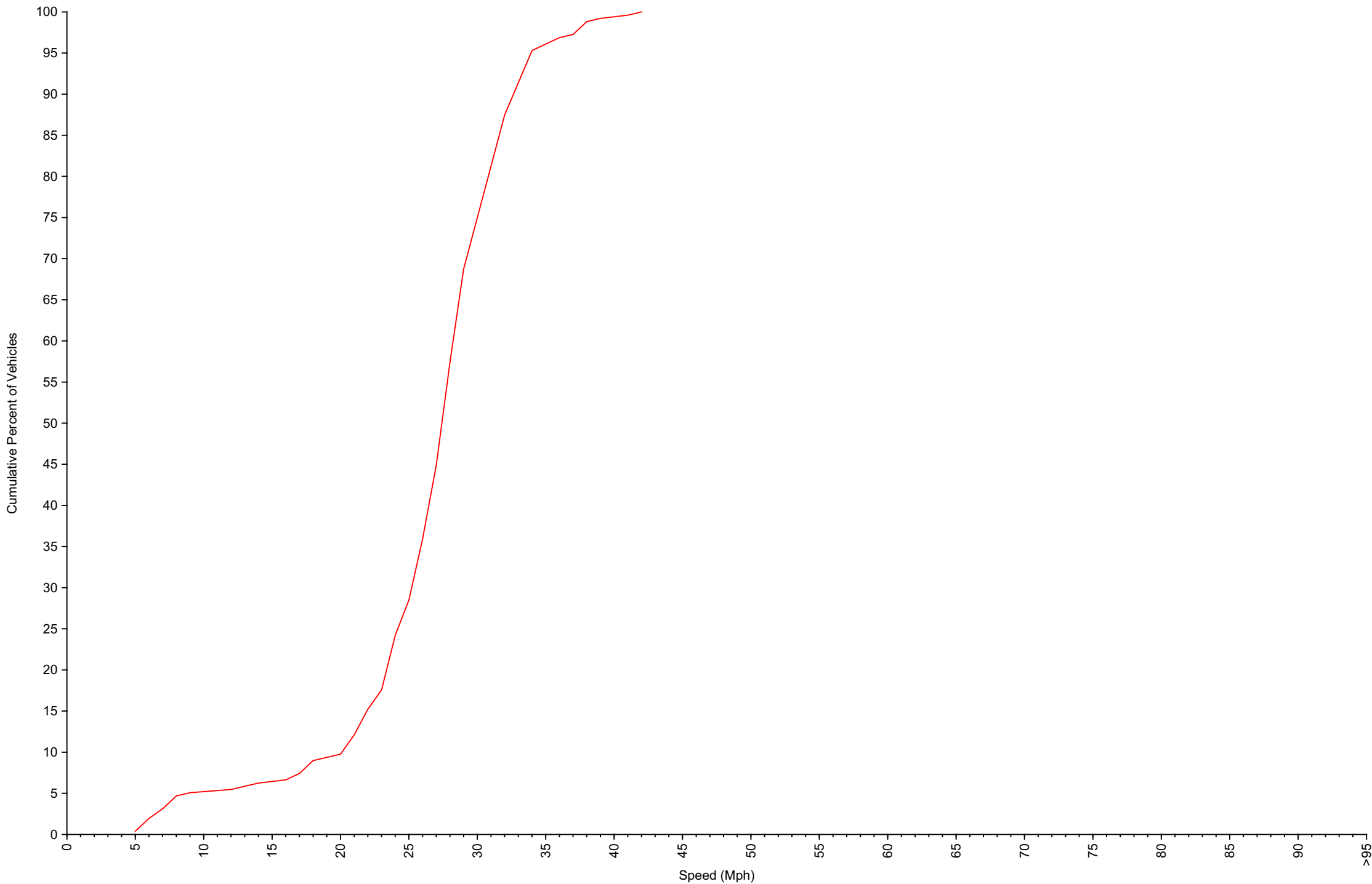
Cumulative Speed Distribution Curve Daily Overview for Sun Aug 18 2024
