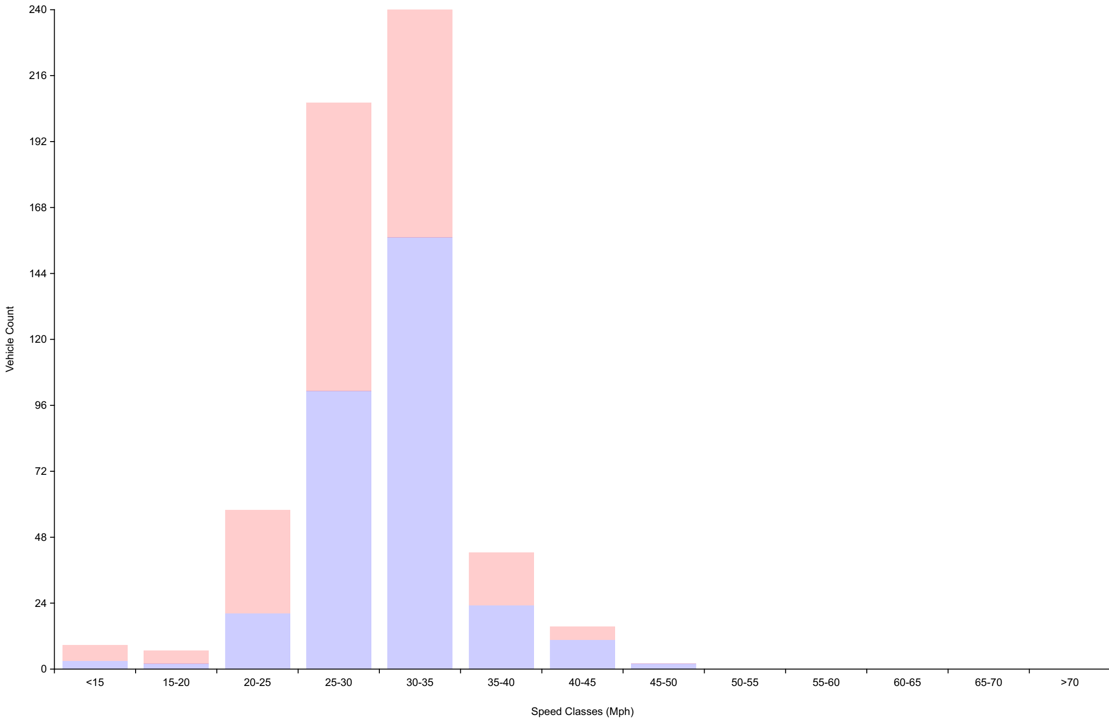
Vehicle Counts By Speed Class Daily Overview for Mon Aug 5 2024
