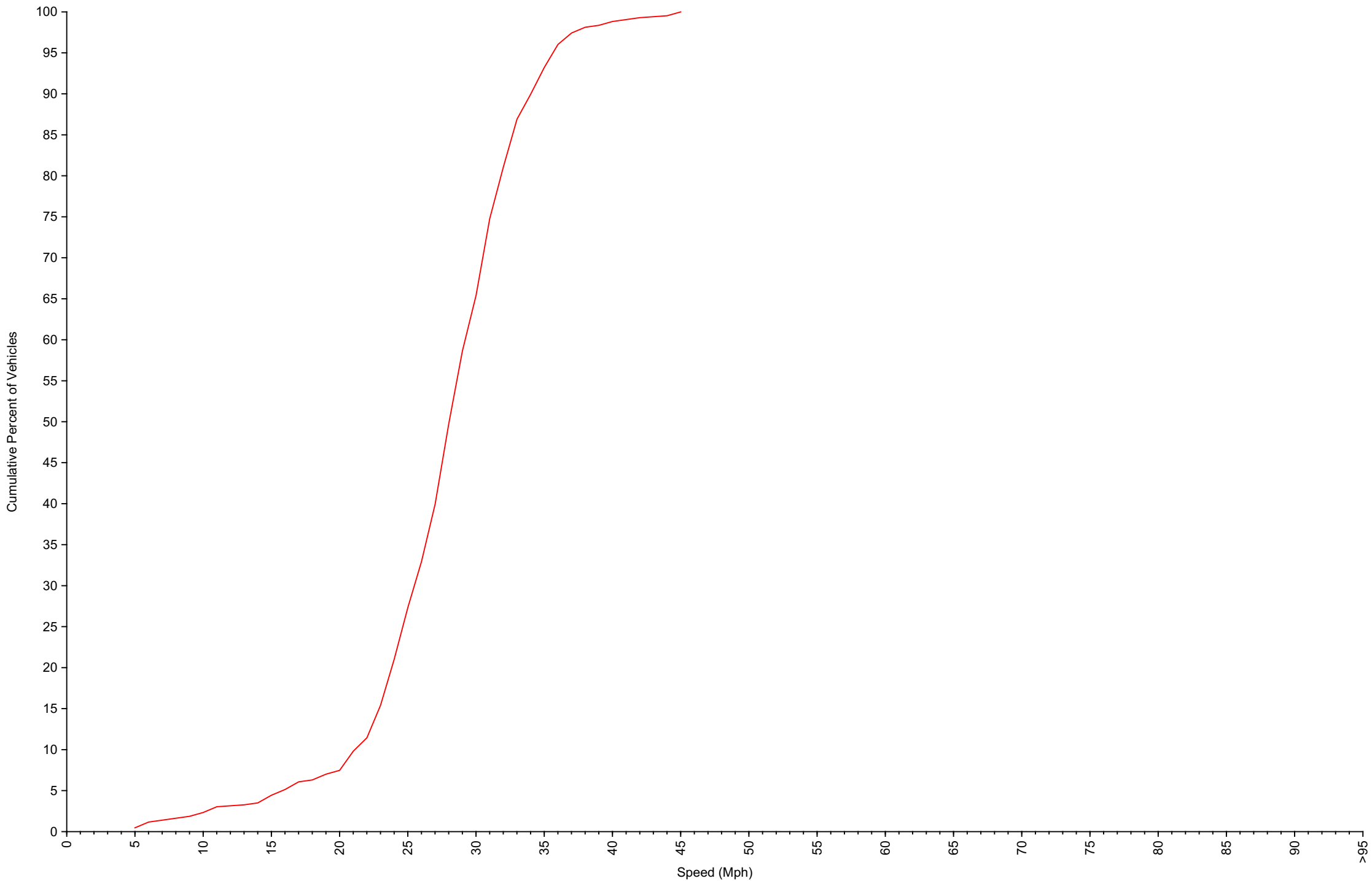
Cumulative Speed Distribution Curve Daily Overview for Tue Aug 6 2024
