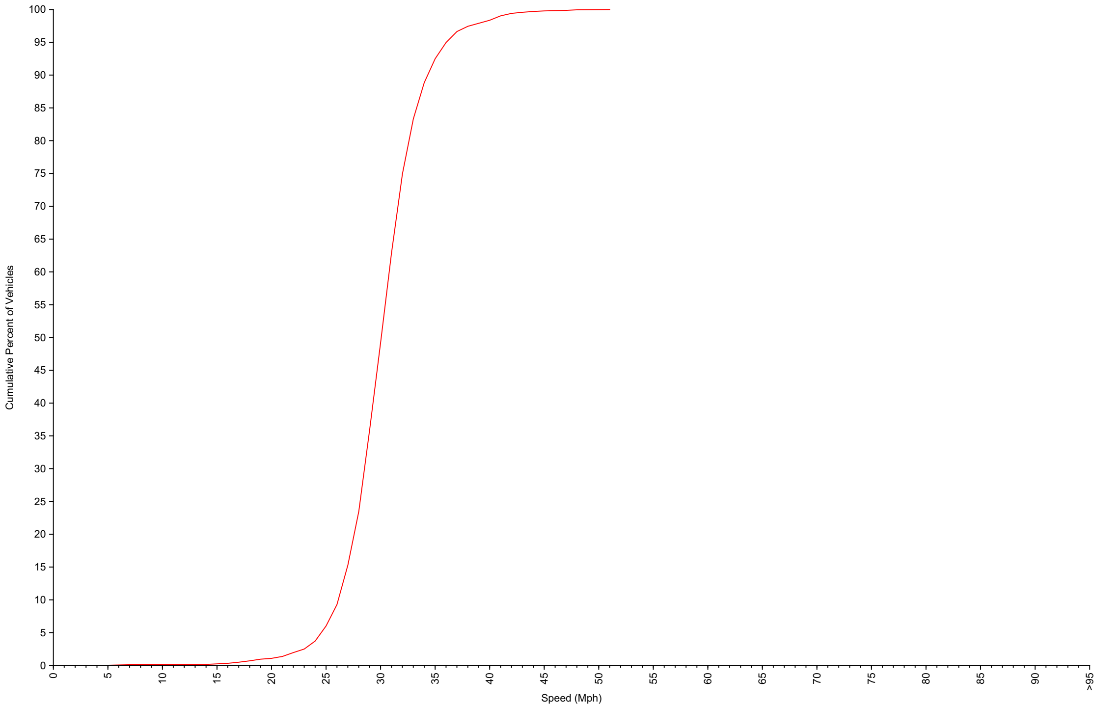
Cumulative Speed Distribution Curve Daily Overview for Thu Apr 10 2025
