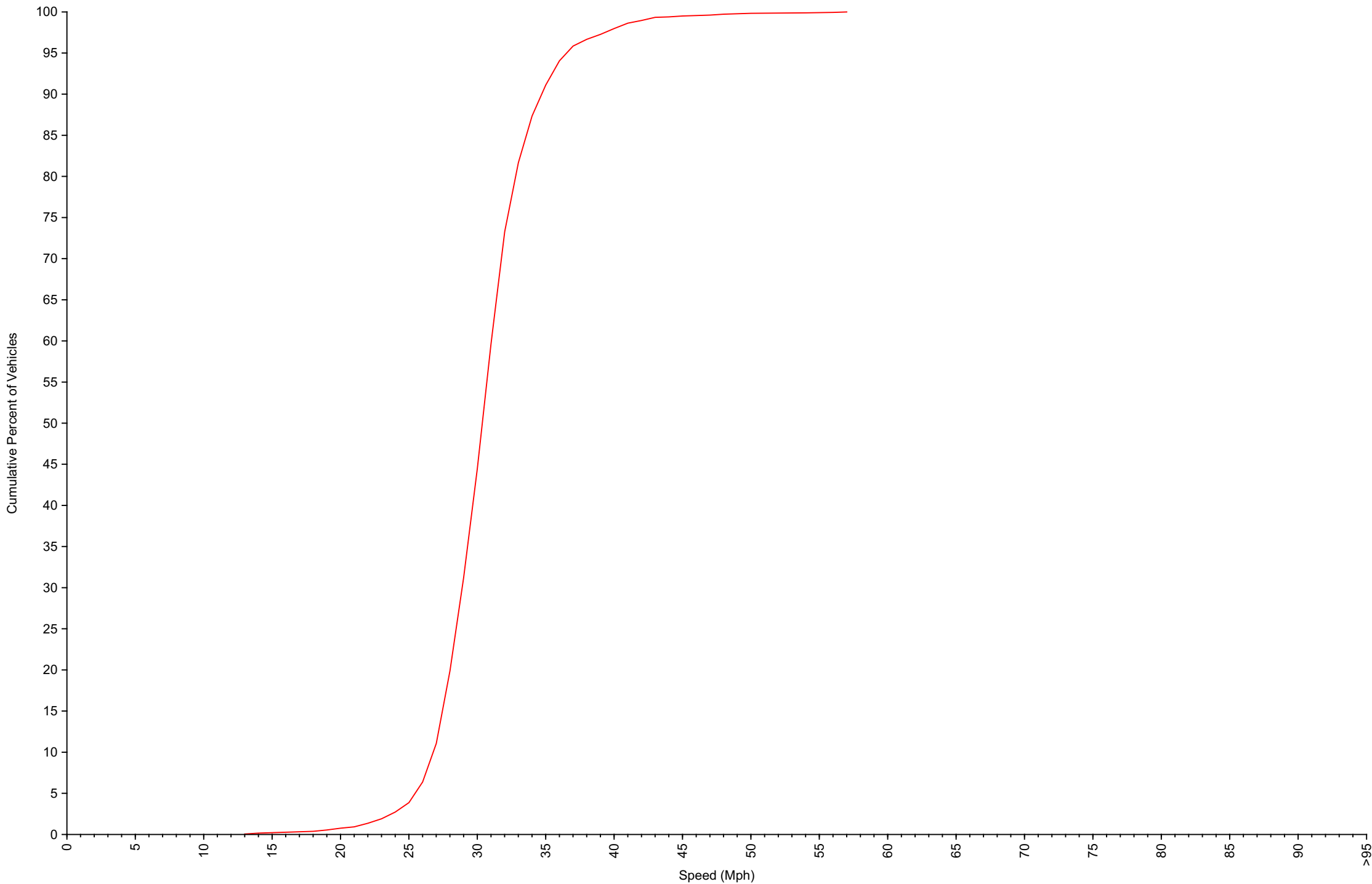
Cumulative Speed Distribution Curve Daily Overview for Fri Apr 18 2025
