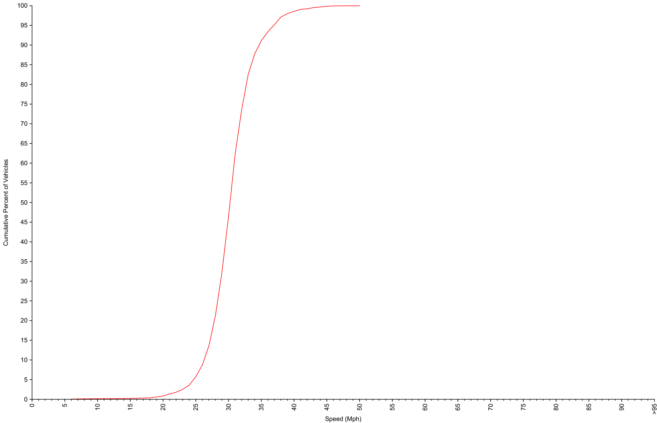
Cumulative Speed Distribution Curve Daily Overview for Mon Apr 14 2025
