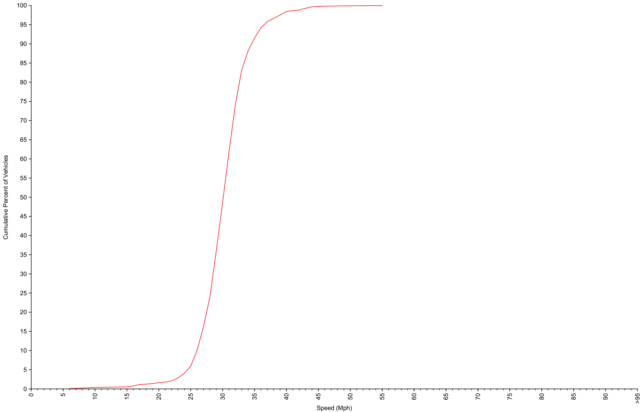
Cumulative Speed Distribution Curve Daily Overview for Sun Apr 20 2025
