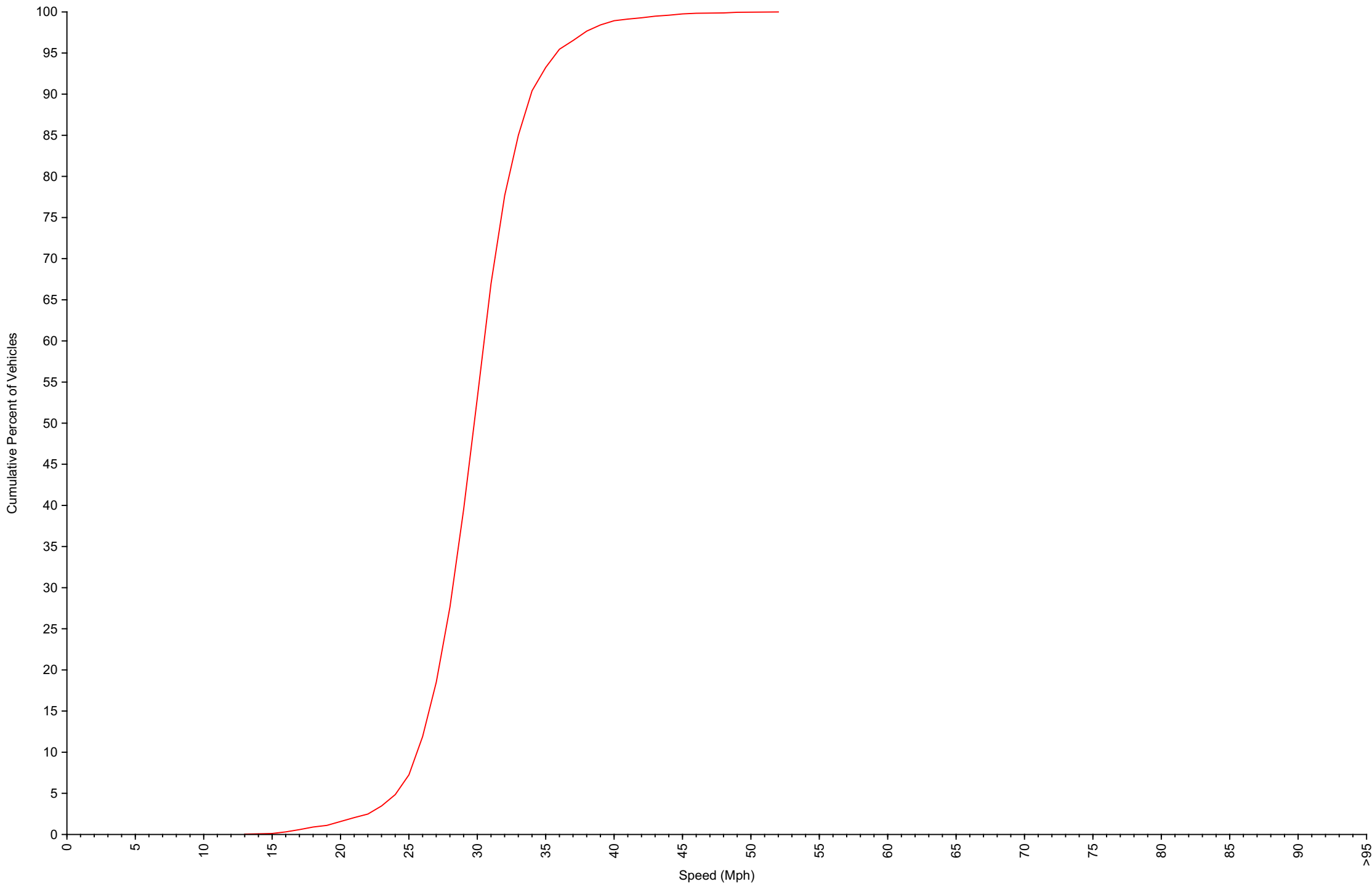
Cumulative Speed Distribution Curve Daily Overview for Wed Apr 2 2025
