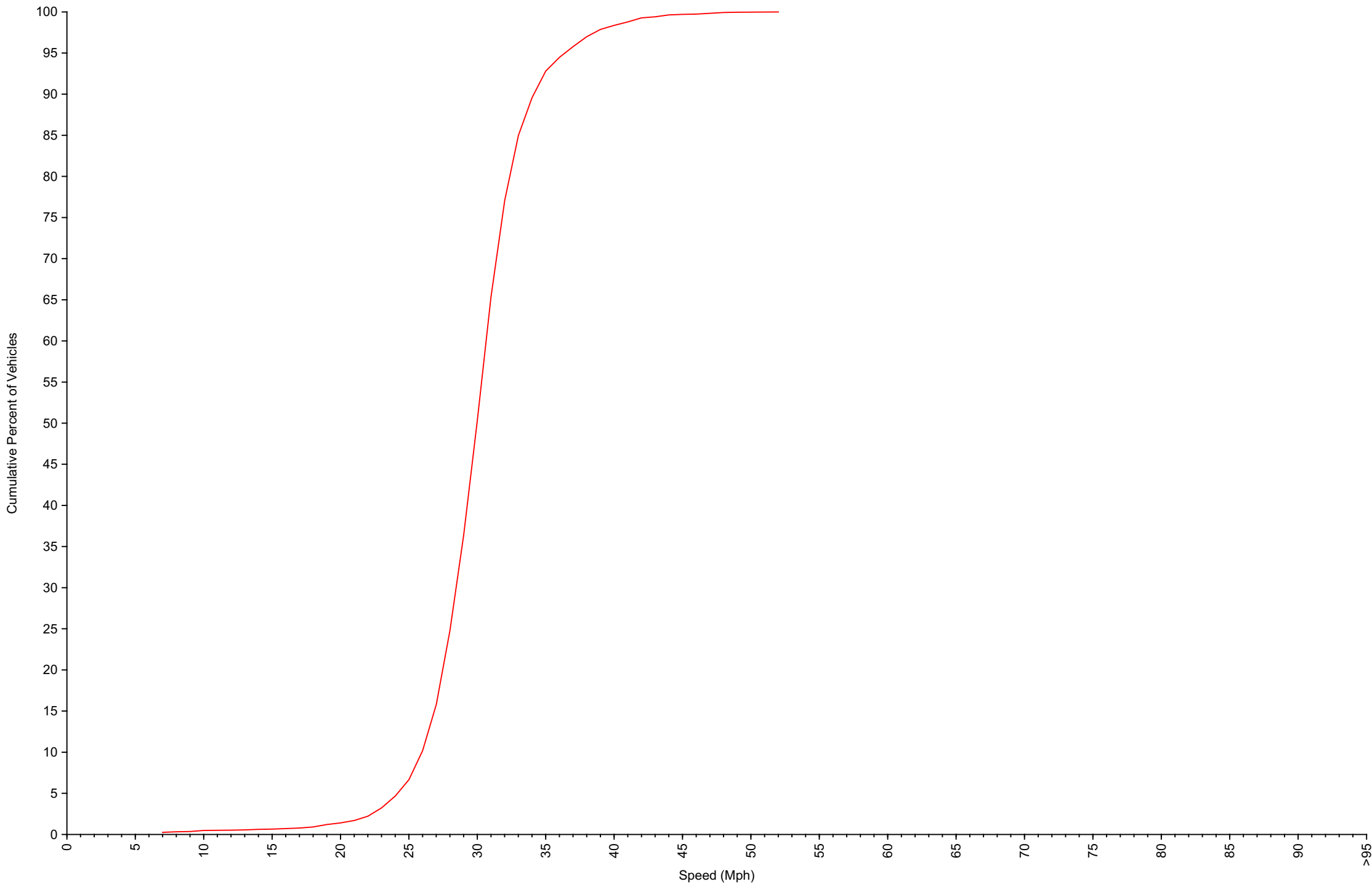
Cumulative Speed Distribution Curve Daily Overview for Fri Apr 4 2025
