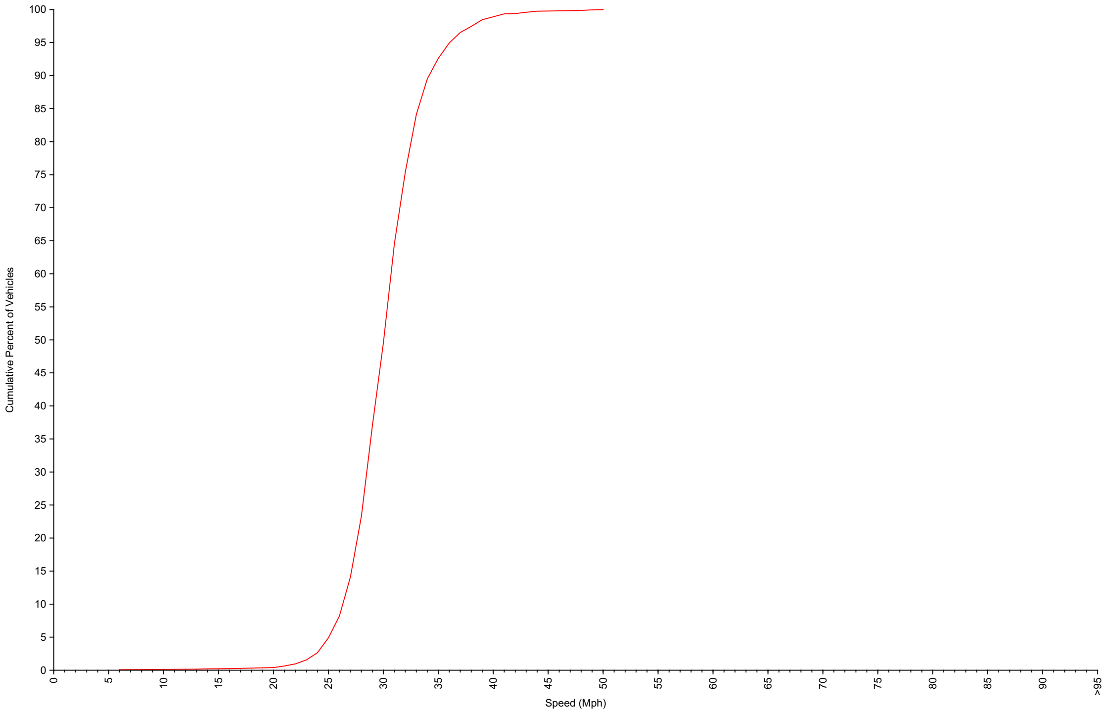
Cumulative Speed Distribution Curve Daily Overview for Wed Apr 23 2025
