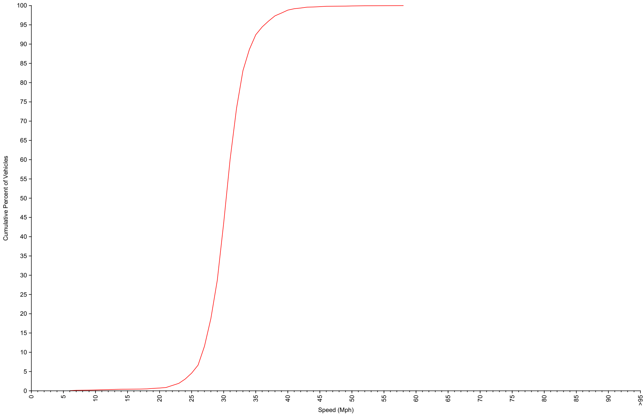
Cumulative Speed Distribution Curve Daily Overview for Tue Apr 15 2025
