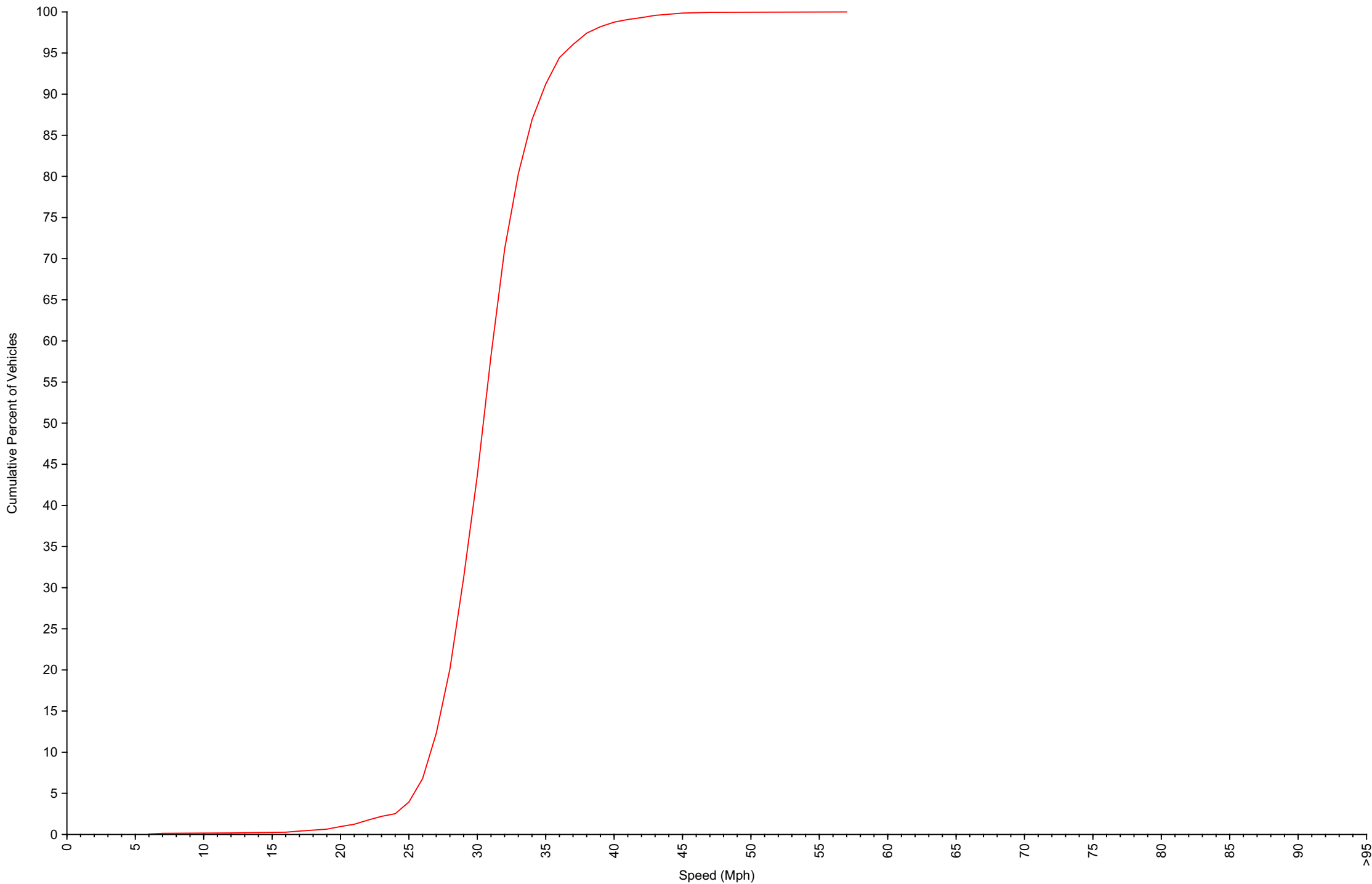
Cumulative Speed Distribution Curve Daily Overview for Wed Apr 16 2025
