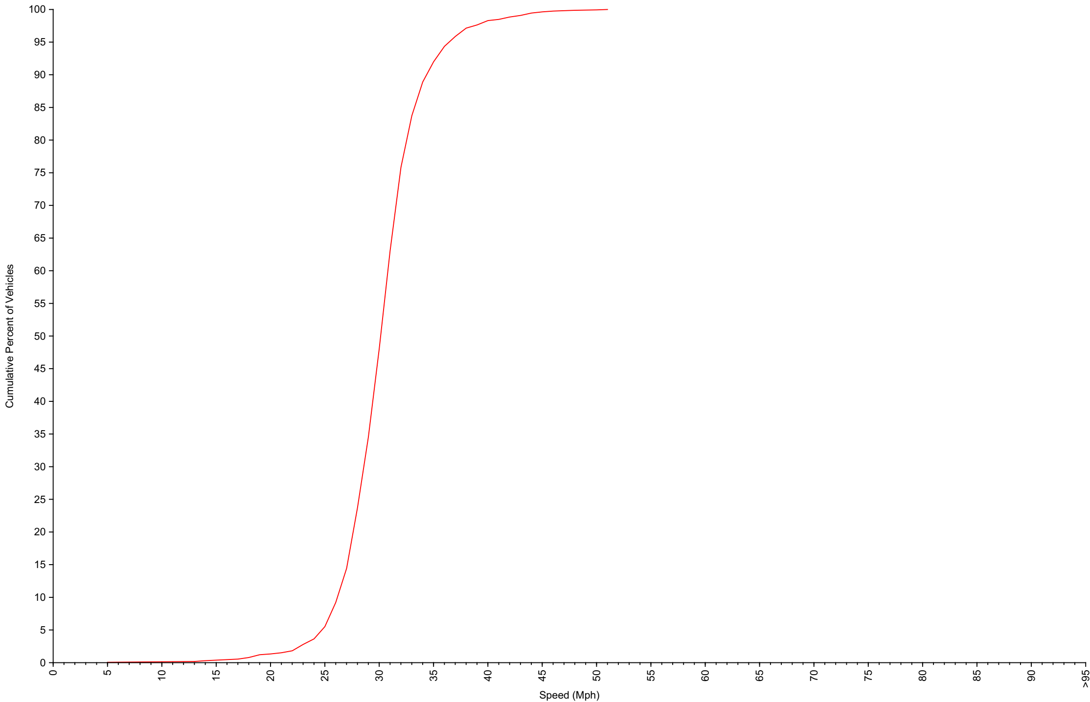
Cumulative Speed Distribution Curve Daily Overview for Sat Apr 19 2025
