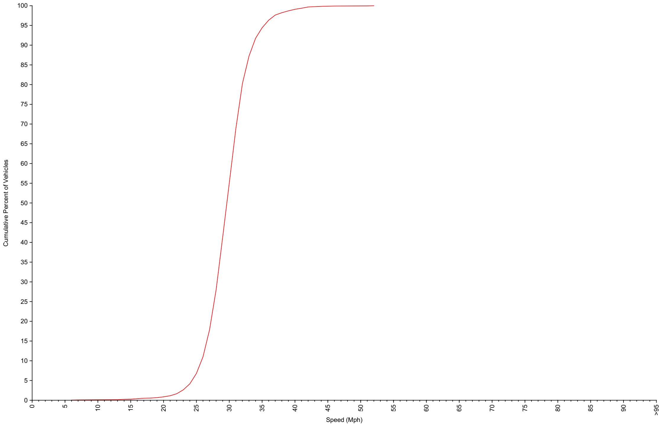
Cumulative Speed Distribution Curve Daily Overview for Fri Apr 25 2025
