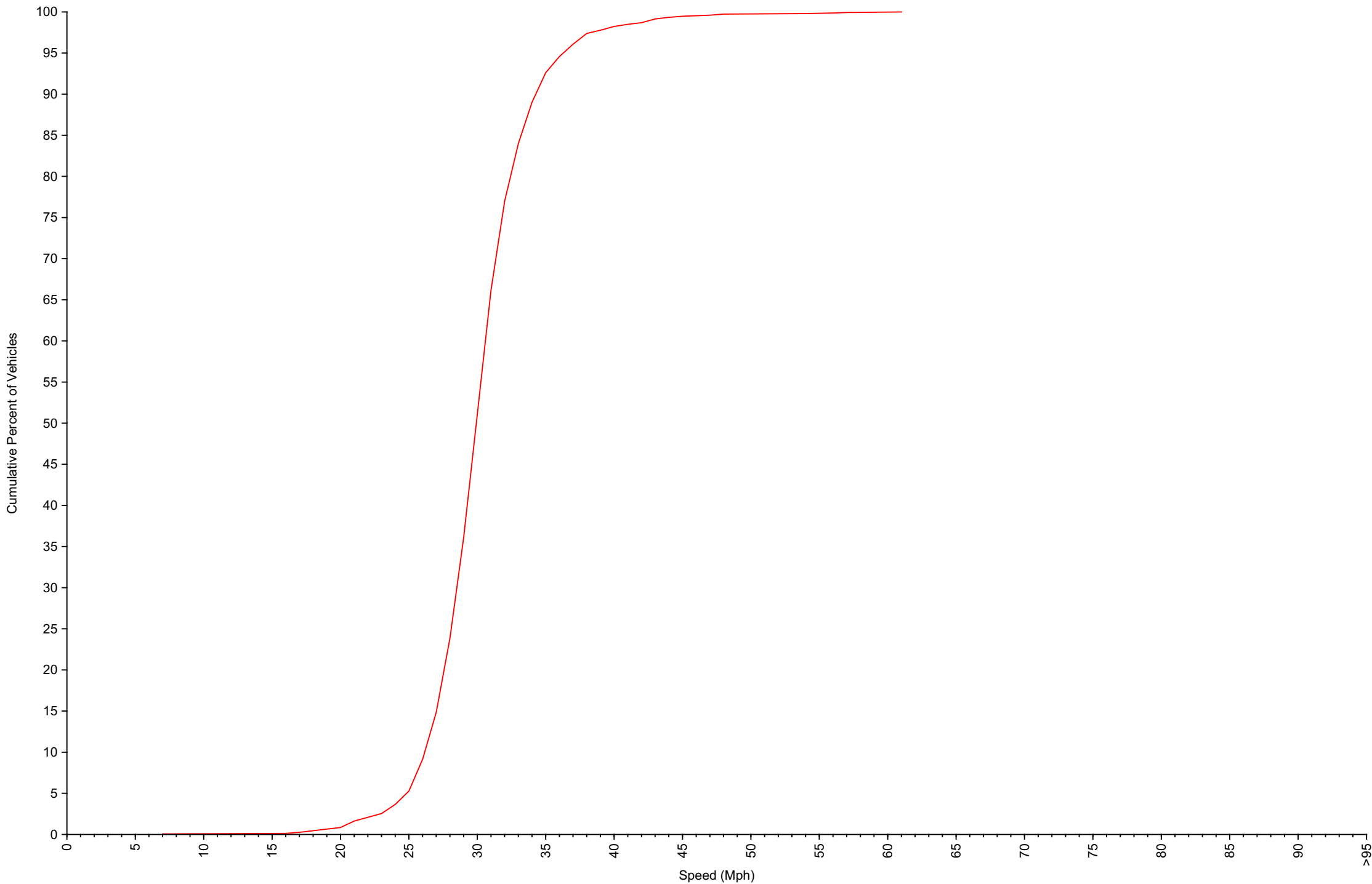
Cumulative Speed Distribution Curve Daily Overview for Sun May 11 2025
