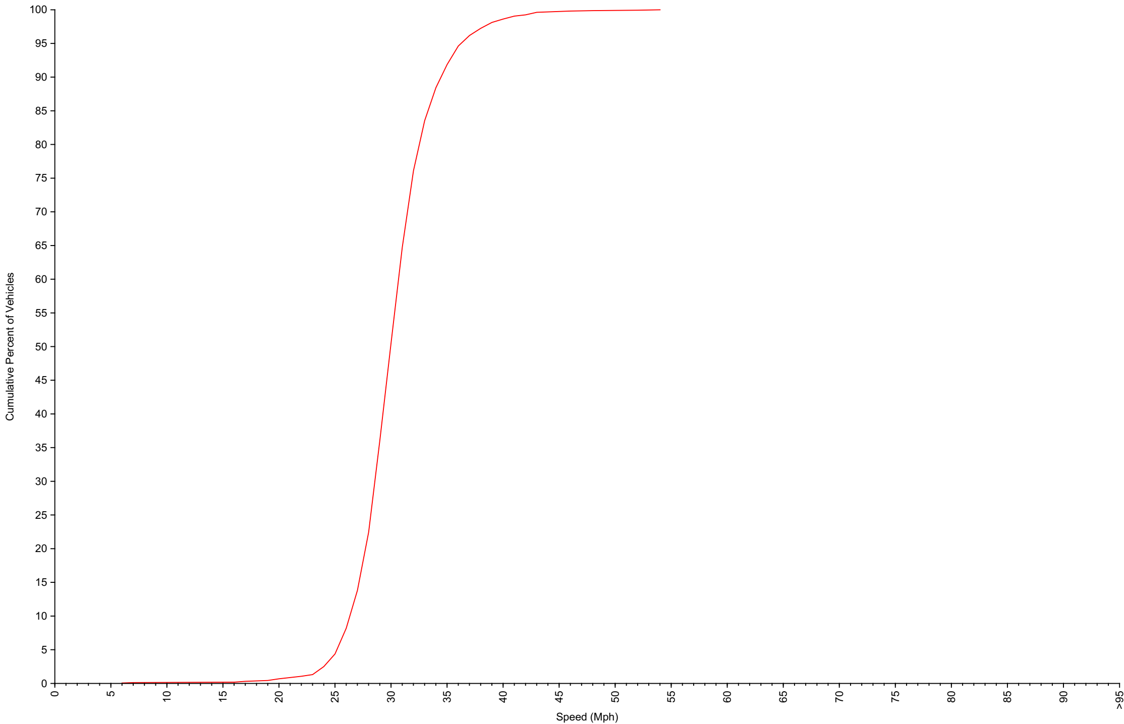
Cumulative Speed Distribution Curve Daily Overview for Sun May 18 2025
