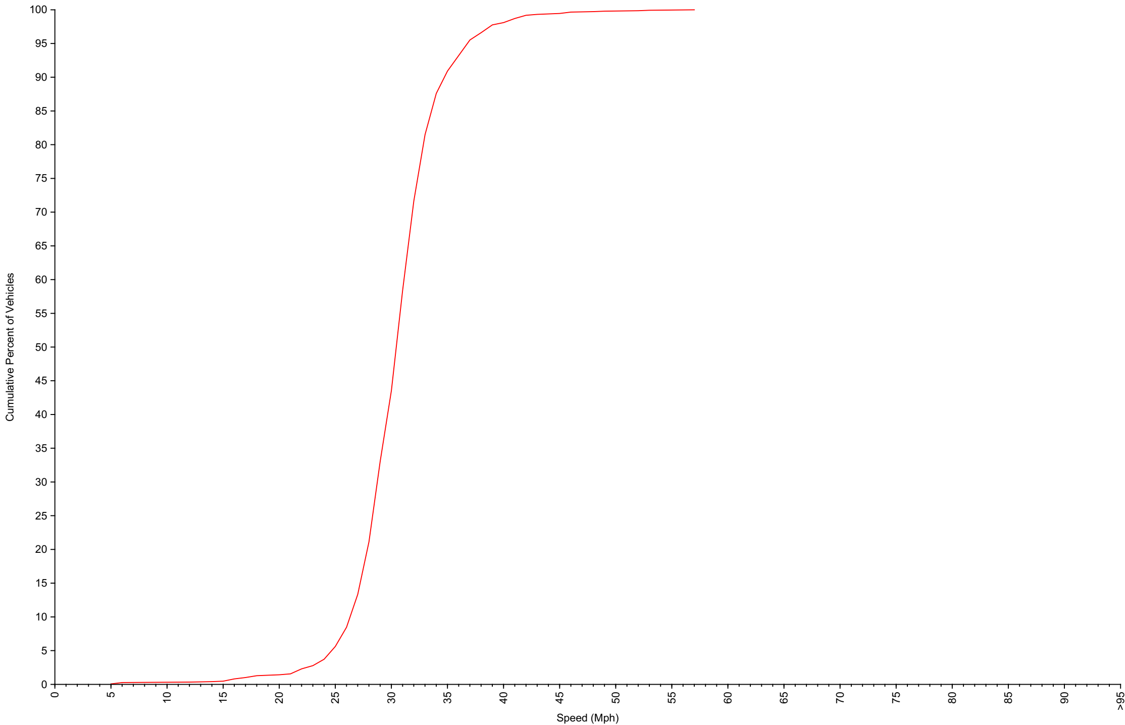
Cumulative Speed Distribution Curve Daily Overview for Mon May 5 2025
