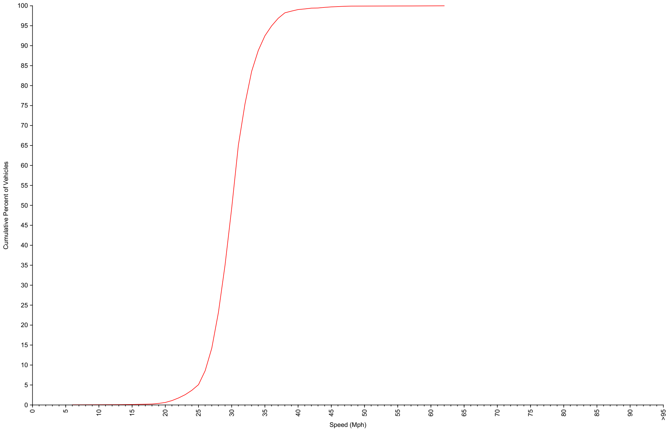
Cumulative Speed Distribution Curve Daily Overview for Thu May 1 2025
