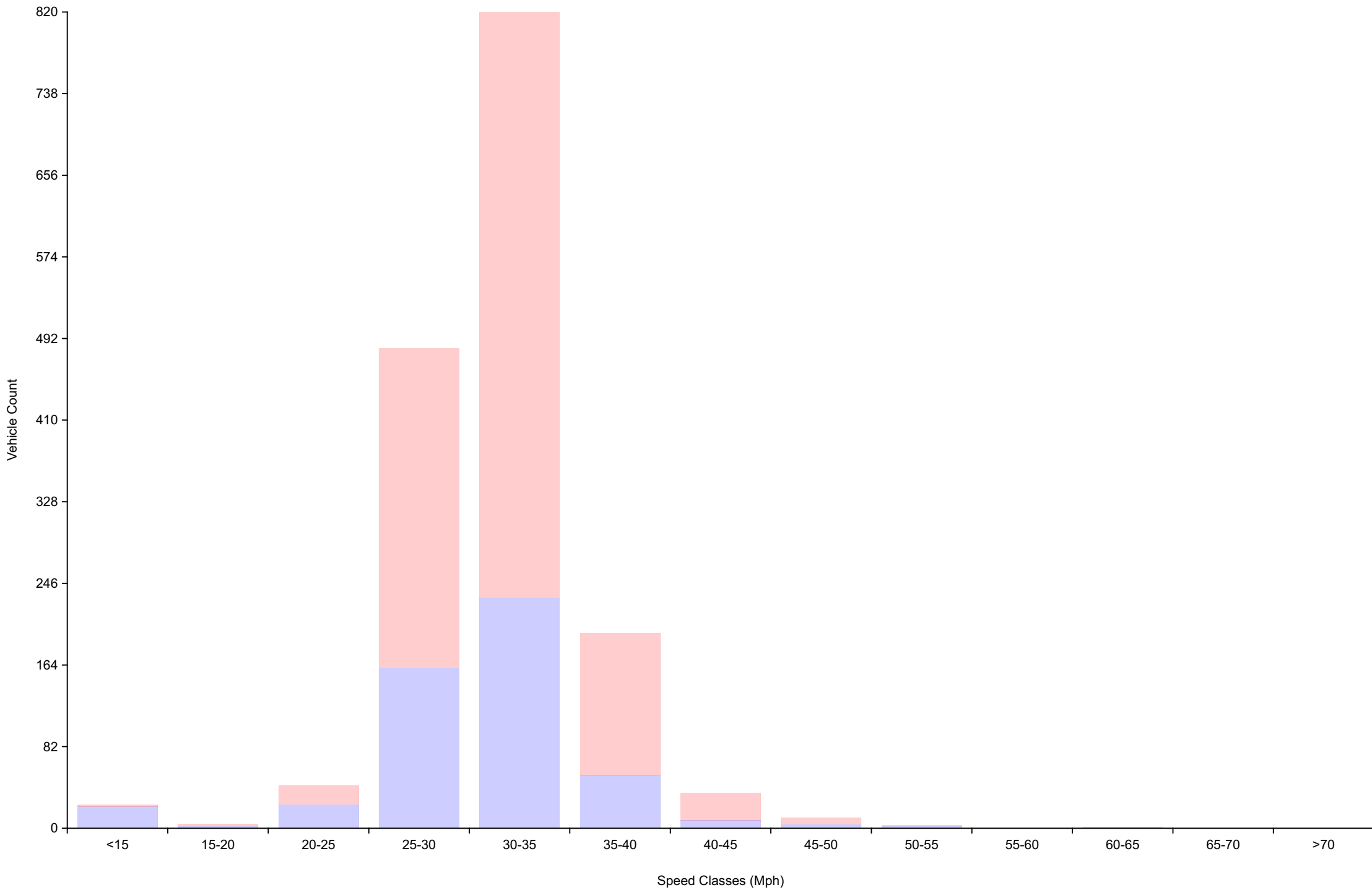
Vehicle Counts By Speed Class Daily Overview for Sat May 24 2025
