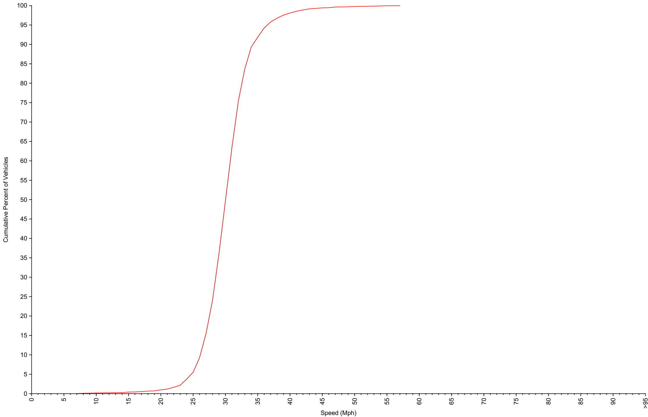
Cumulative Speed Distribution Curve Daily Overview for Wed May 21 2025
