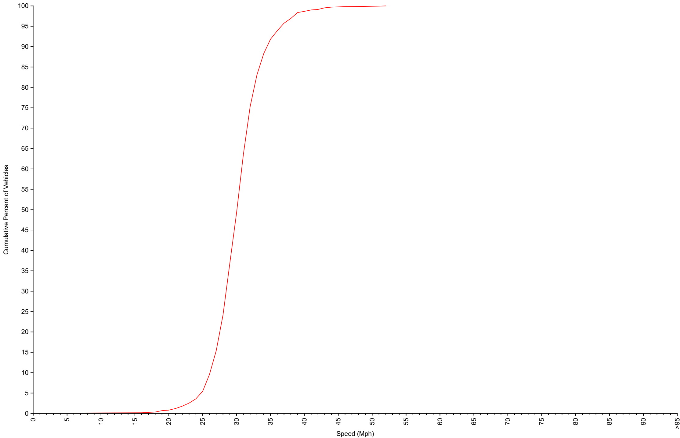
Cumulative Speed Distribution Curve Daily Overview for Sat May 10 2025
