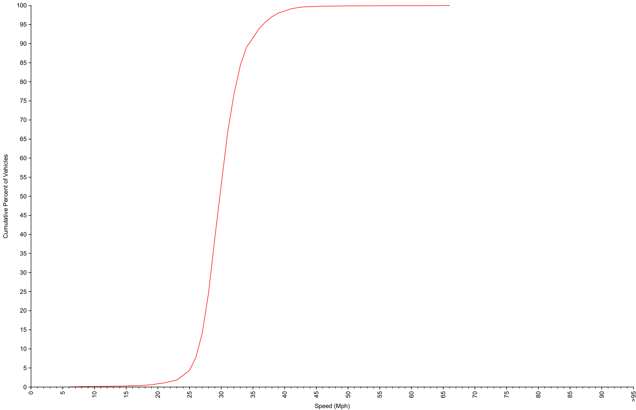
Cumulative Speed Distribution Curve Daily Overview for Thu May 22 2025
