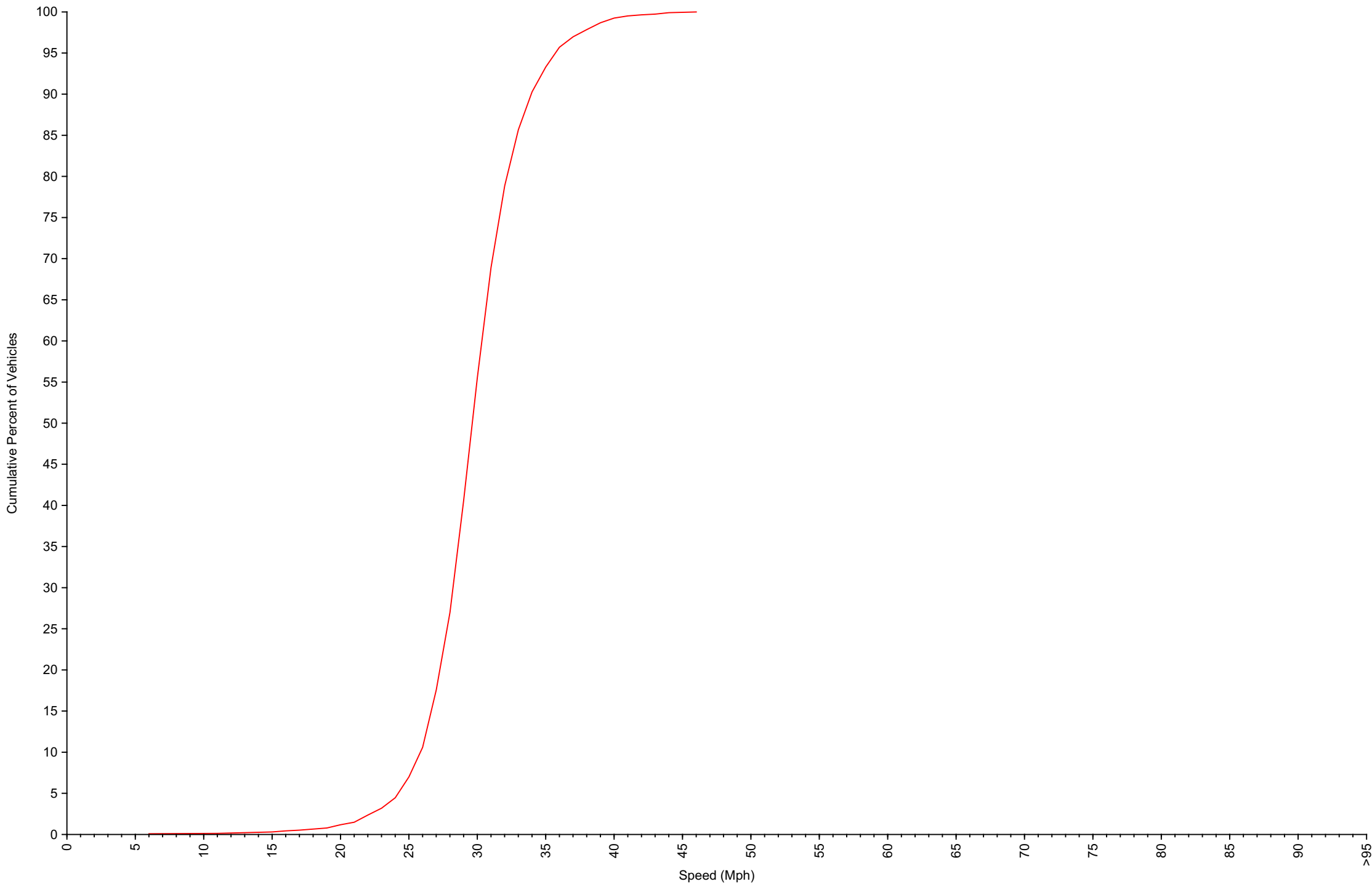
Cumulative Speed Distribution Curve Daily Overview for Tue May 6 2025
