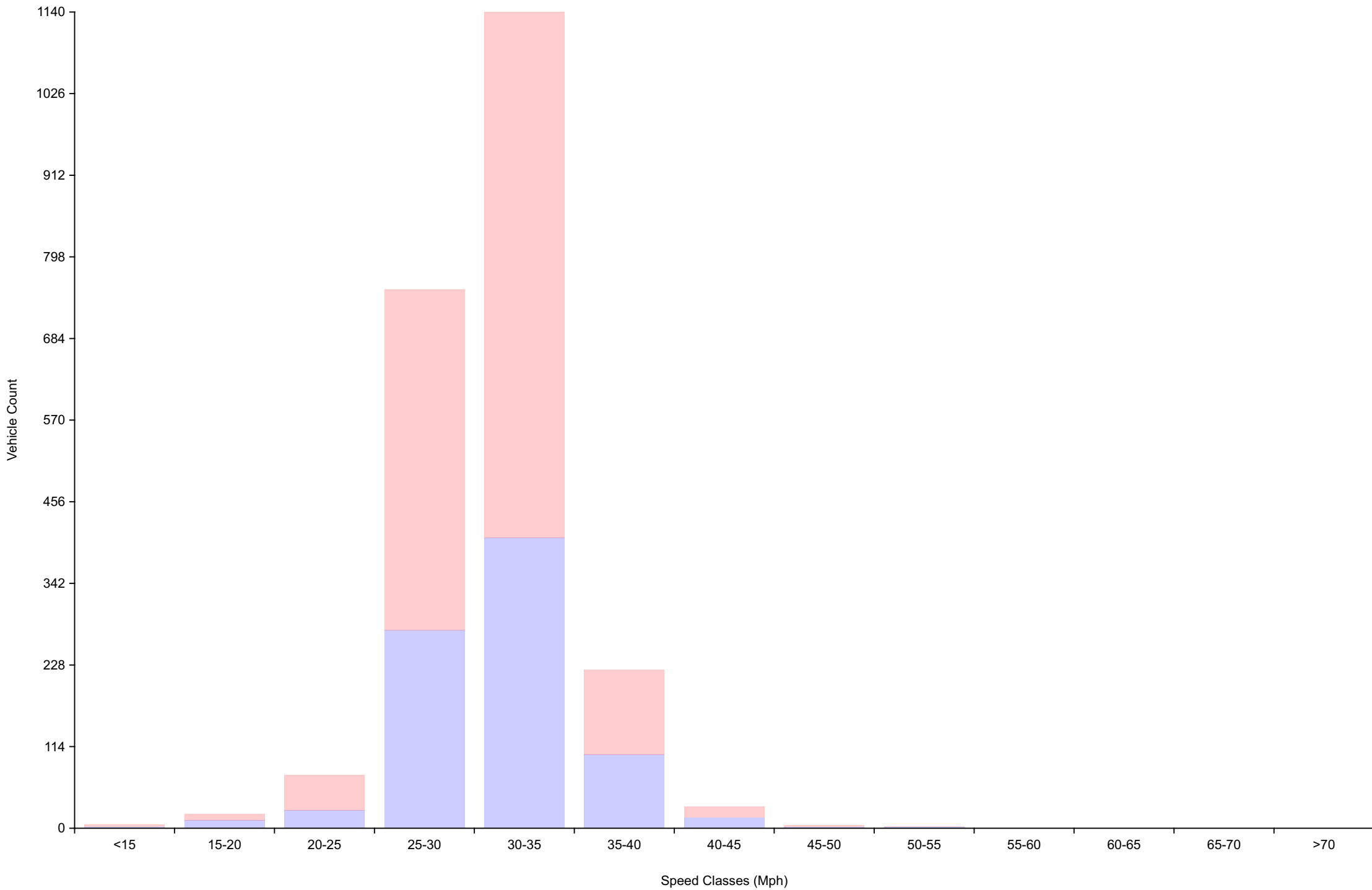
Vehicle Counts By Speed Class Daily Overview for Tue May 20 2025
