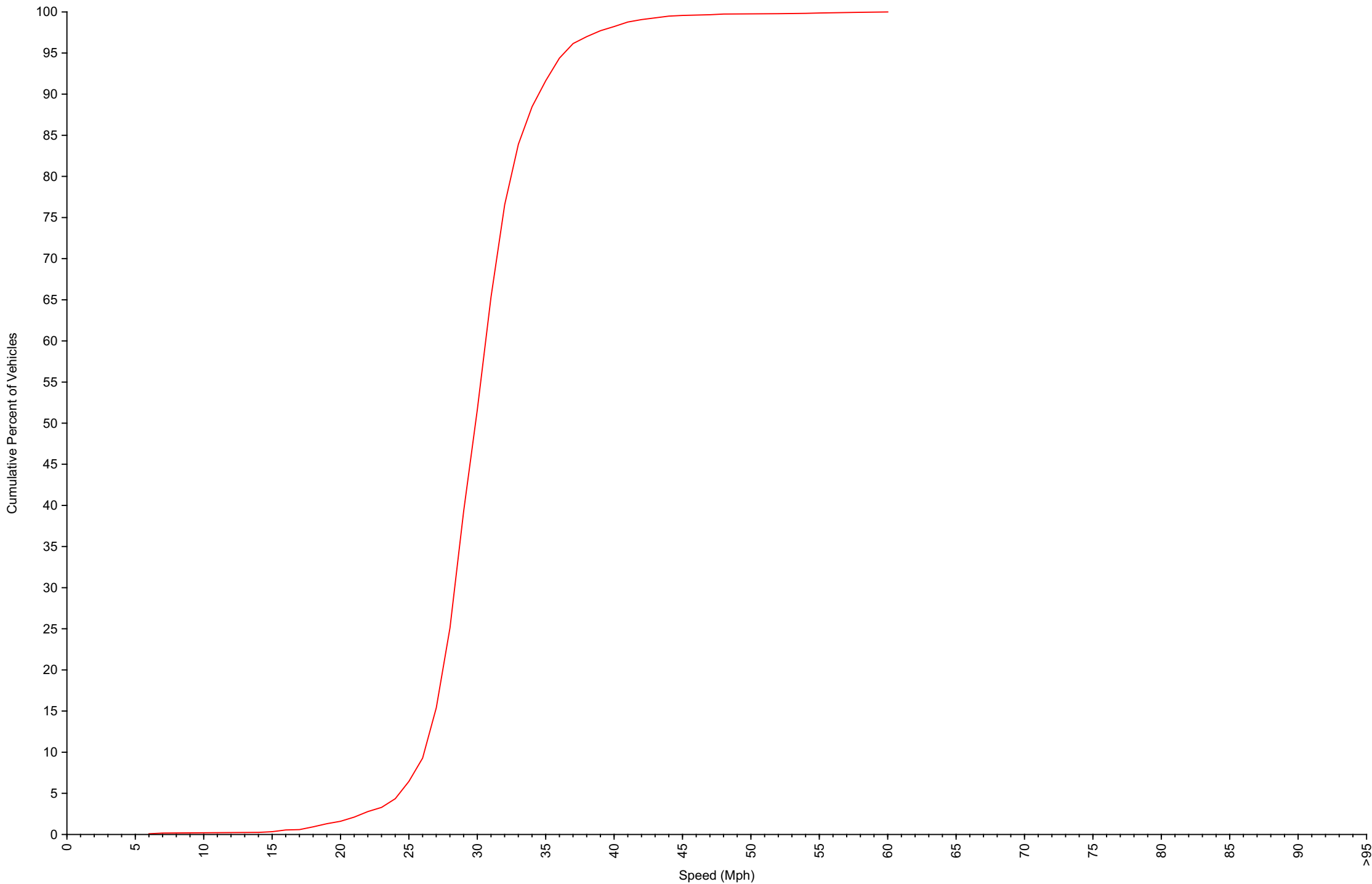
Cumulative Speed Distribution Curve Daily Overview for Tue May 13 2025
