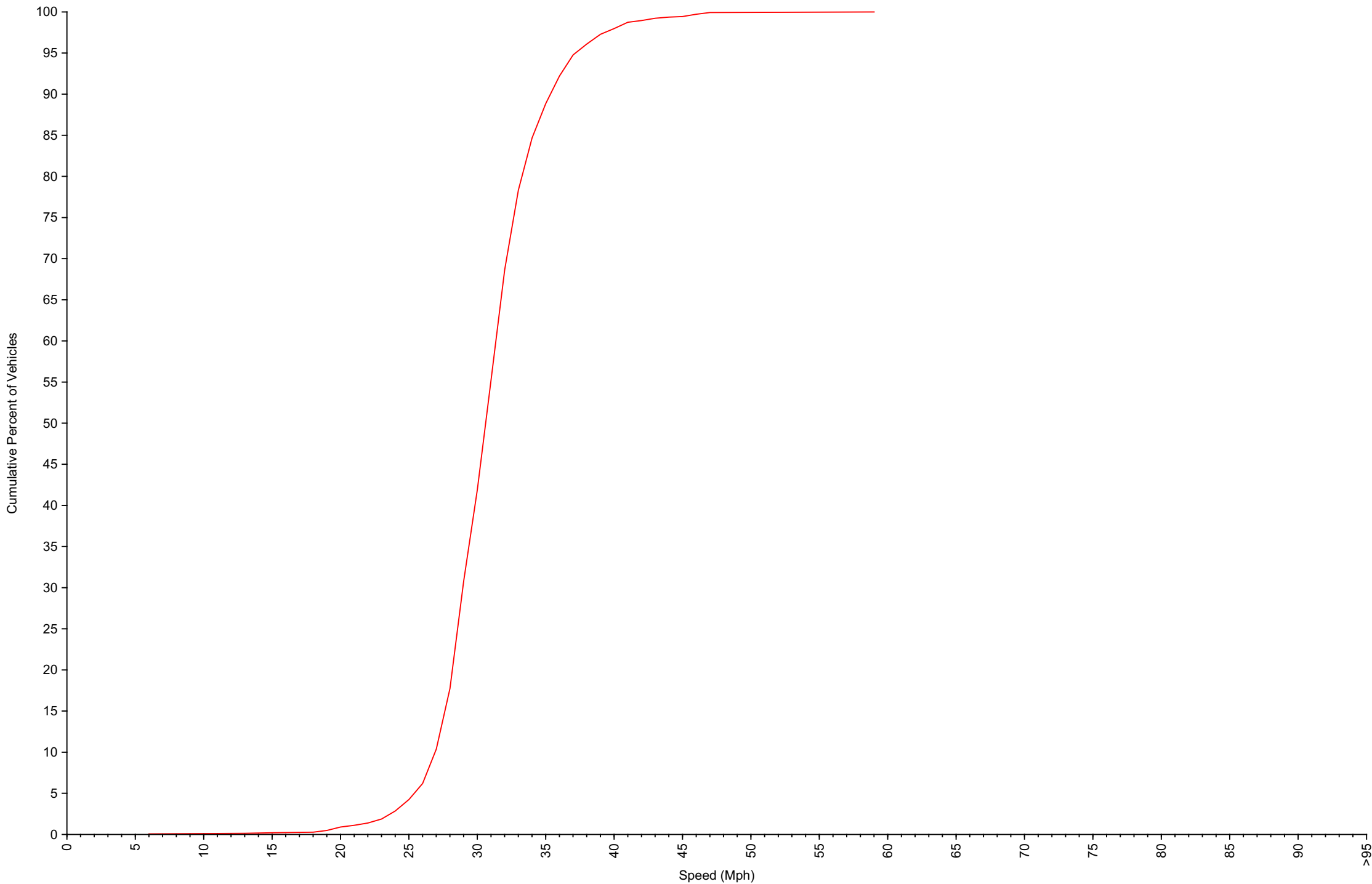
Cumulative Speed Distribution Curve Daily Overview for Sun May 4 2025
