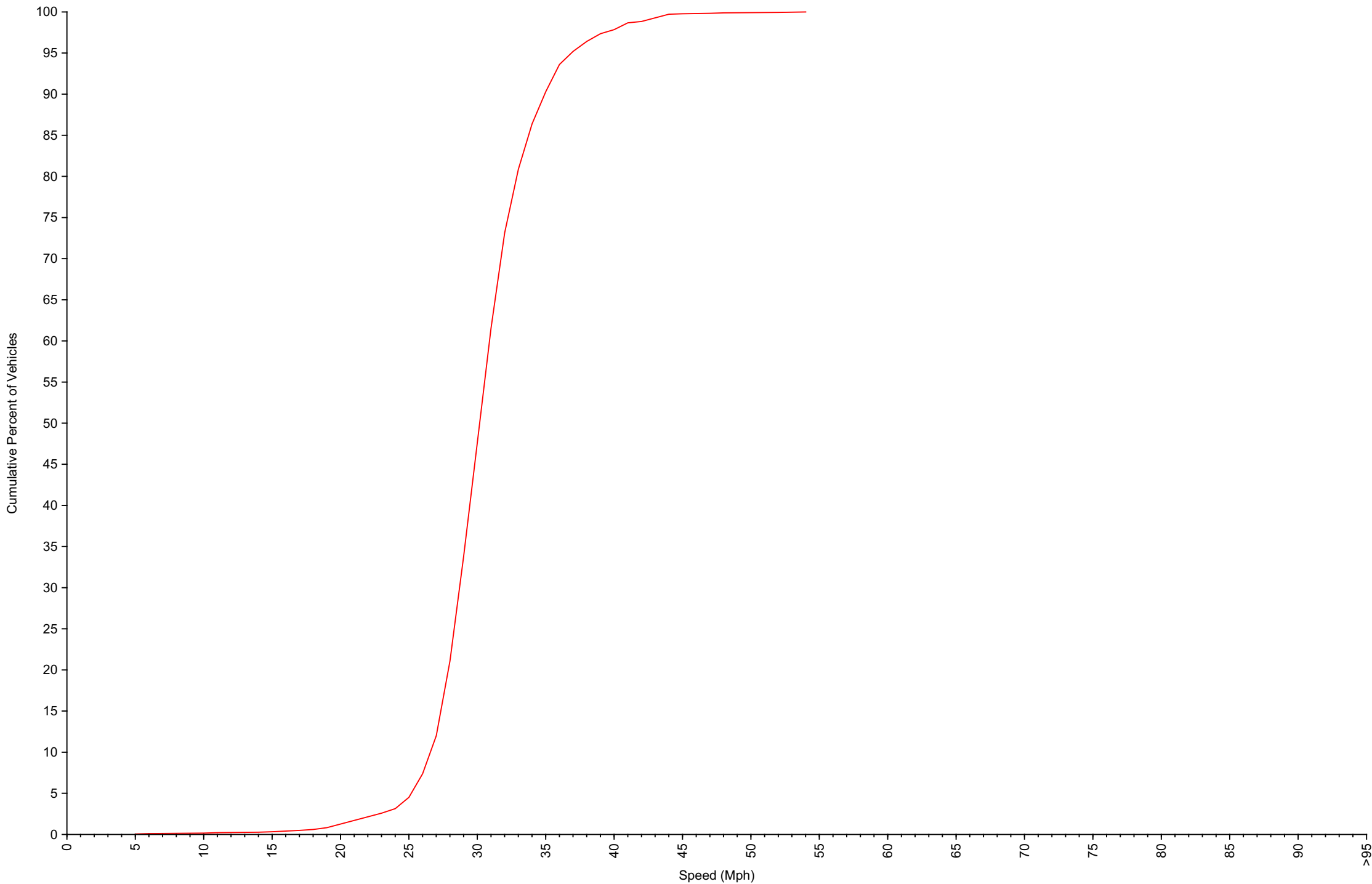
Cumulative Speed Distribution Curve Daily Overview for Wed May 28 2025
