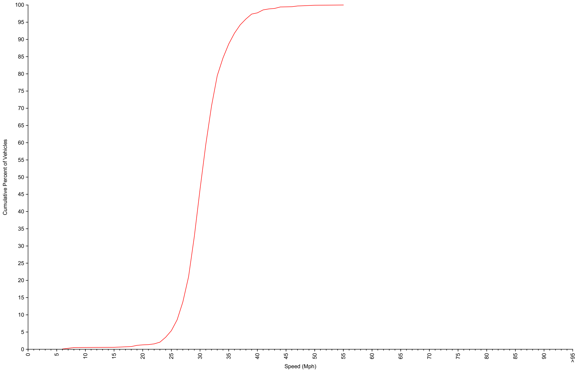
Cumulative Speed Distribution Curve Daily Overview for Mon May 26 2025
