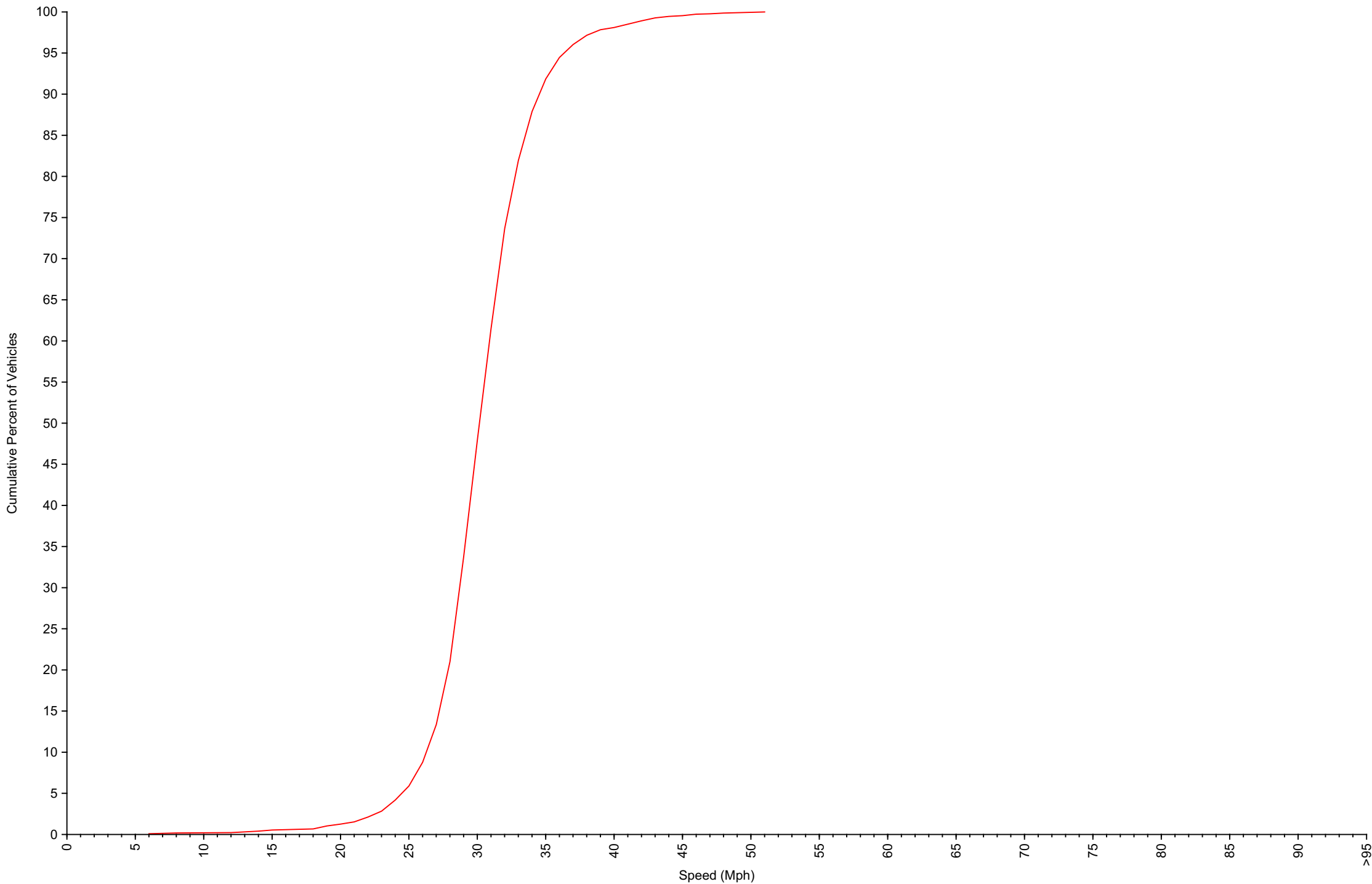
Cumulative Speed Distribution Curve Daily Overview for Thu May 29 2025
