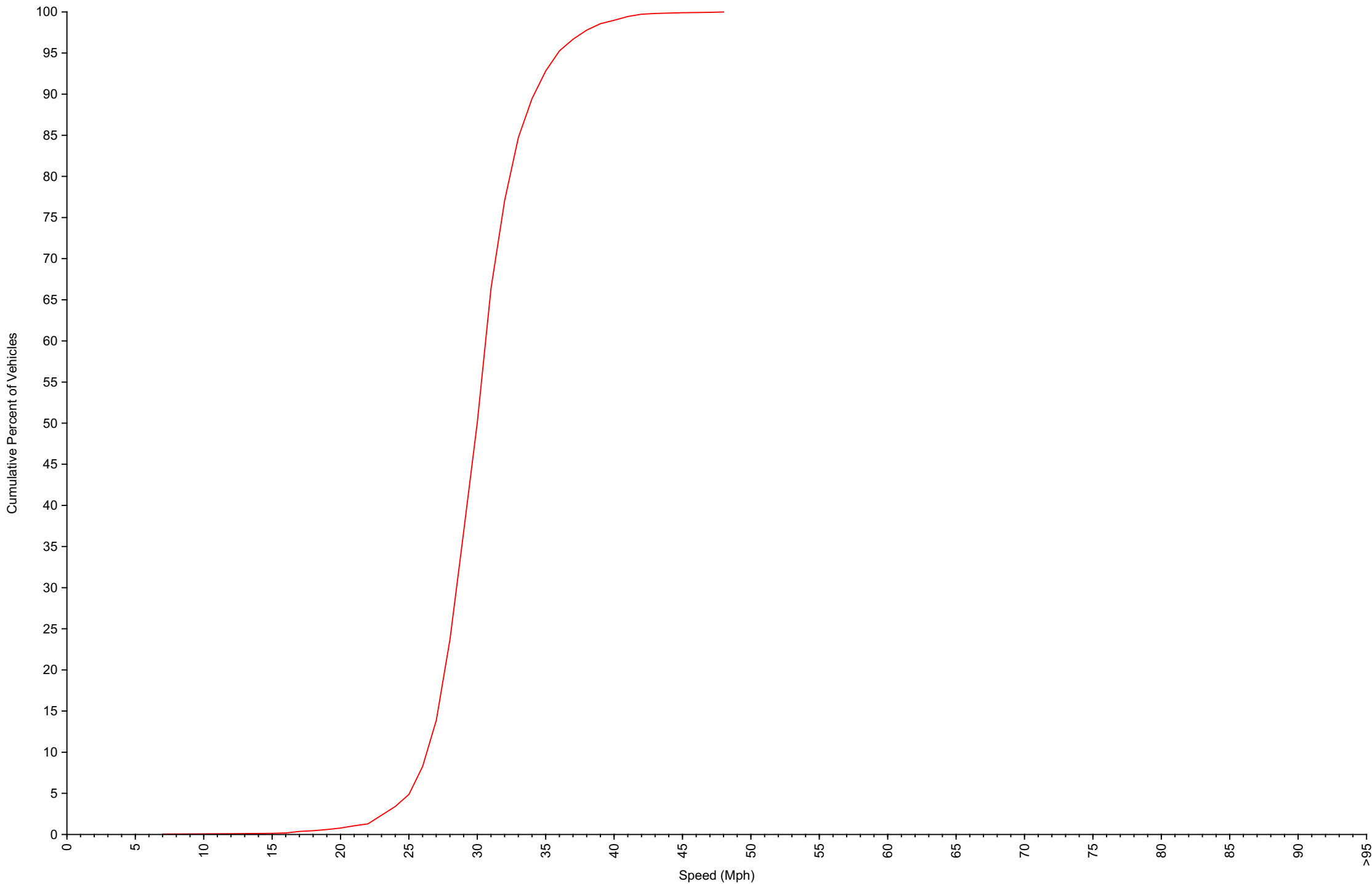
Cumulative Speed Distribution Curve Daily Overview for Mon May 19 2025
