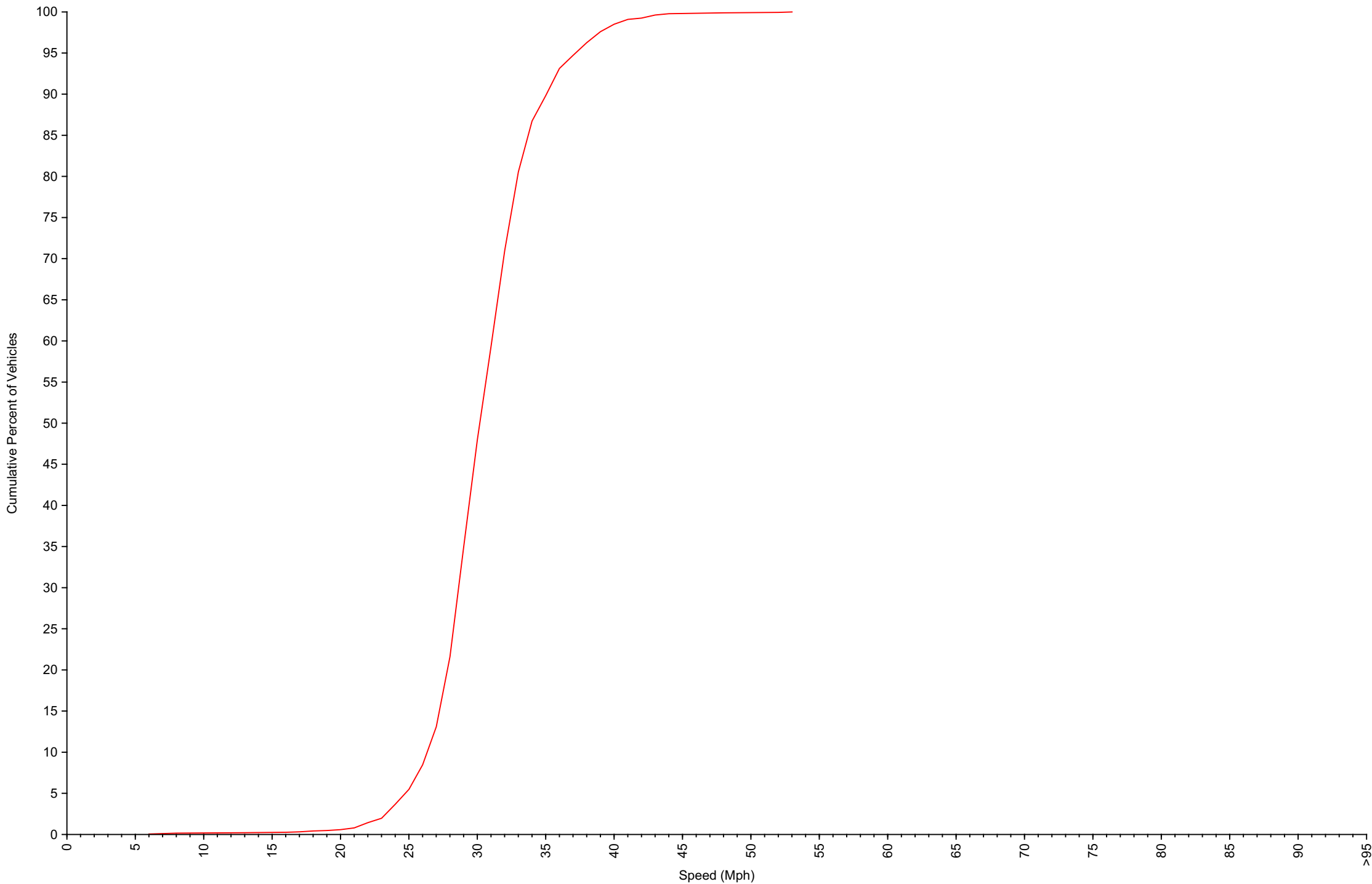
Cumulative Speed Distribution Curve Daily Overview for Tue May 27 2025
