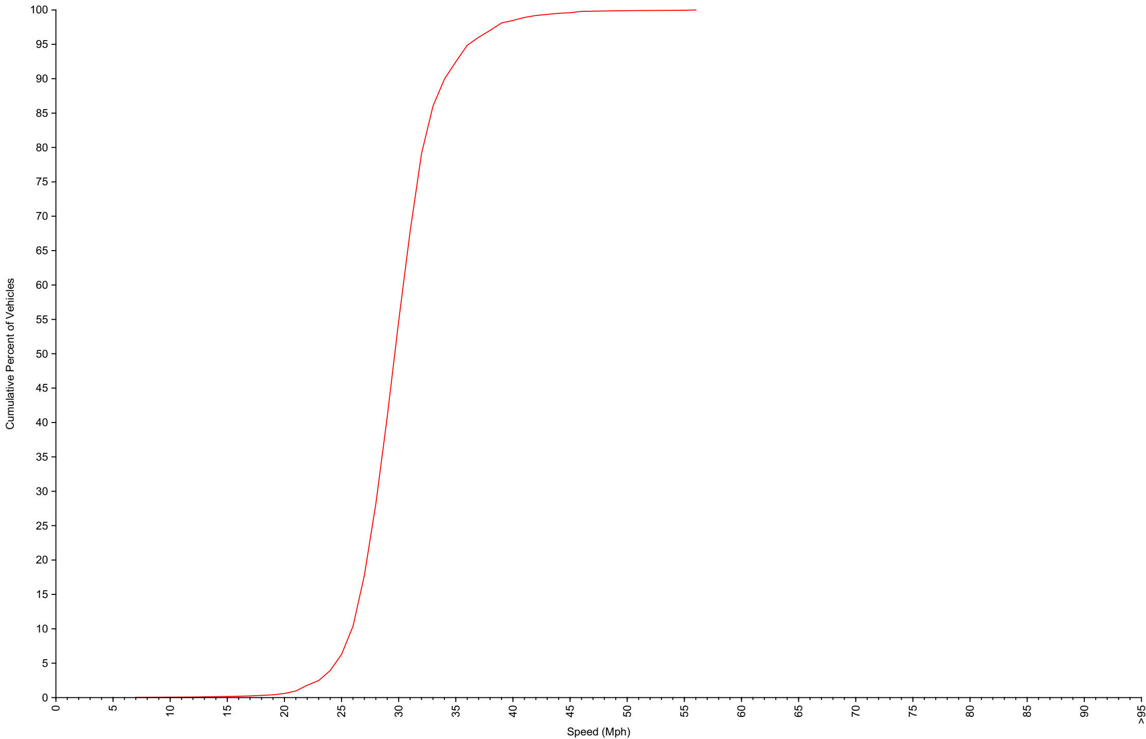
Cumulative Speed Distribution Curve Daily Overview for Fri May 16 2025
