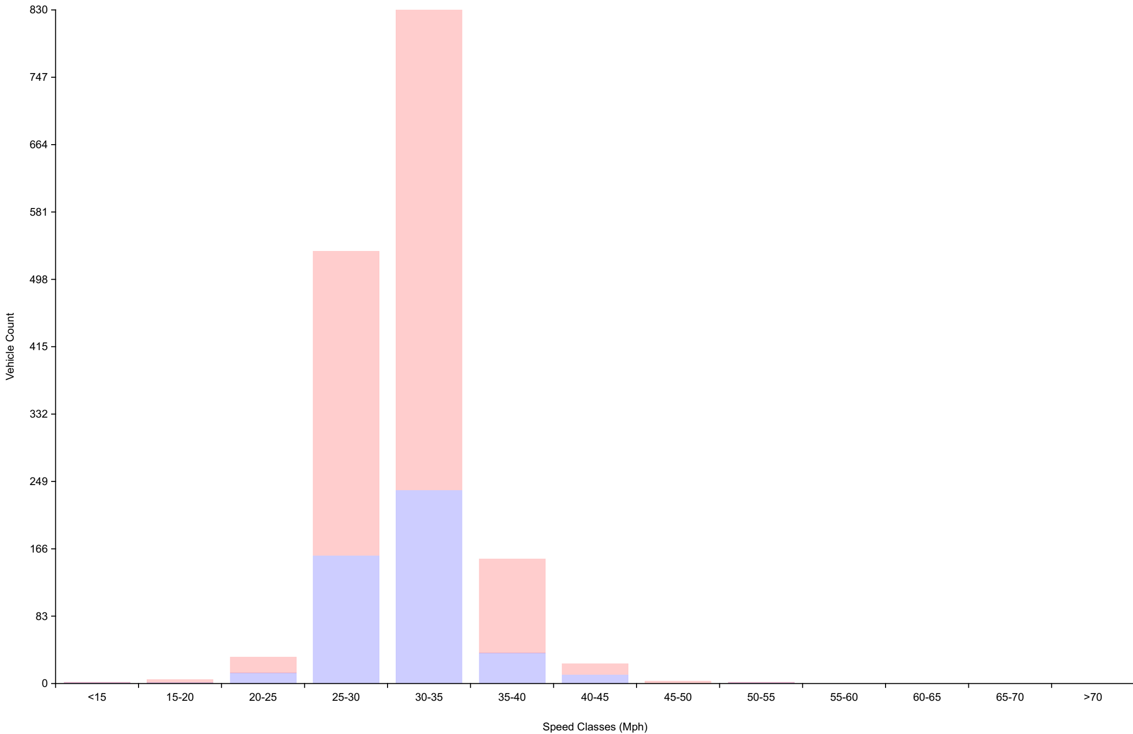
Vehicle Counts By Speed Class Daily Overview for Sun May 18 2025
