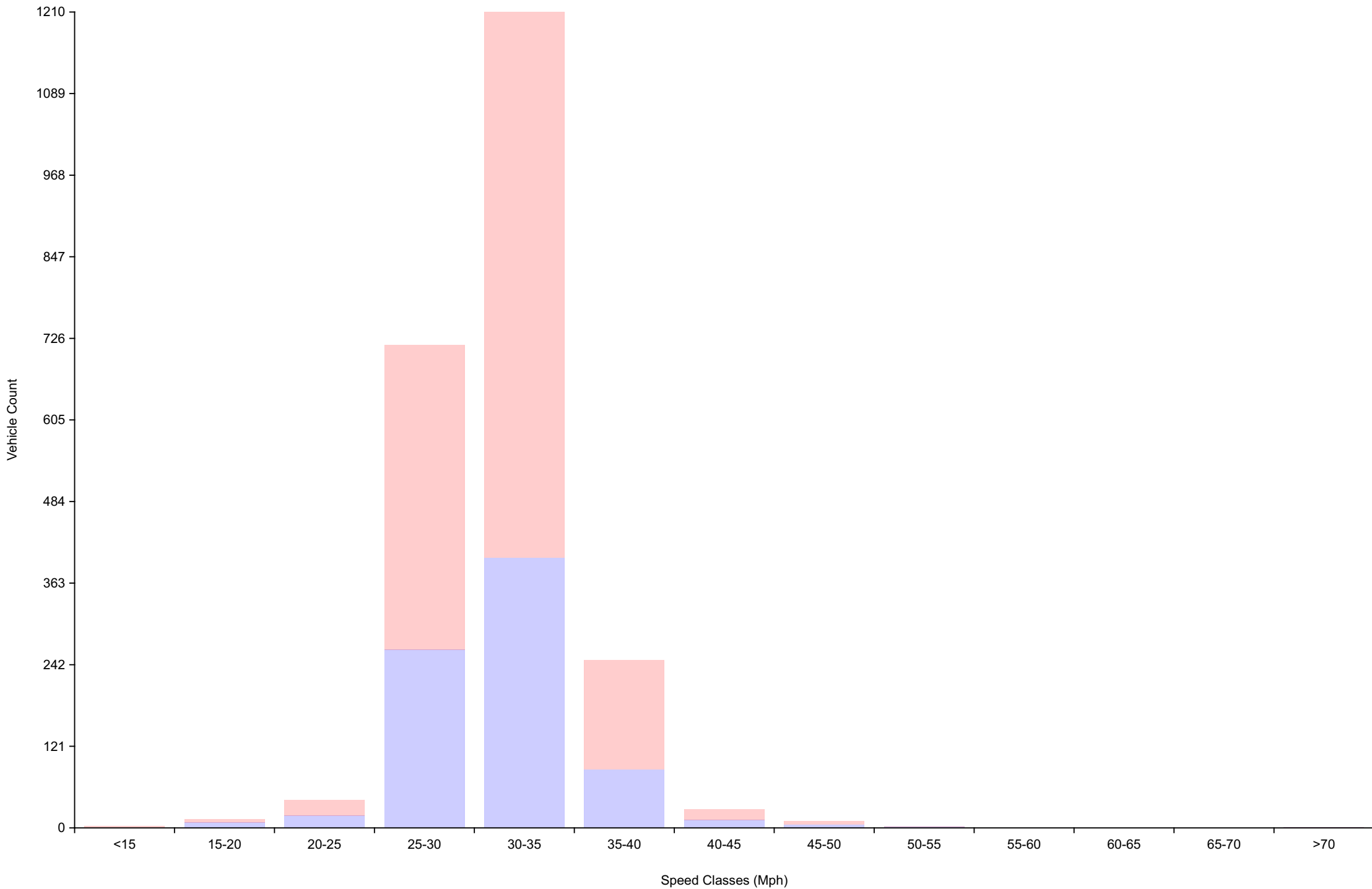
Vehicle Counts By Speed Class Daily Overview for Fri May 23 2025
