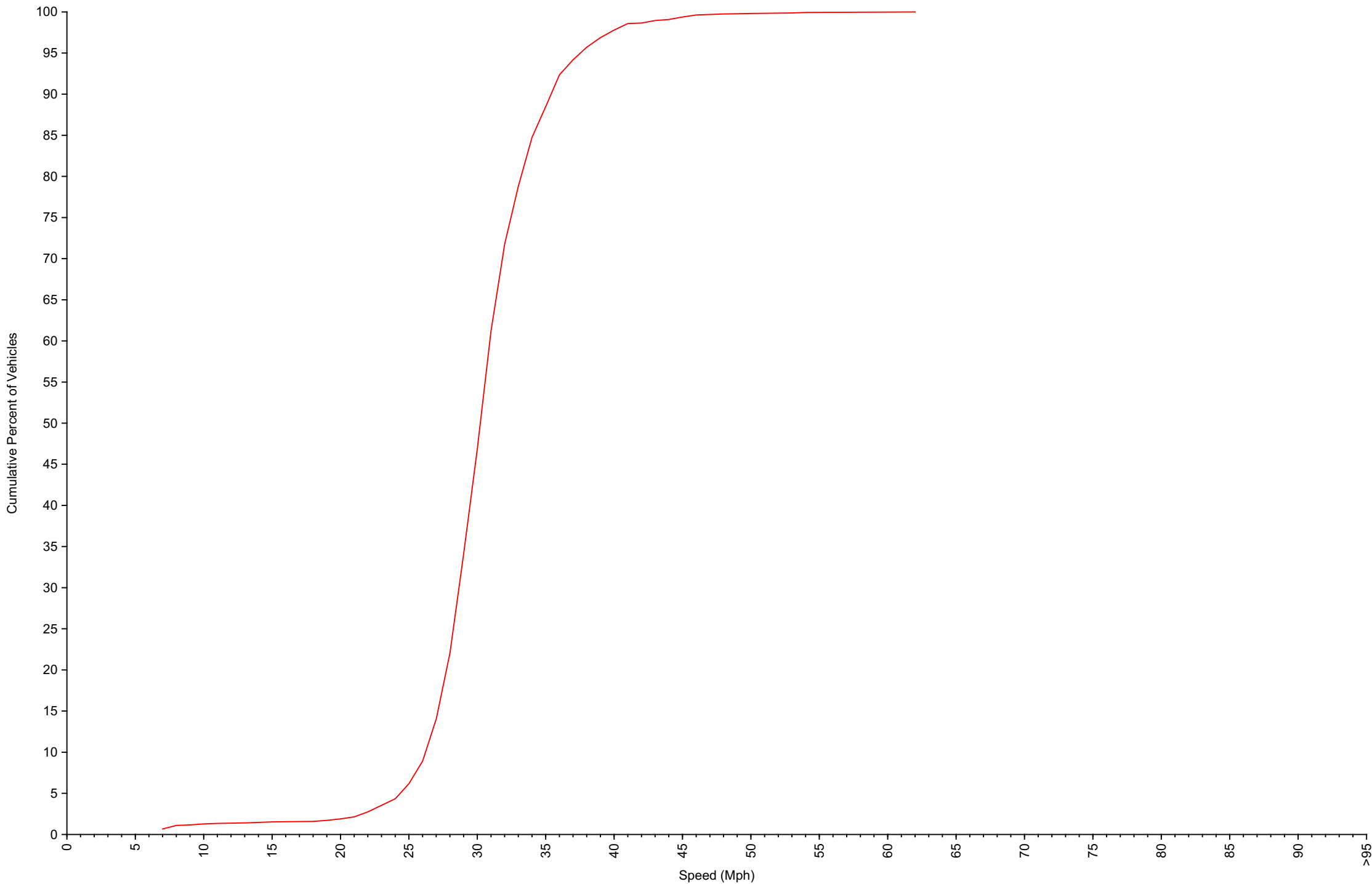
Cumulative Speed Distribution Curve Daily Overview for Sat May 24 2025
