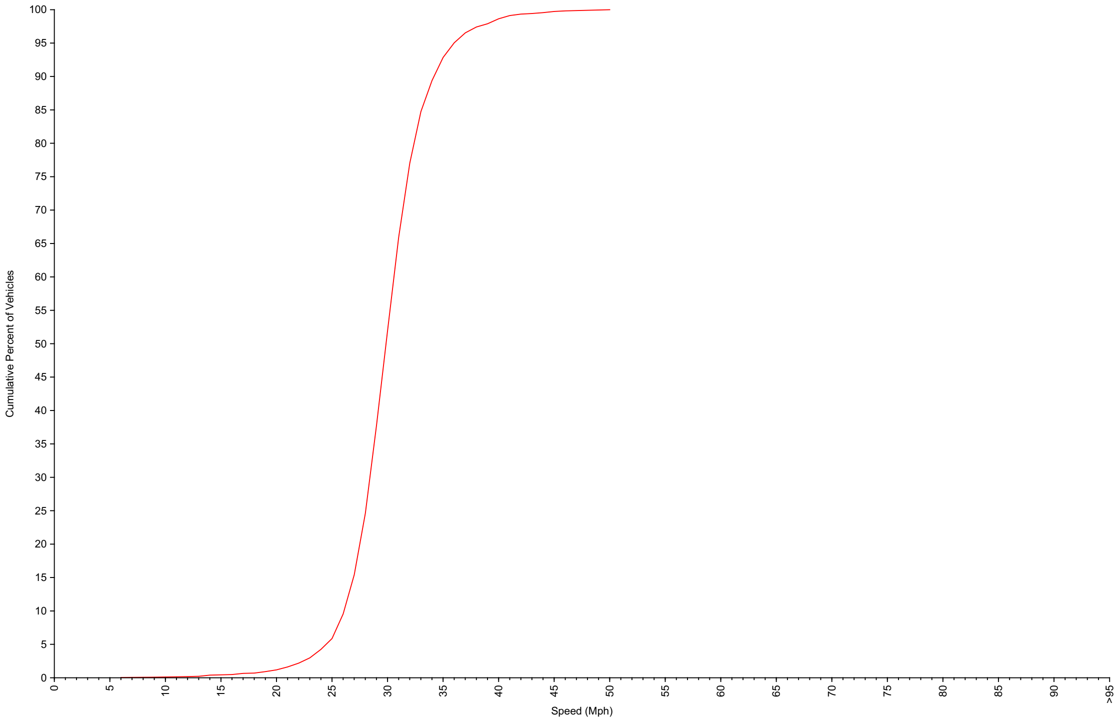
Cumulative Speed Distribution Curve Daily Overview for Mon May 12 2025
