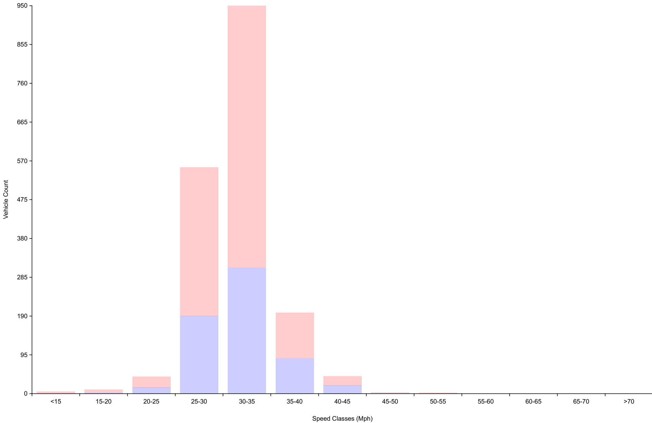
Vehicle Counts By Speed Class Daily Overview for Wed May 28 2025
