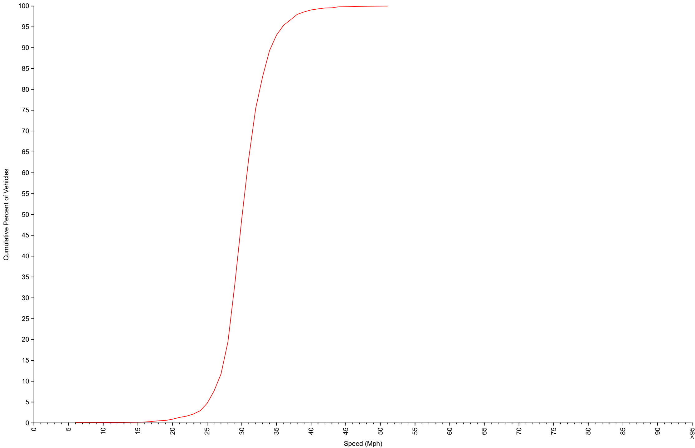
Cumulative Speed Distribution Curve Daily Overview for Thu May 15 2025
