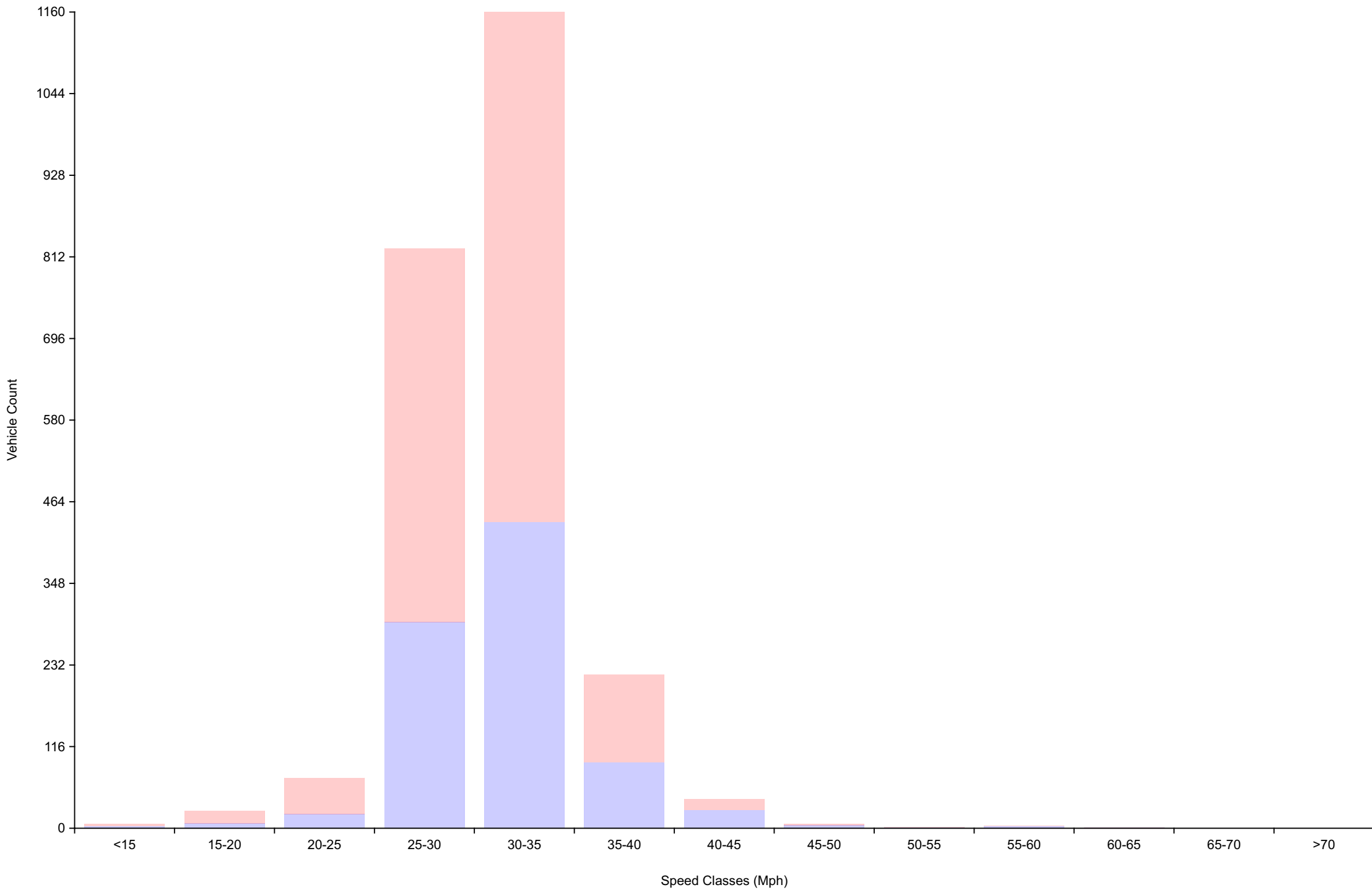
Vehicle Counts By Speed Class Daily Overview for Tue May 13 2025
