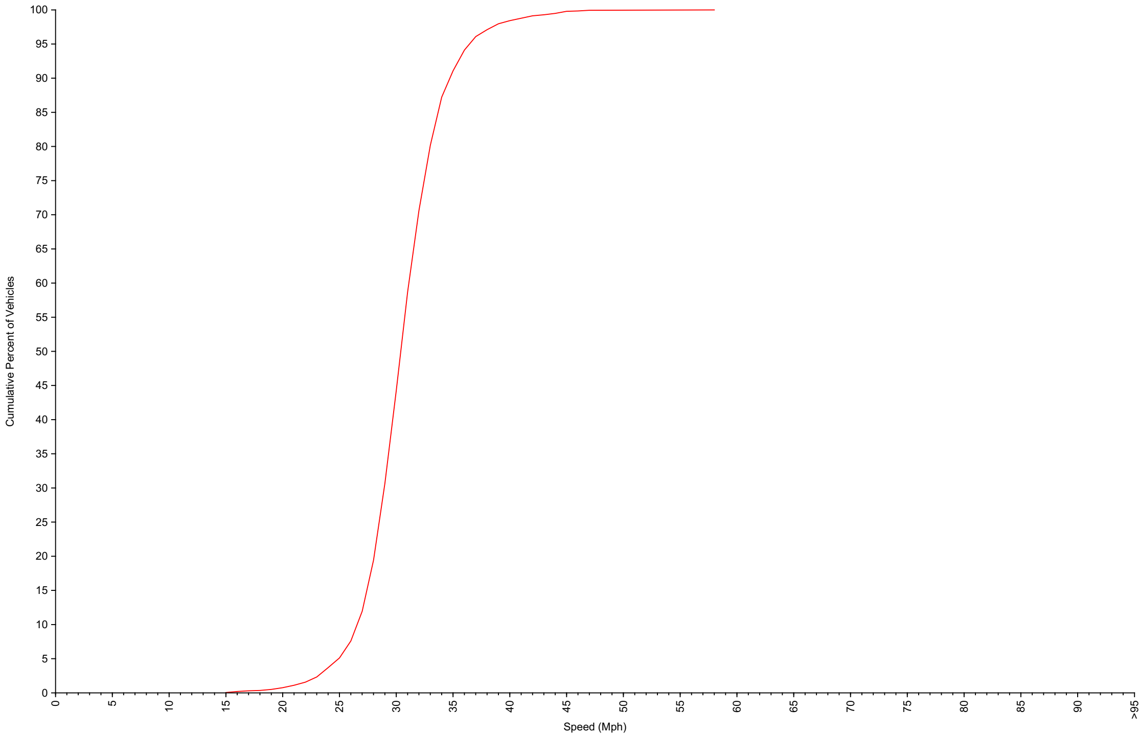
Cumulative Speed Distribution Curve Daily Overview for Sat May 17 2025
