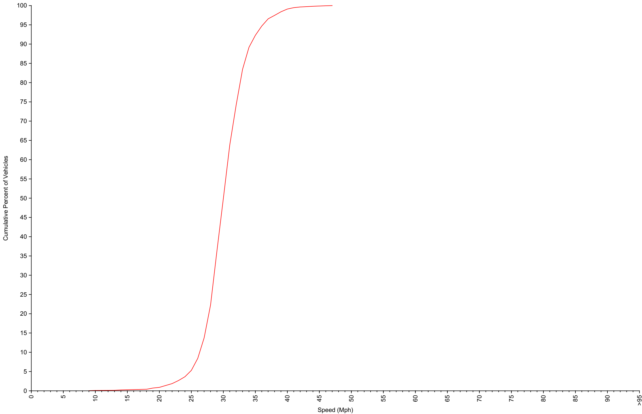
Cumulative Speed Distribution Curve Daily Overview for Wed May 14 2025
