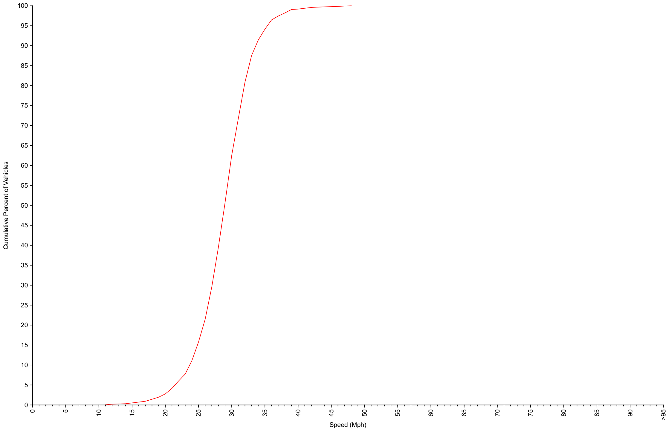
Cumulative Speed Distribution Curve Daily Overview for Fri Feb 28 2025
