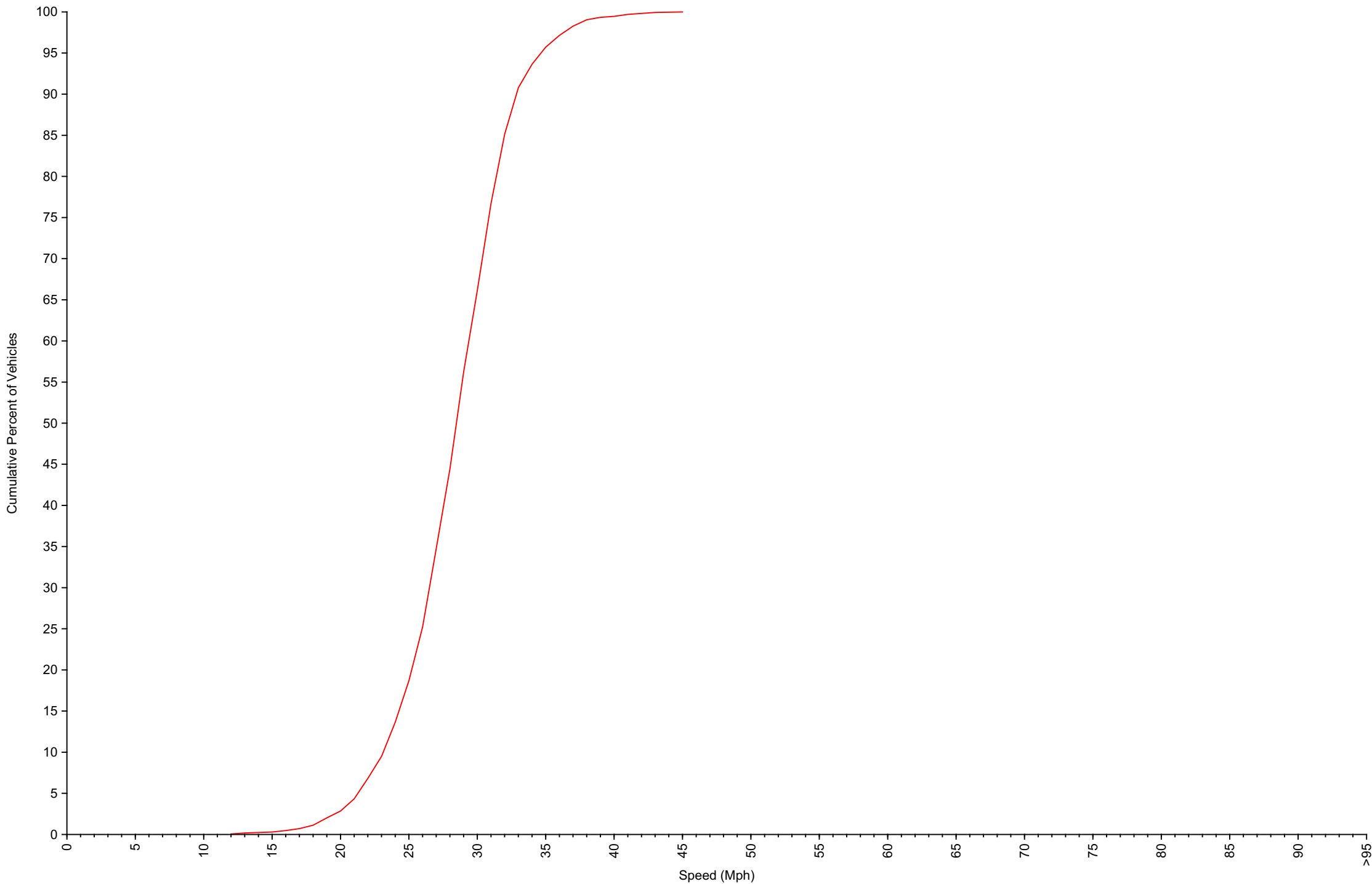
Cumulative Speed Distribution Curve Daily Overview for Wed Feb 12 2025
