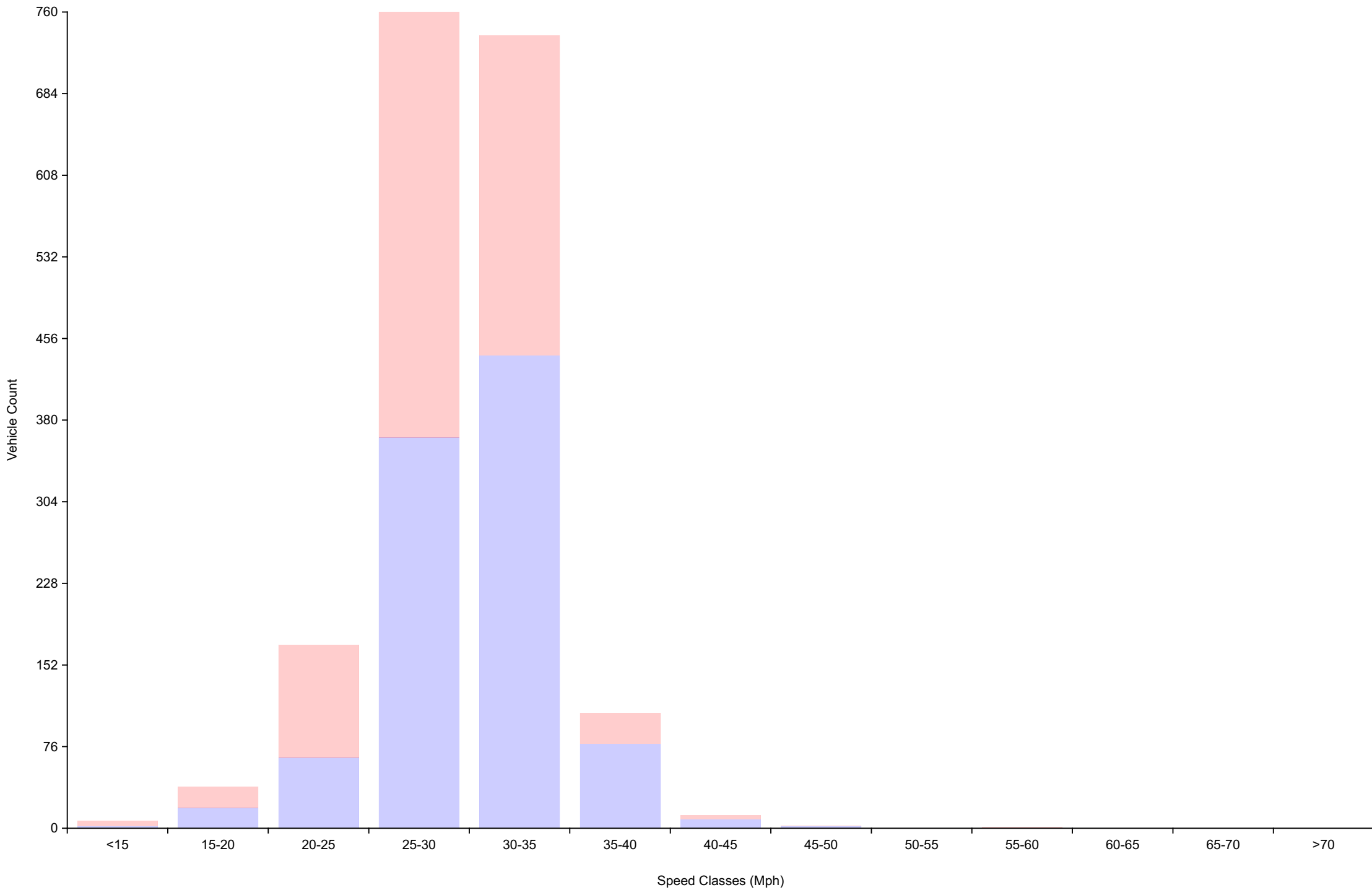
Vehicle Counts By Speed Class Daily Overview for Tue Feb 25 2025
