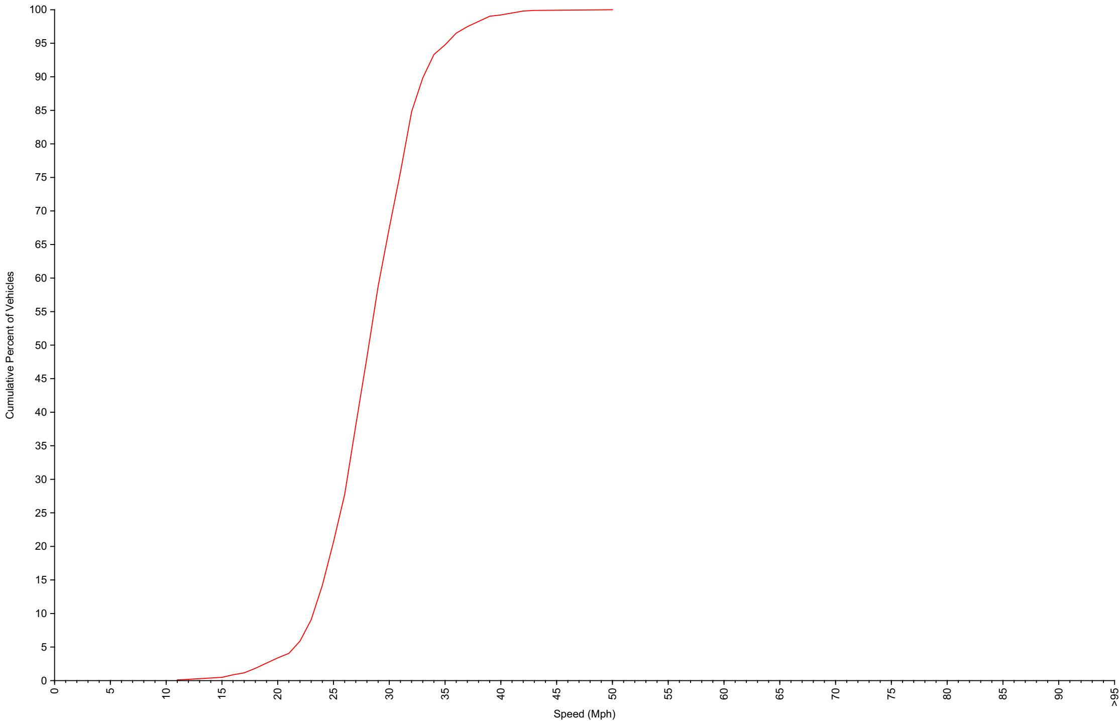
Cumulative Speed Distribution Curve Daily Overview for Sun Feb 23 2025
