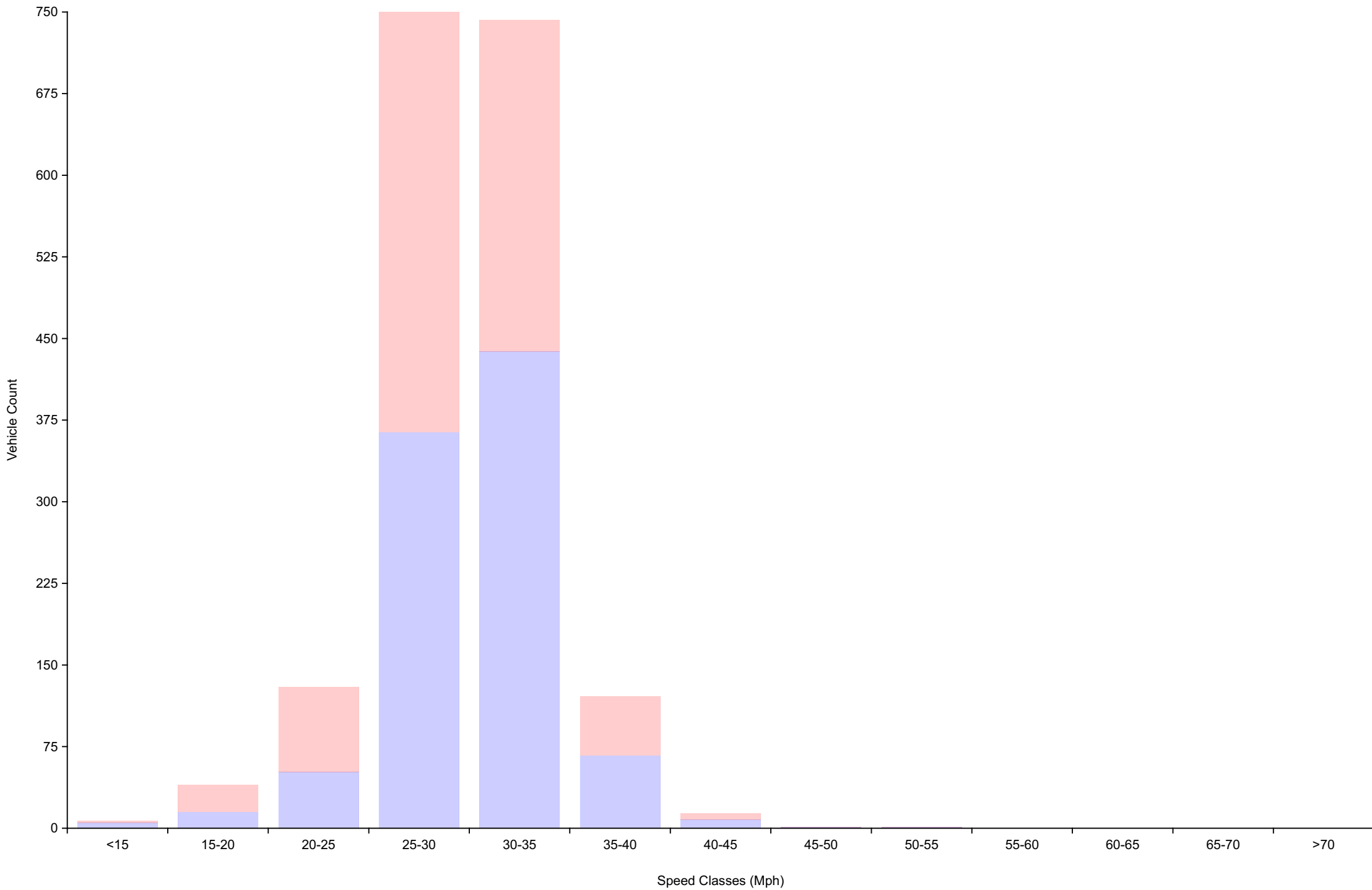
Vehicle Counts By Speed Class Daily Overview for Thu Feb 20 2025
