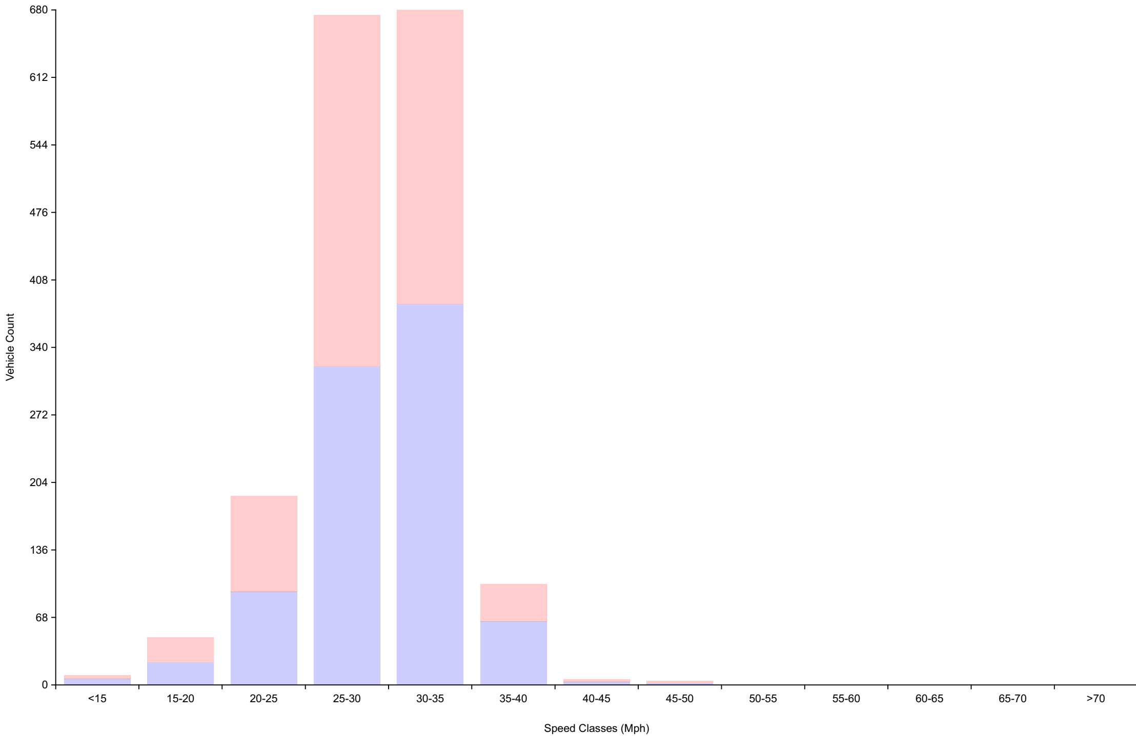
Vehicle Counts By Speed Class Daily Overview for Tue Feb 18 2025
