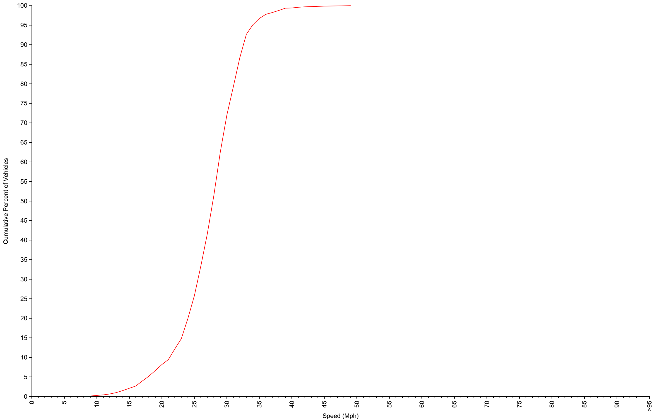
Cumulative Speed Distribution Curve Daily Overview for Thu Feb 13 2025
