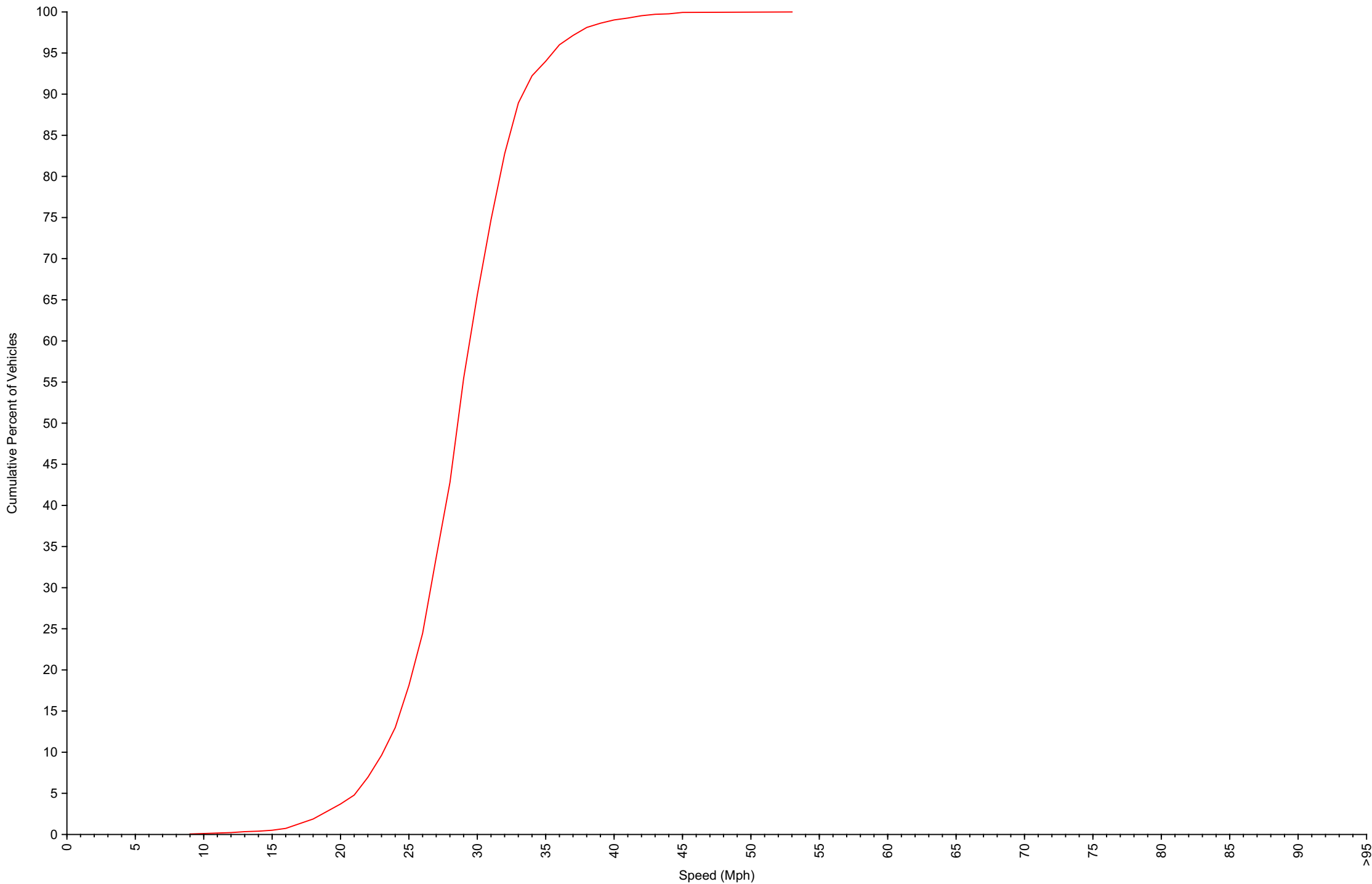
Cumulative Speed Distribution Curve Daily Overview for Fri Feb 14 2025
