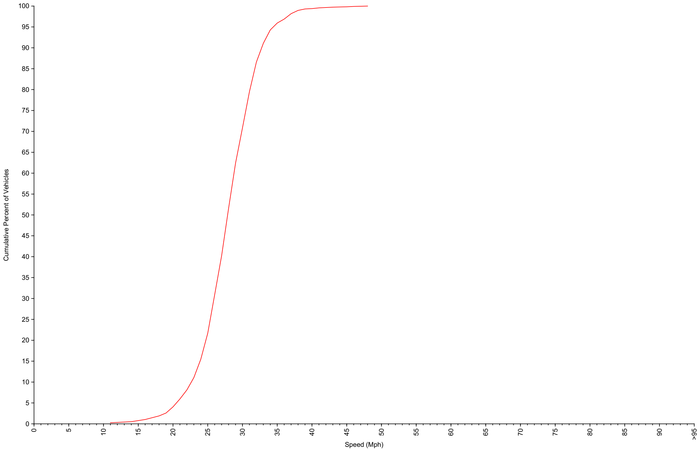
Cumulative Speed Distribution Curve Daily Overview for Sat Feb 15 2025
