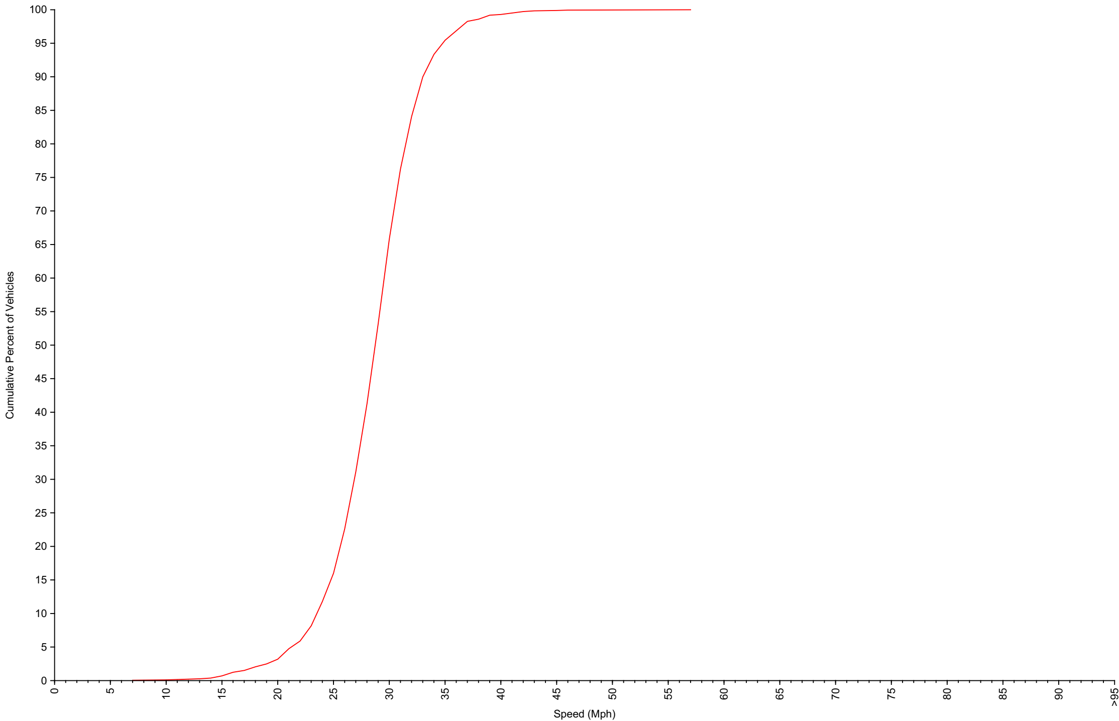
Cumulative Speed Distribution Curve Daily Overview for Tue Feb 25 2025
