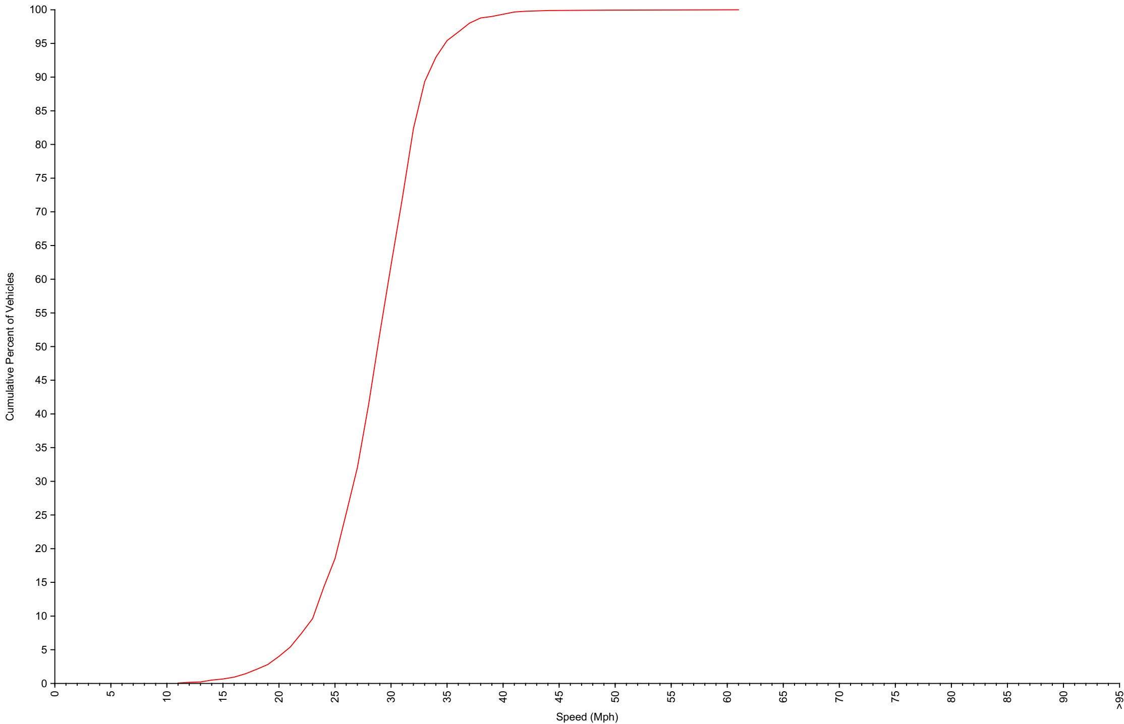
Cumulative Speed Distribution Curve Daily Overview for Wed Feb 19 2025
