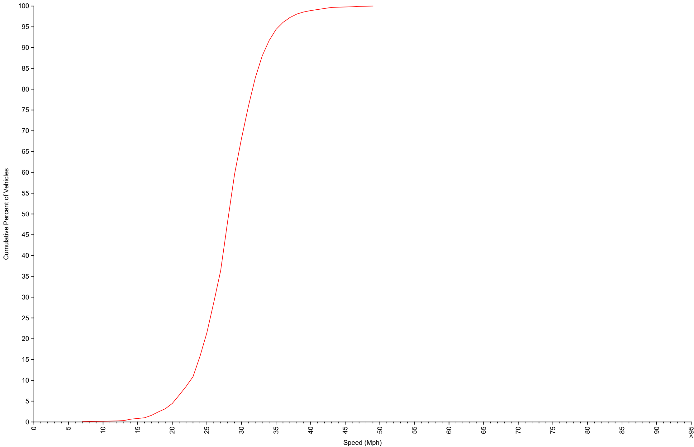
Cumulative Speed Distribution Curve Daily Overview for Sat Feb 1 2025
