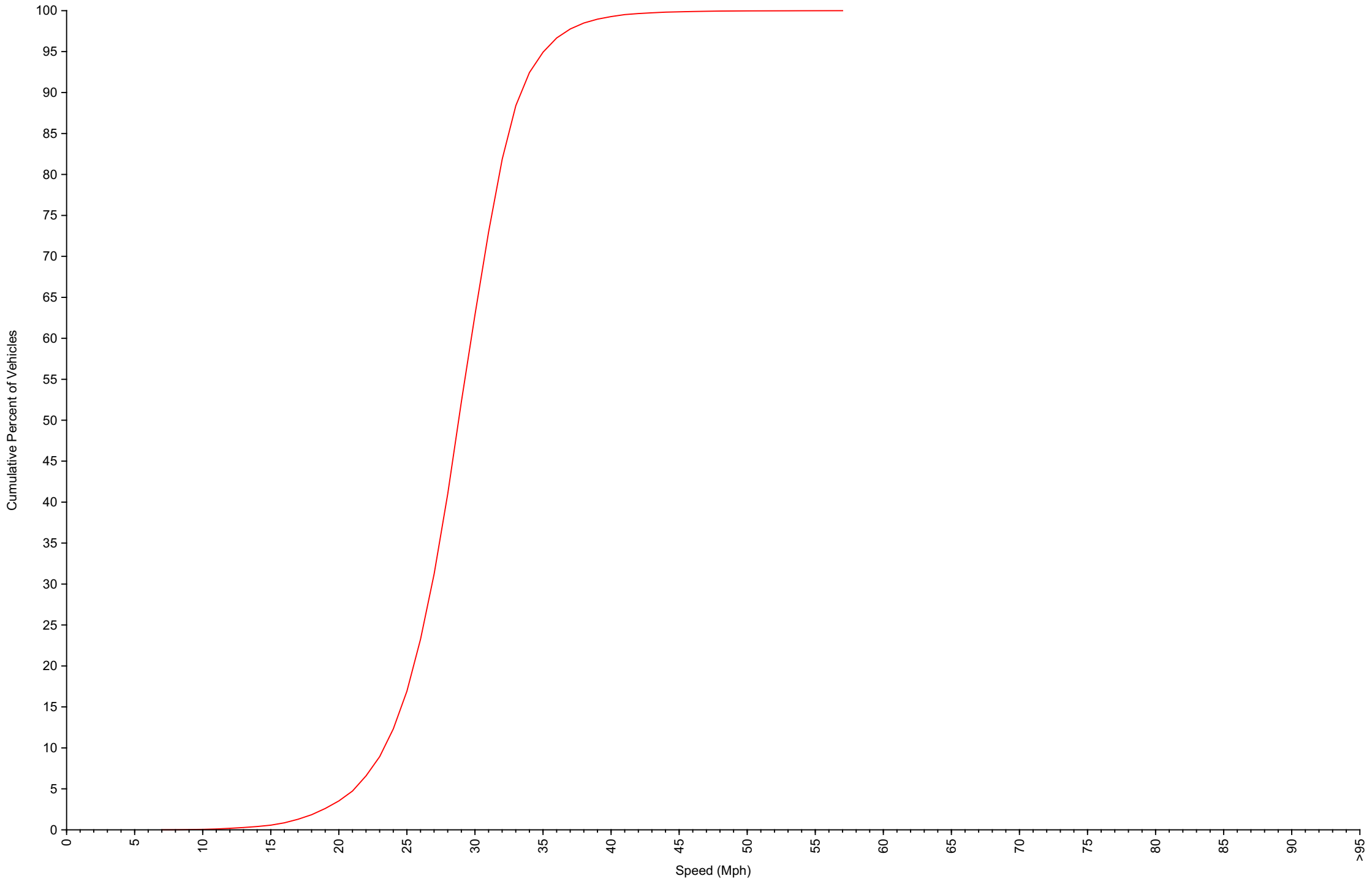
Cumulative Speed Distribution Curve Traffic Overview from Sat Mar 1 2025 to Mon Mar 31 2025
