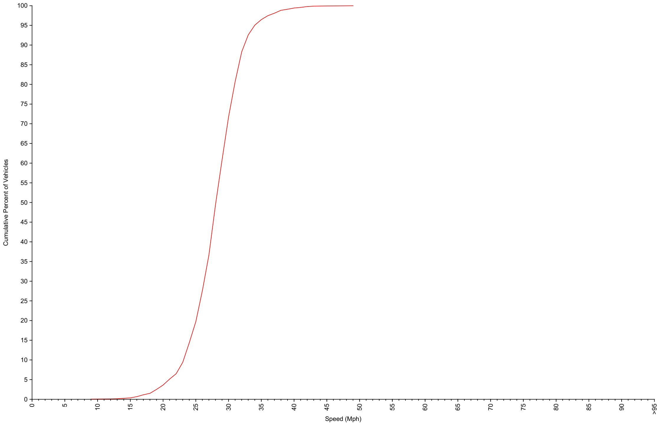
Cumulative Speed Distribution Curve Daily Overview for Tue Oct 14 2025
