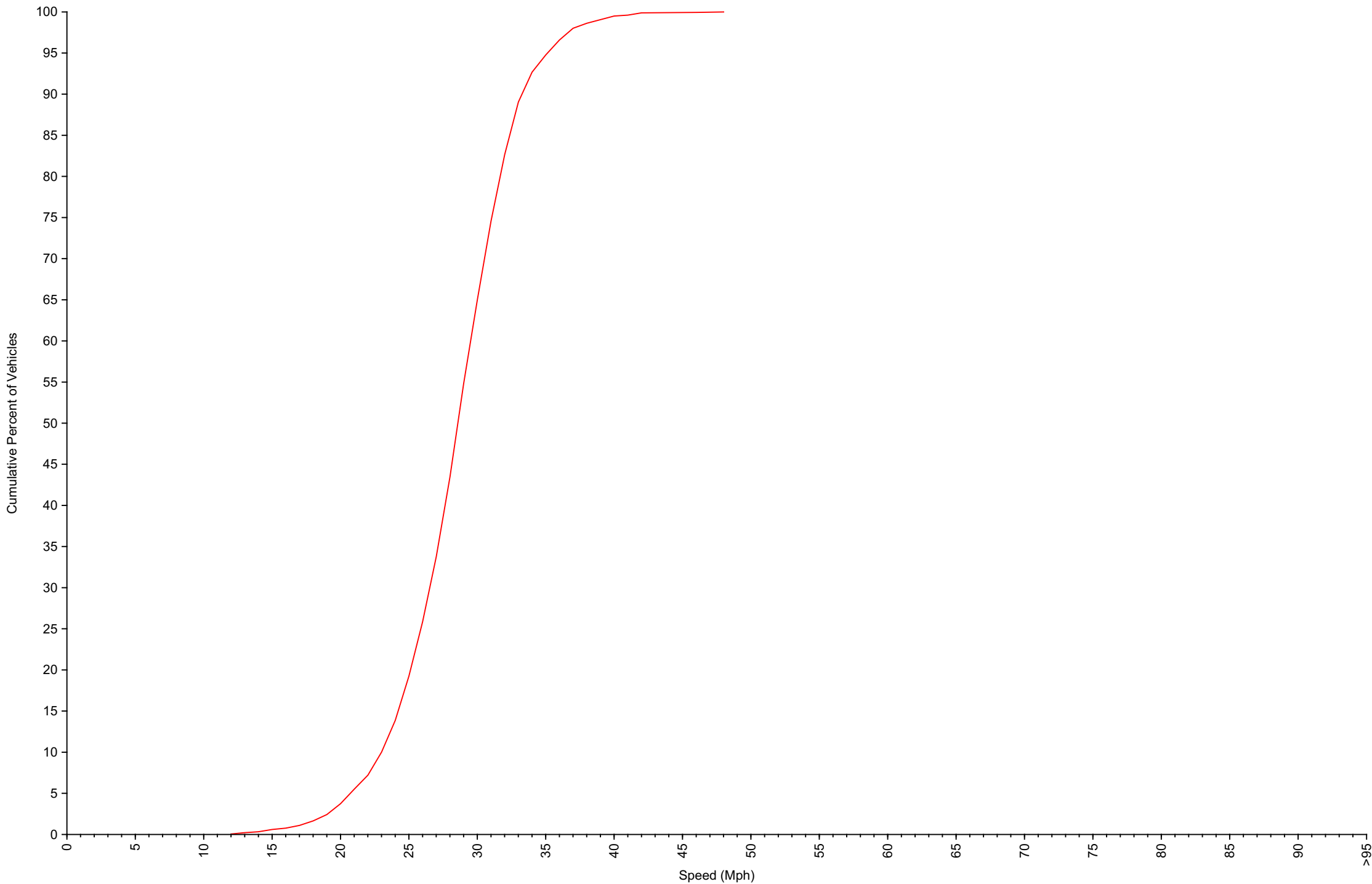
Cumulative Speed Distribution Curve Daily Overview for Thu Oct 30 2025
