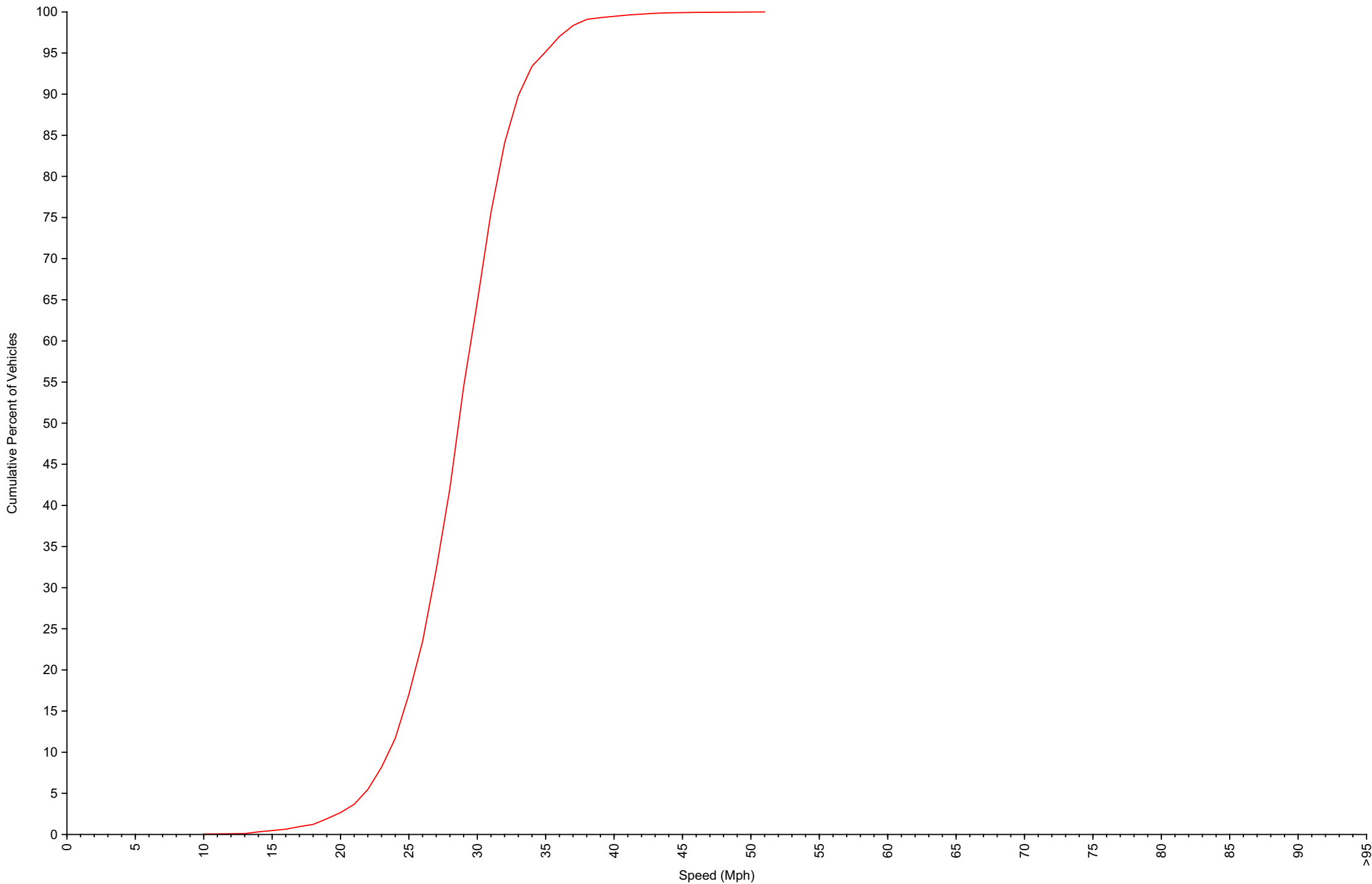
Cumulative Speed Distribution Curve Daily Overview for Thu Oct 23 2025
