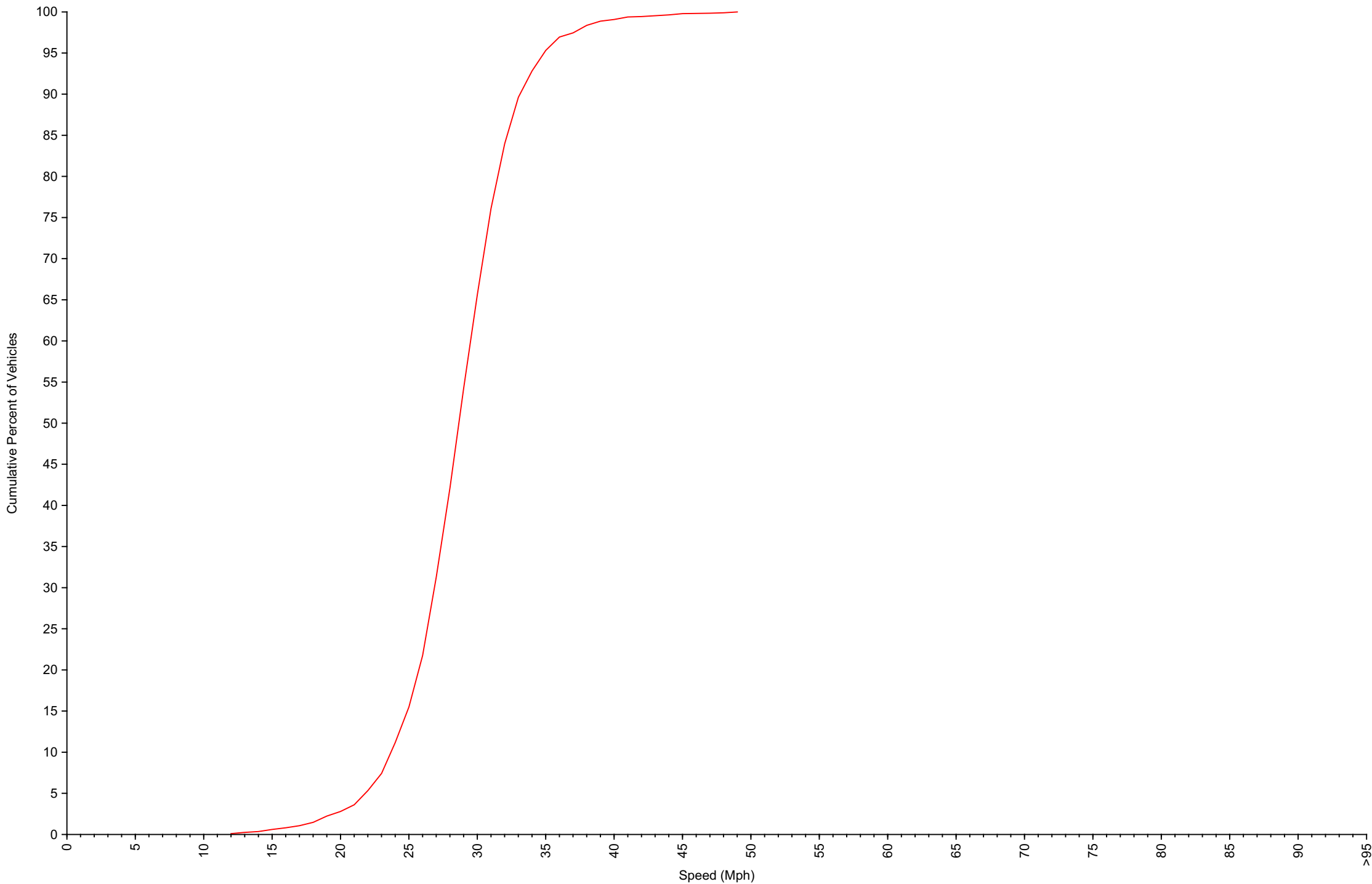
Cumulative Speed Distribution Curve Daily Overview for Wed Oct 22 2025
