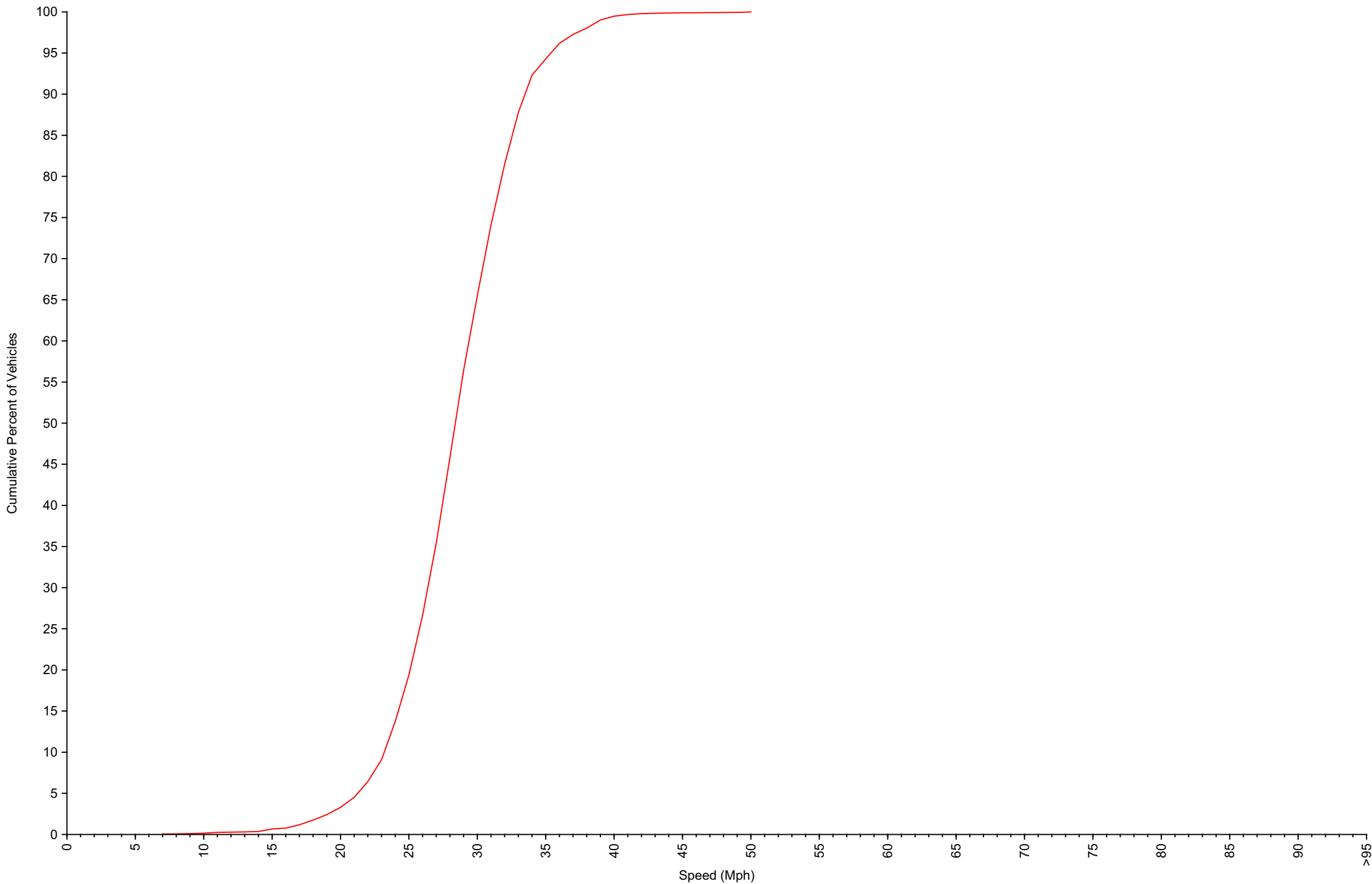
Cumulative Speed Distribution Curve Daily Overview for Wed Oct 29 2025
