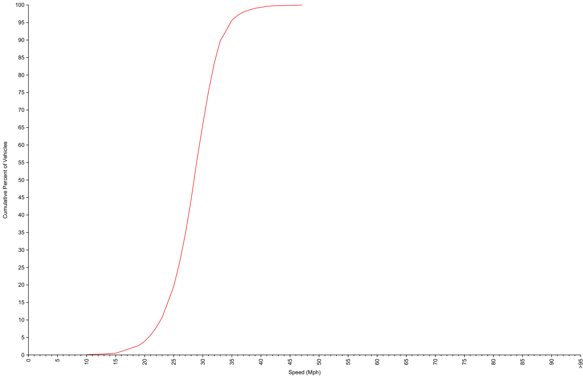
Cumulative Speed Distribution Curve Daily Overview for Mon Oct 27 2025
