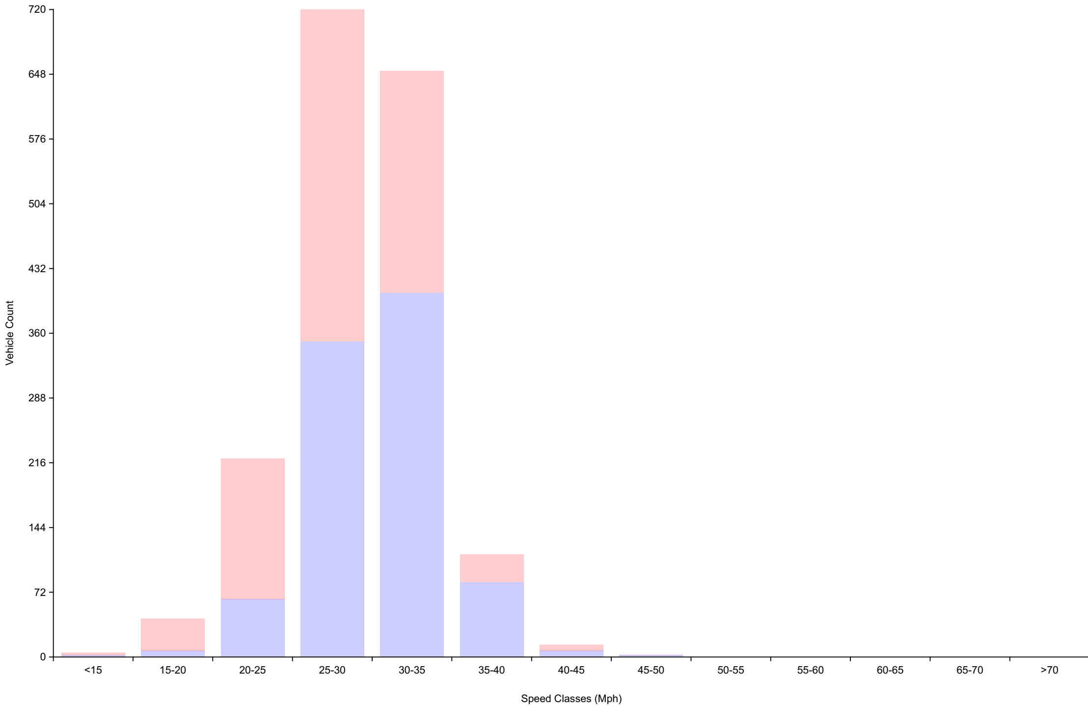
Vehicle Counts By Speed Class Daily Overview for Mon Oct 27 2025
