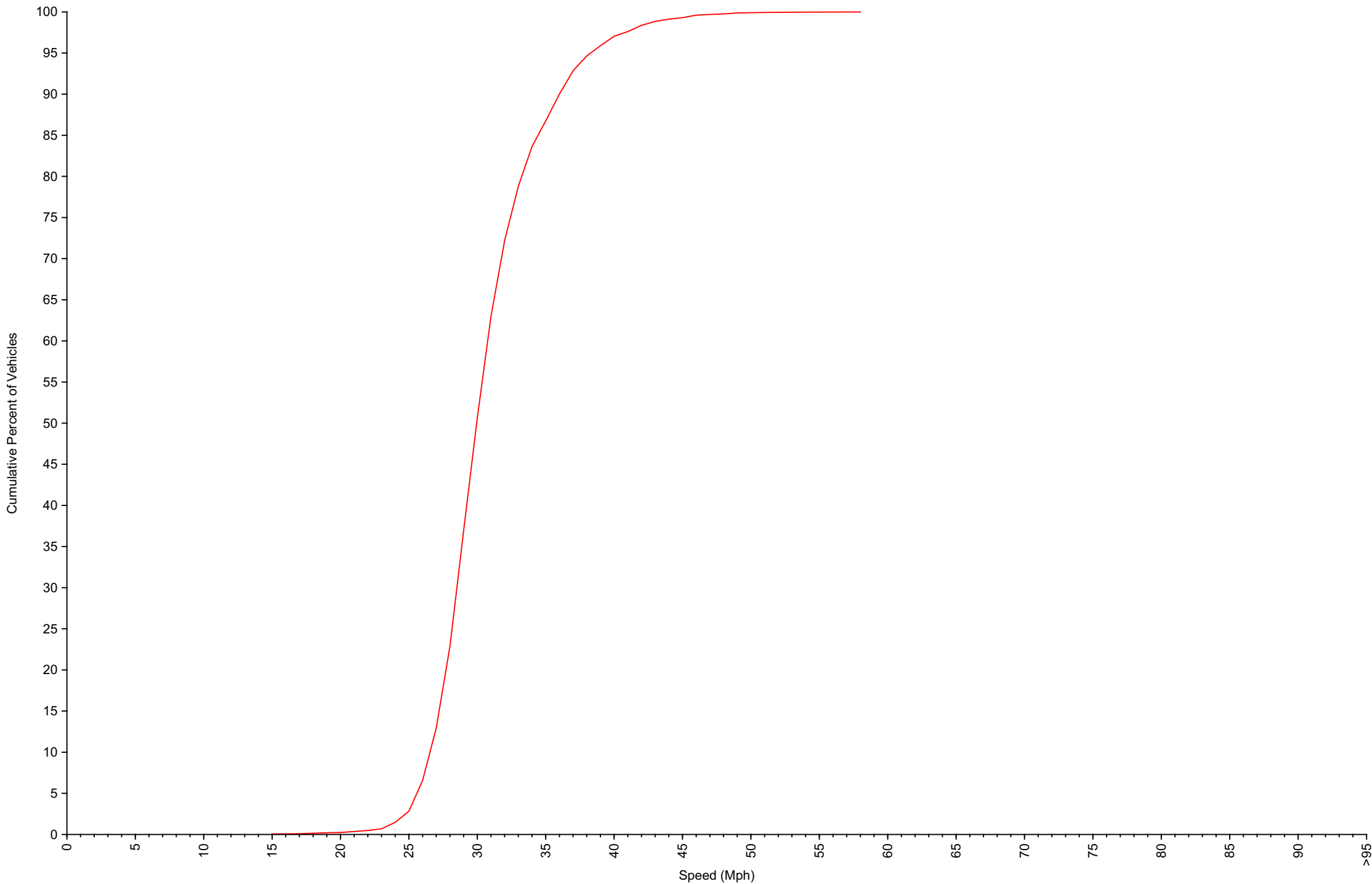
Cumulative Speed Distribution Curve Daily Overview for Tue Apr 14 2026
