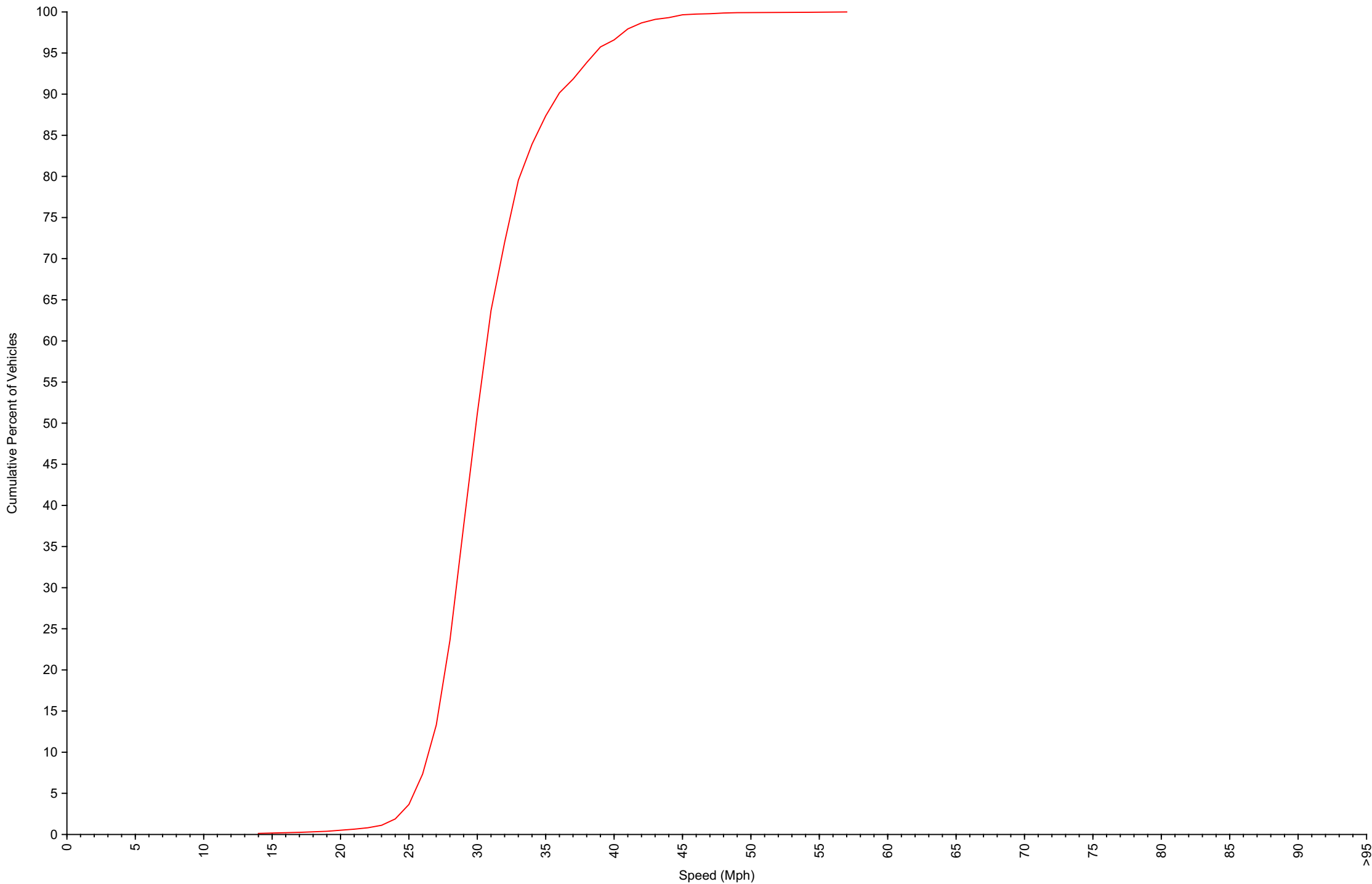
Cumulative Speed Distribution Curve Daily Overview for Sat Apr 25 2026
