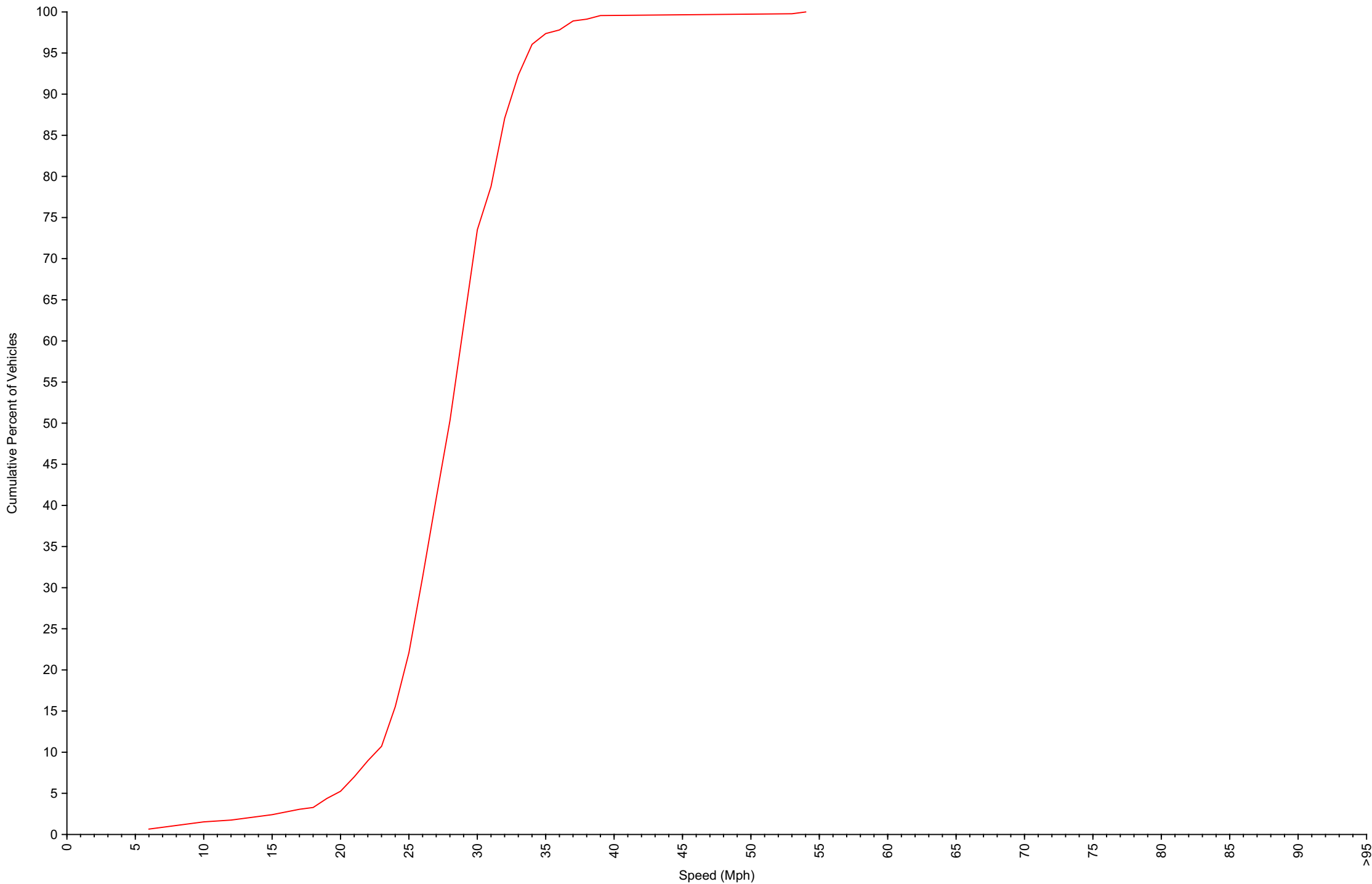
Cumulative Speed Distribution Curve Daily Overview for Wed Apr 1 2026
