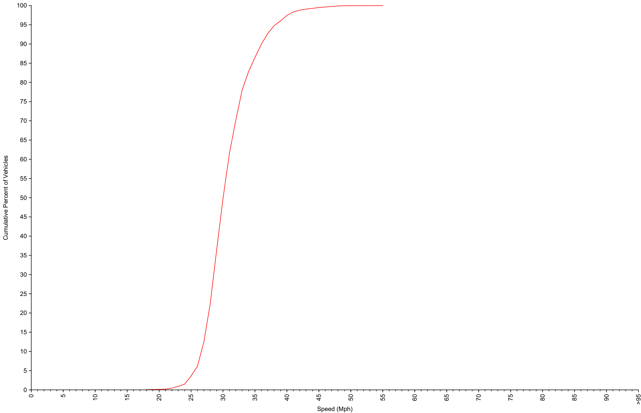
Cumulative Speed Distribution Curve Daily Overview for Sat Apr 11 2026
