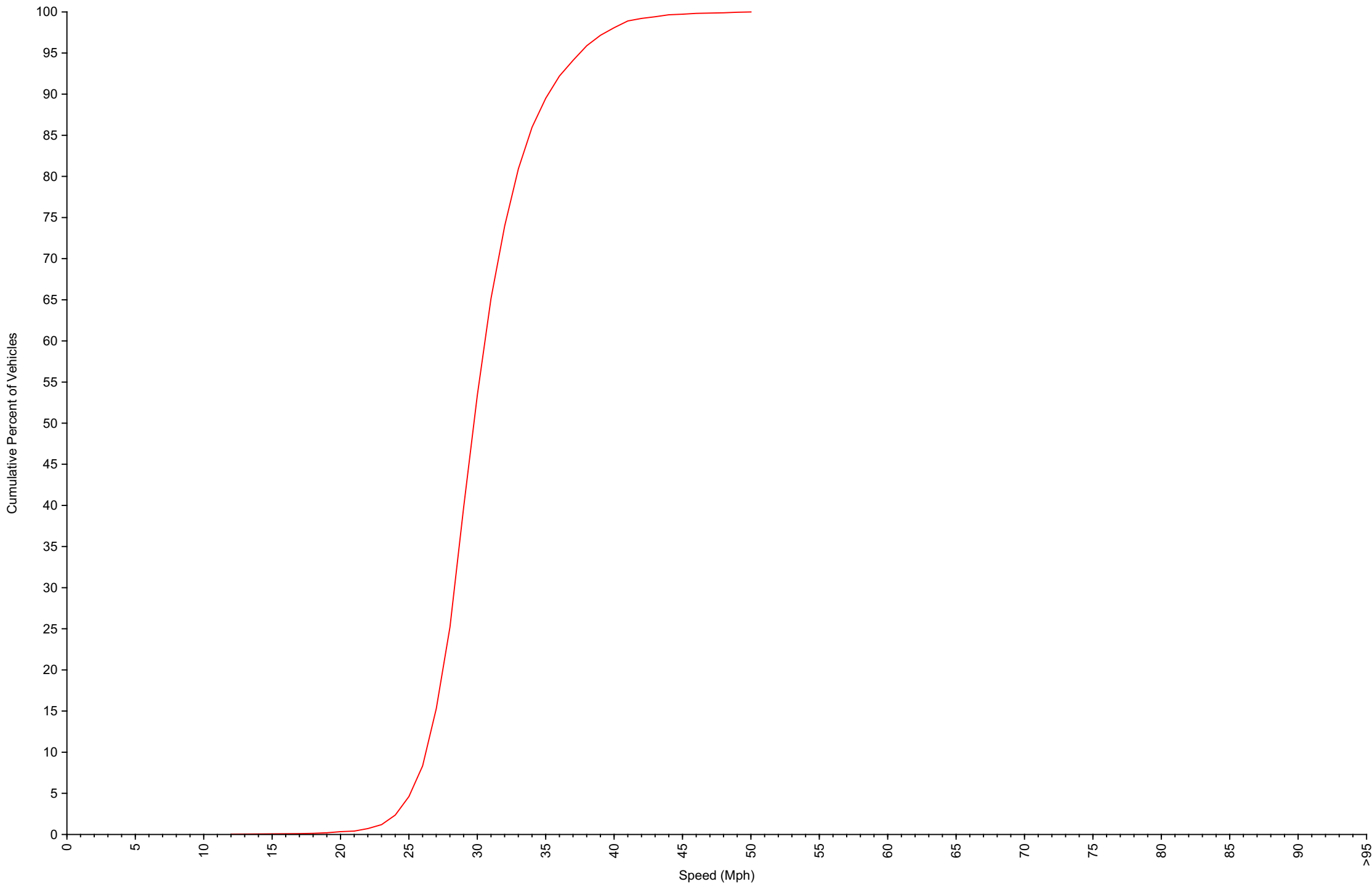
Cumulative Speed Distribution Curve Daily Overview for Mon Apr 13 2026
