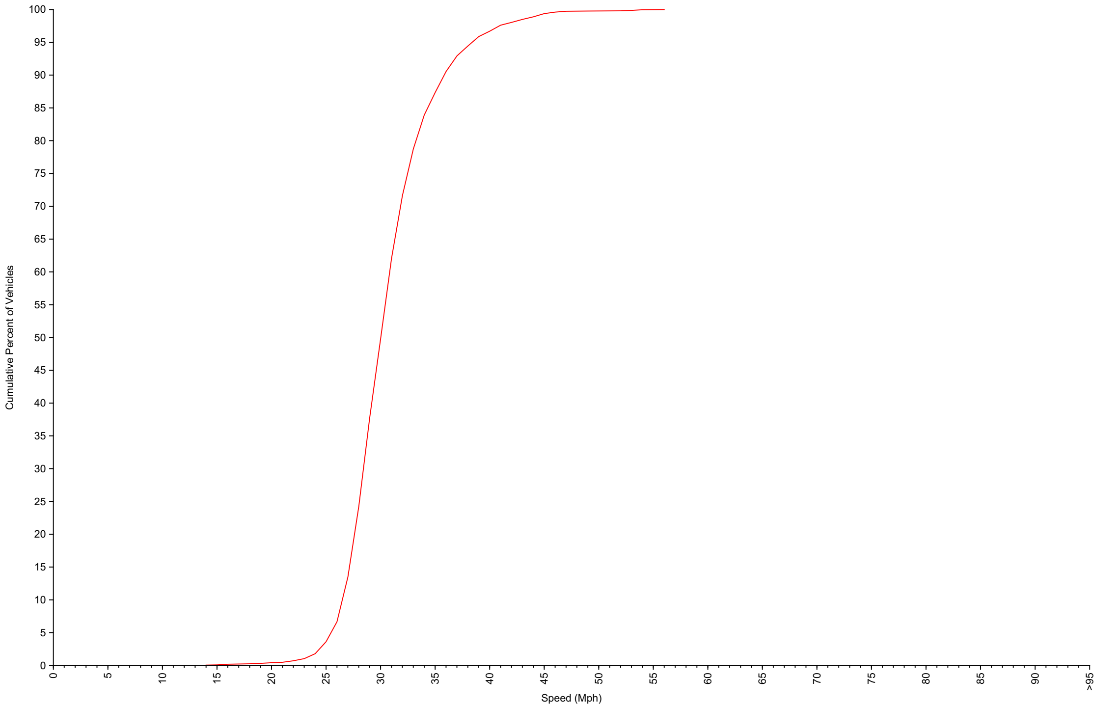
Cumulative Speed Distribution Curve Daily Overview for Tue Apr 28 2026
