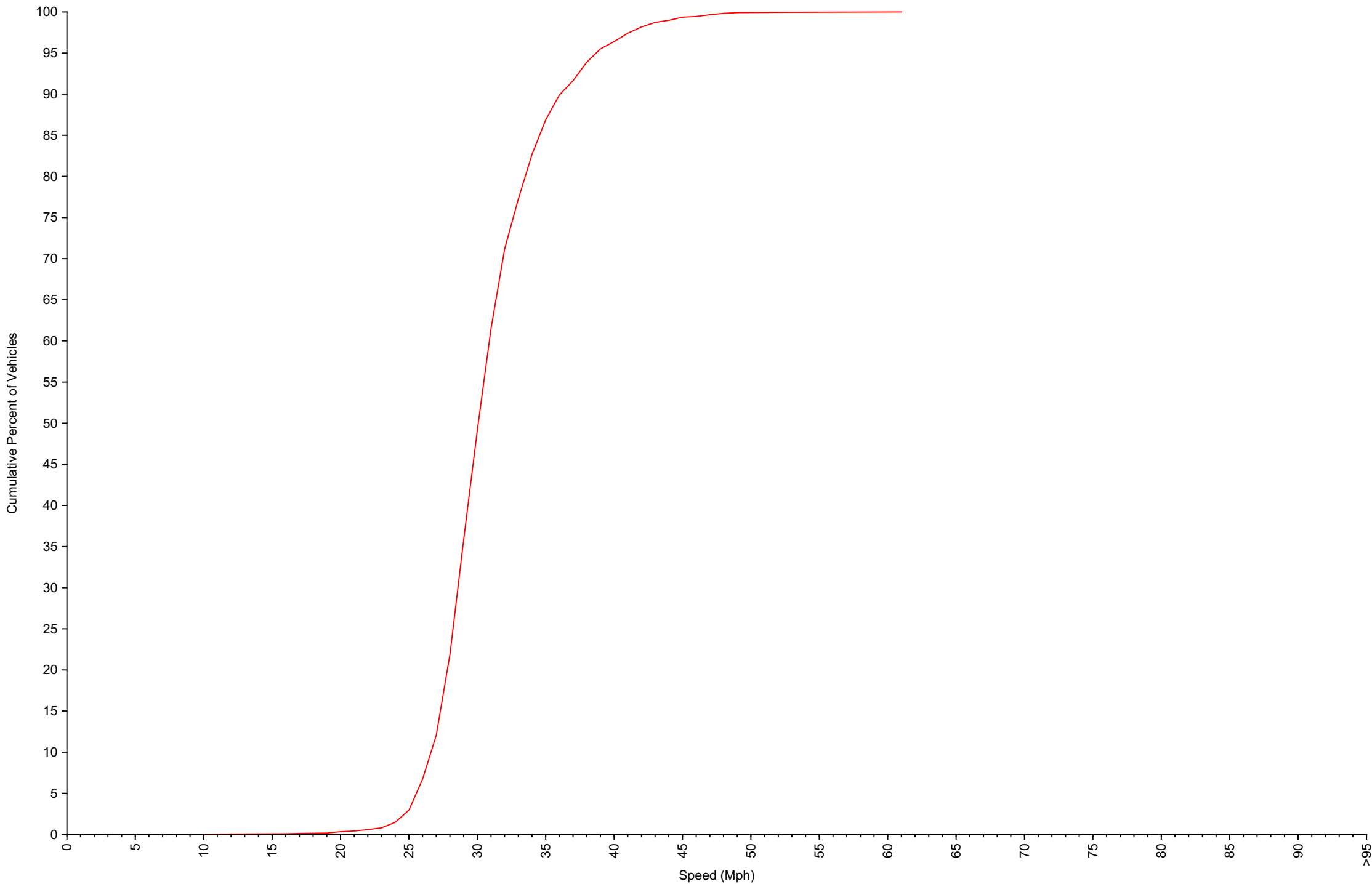
Cumulative Speed Distribution Curve Daily Overview for Sat Apr 18 2026
