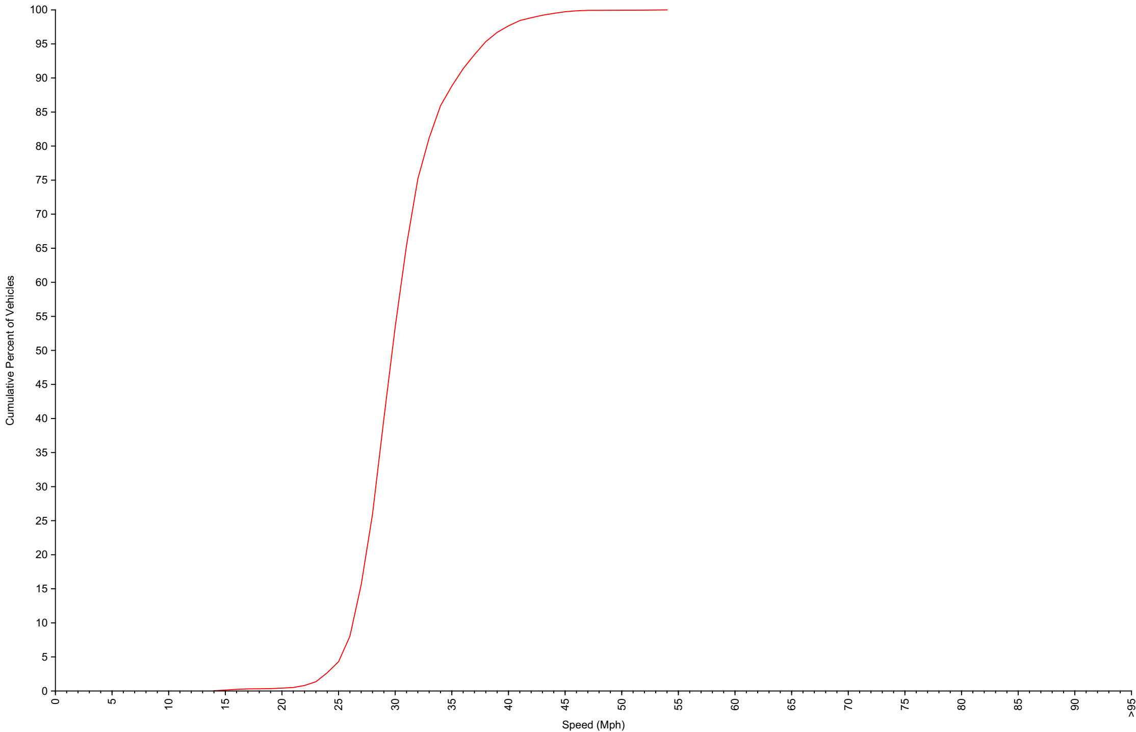
Cumulative Speed Distribution Curve Daily Overview for Mon Apr 20 2026
