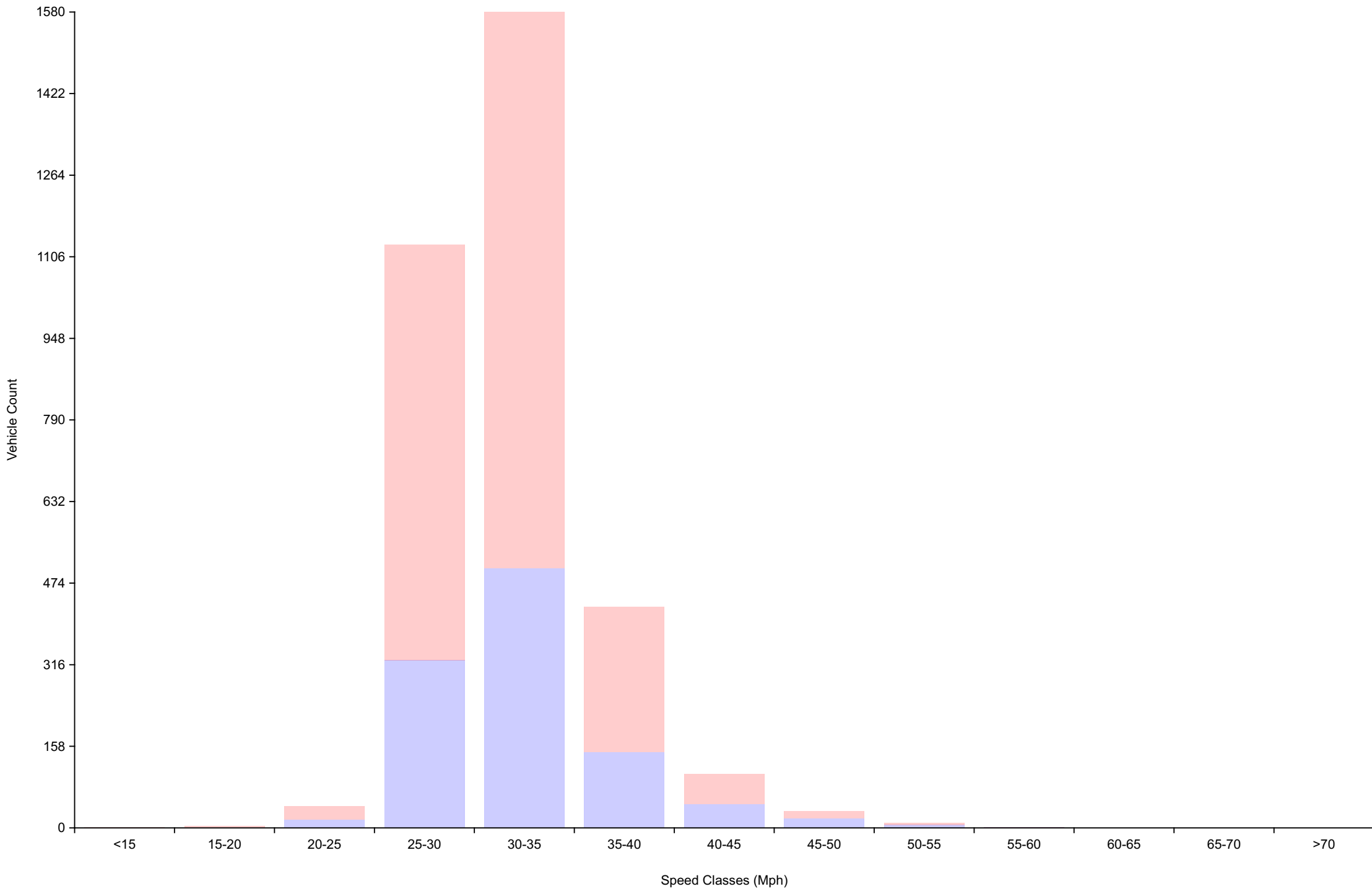
Vehicle Counts By Speed Class Daily Overview for Wed Apr 22 2026
