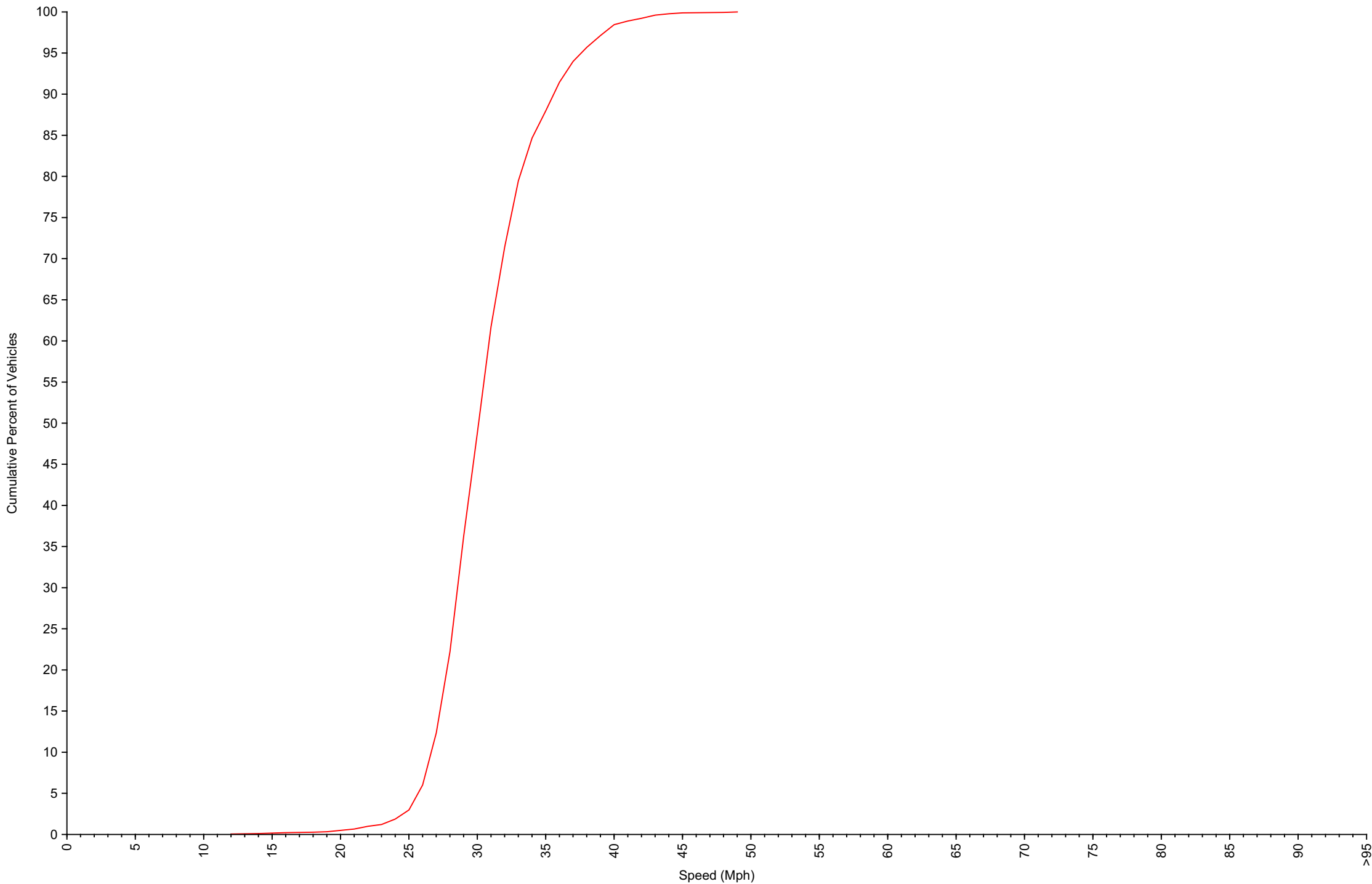
Cumulative Speed Distribution Curve Daily Overview for Sun Apr 12 2026
