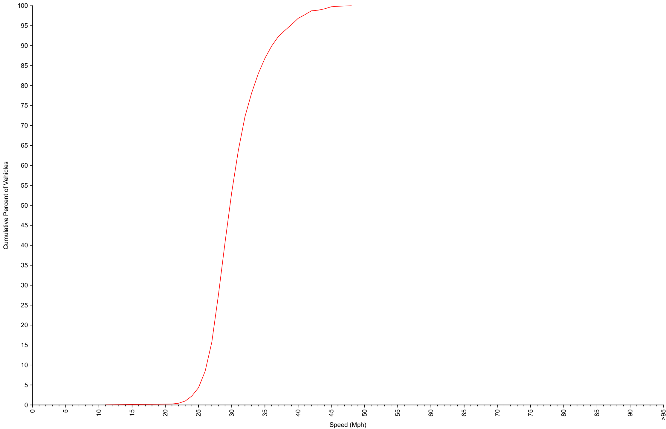
Cumulative Speed Distribution Curve Daily Overview for Sat May 16 2026
