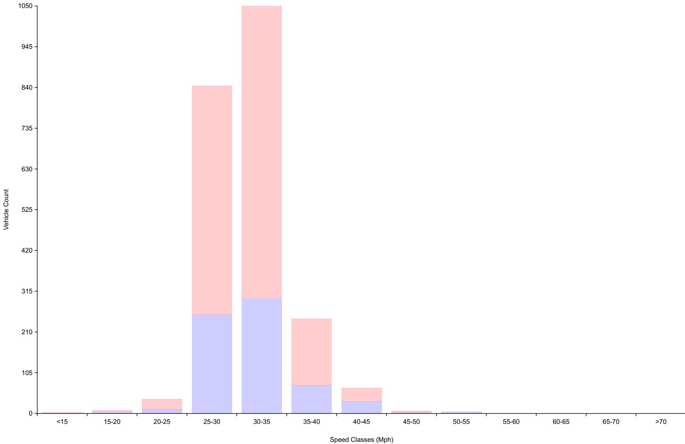
Vehicle Counts By Speed Class Daily Overview for Sat May 23 2026
