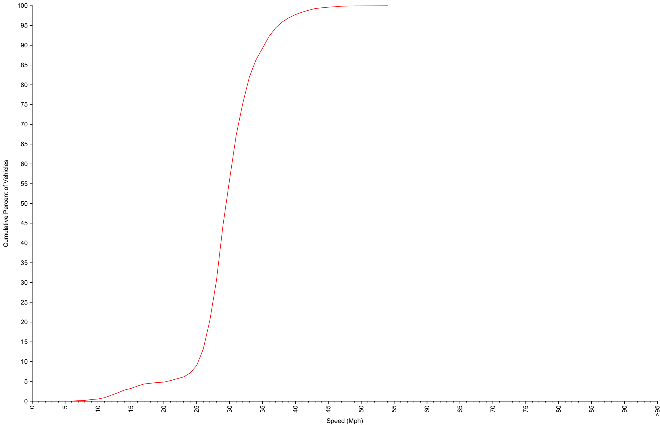
Cumulative Speed Distribution Curve Daily Overview for Tue May 26 2026
