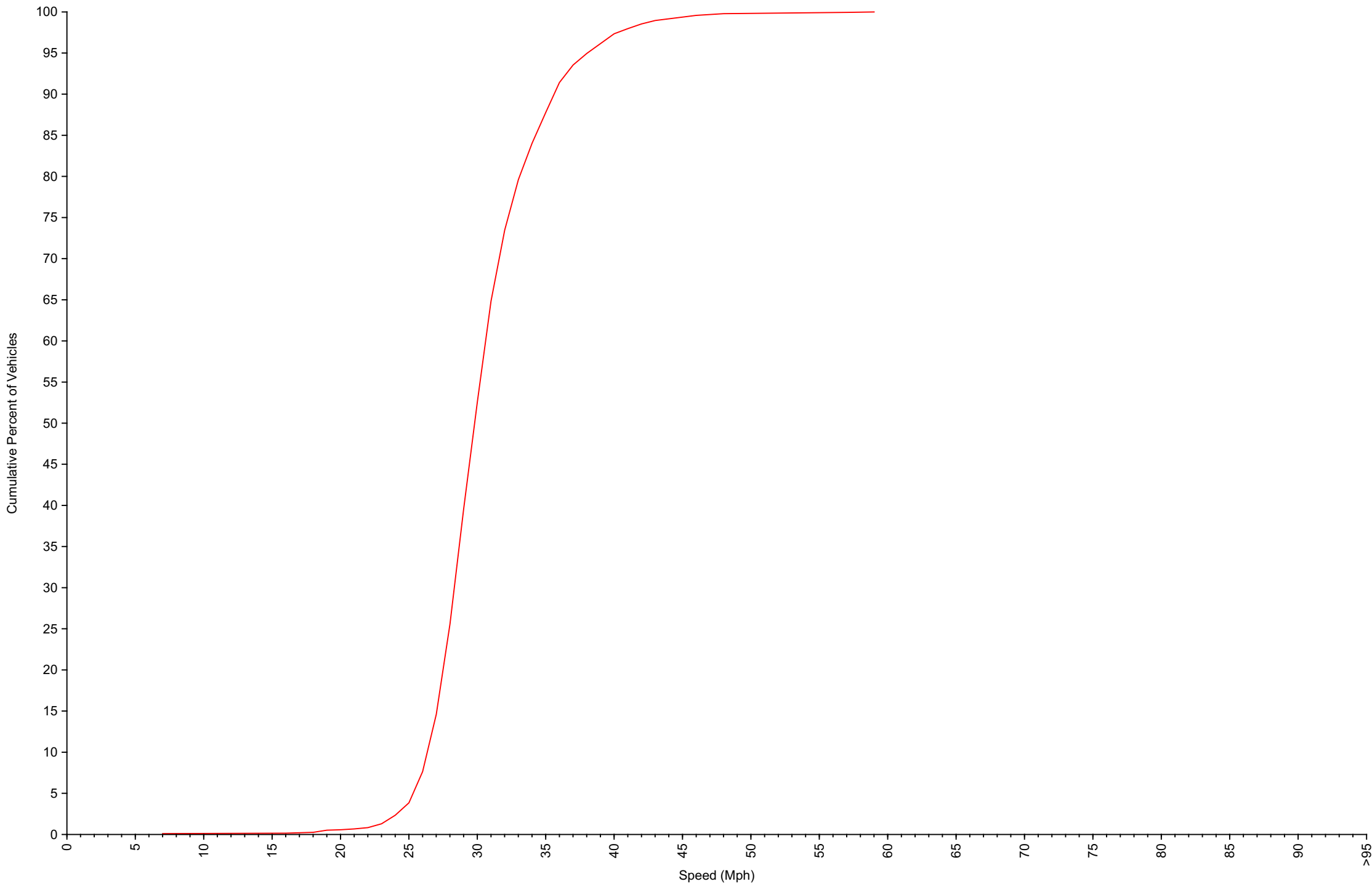
Cumulative Speed Distribution Curve Daily Overview for Sun May 17 2026
