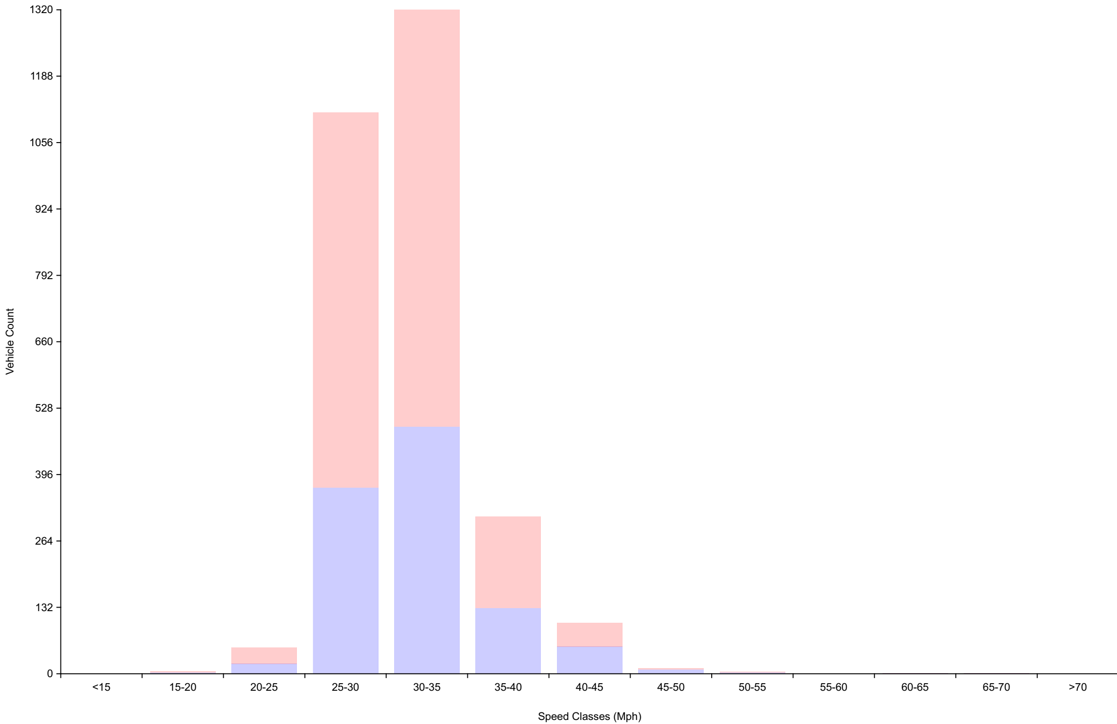
Vehicle Counts By Speed Class Daily Overview for Fri May 22 2026
