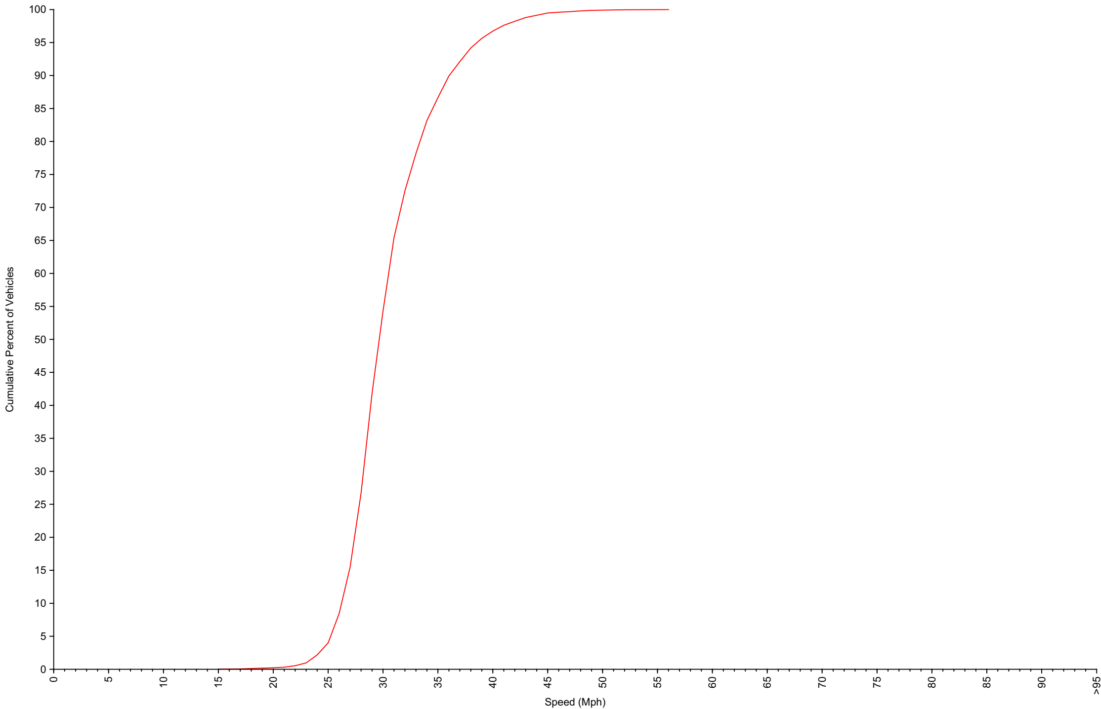
Cumulative Speed Distribution Curve Daily Overview for Tue May 19 2026
