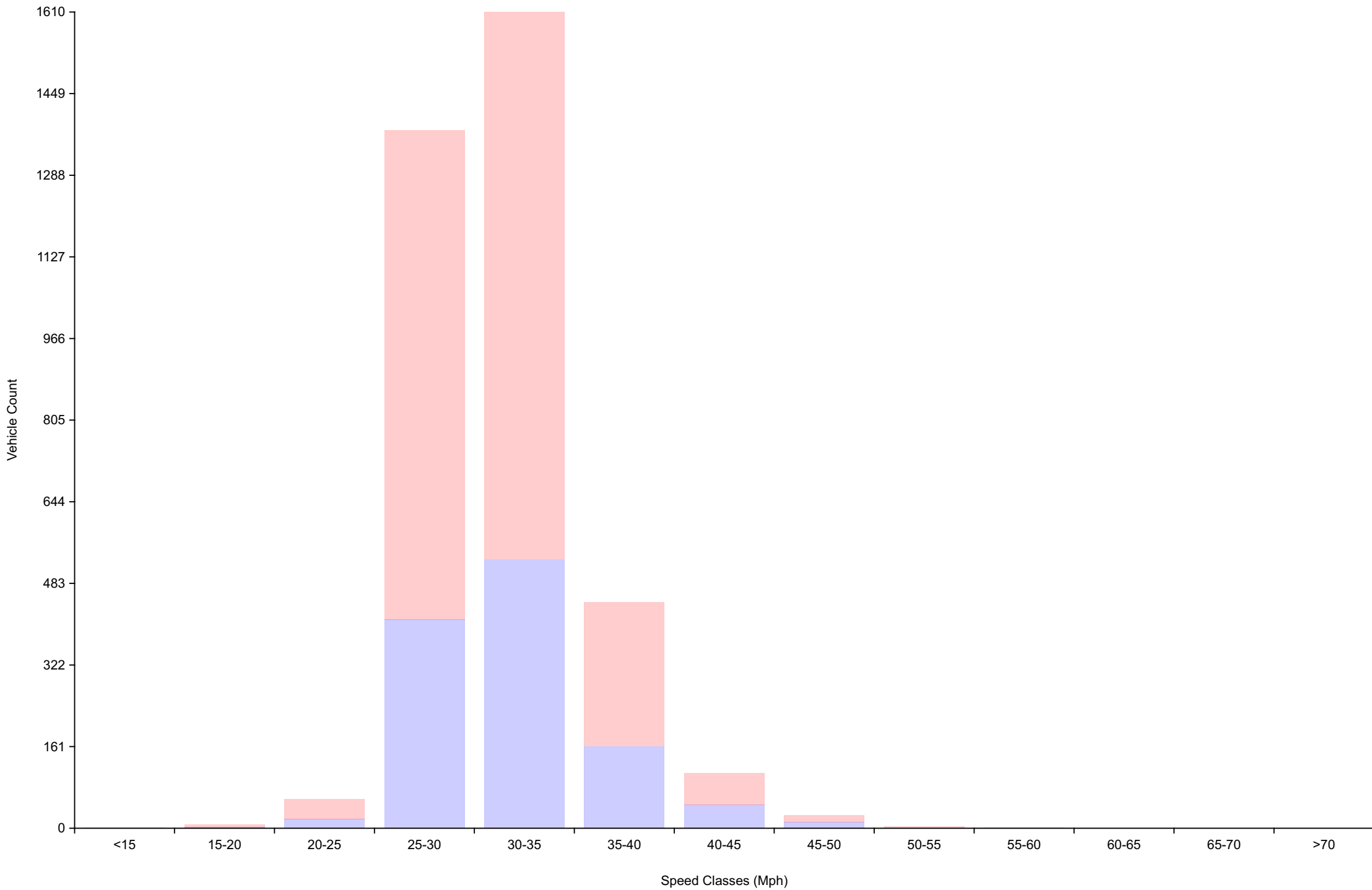
Vehicle Counts By Speed Class Daily Overview for Wed May 20 2026
