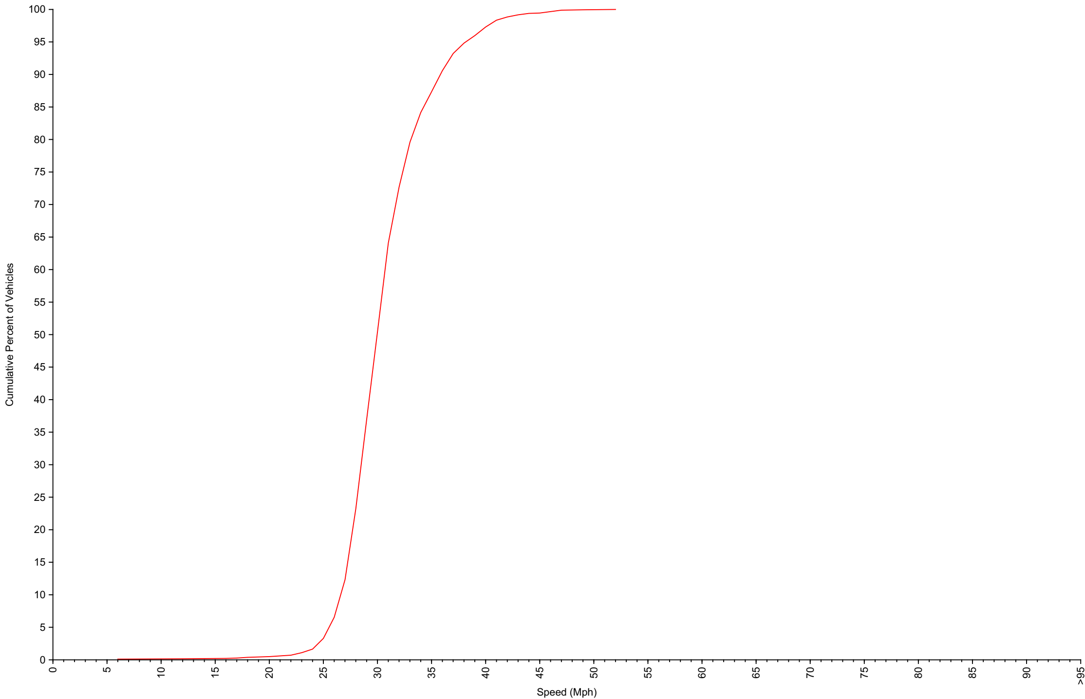
Cumulative Speed Distribution Curve Daily Overview for Sun May 10 2026
