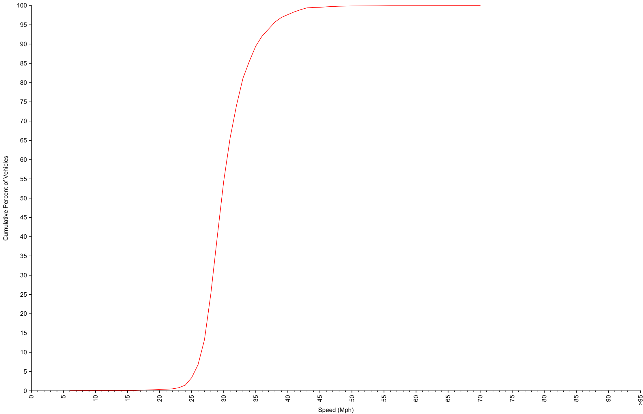
Cumulative Speed Distribution Curve Daily Overview for Tue May 5 2026
