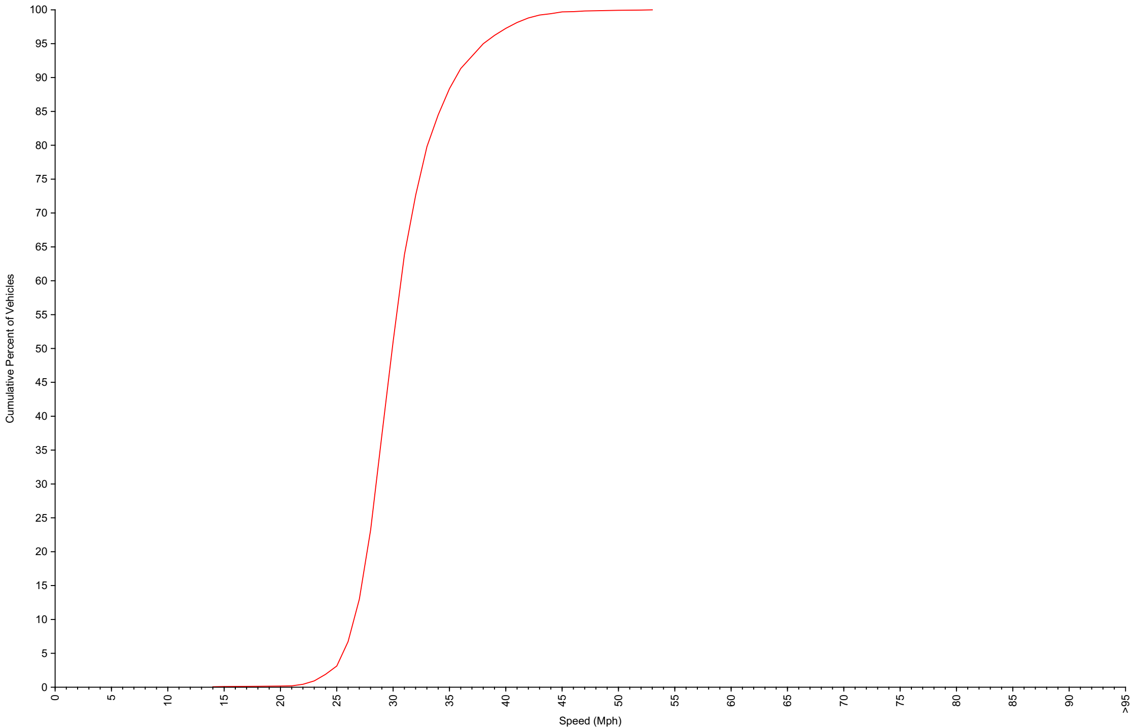
Cumulative Speed Distribution Curve Daily Overview for Wed May 6 2026
