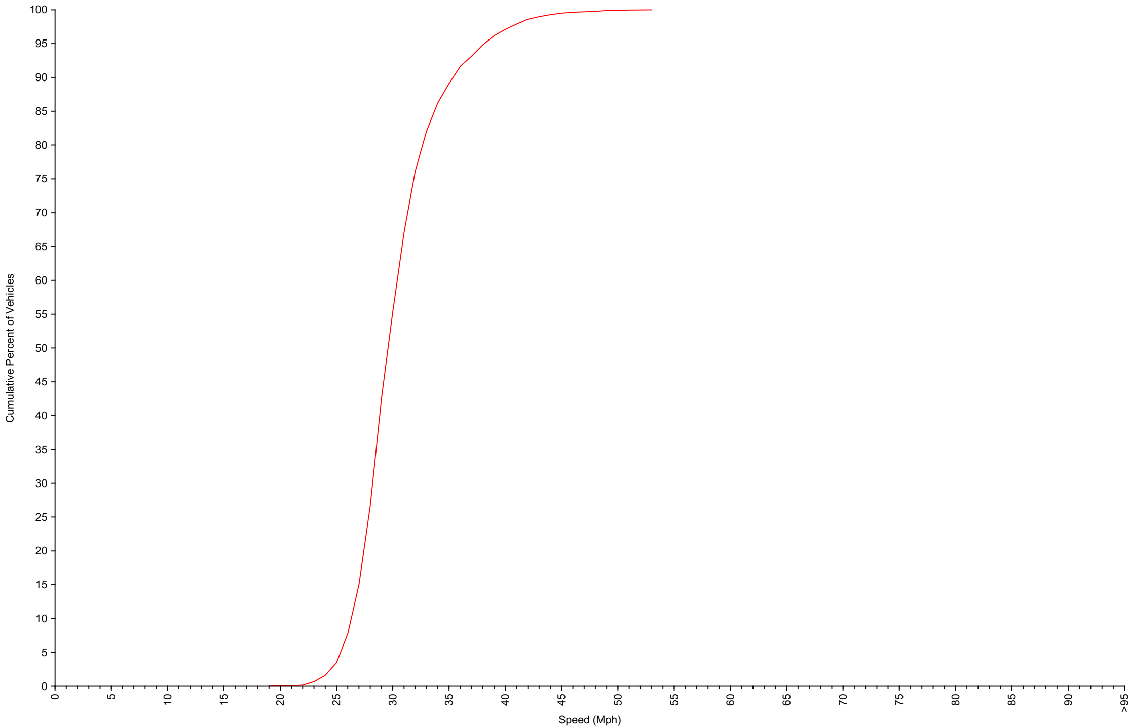
Cumulative Speed Distribution Curve Daily Overview for Mon May 18 2026
