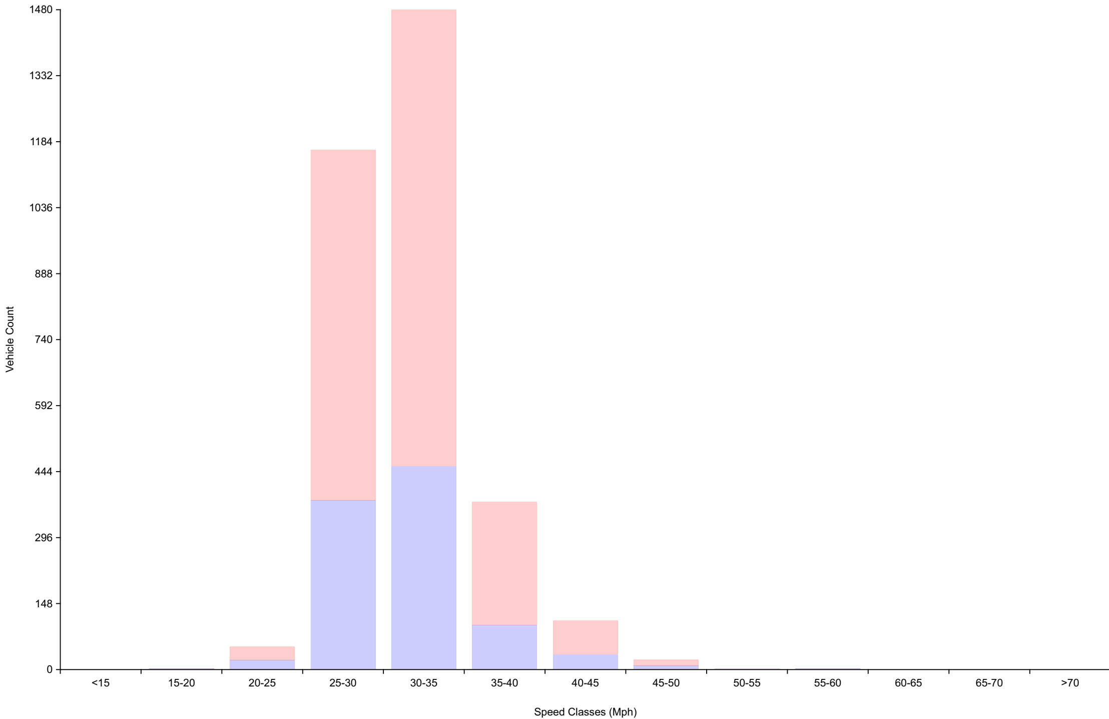
Vehicle Counts By Speed Class Daily Overview for Thu May 7 2026
