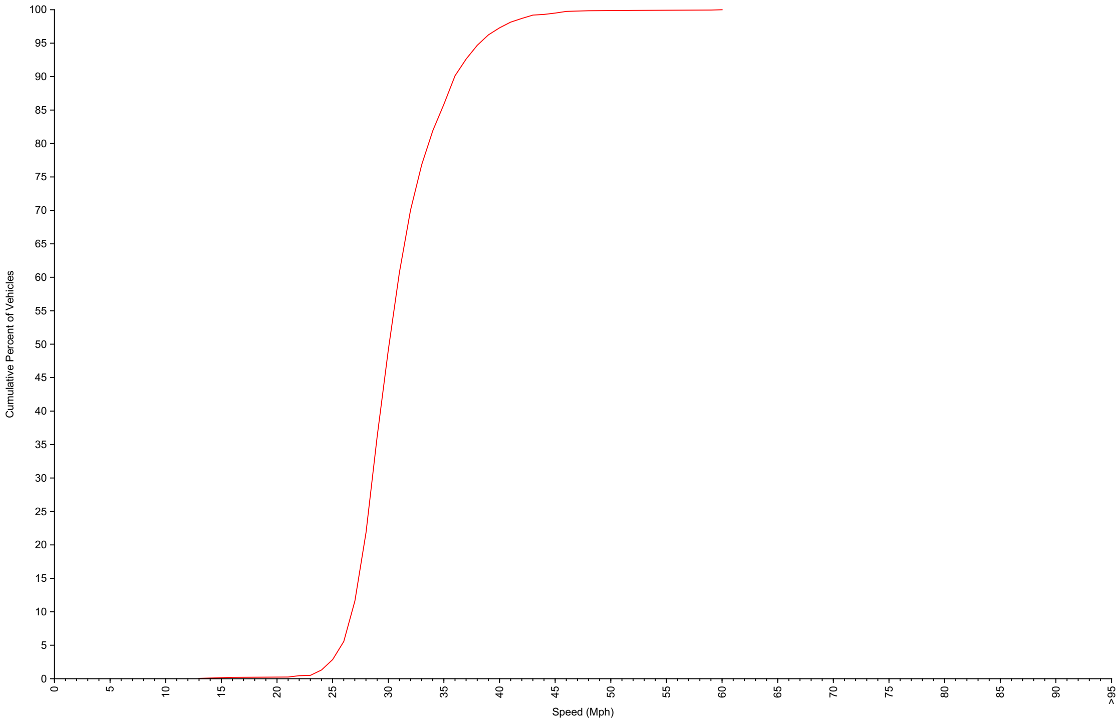
Cumulative Speed Distribution Curve Daily Overview for Mon May 4 2026
