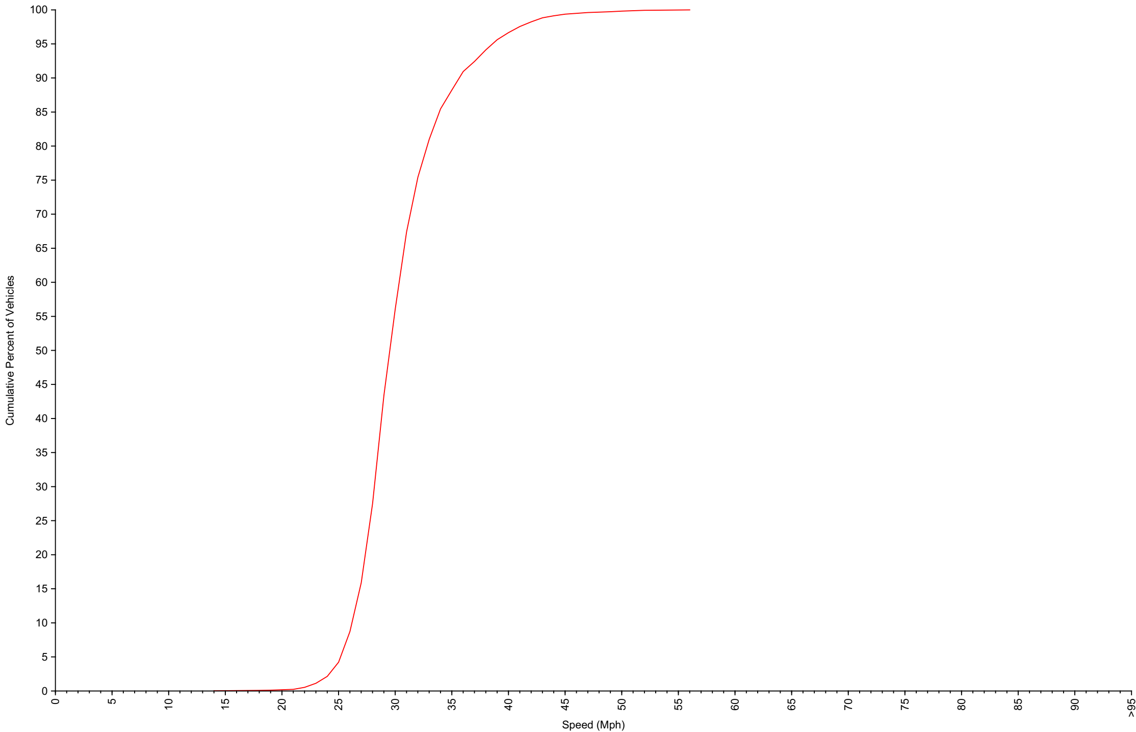
Cumulative Speed Distribution Curve Daily Overview for Tue May 12 2026
