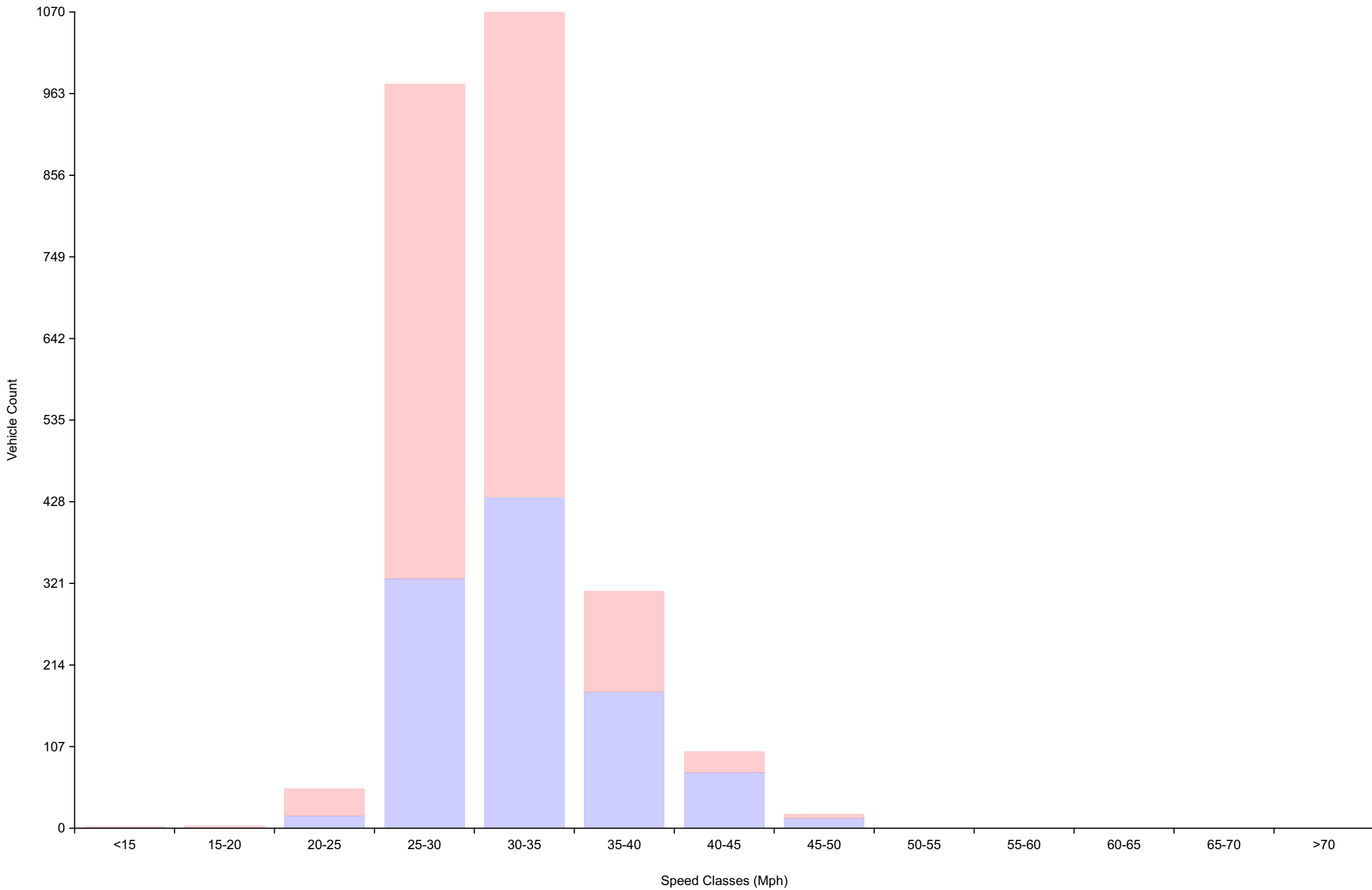
Vehicle Counts By Speed Class Daily Overview for Sat May 16 2026
