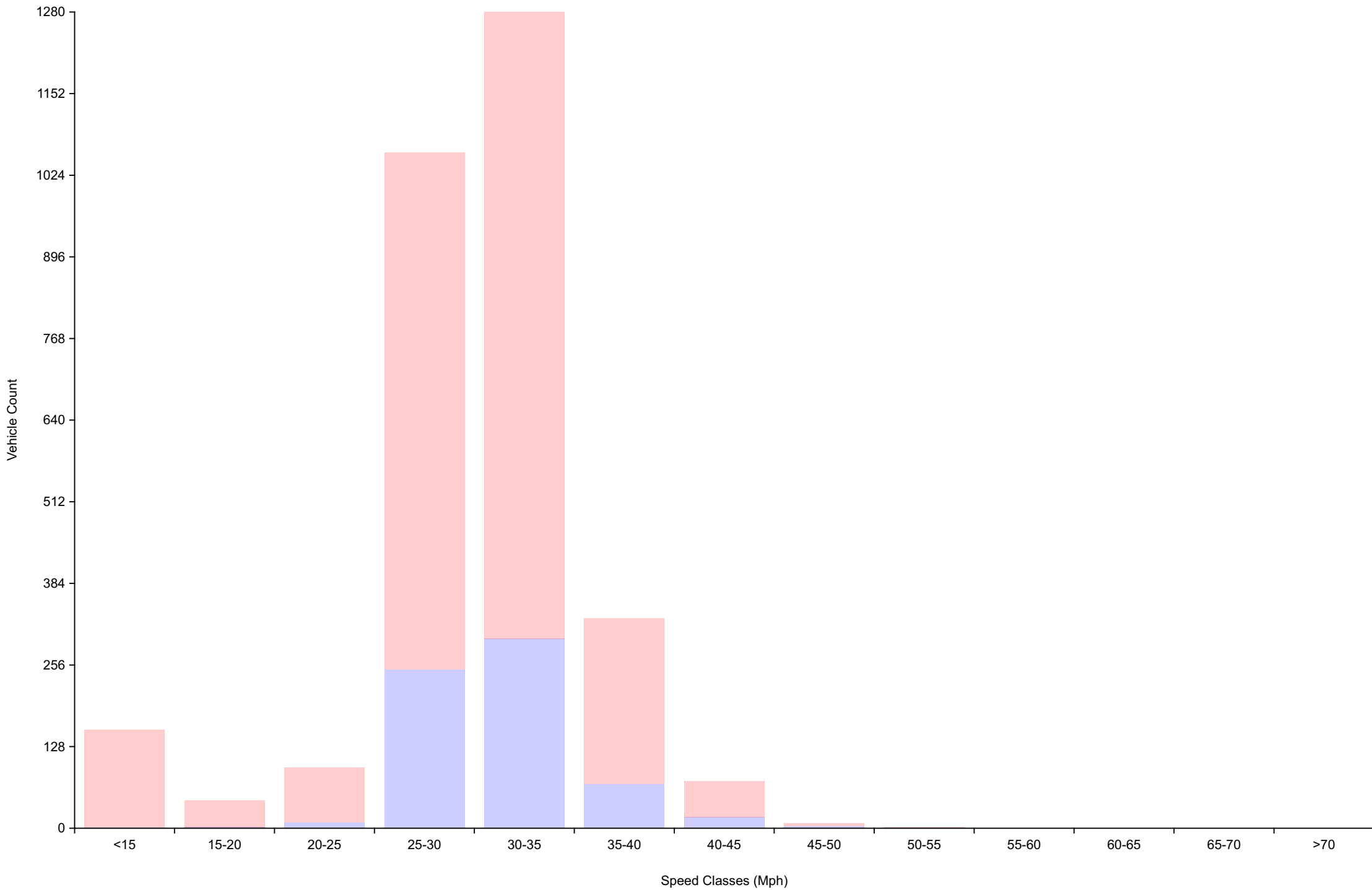
Vehicle Counts By Speed Class Daily Overview for Sat May 30 2026
