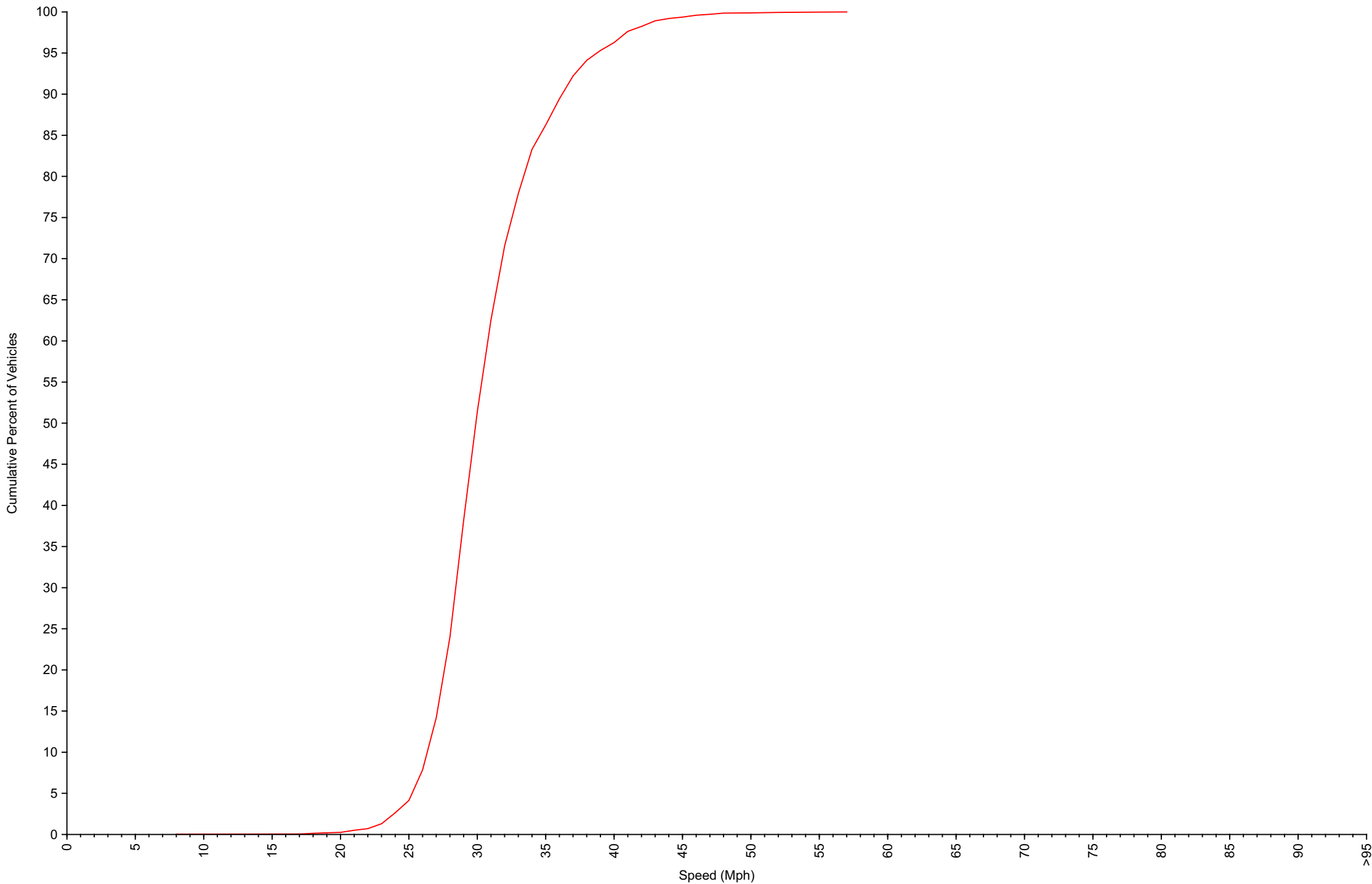
Cumulative Speed Distribution Curve Daily Overview for Thu May 14 2026
