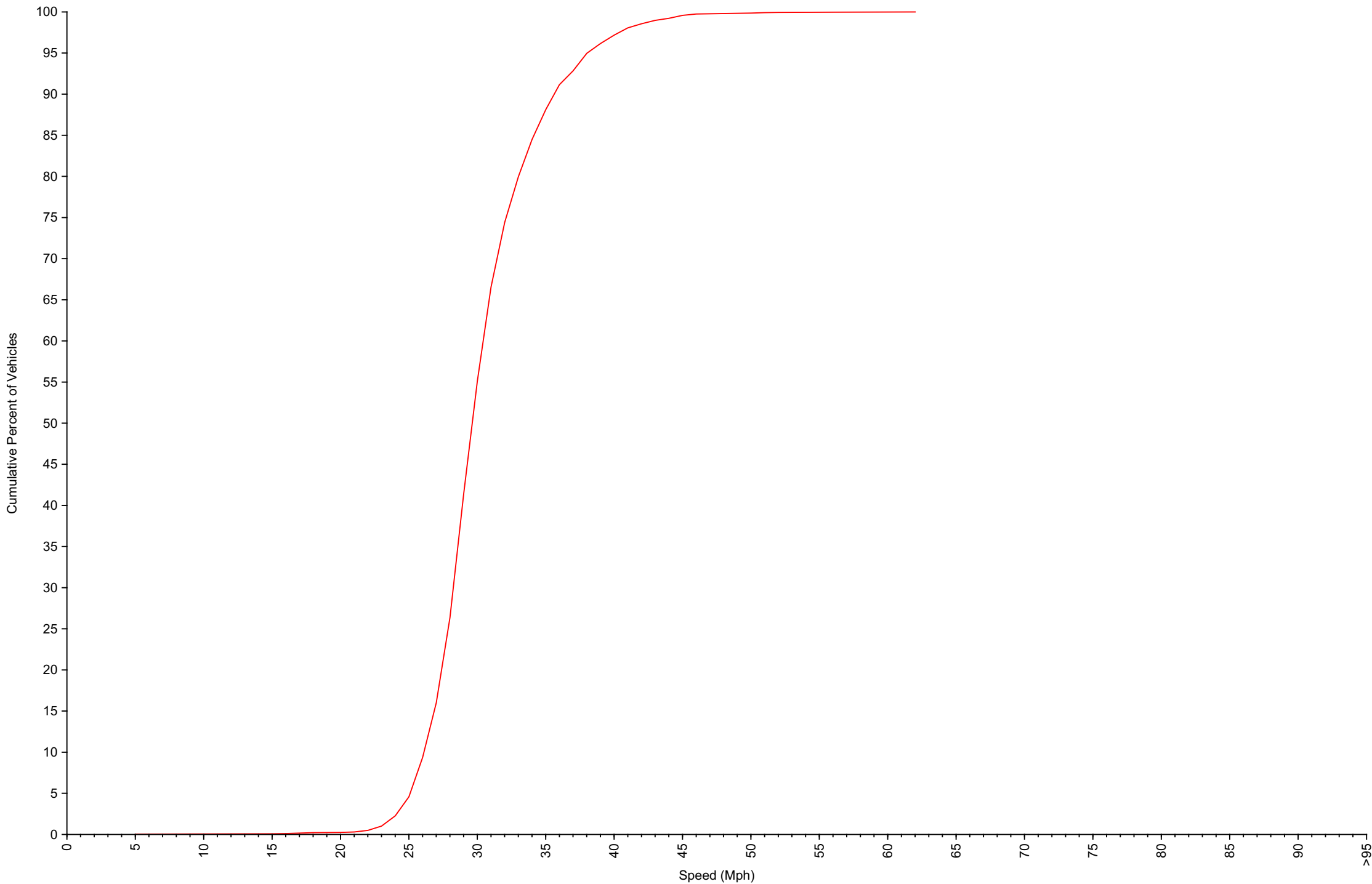
Cumulative Speed Distribution Curve Daily Overview for Fri May 15 2026
