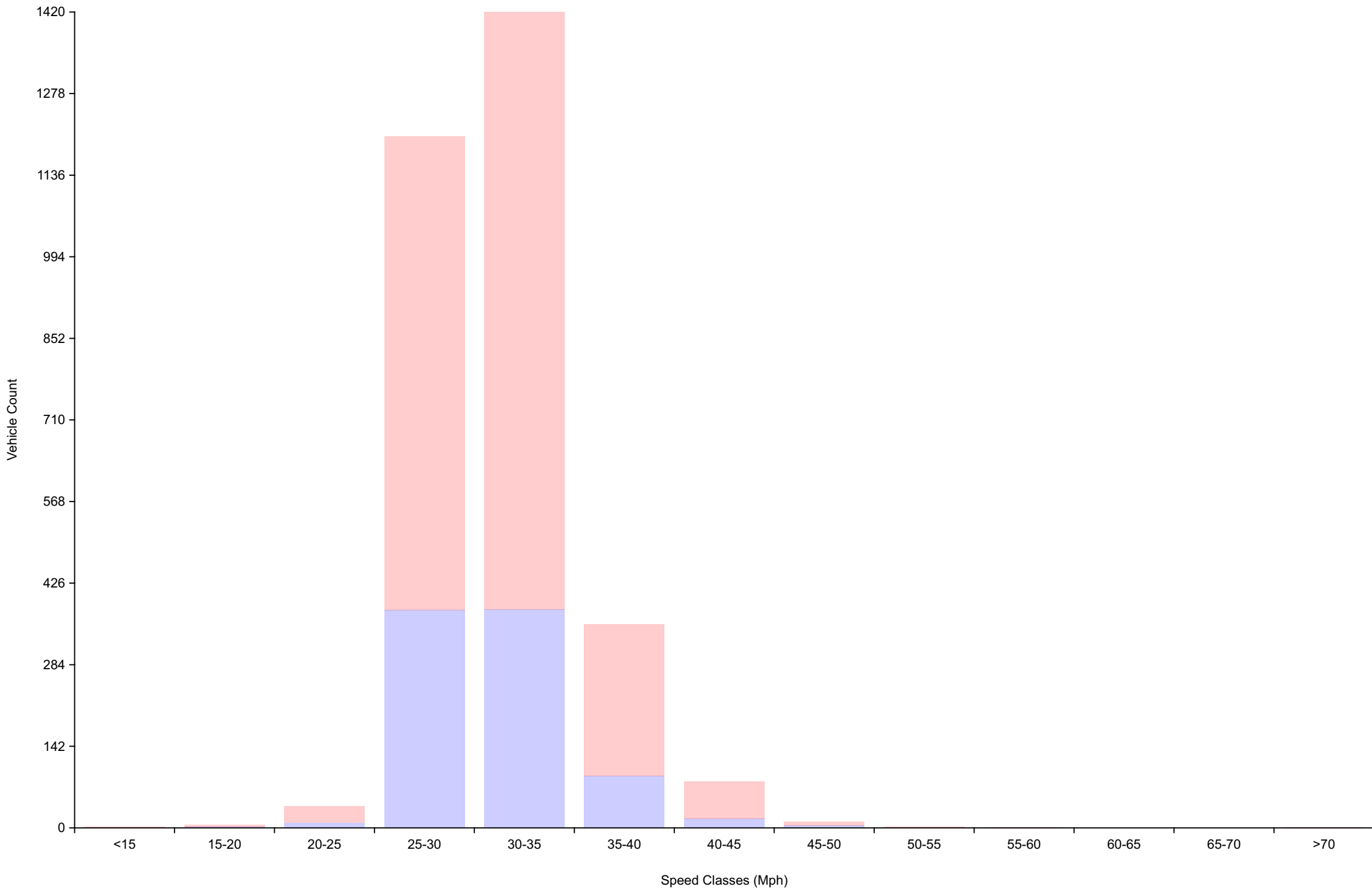
Vehicle Counts By Speed Class Daily Overview for Tue May 5 2026
