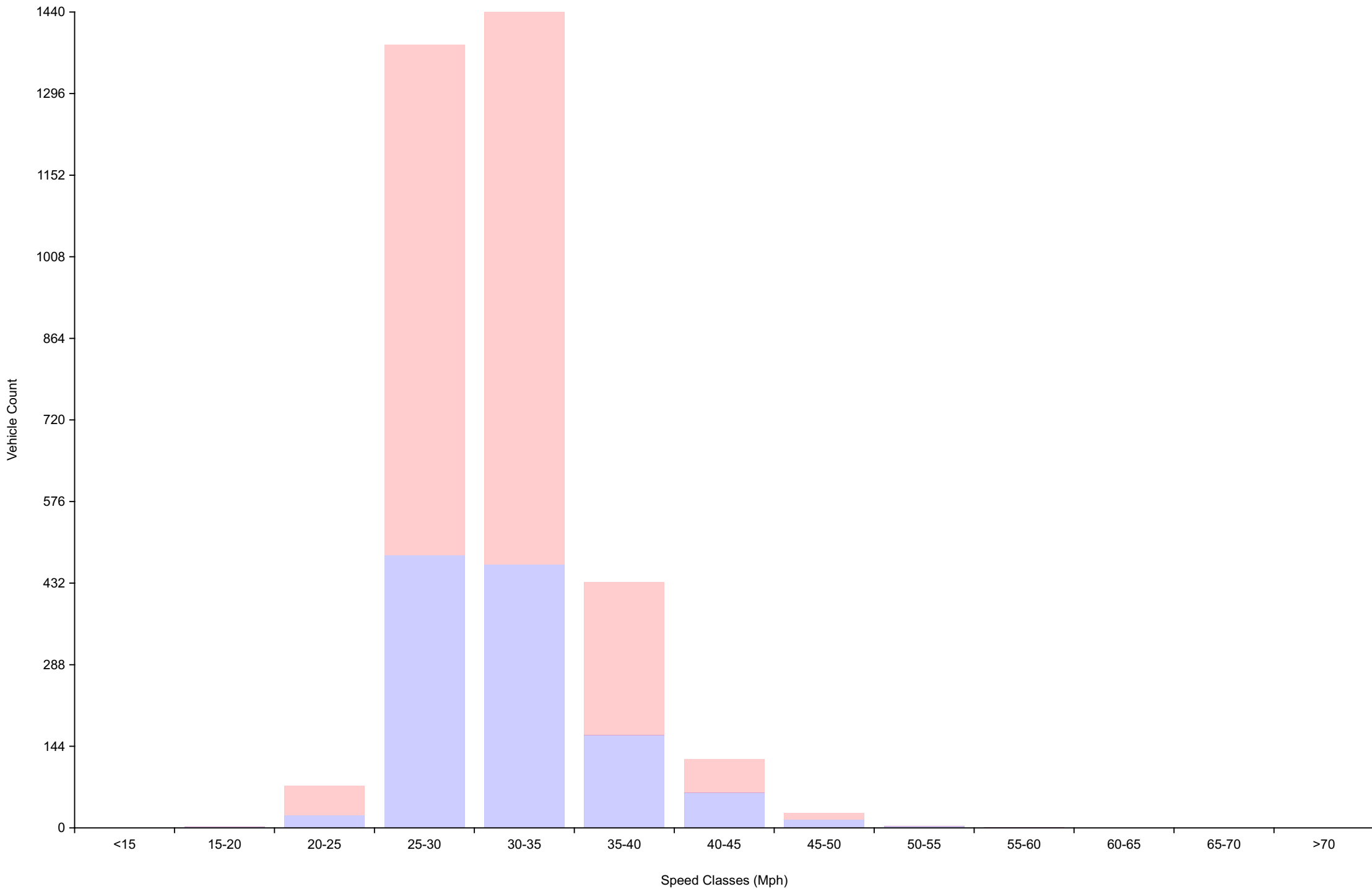
Vehicle Counts By Speed Class Daily Overview for Tue May 19 2026
