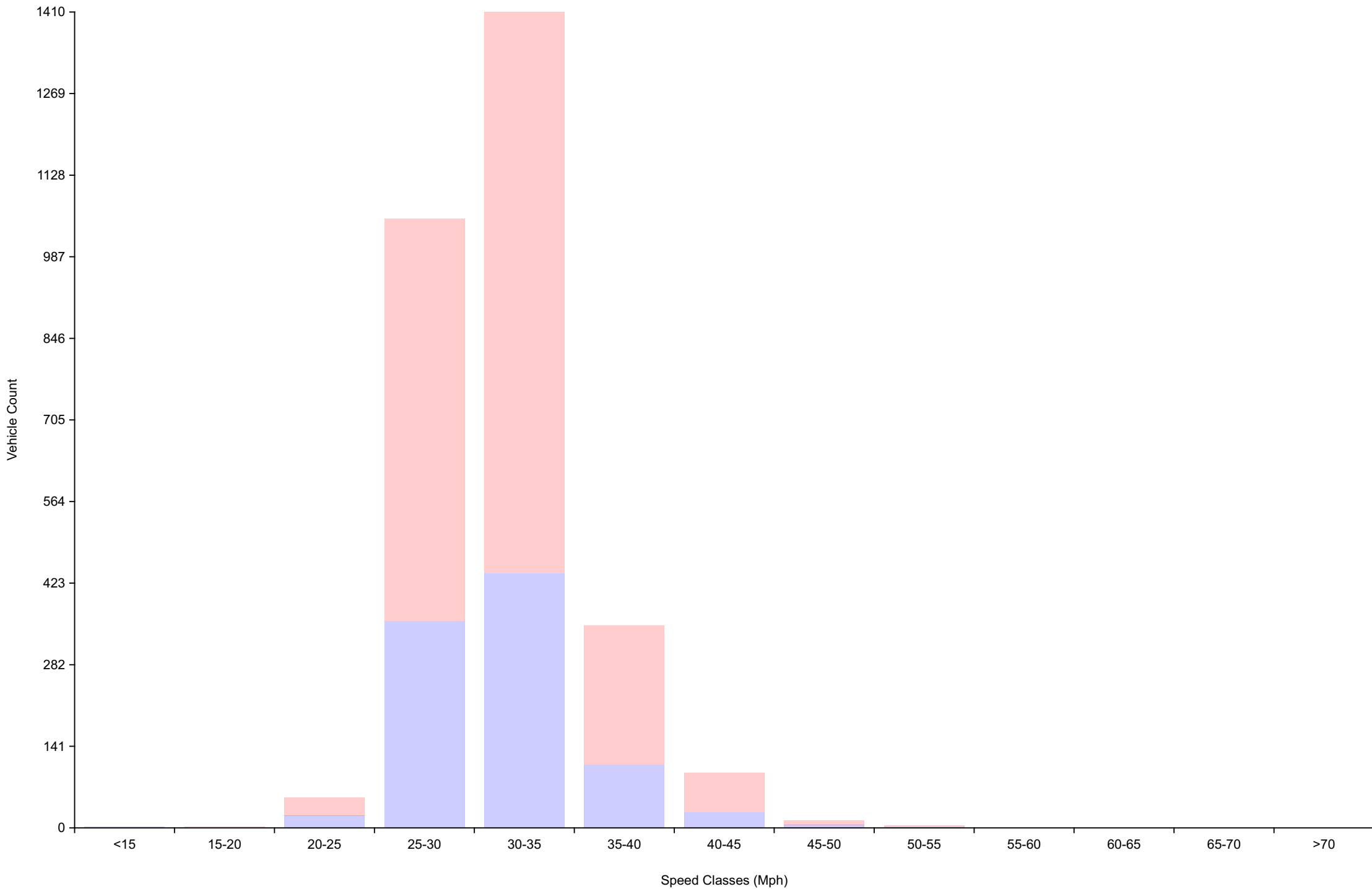
Vehicle Counts By Speed Class Daily Overview for Wed May 6 2026
