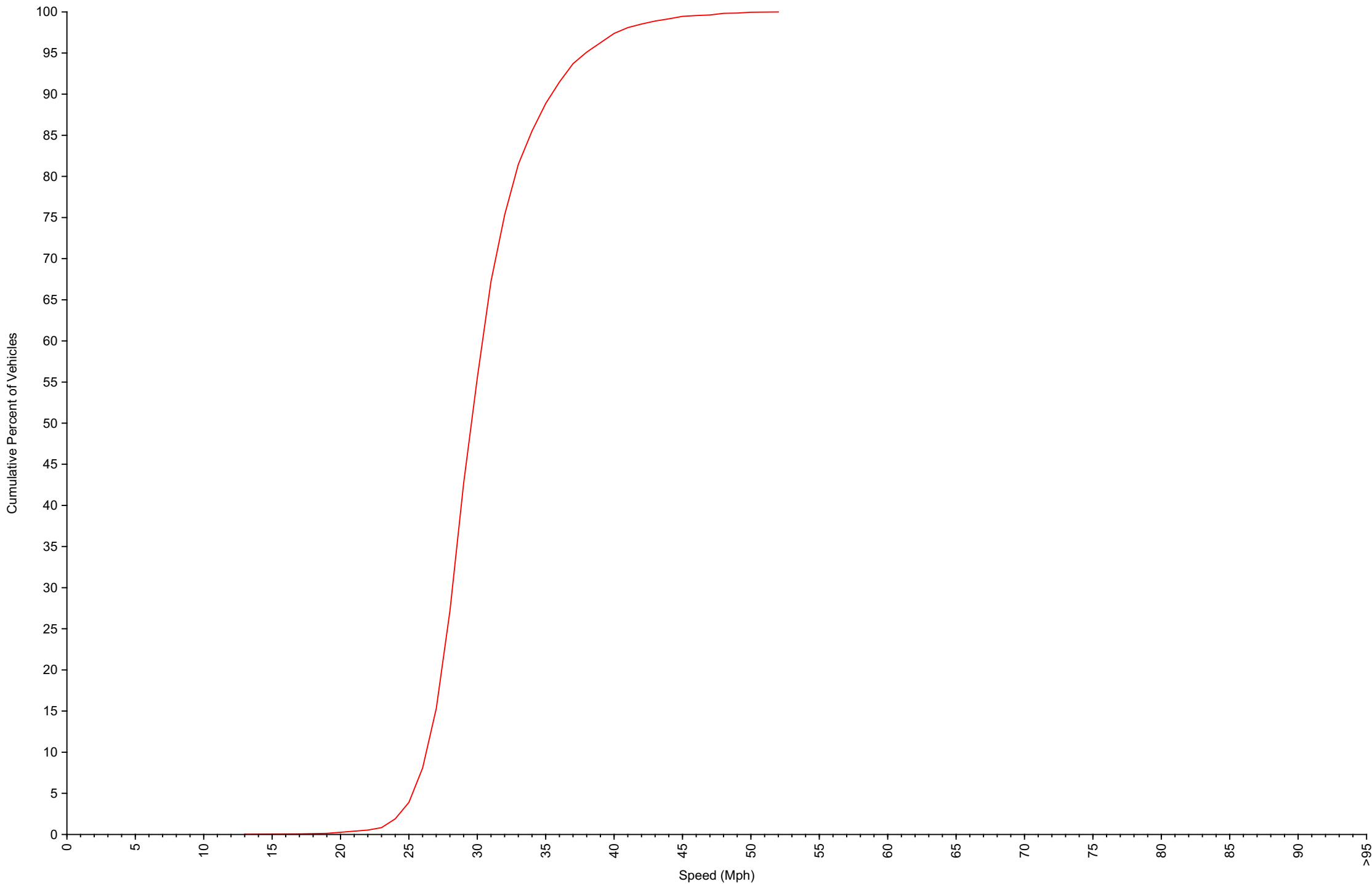
Cumulative Speed Distribution Curve Daily Overview for Mon May 11 2026
