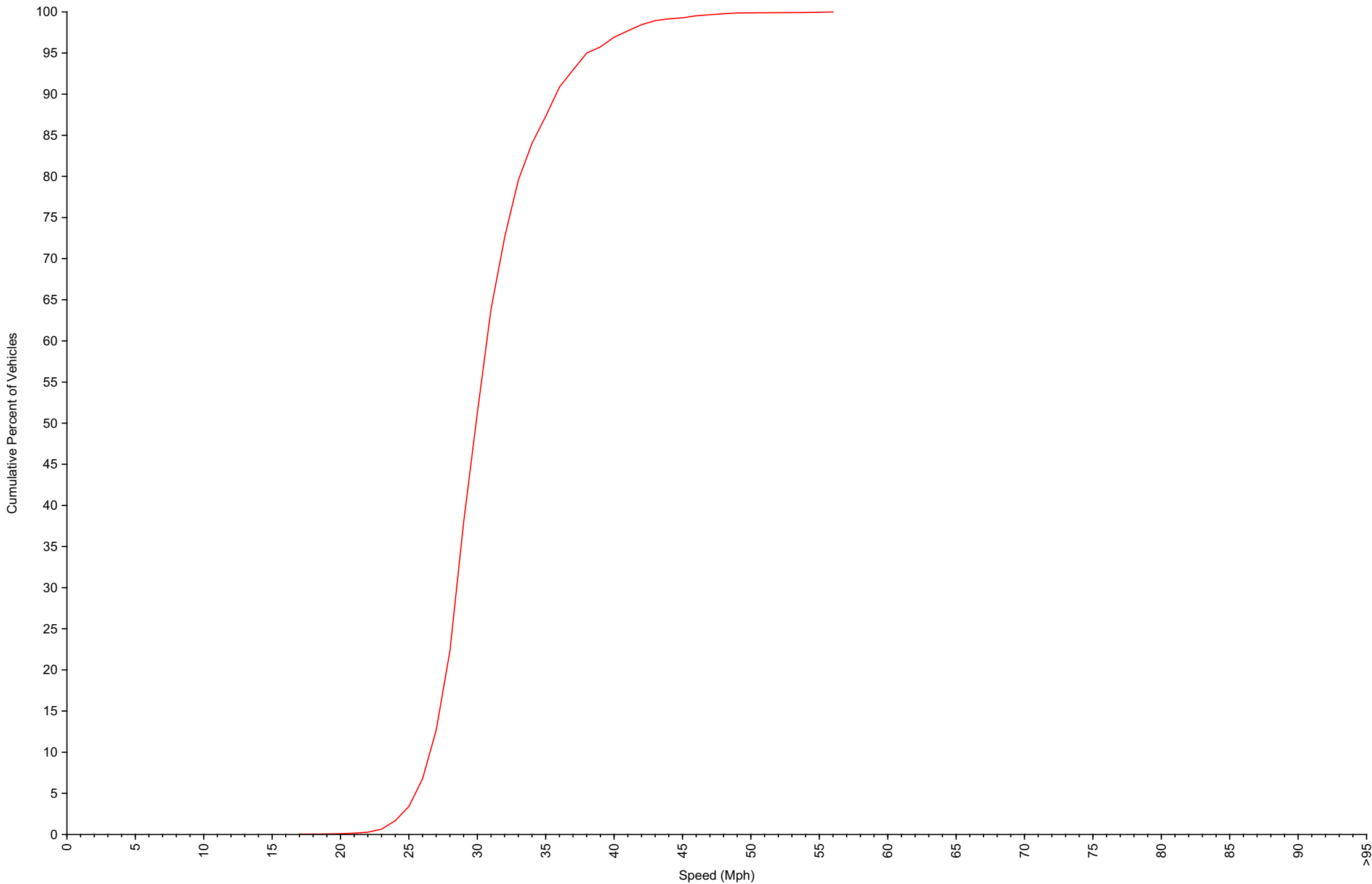
Cumulative Speed Distribution Curve Daily Overview for Thu May 7 2026
