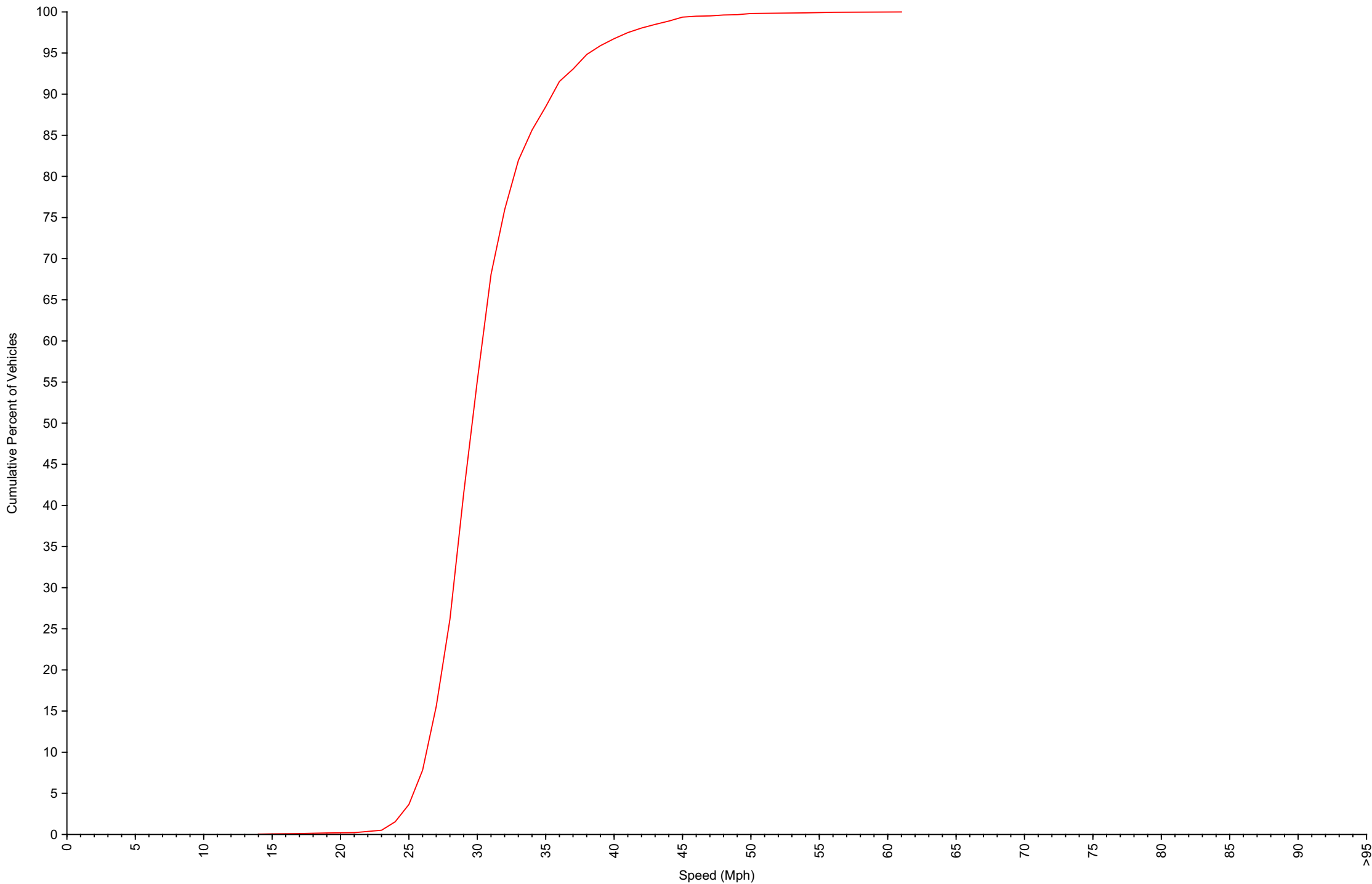
Cumulative Speed Distribution Curve Daily Overview for Thu May 28 2026
