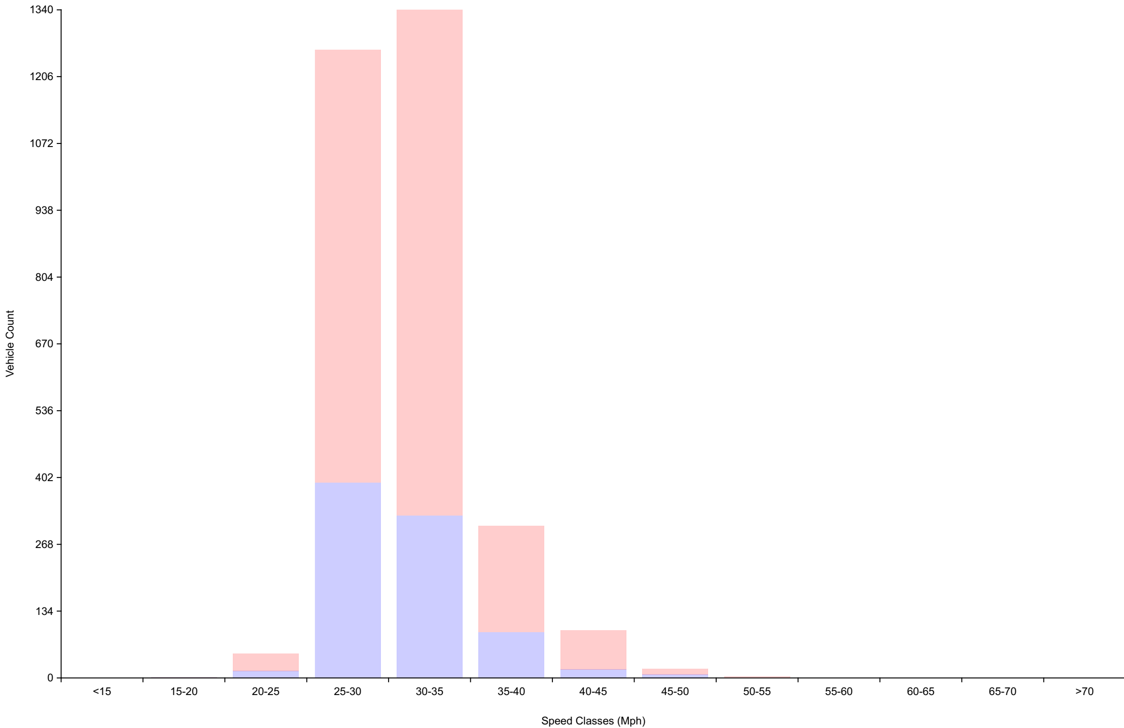
Vehicle Counts By Speed Class Daily Overview for Mon May 18 2026
