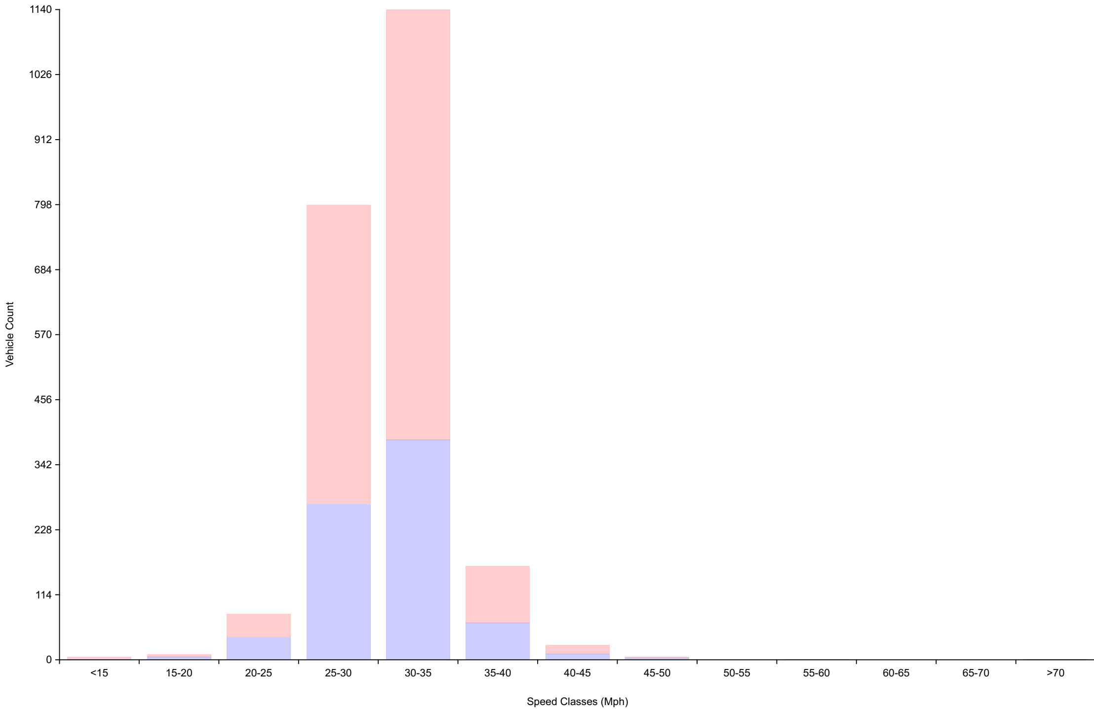
Vehicle Counts By Speed Class Daily Overview for Tue Dec 23 2025
