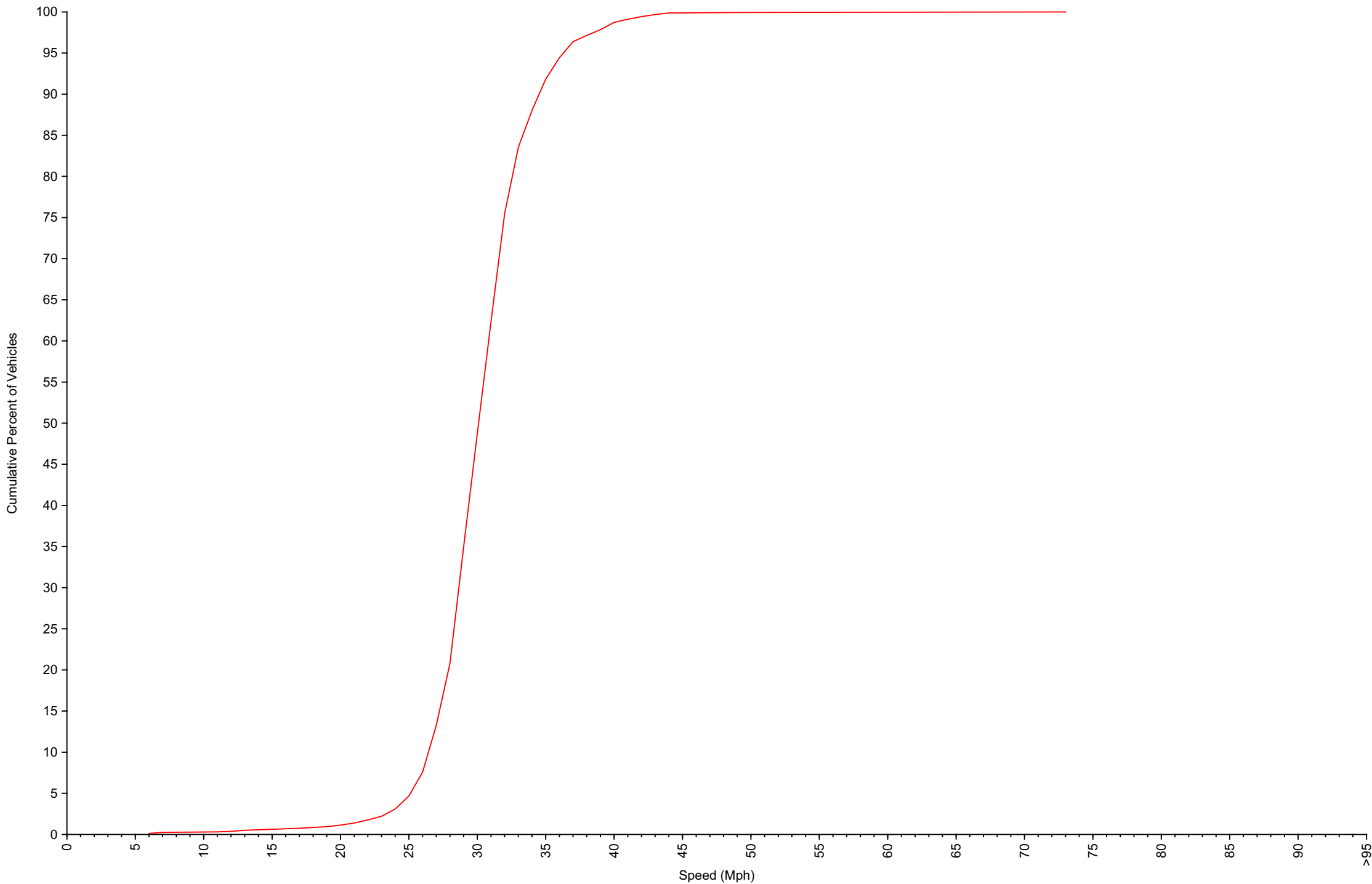
Cumulative Speed Distribution Curve Daily Overview for Wed Dec 31 2025
