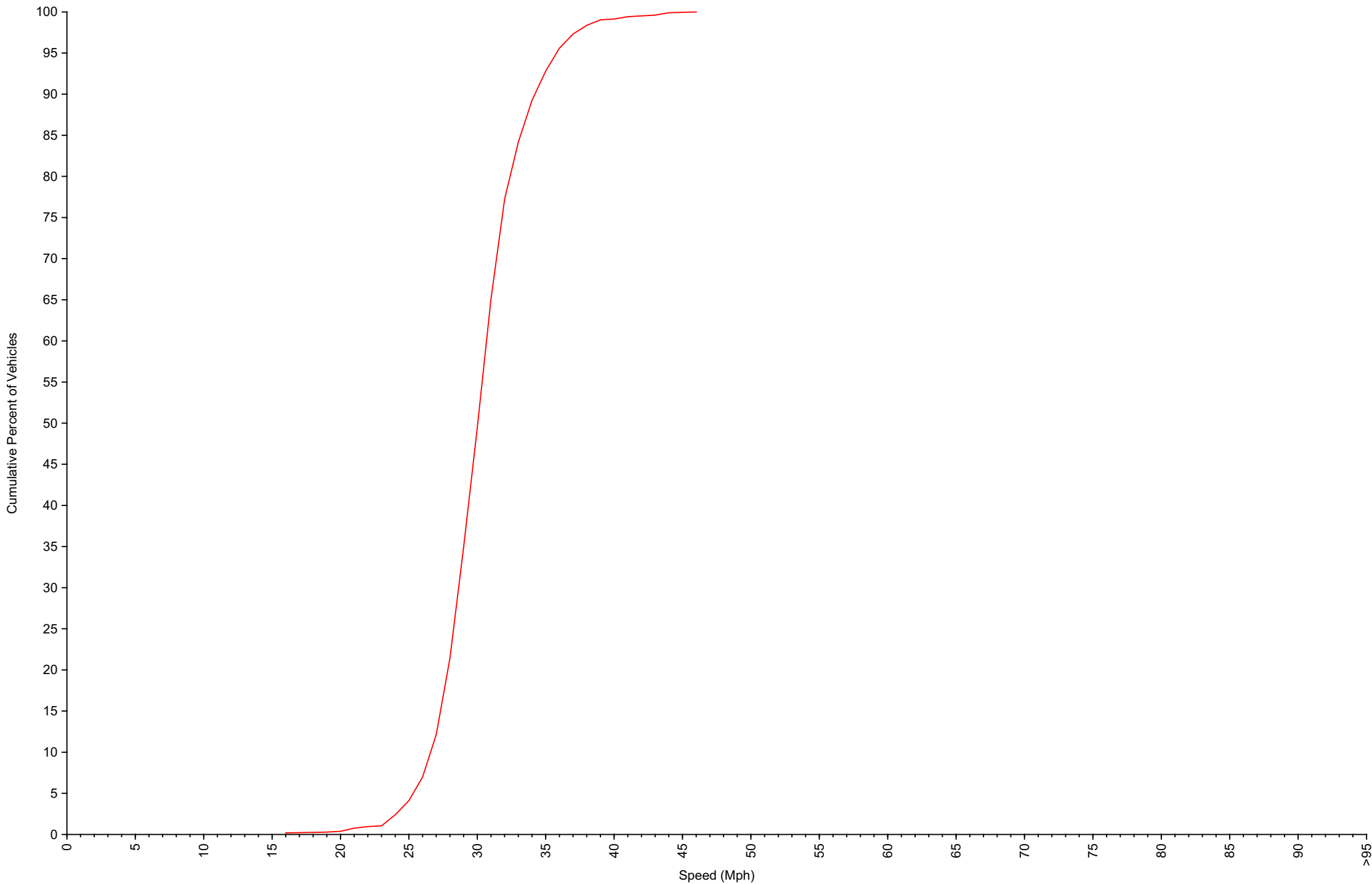
Cumulative Speed Distribution Curve Daily Overview for Fri Dec 19 2025
