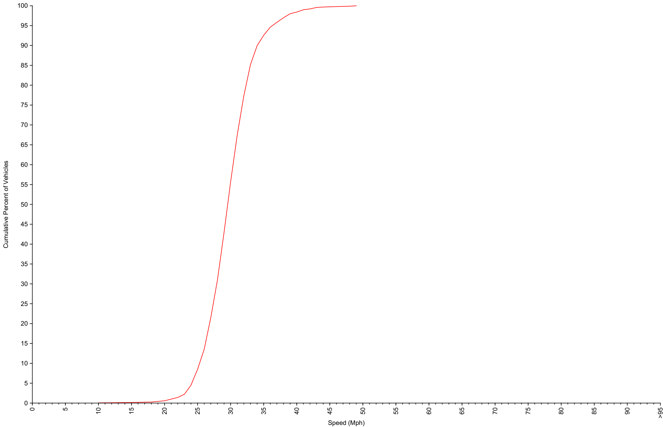
Cumulative Speed Distribution Curve Daily Overview for Sat Dec 20 2025
