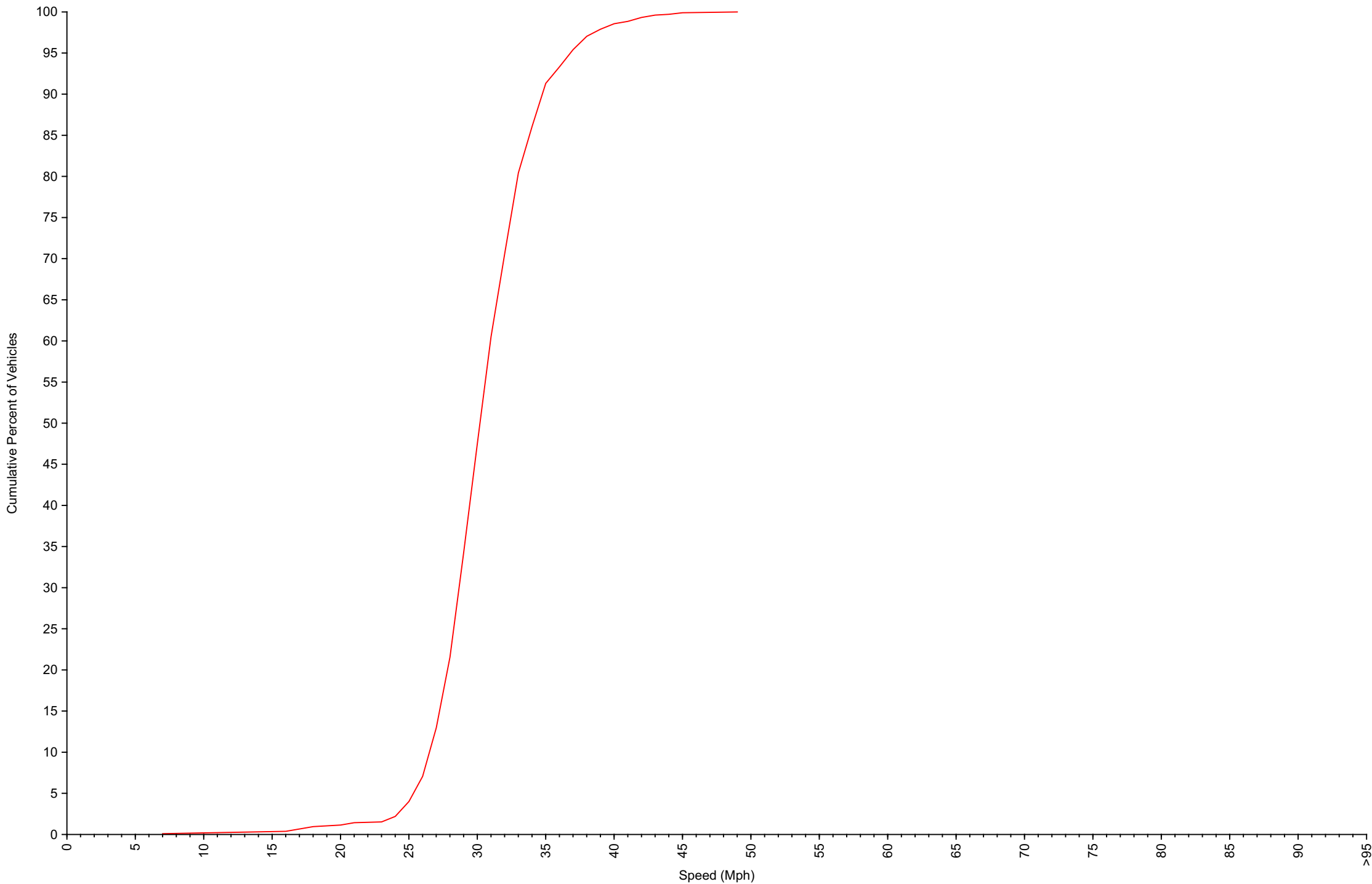
Cumulative Speed Distribution Curve Daily Overview for Fri Dec 26 2025
