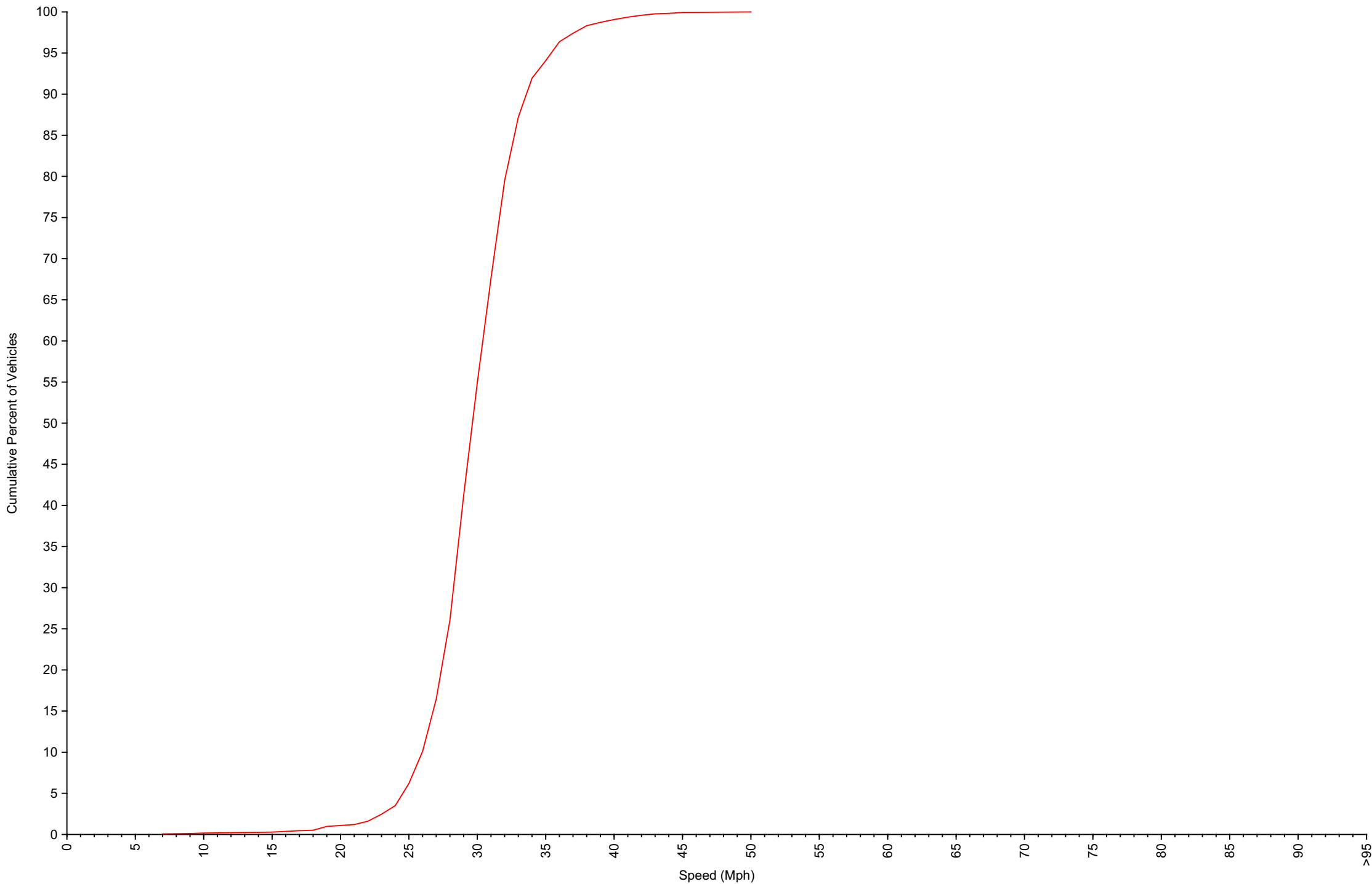
Cumulative Speed Distribution Curve Daily Overview for Tue Dec 30 2025
