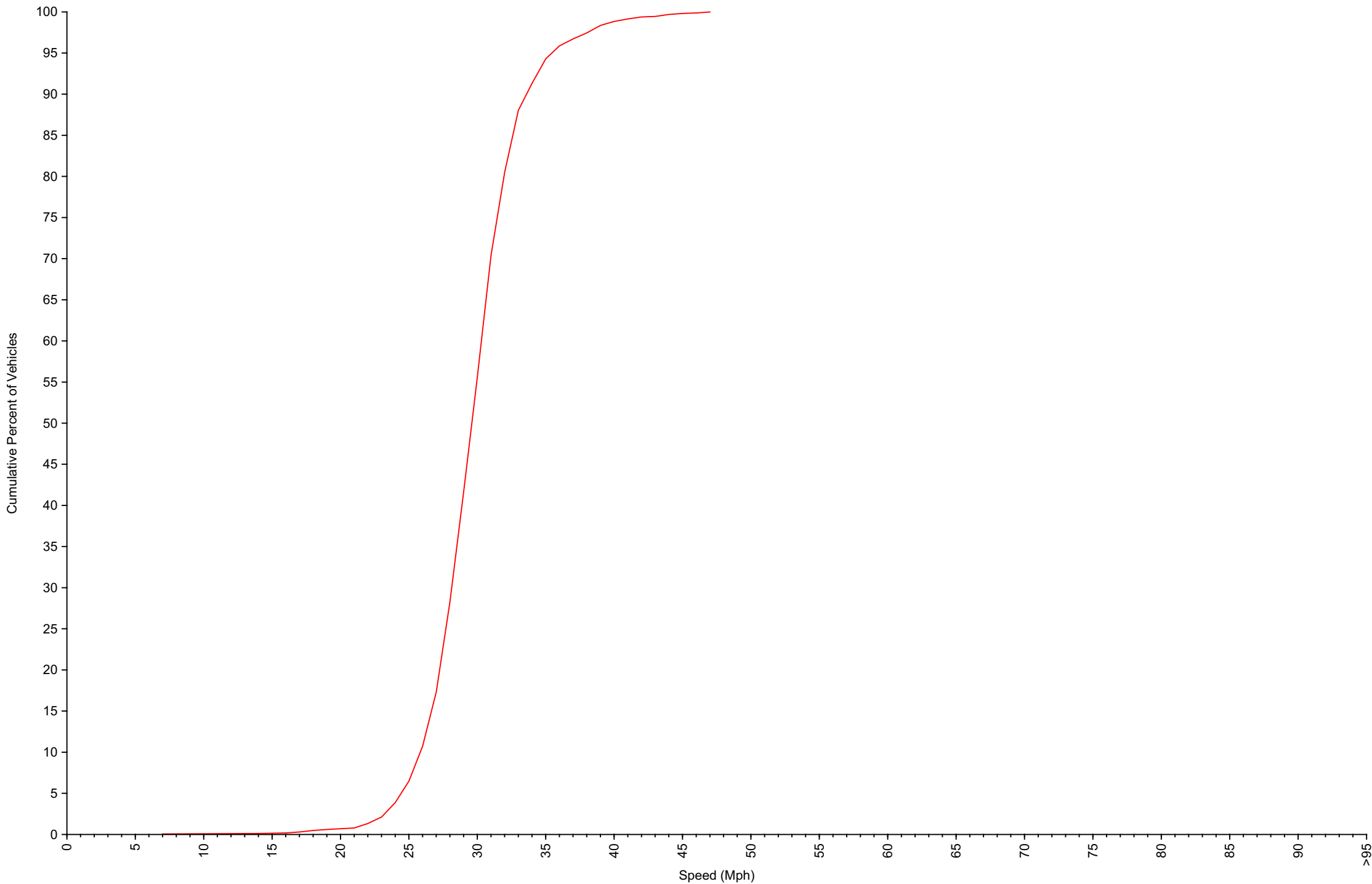
Cumulative Speed Distribution Curve Daily Overview for Mon Dec 29 2025
