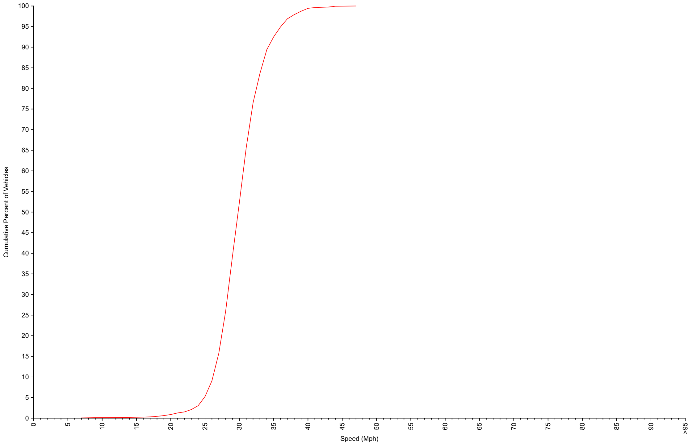
Cumulative Speed Distribution Curve Daily Overview for Sun Dec 21 2025
