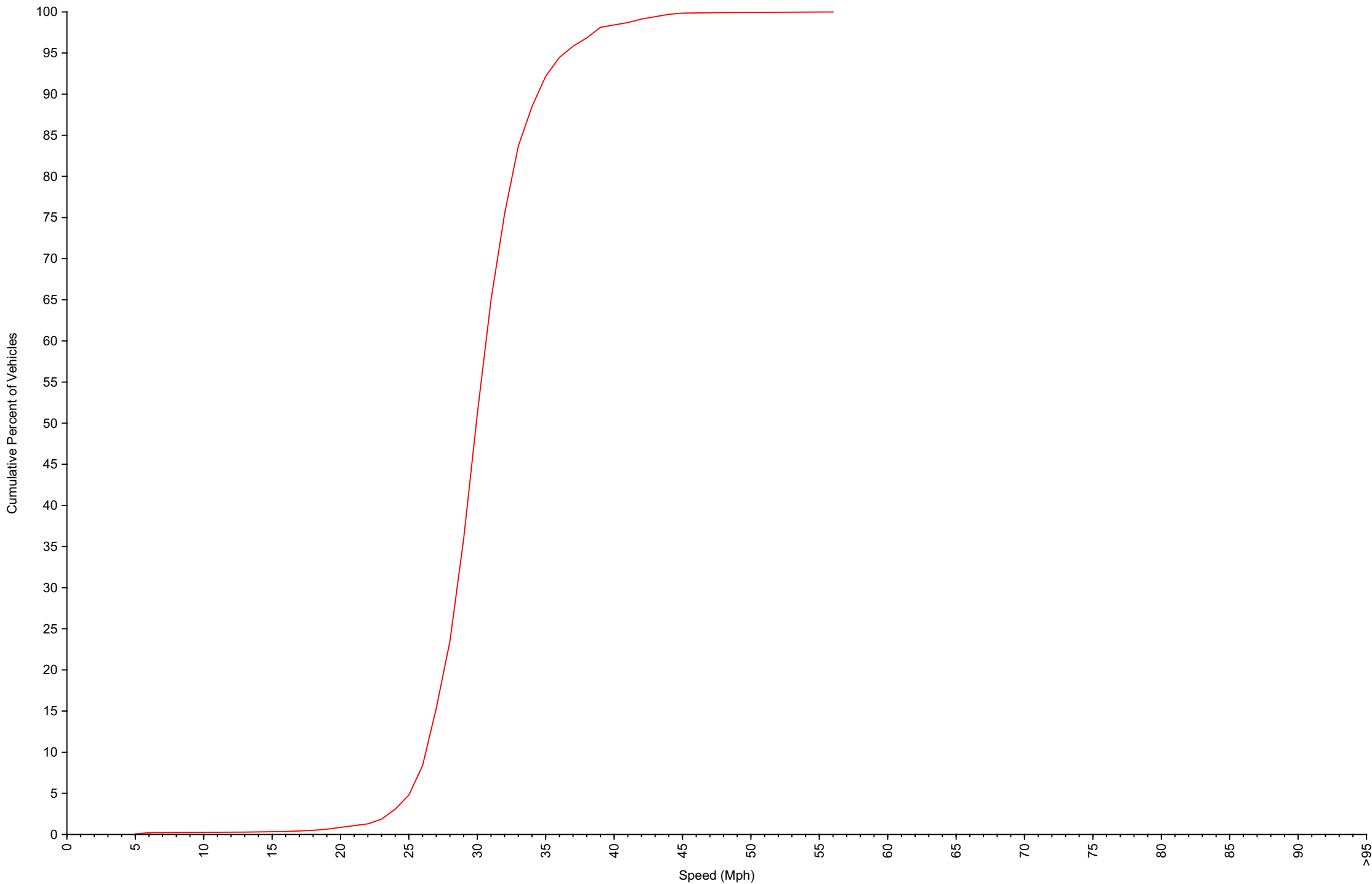
Cumulative Speed Distribution Curve Daily Overview for Sat Dec 27 2025
