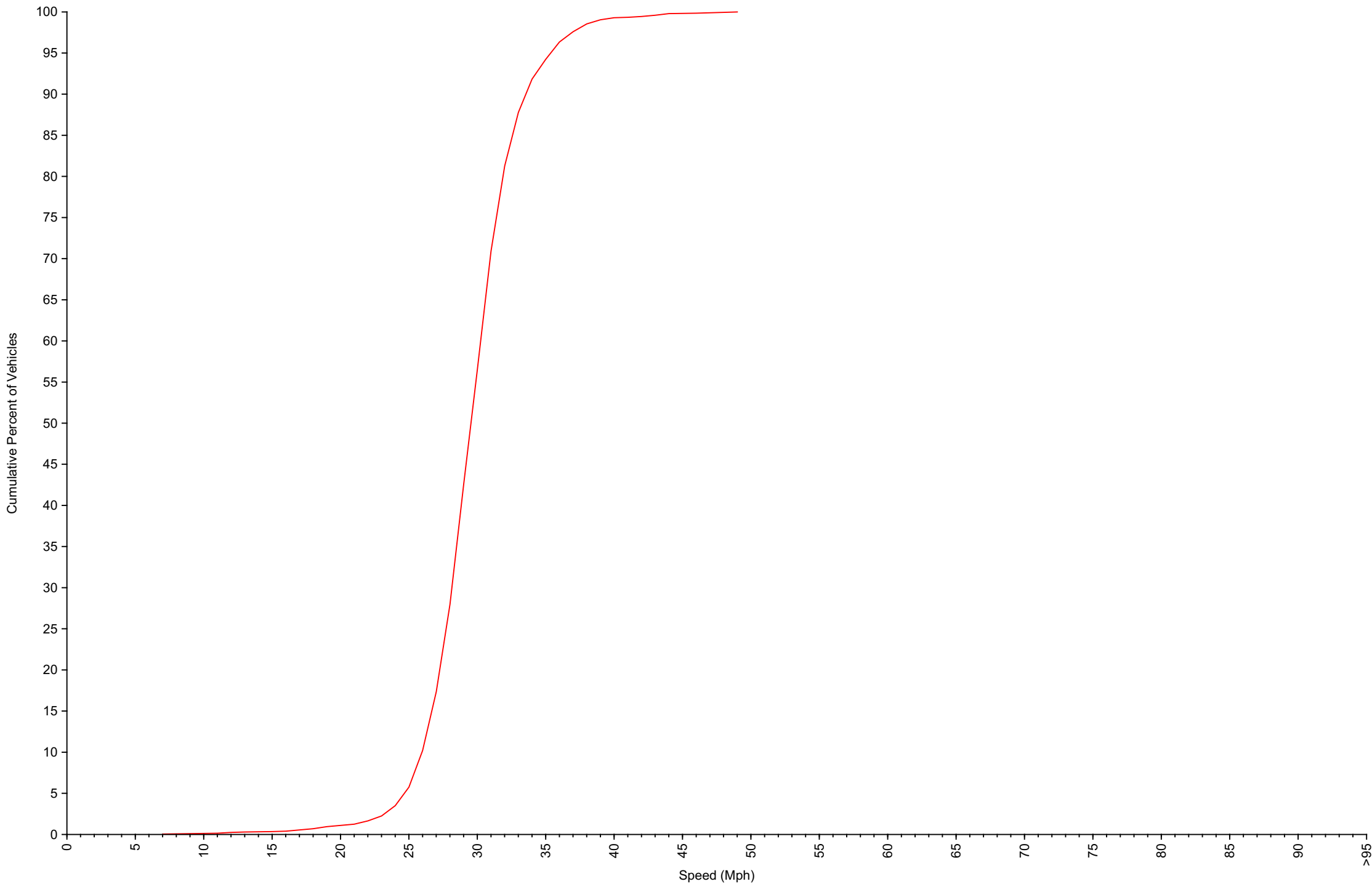
Cumulative Speed Distribution Curve Daily Overview for Tue Jan 27 2026
