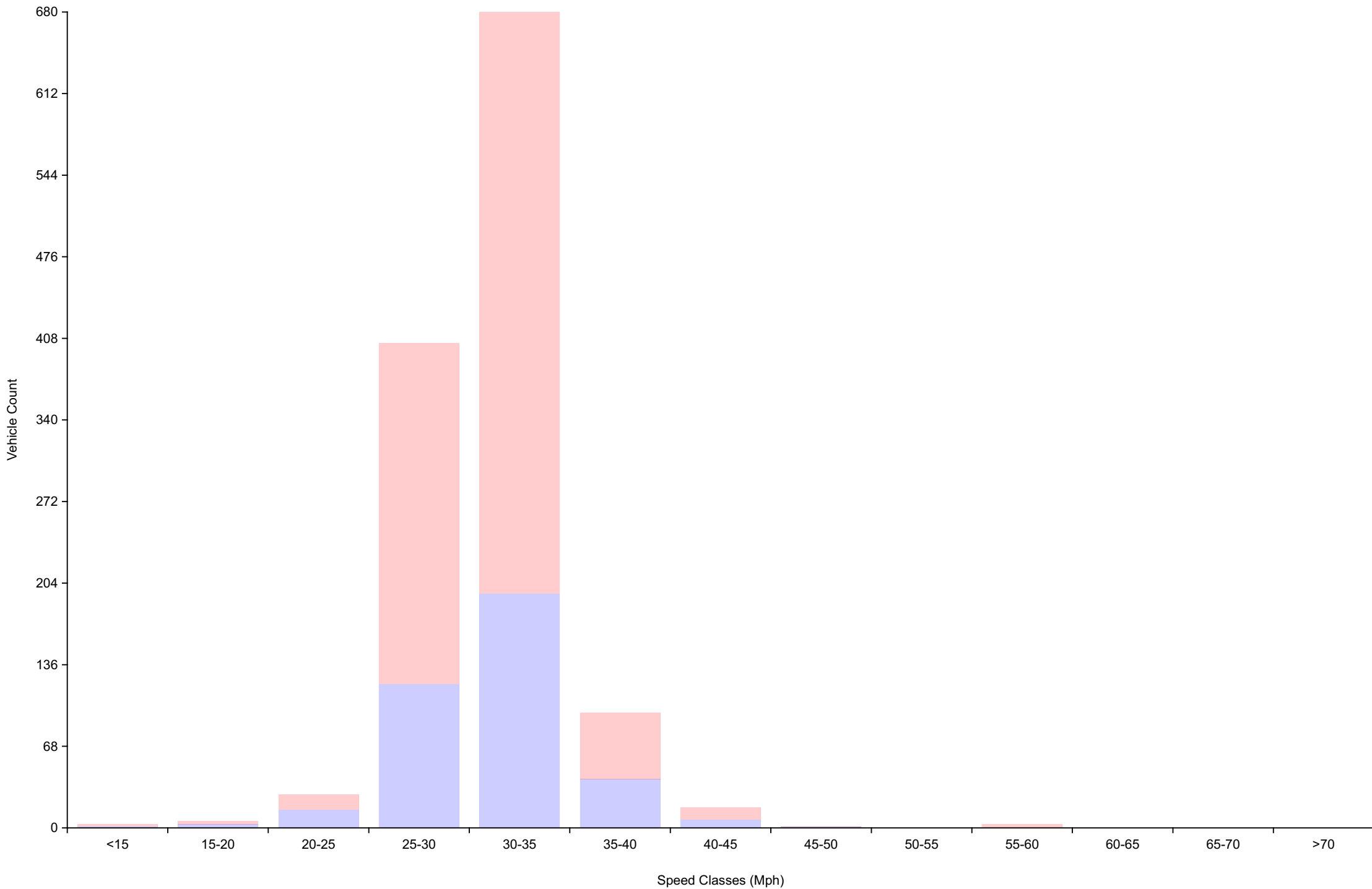
Vehicle Counts By Speed Class Daily Overview for Sun Jan 18 2026
