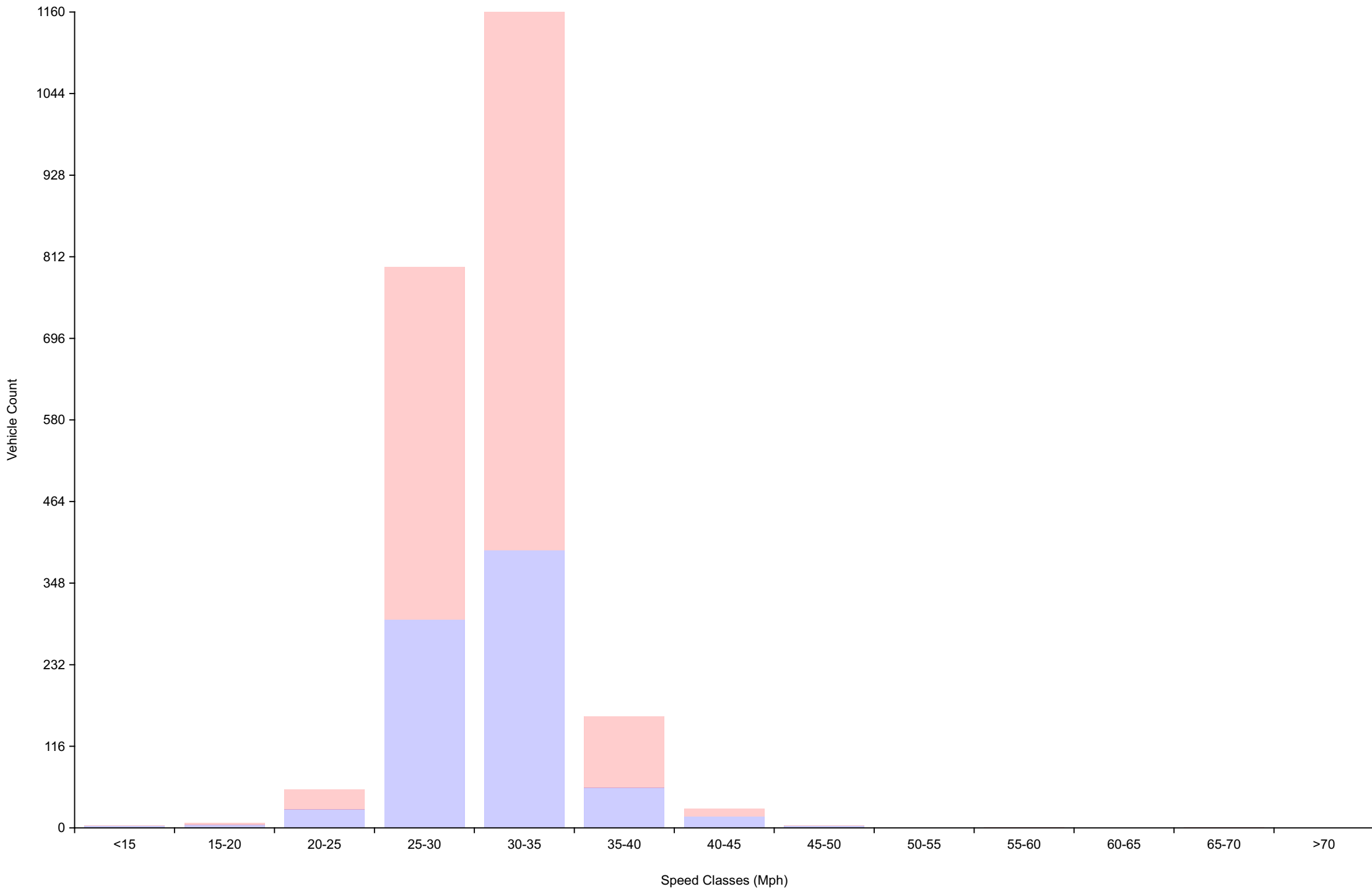
Vehicle Counts By Speed Class Daily Overview for Wed Jan 21 2026
