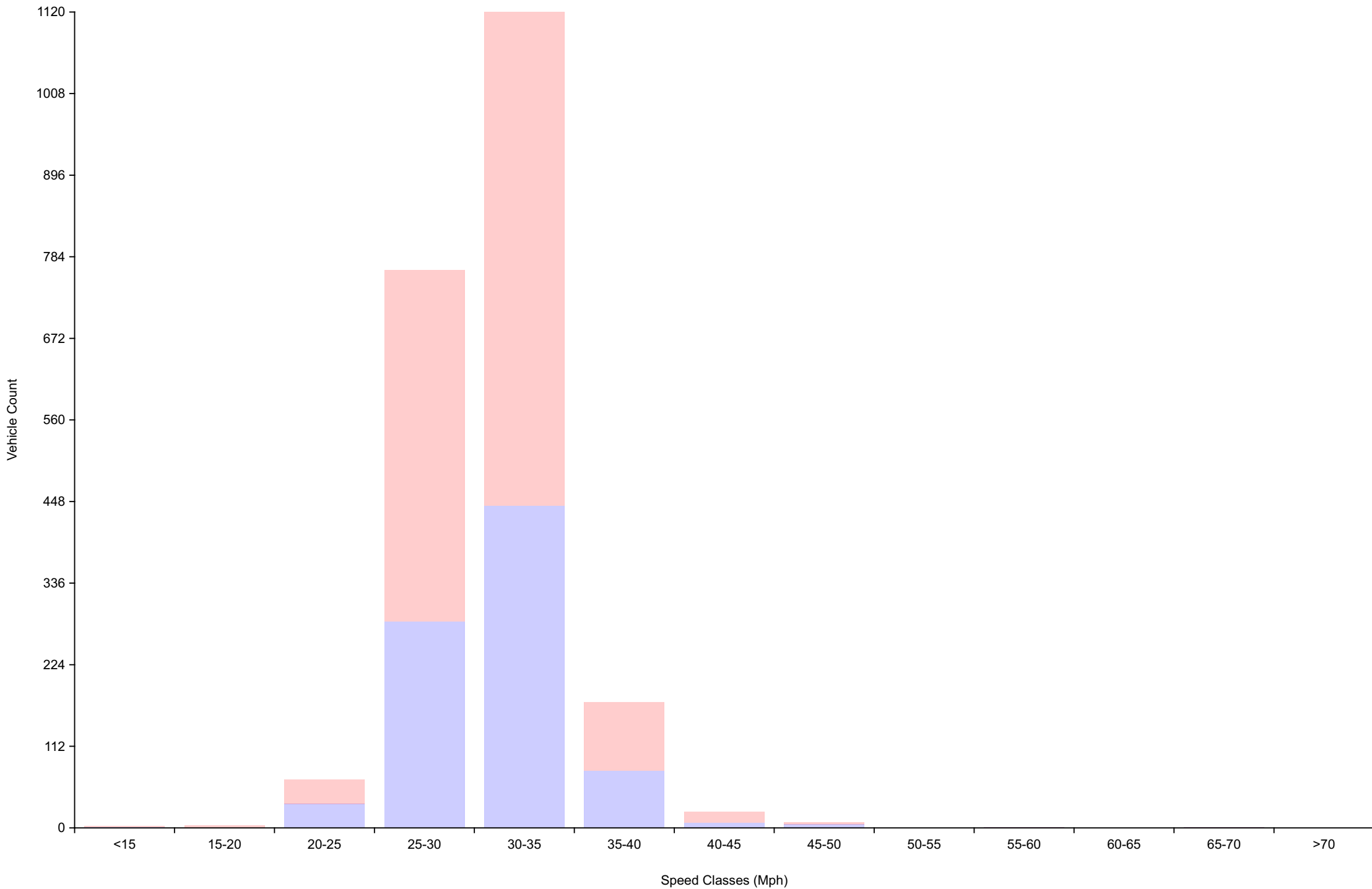
Vehicle Counts By Speed Class Daily Overview for Wed Jan 14 2026
