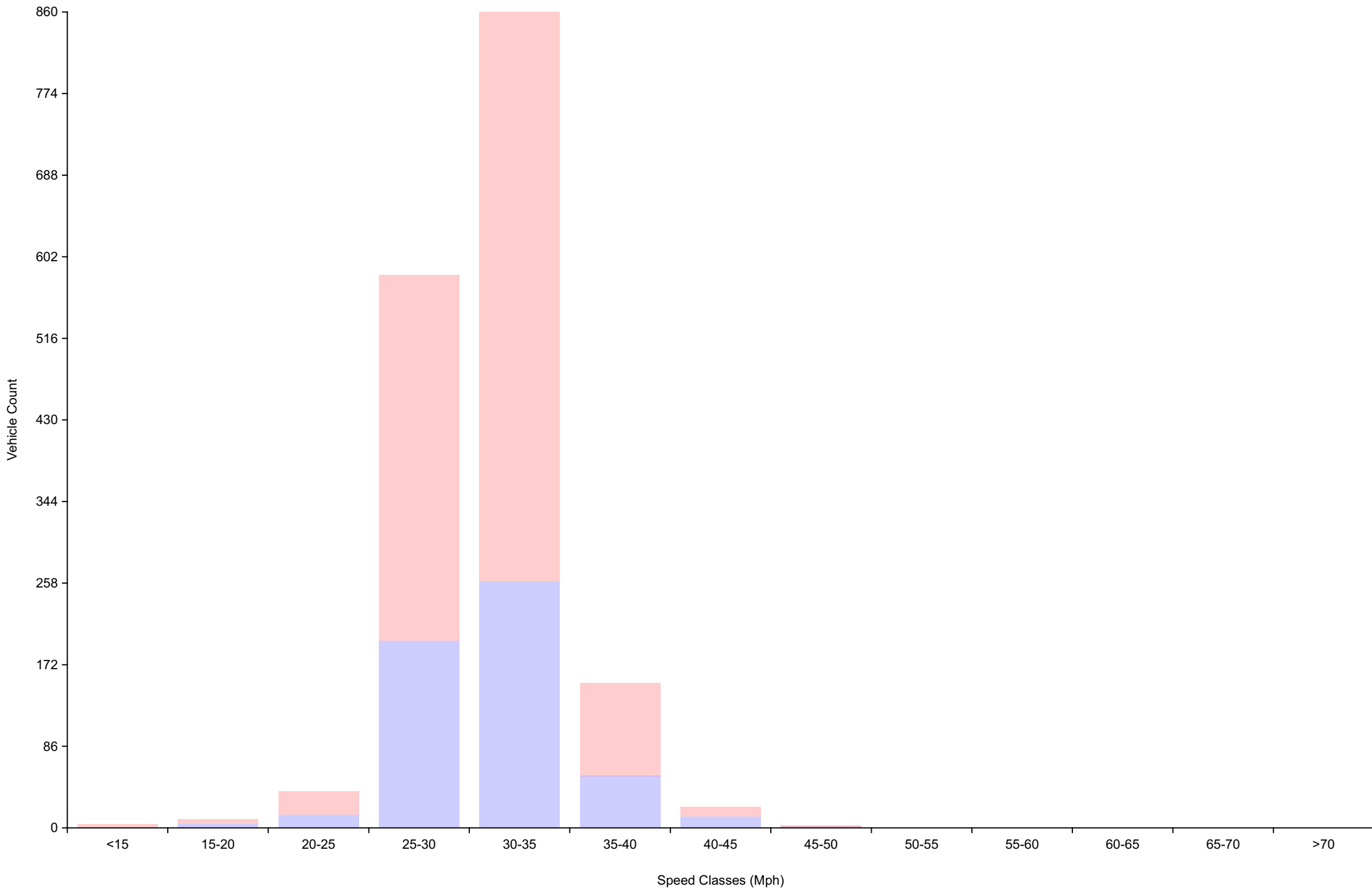
Vehicle Counts By Speed Class Daily Overview for Sat Jan 24 2026
