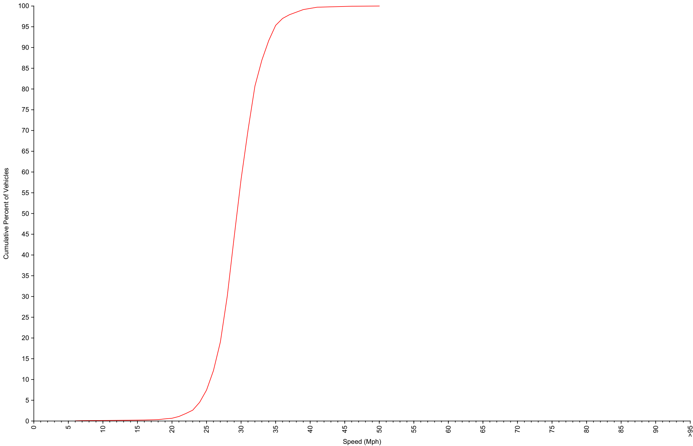
Cumulative Speed Distribution Curve Daily Overview for Mon Jan 26 2026
