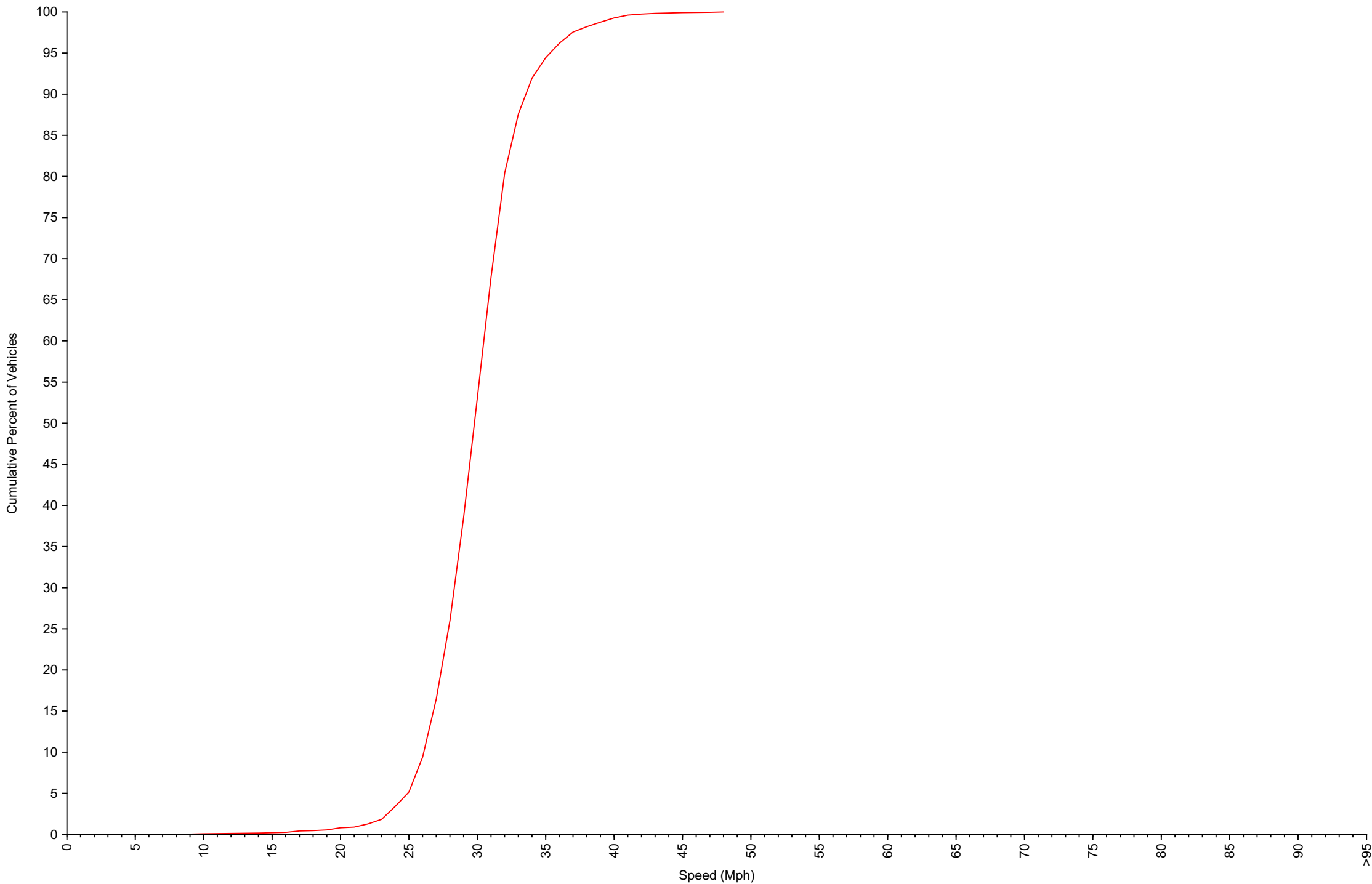
Cumulative Speed Distribution Curve Daily Overview for Tue Jan 20 2026
