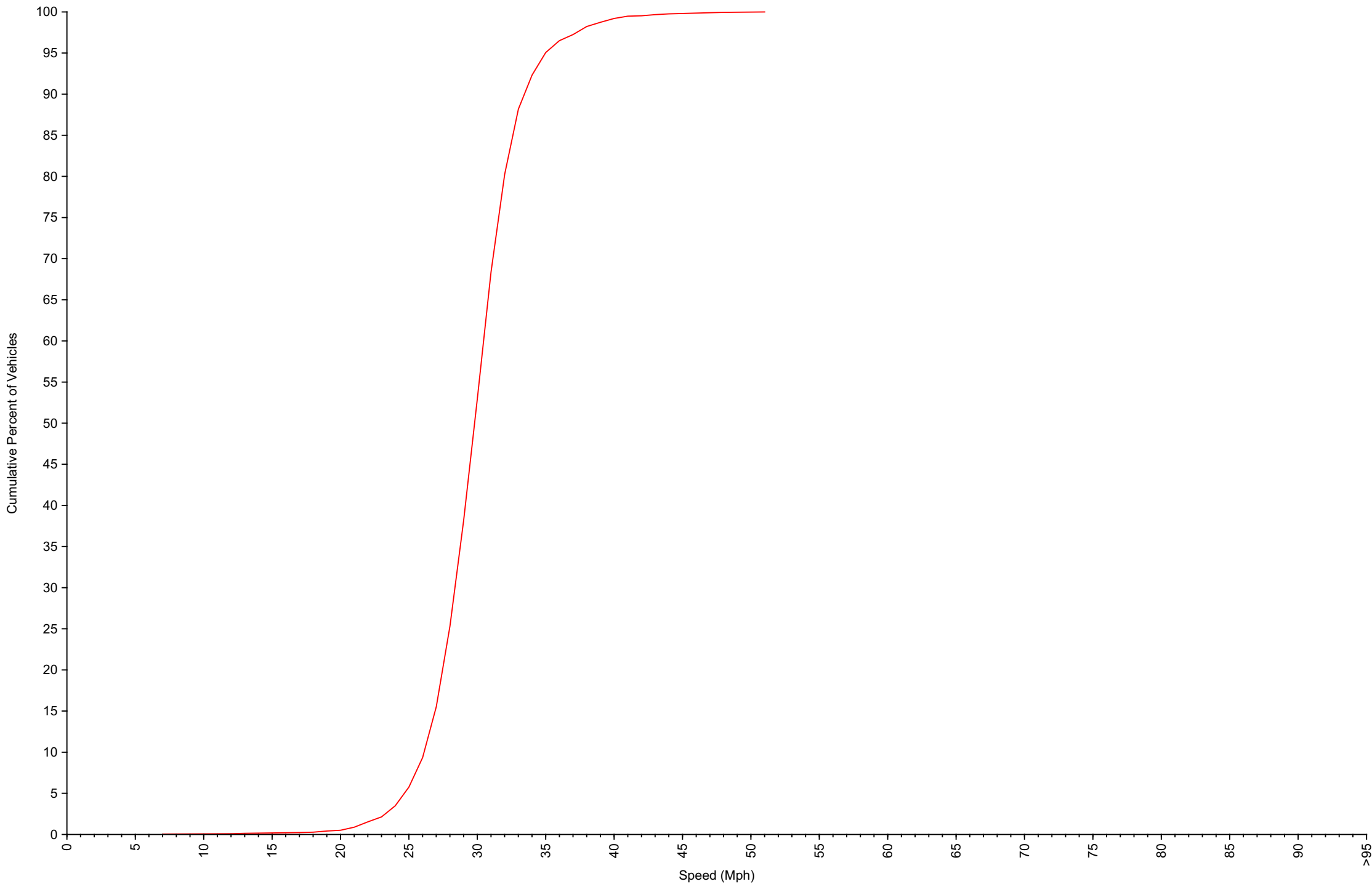
Cumulative Speed Distribution Curve Daily Overview for Mon Jan 12 2026
