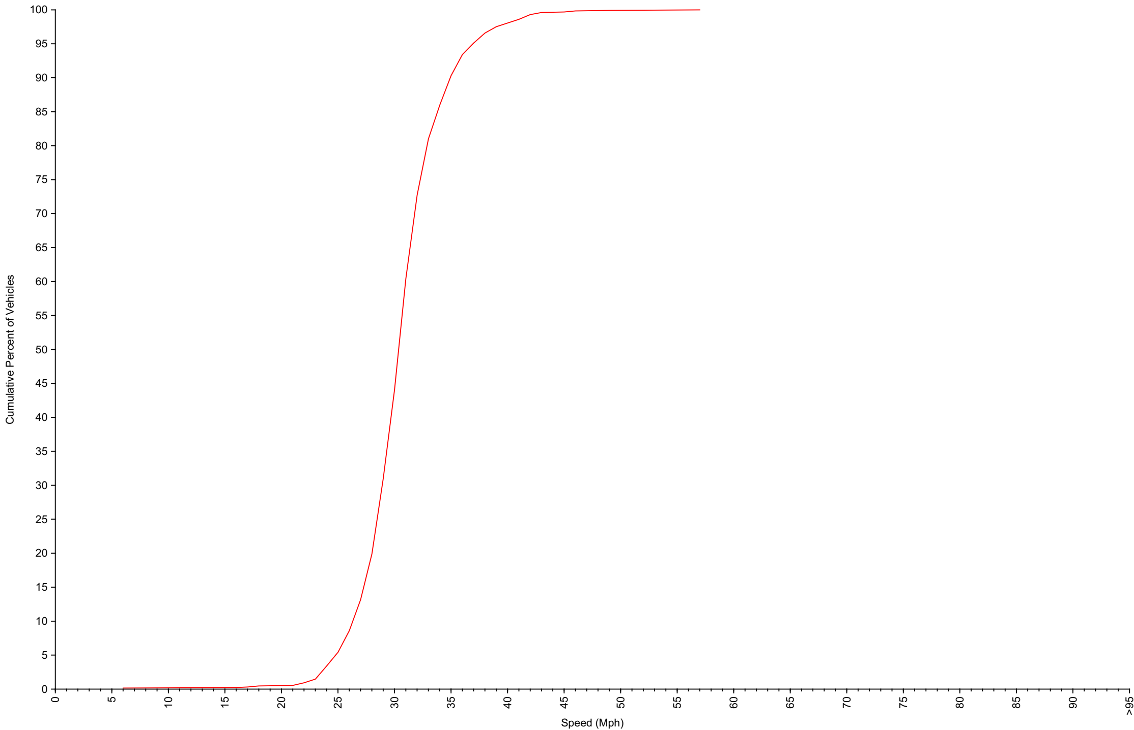
Cumulative Speed Distribution Curve Daily Overview for Sun Jan 4 2026
