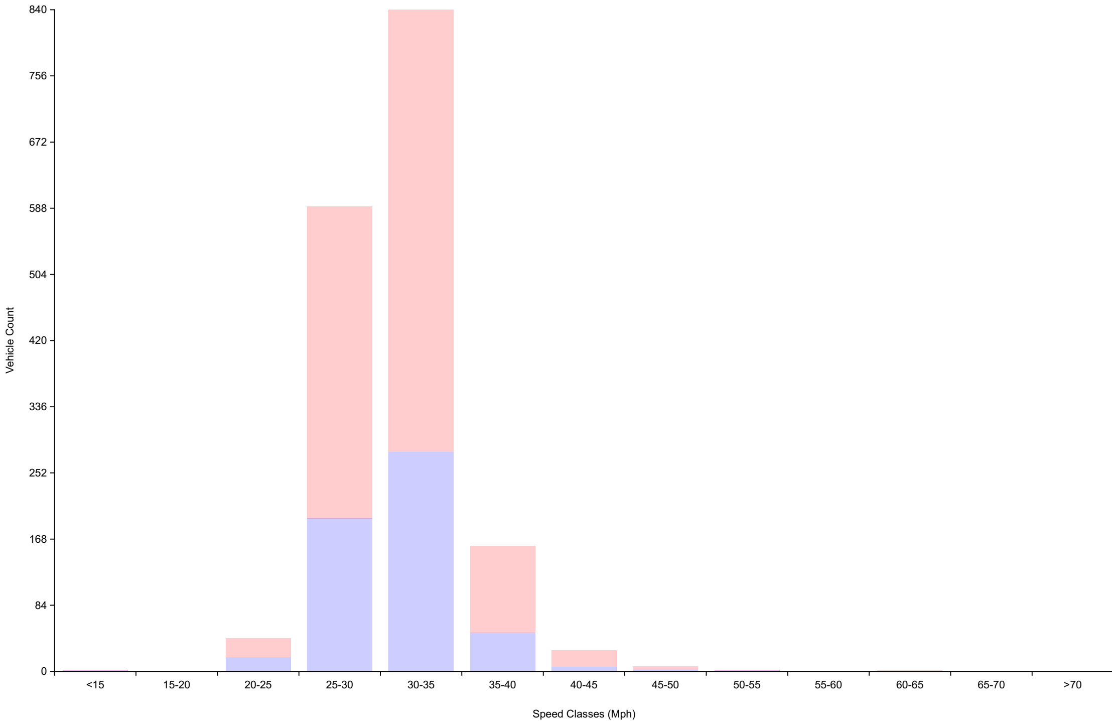
Vehicle Counts By Speed Class Daily Overview for Sat Jan 10 2026
