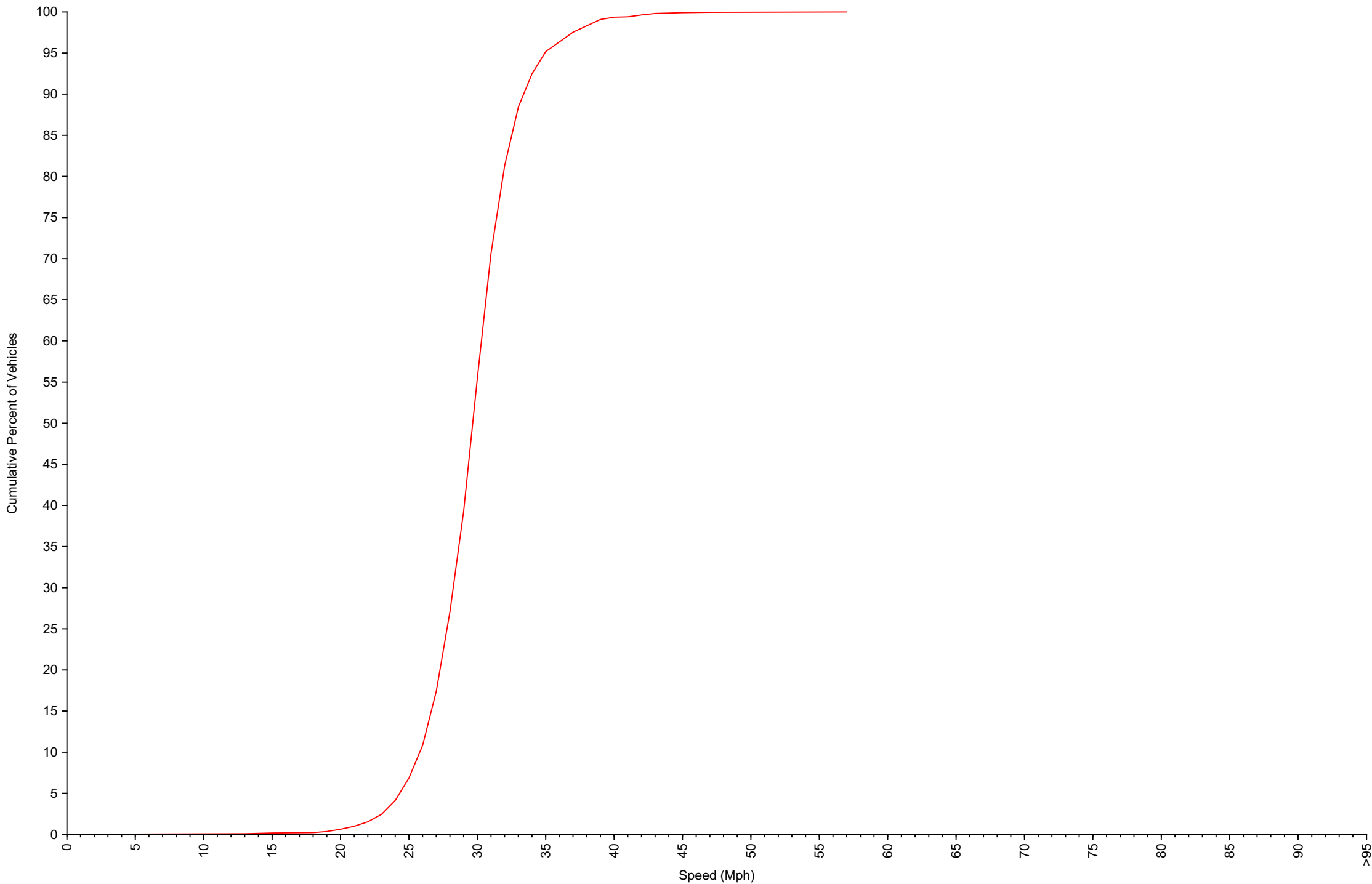
Cumulative Speed Distribution Curve Daily Overview for Thu Jan 15 2026
