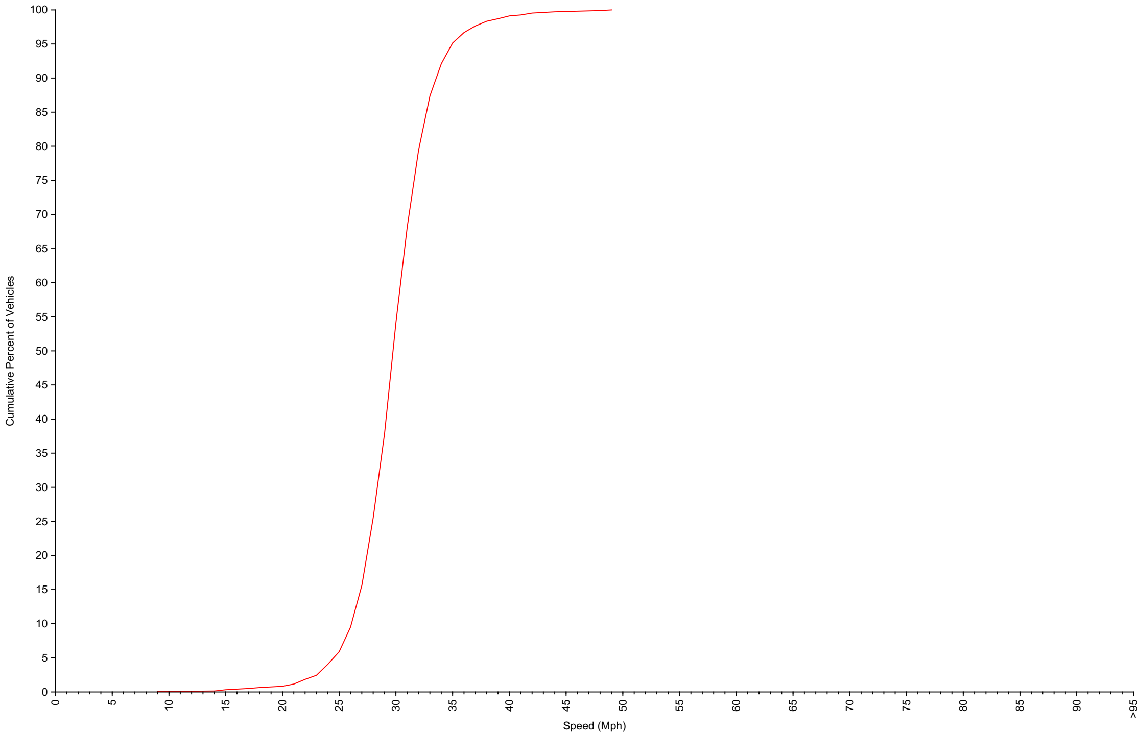
Cumulative Speed Distribution Curve Daily Overview for Mon Jan 19 2026
