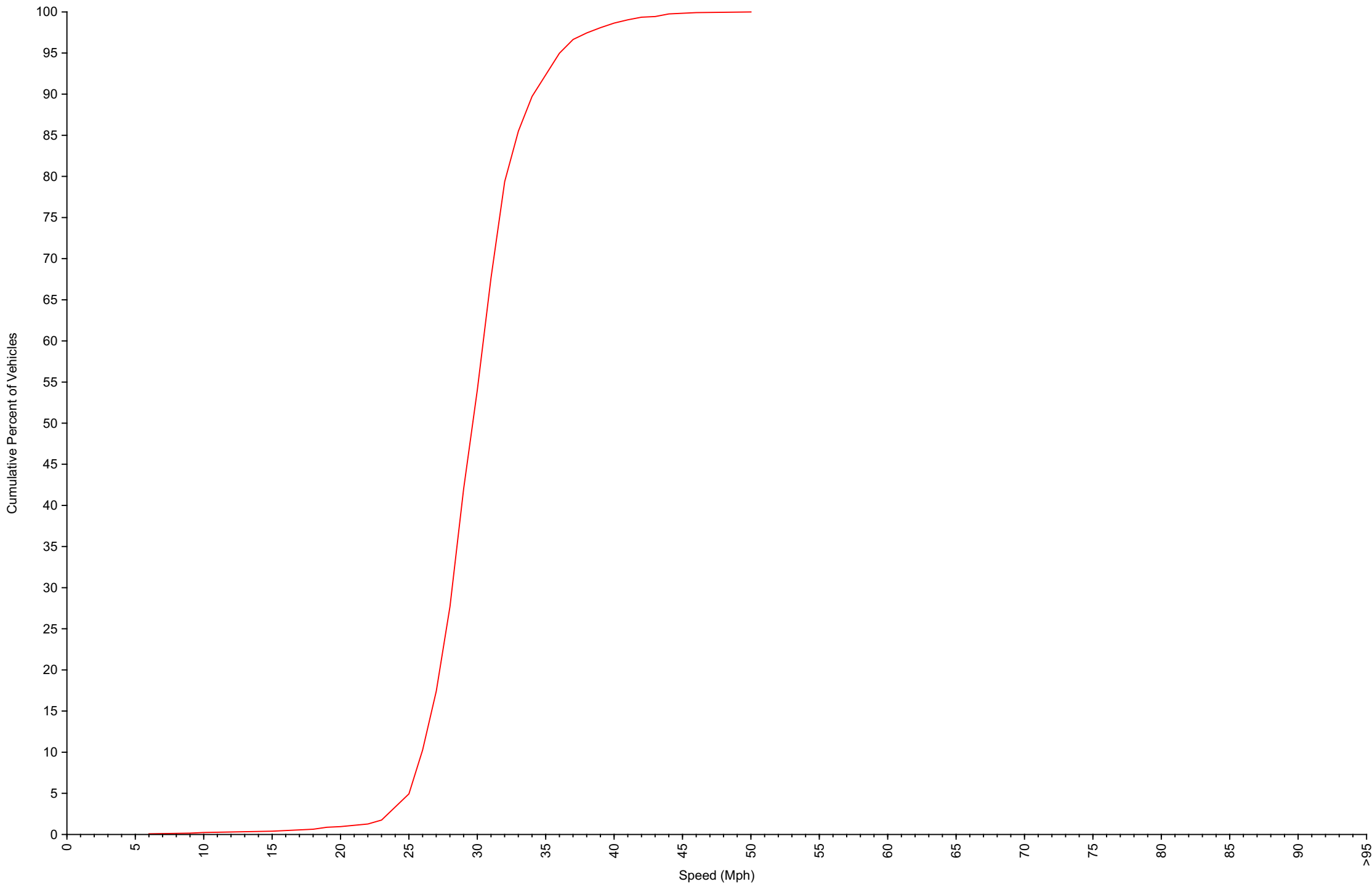
Cumulative Speed Distribution Curve Daily Overview for Sun Jan 25 2026
