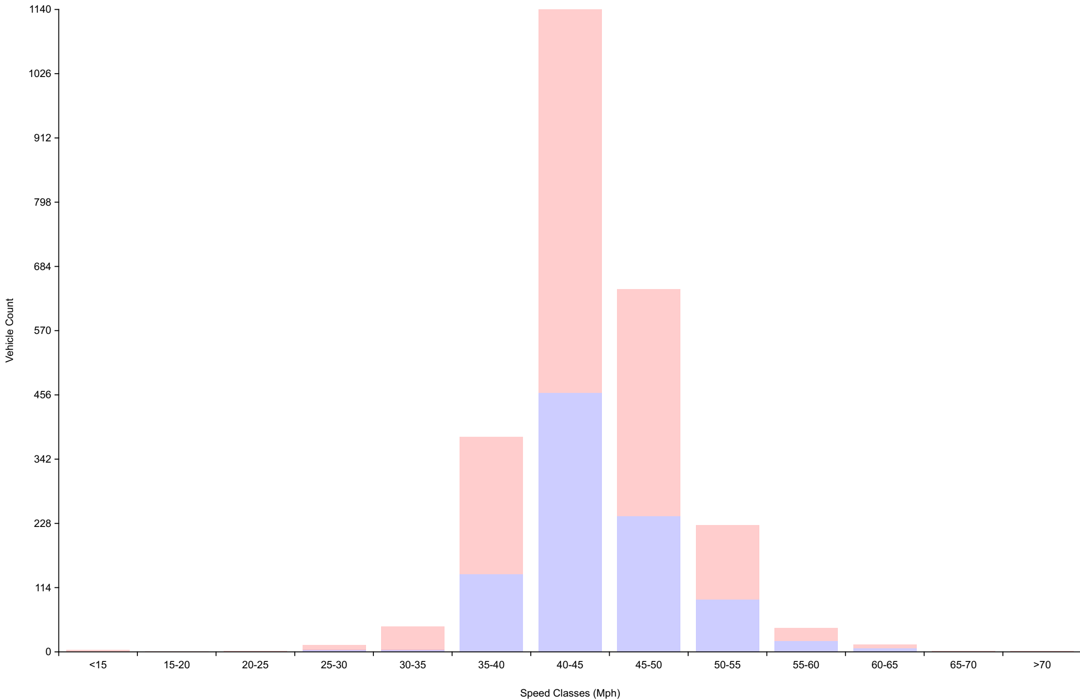
Vehicle Counts By Speed Class Daily Overview for Mon Aug 10 2026
