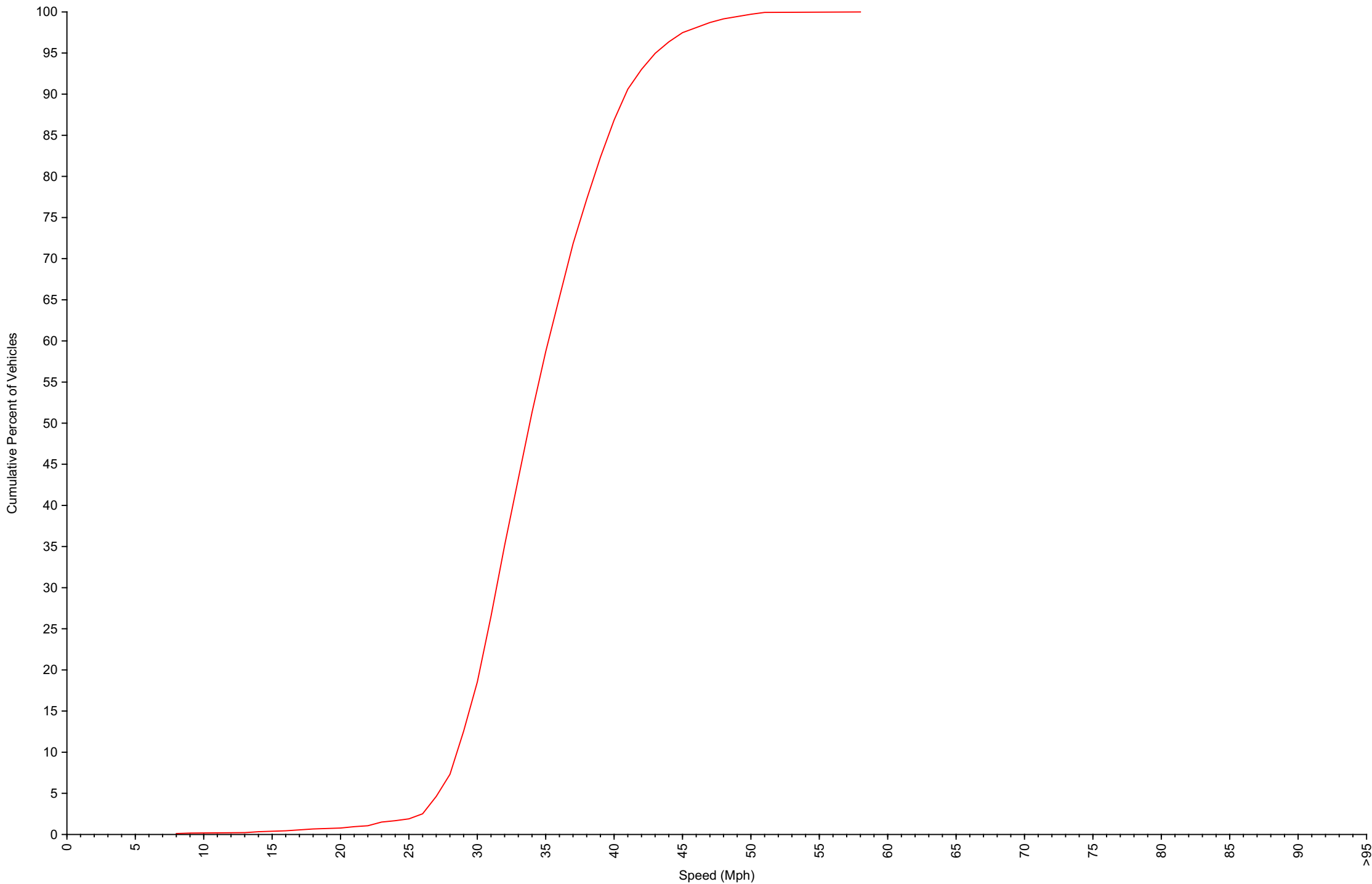
Cumulative Speed Distribution Curve Daily Overview for Mon Jun 29 2026
