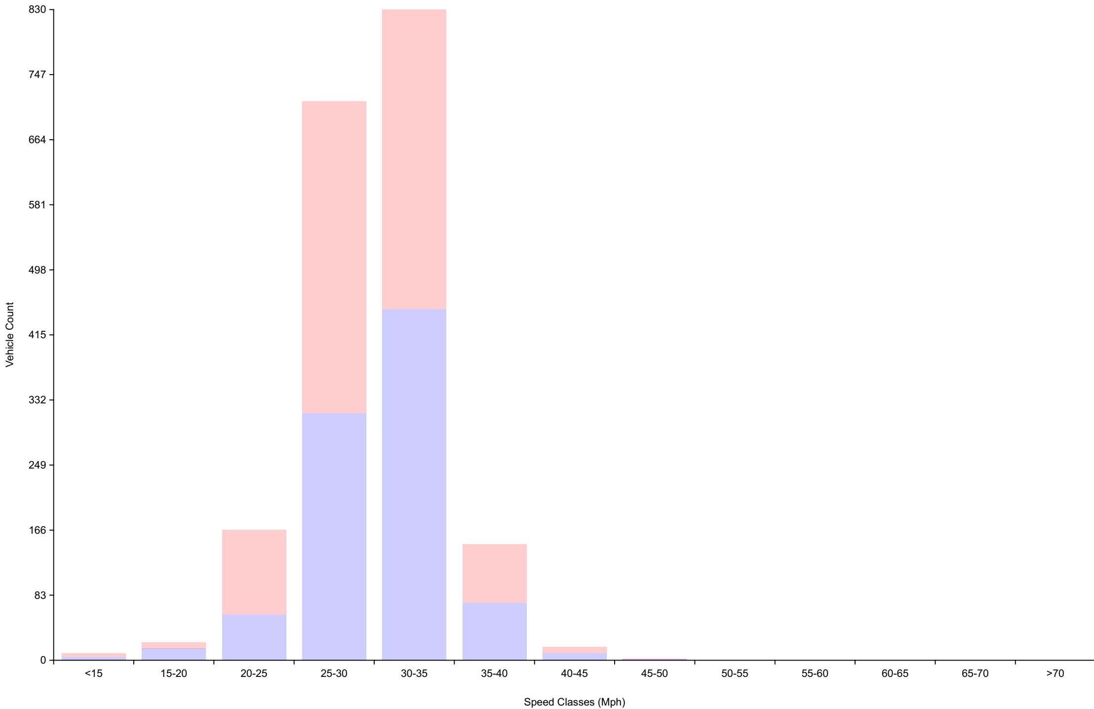
Vehicle Counts By Speed Class Daily Overview for Wed Jun 10 2026
