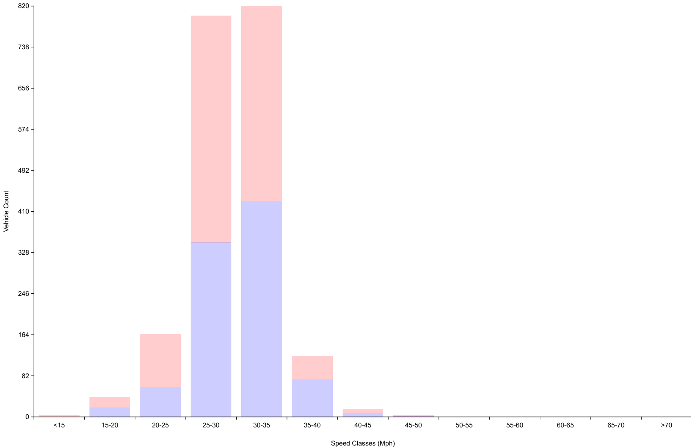
Vehicle Counts By Speed Class Daily Overview for Mon Jun 15 2026
