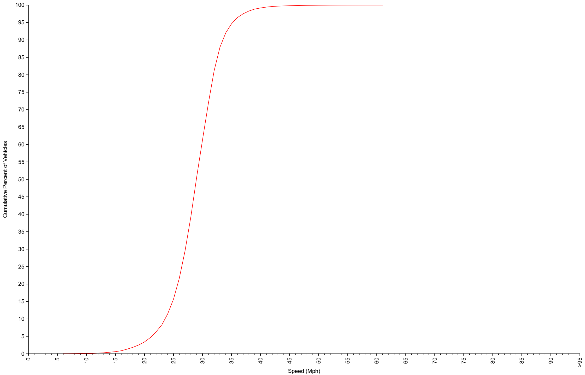
Cumulative Speed Distribution Curve Traffic Overview from Mon Jun 8 2026 to Tue Jun 30 2026
