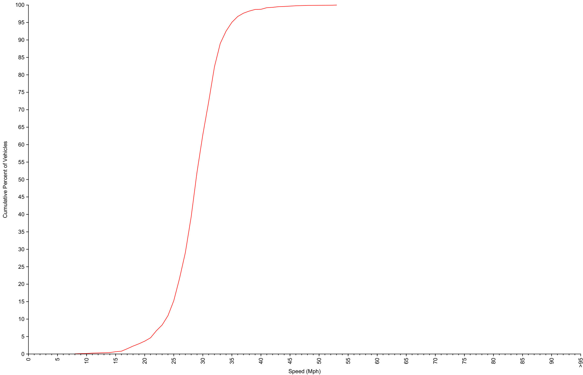
Cumulative Speed Distribution Curve Daily Overview for Tue Jun 16 2026
