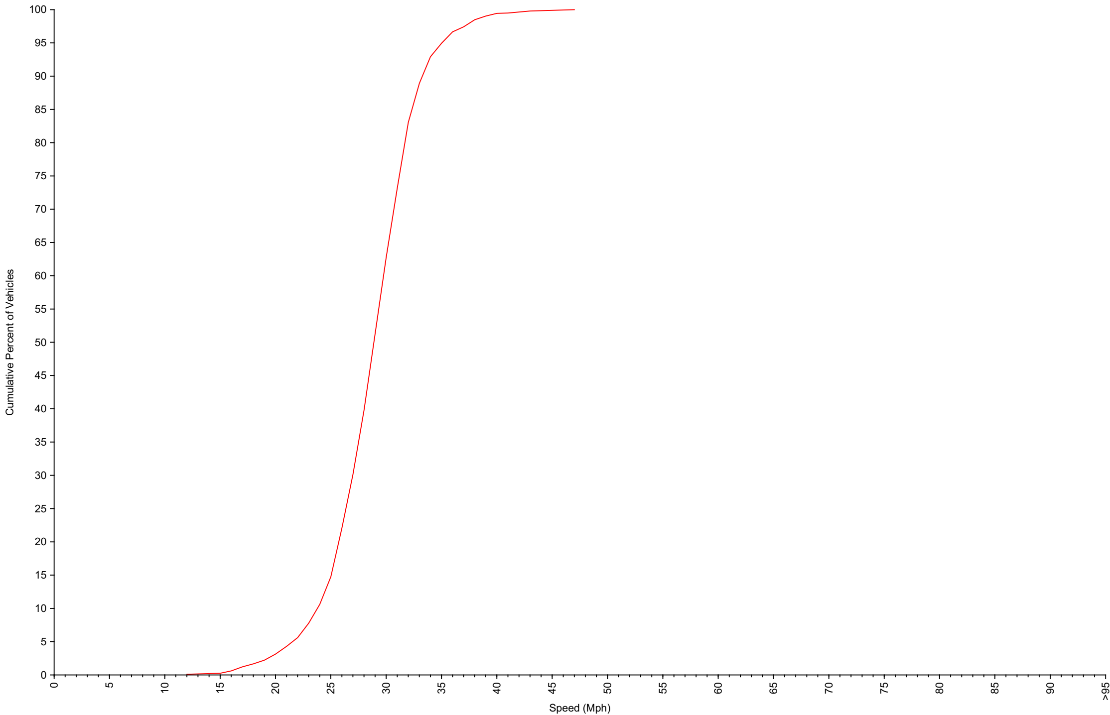
Cumulative Speed Distribution Curve Daily Overview for Mon Jun 15 2026
