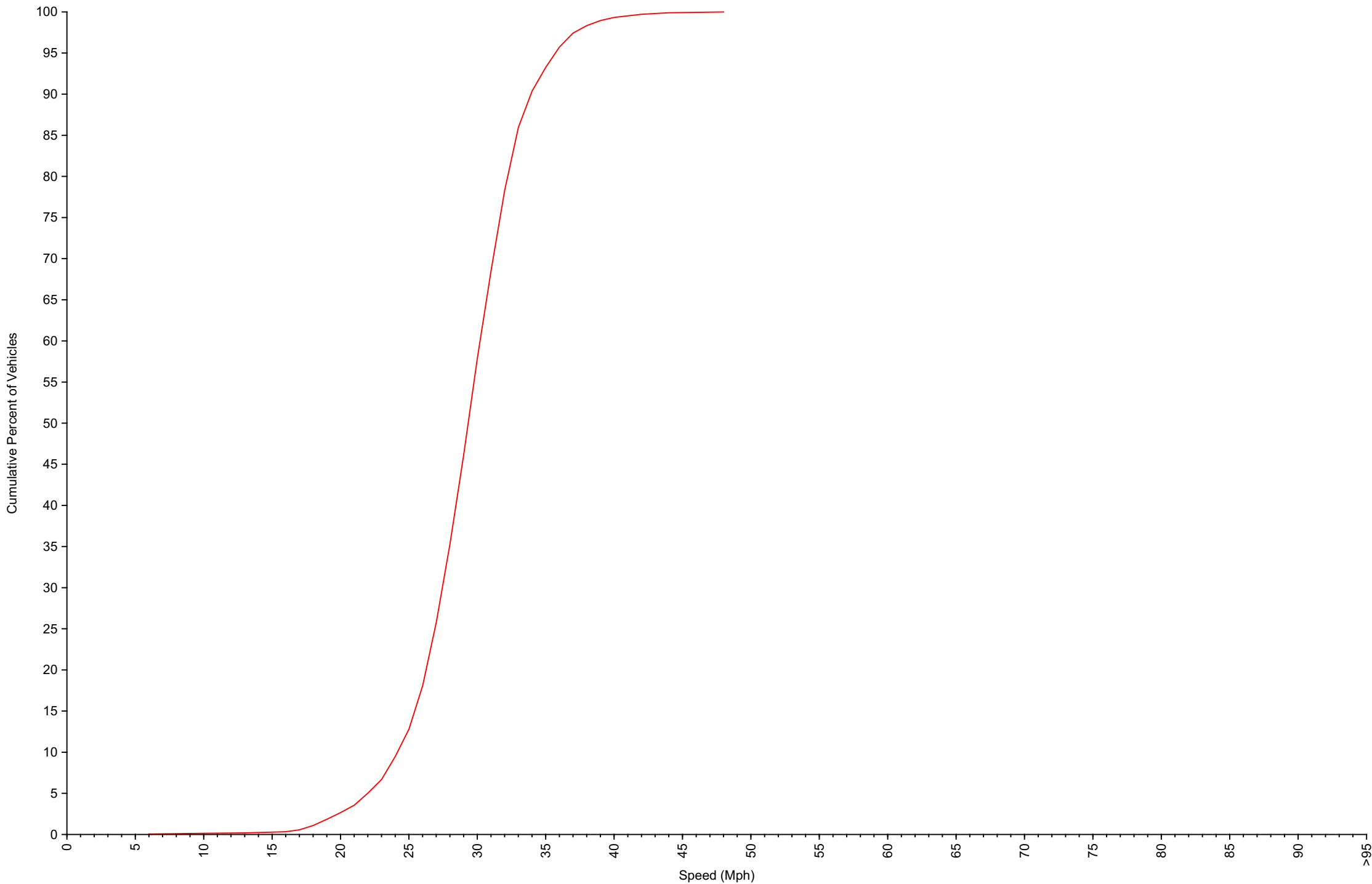
Cumulative Speed Distribution Curve Daily Overview for Thu Jun 25 2026
