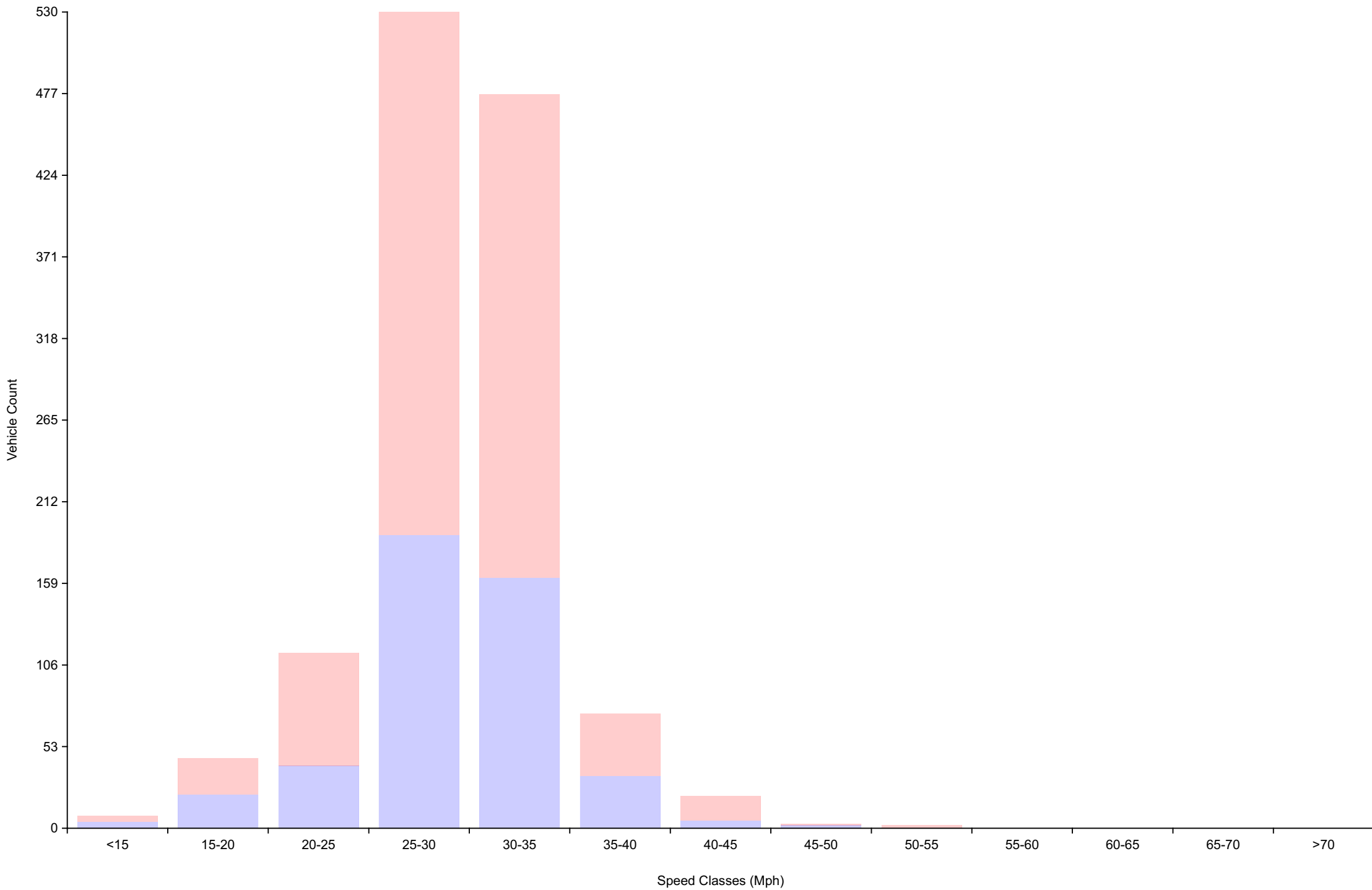
Vehicle Counts By Speed Class Daily Overview for Sun Jun 21 2026
