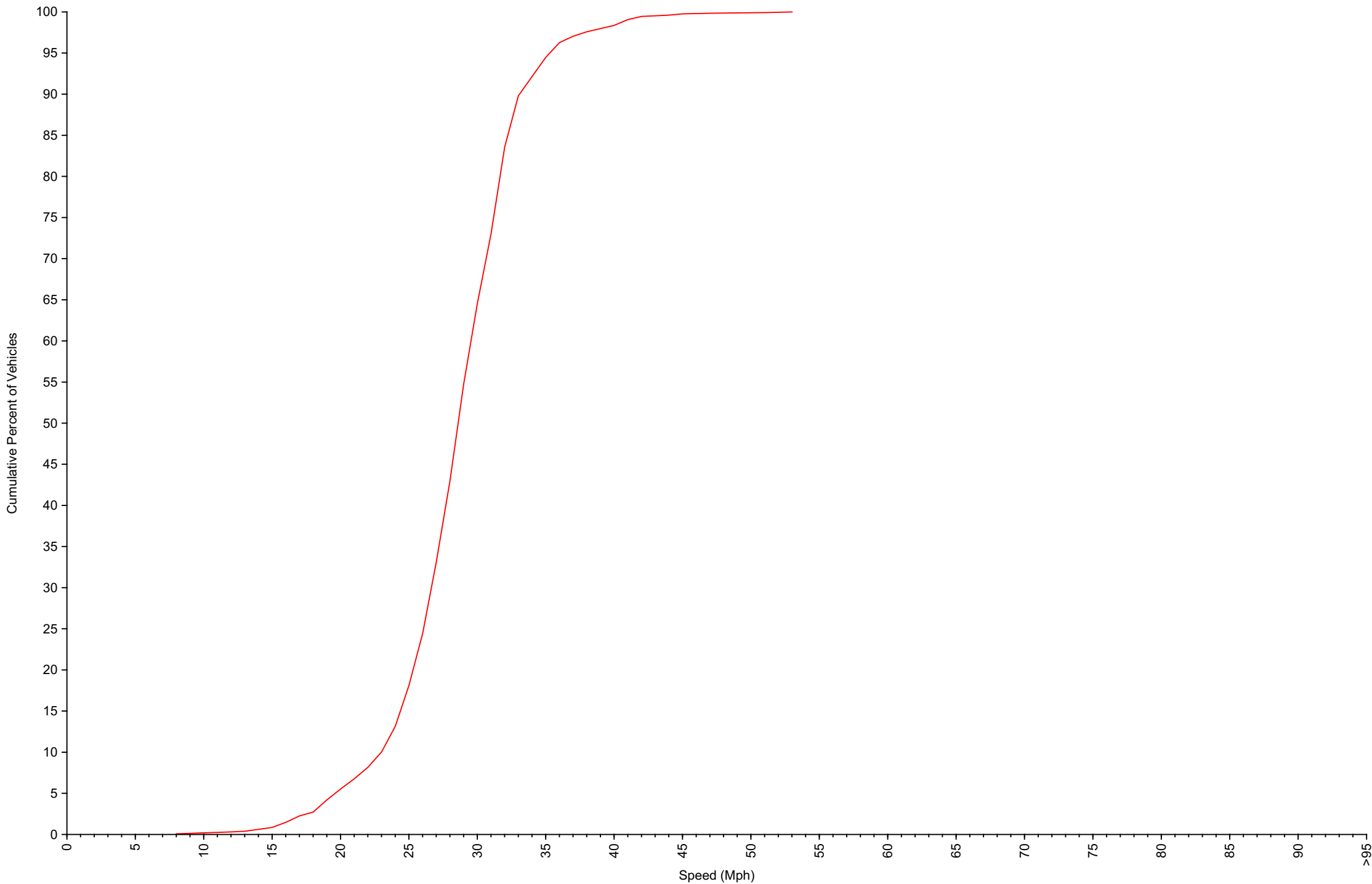
Cumulative Speed Distribution Curve Daily Overview for Sun Jun 21 2026
