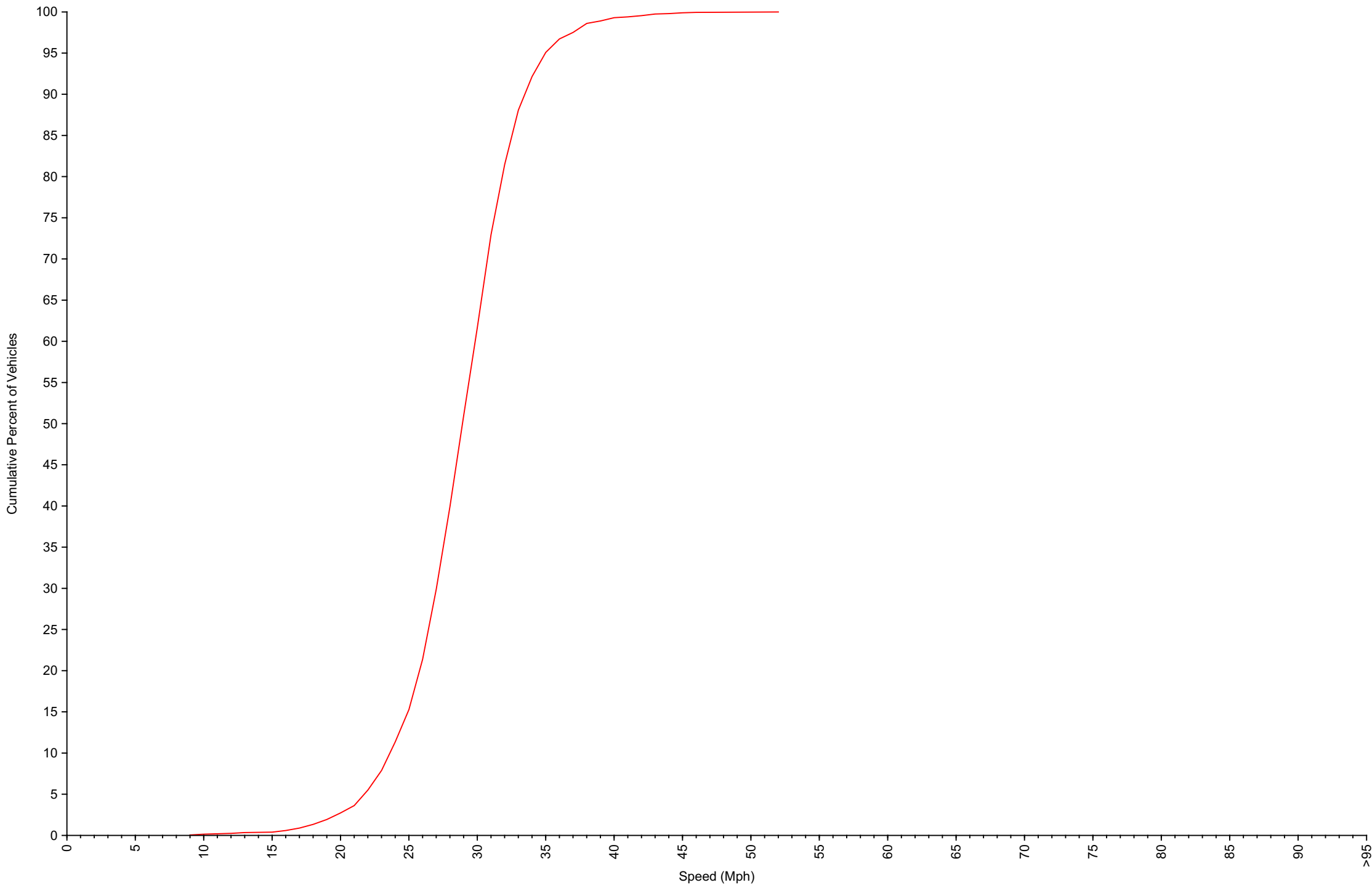
Cumulative Speed Distribution Curve Daily Overview for Thu Jun 11 2026
