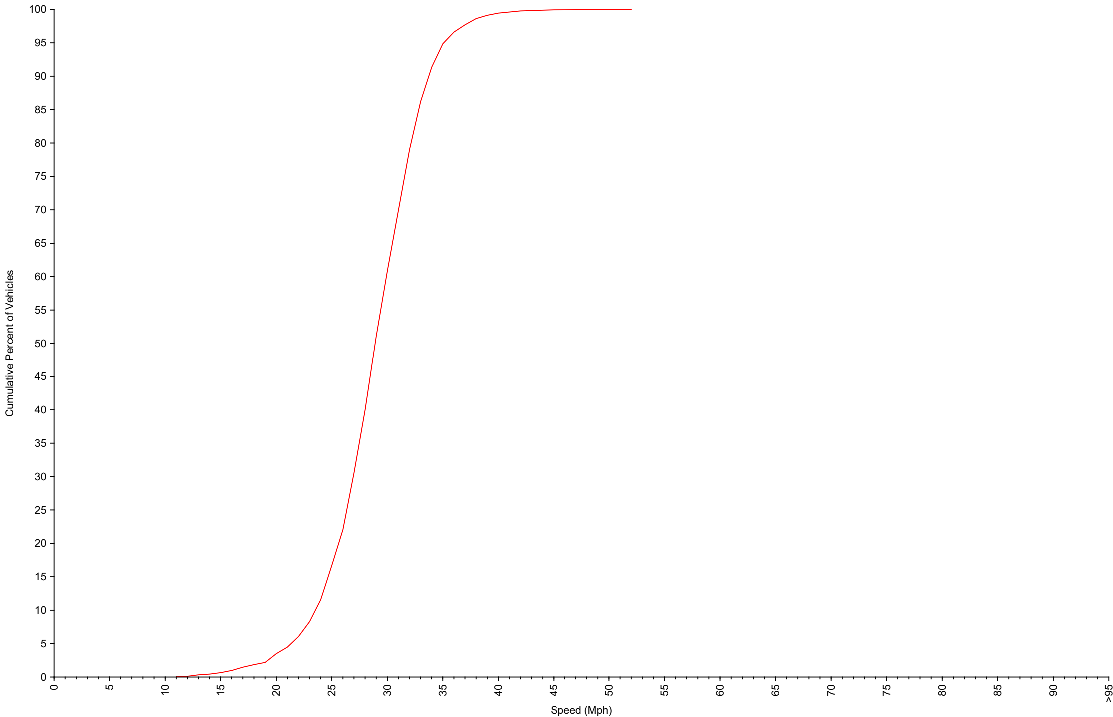
Cumulative Speed Distribution Curve Daily Overview for Fri Jun 12 2026
