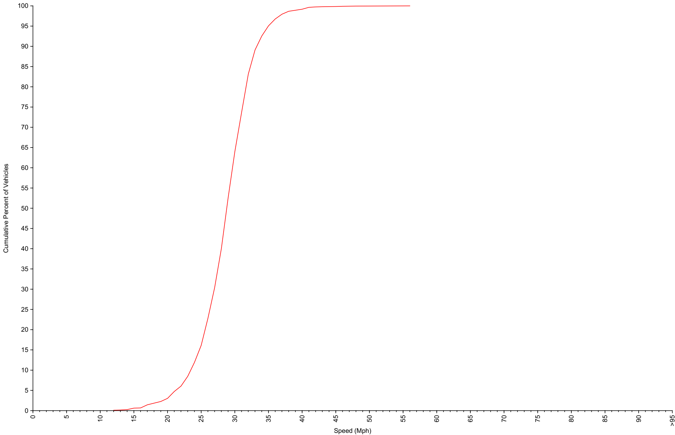
Cumulative Speed Distribution Curve Daily Overview for Mon Jun 22 2026
