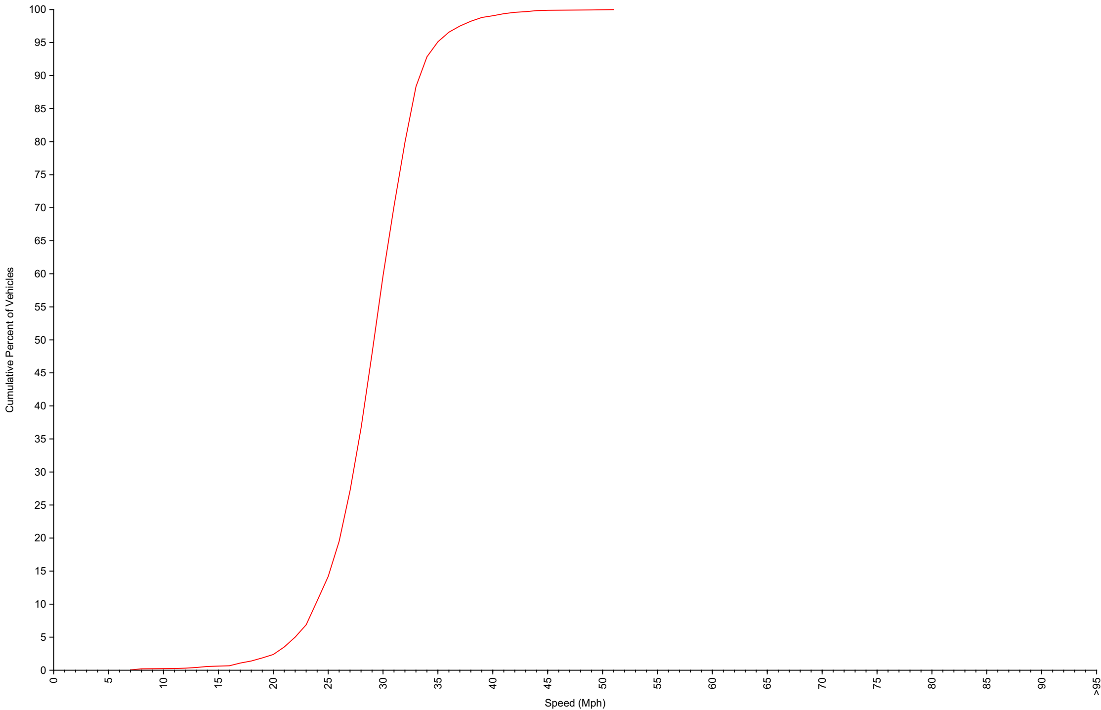
Cumulative Speed Distribution Curve Daily Overview for Mon Jun 8 2026
