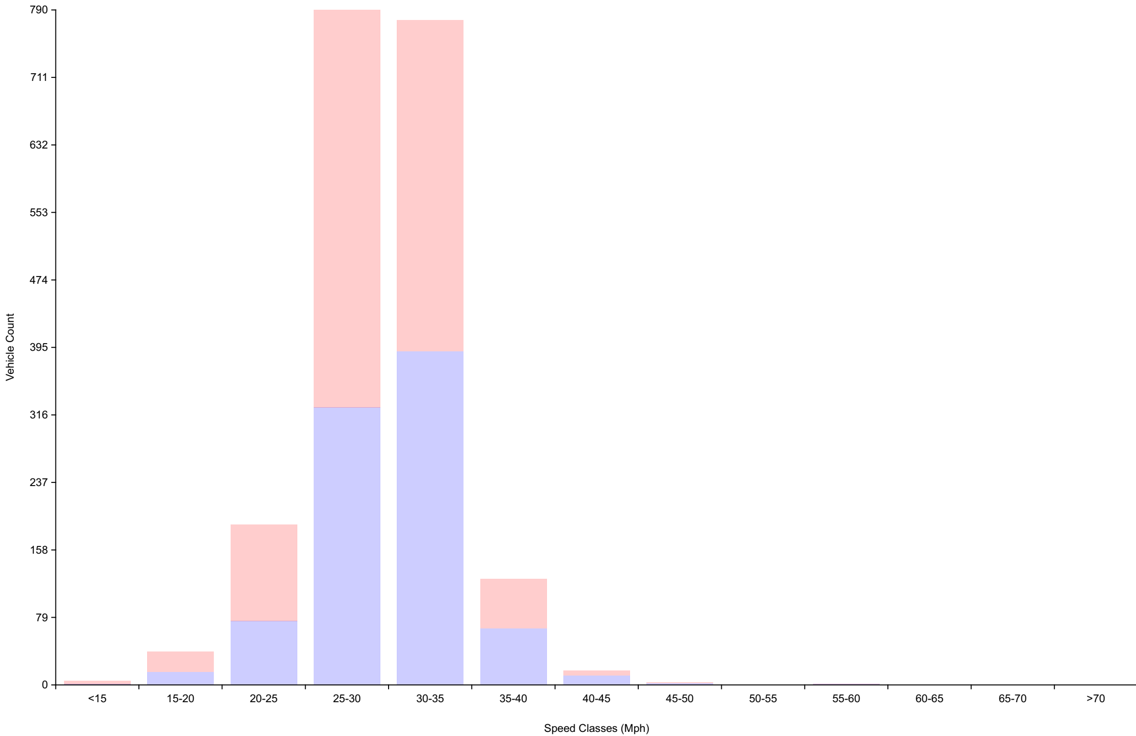
Vehicle Counts By Speed Class Daily Overview for Mon Jun 22 2026
