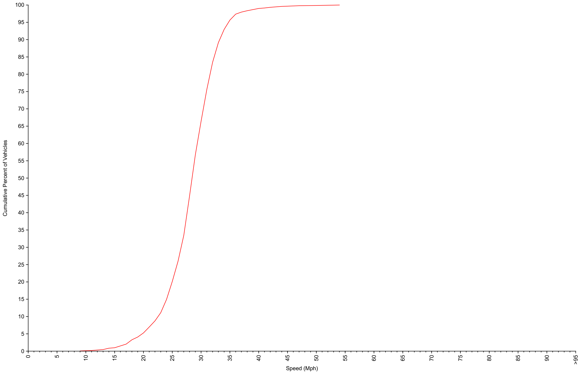
Cumulative Speed Distribution Curve Daily Overview for Sat Jun 20 2026
