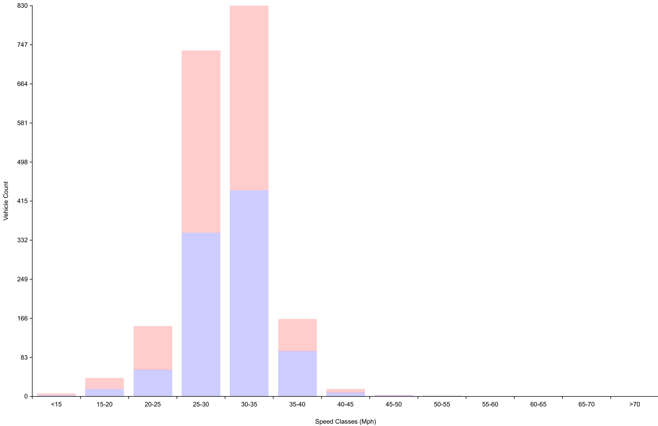
Vehicle Counts By Speed Class Daily Overview for Wed Jun 24 2026
