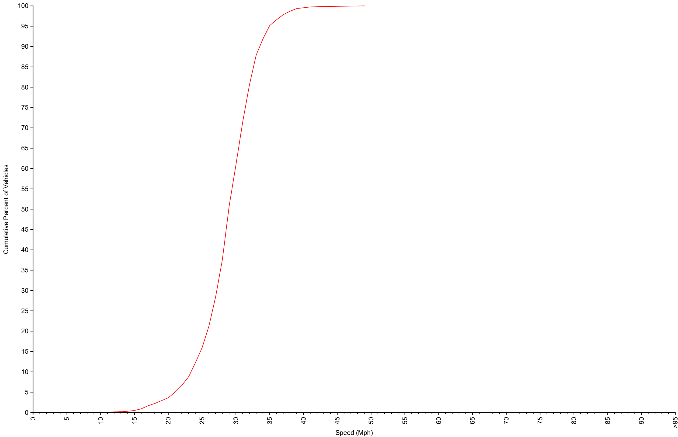
Cumulative Speed Distribution Curve Daily Overview for Tue Jun 23 2026
