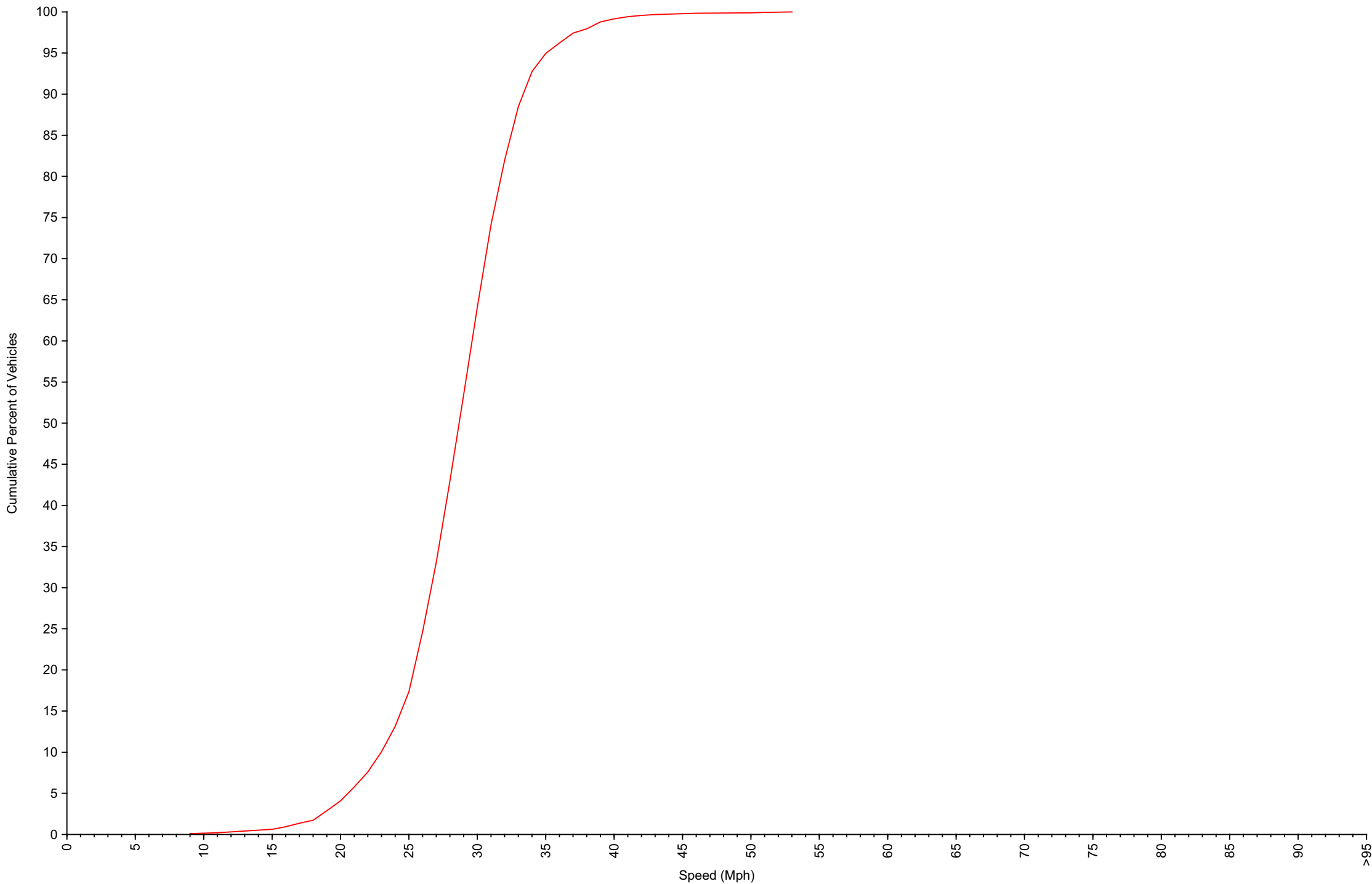
Cumulative Speed Distribution Curve Daily Overview for Thu Jun 18 2026
