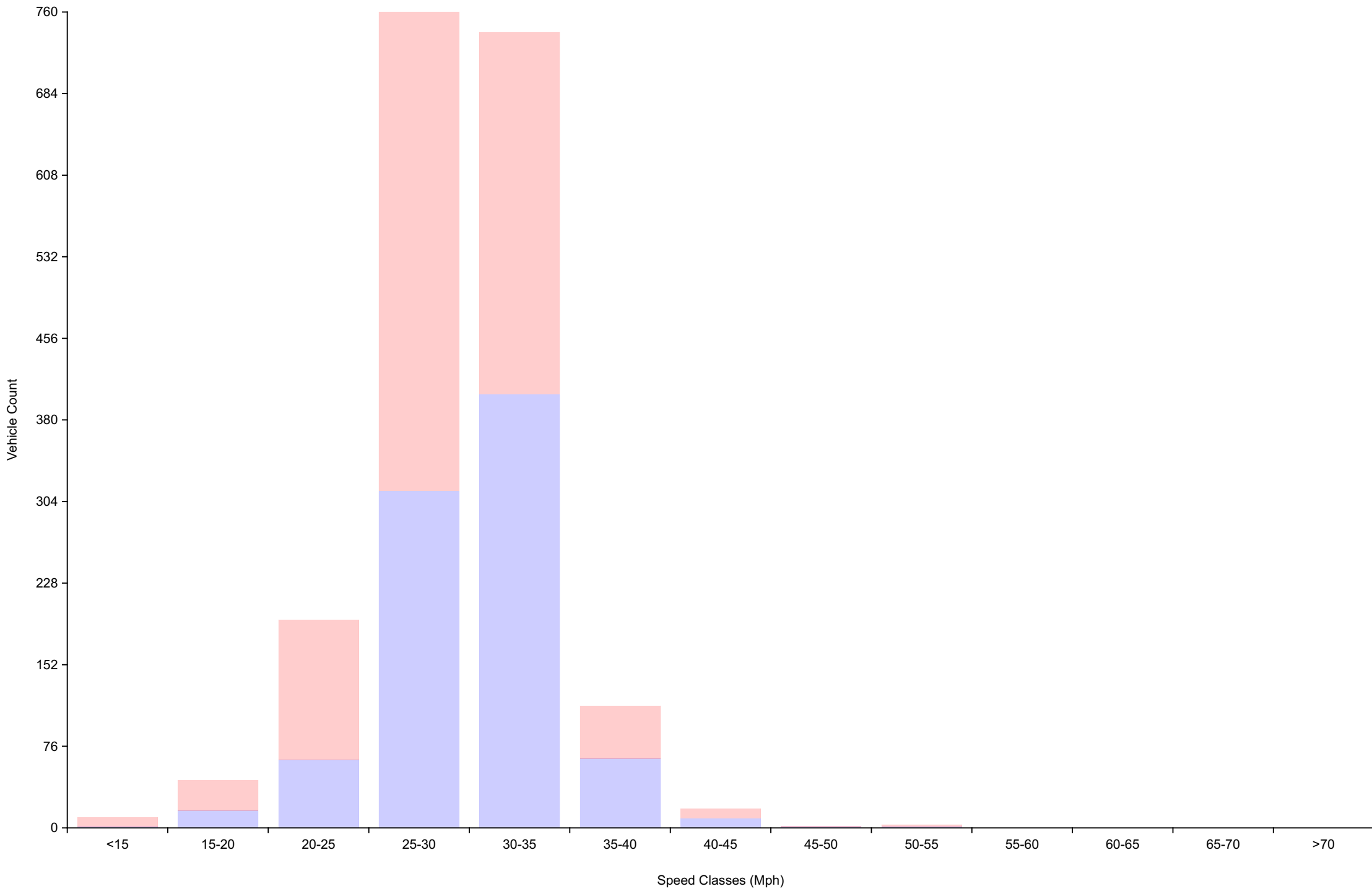
Vehicle Counts By Speed Class Daily Overview for Thu Jun 18 2026
