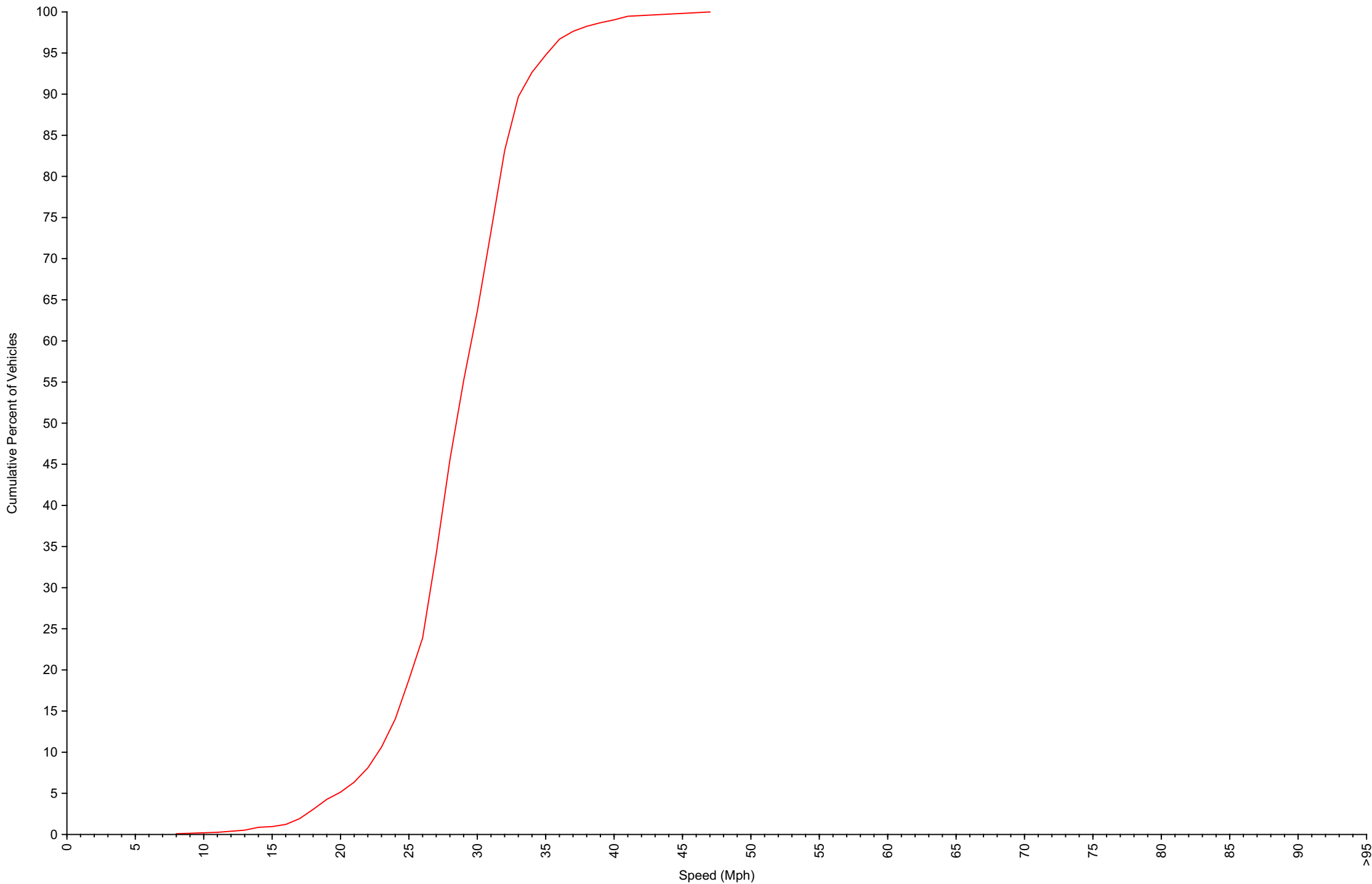
Cumulative Speed Distribution Curve Daily Overview for Sun Jun 14 2026
