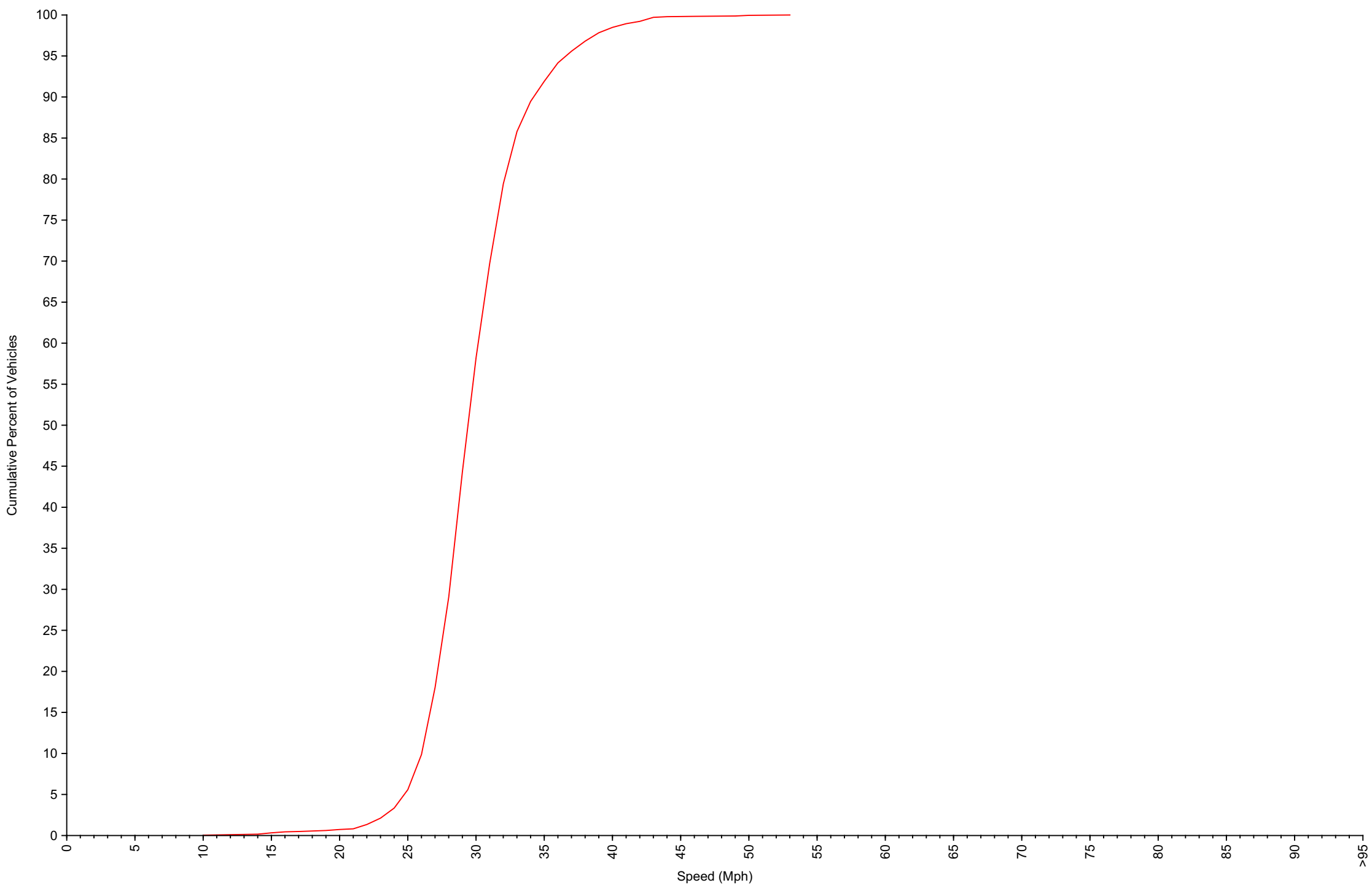
Cumulative Speed Distribution Curve Daily Overview for Tue Aug 26 2025
