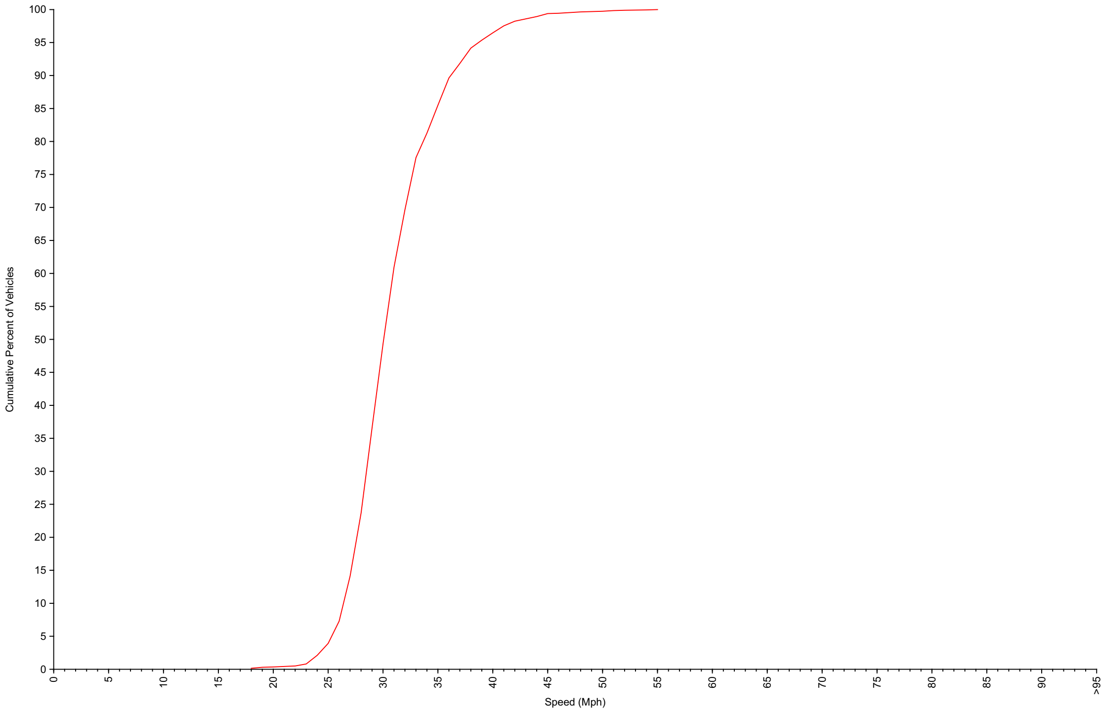
Cumulative Speed Distribution Curve Daily Overview for Sat Aug 16 2025
