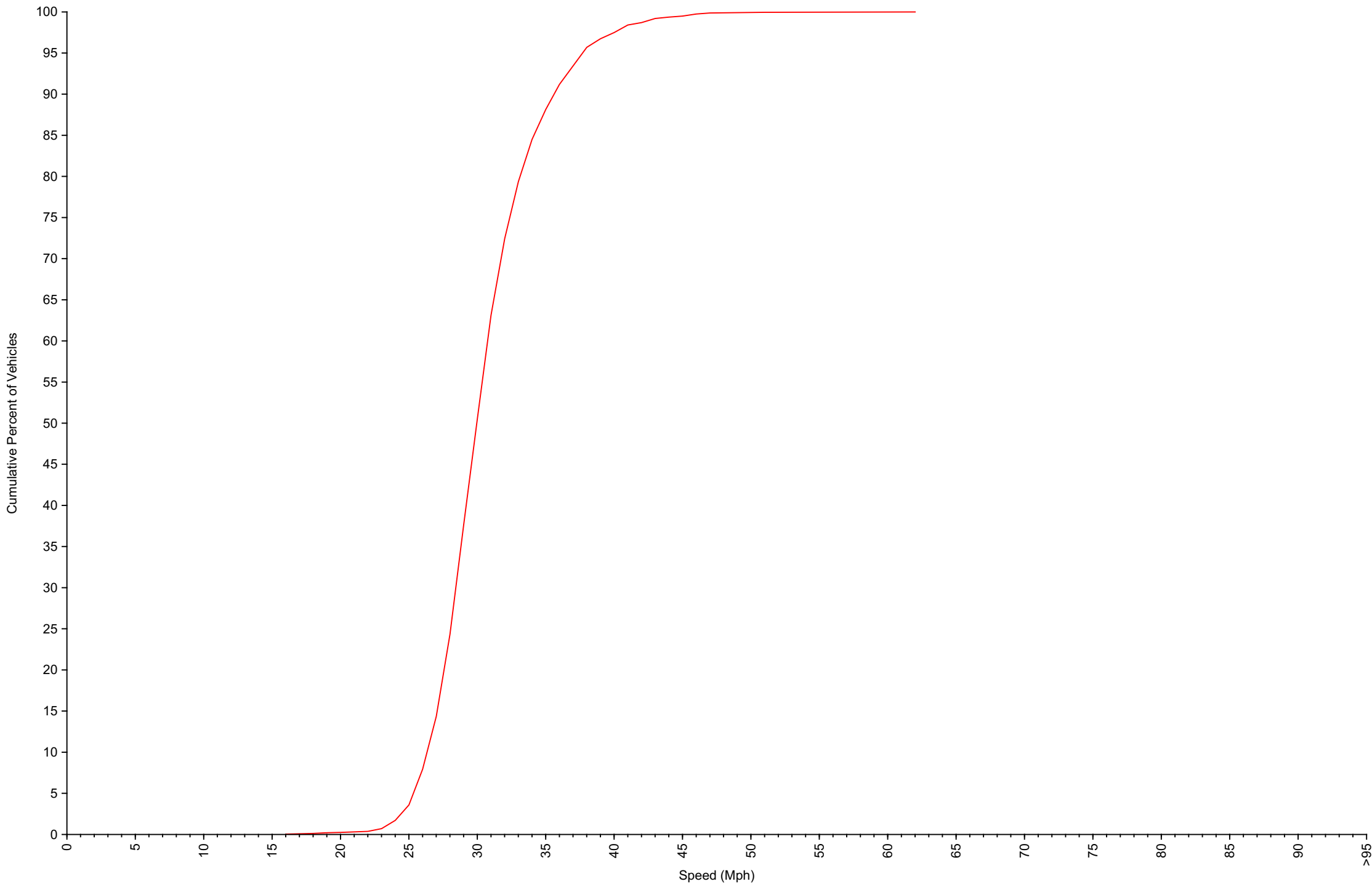
Cumulative Speed Distribution Curve Daily Overview for Fri Aug 15 2025
