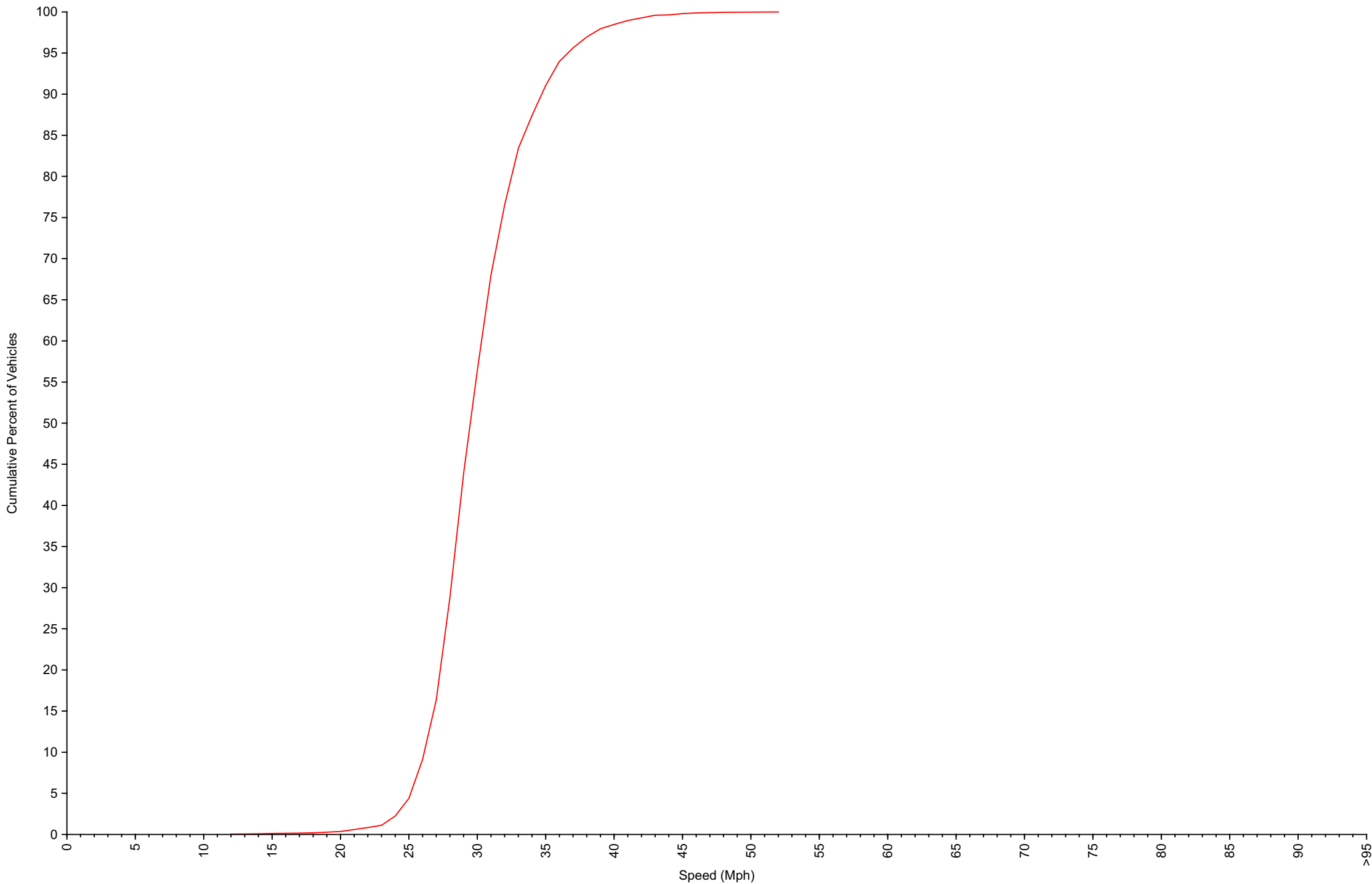
Cumulative Speed Distribution Curve Daily Overview for Thu Aug 28 2025
