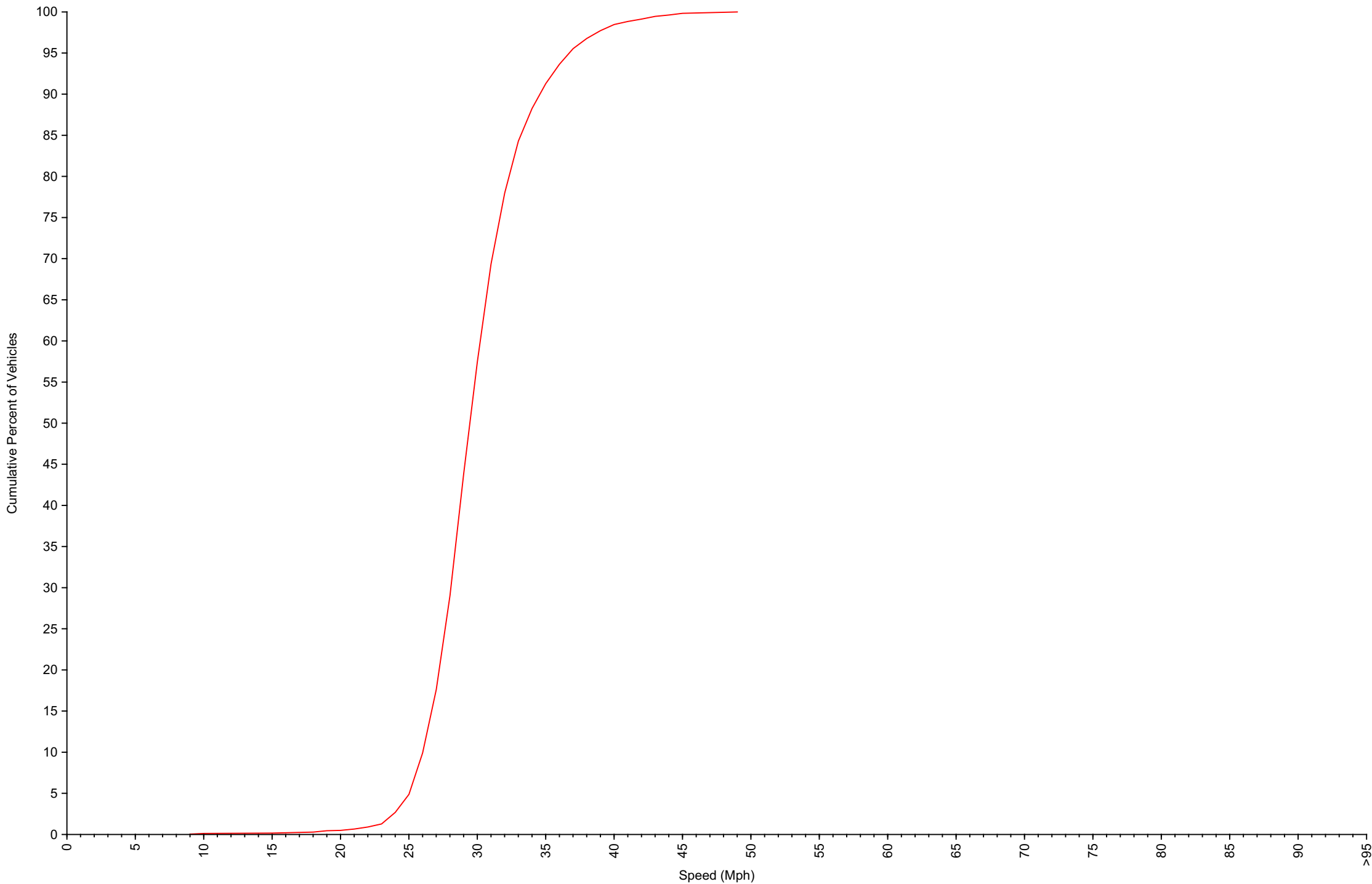
Cumulative Speed Distribution Curve Daily Overview for Wed Aug 27 2025
