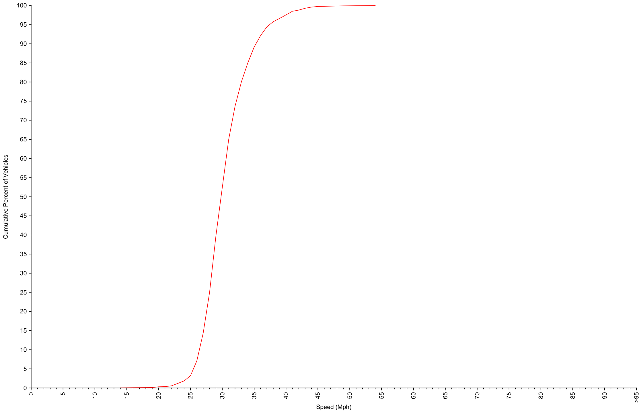
Cumulative Speed Distribution Curve Daily Overview for Thu Aug 21 2025
