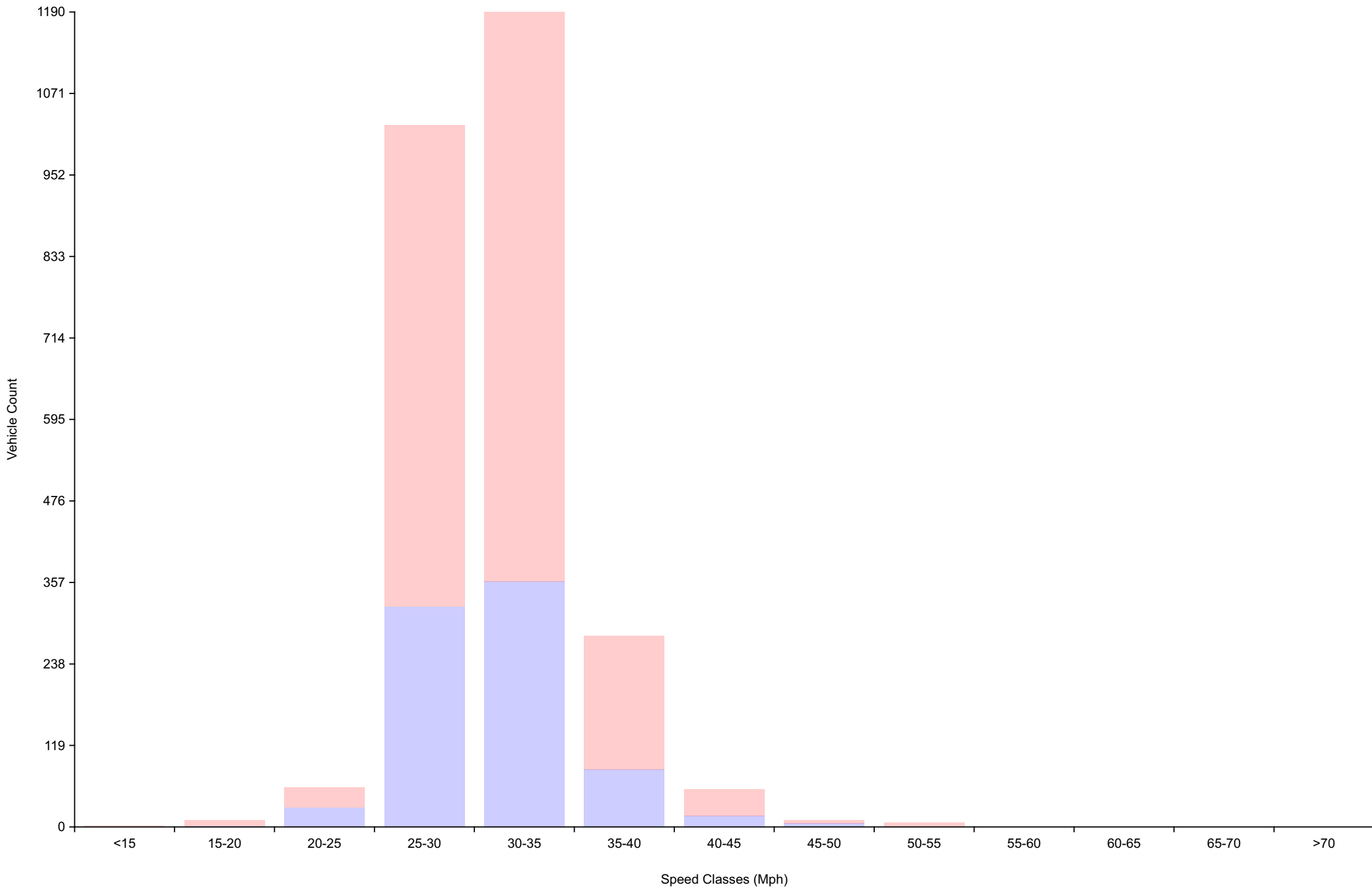
Vehicle Counts By Speed Class Daily Overview for Wed Aug 20 2025
