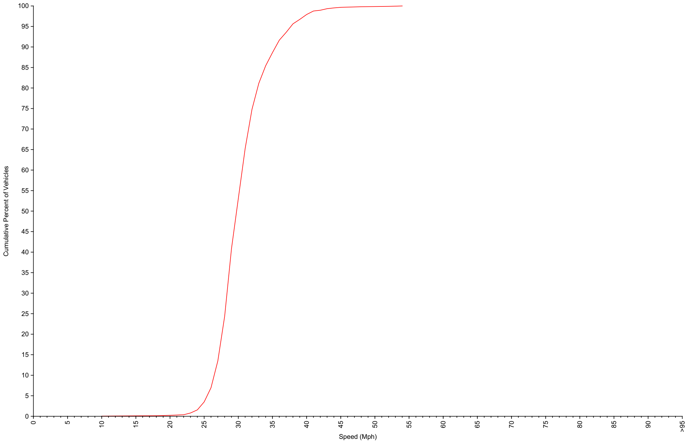
Cumulative Speed Distribution Curve Daily Overview for Mon Aug 4 2025
