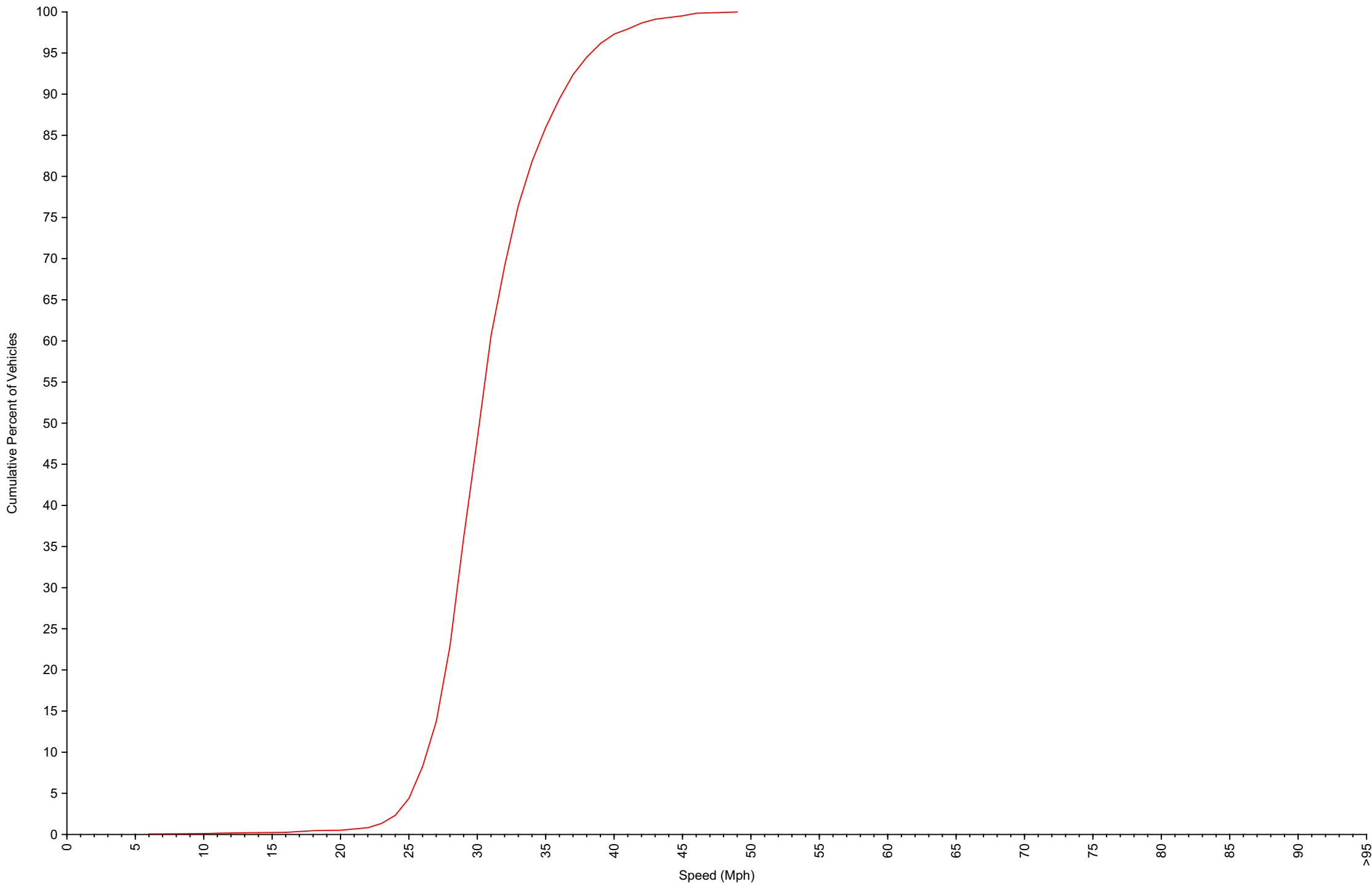
Cumulative Speed Distribution Curve Daily Overview for Mon Aug 25 2025
