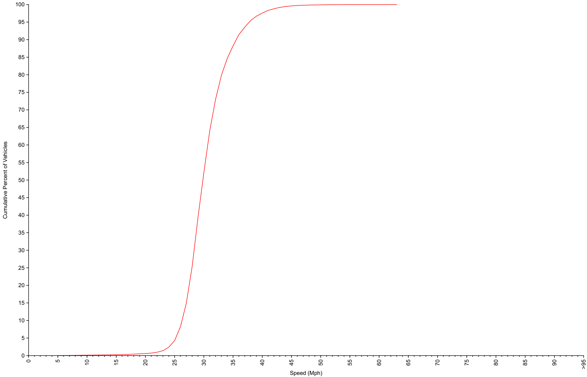
Cumulative Speed Distribution Curve Traffic Overview from Sat Aug 2 2025 to Sun Aug 31 2025
