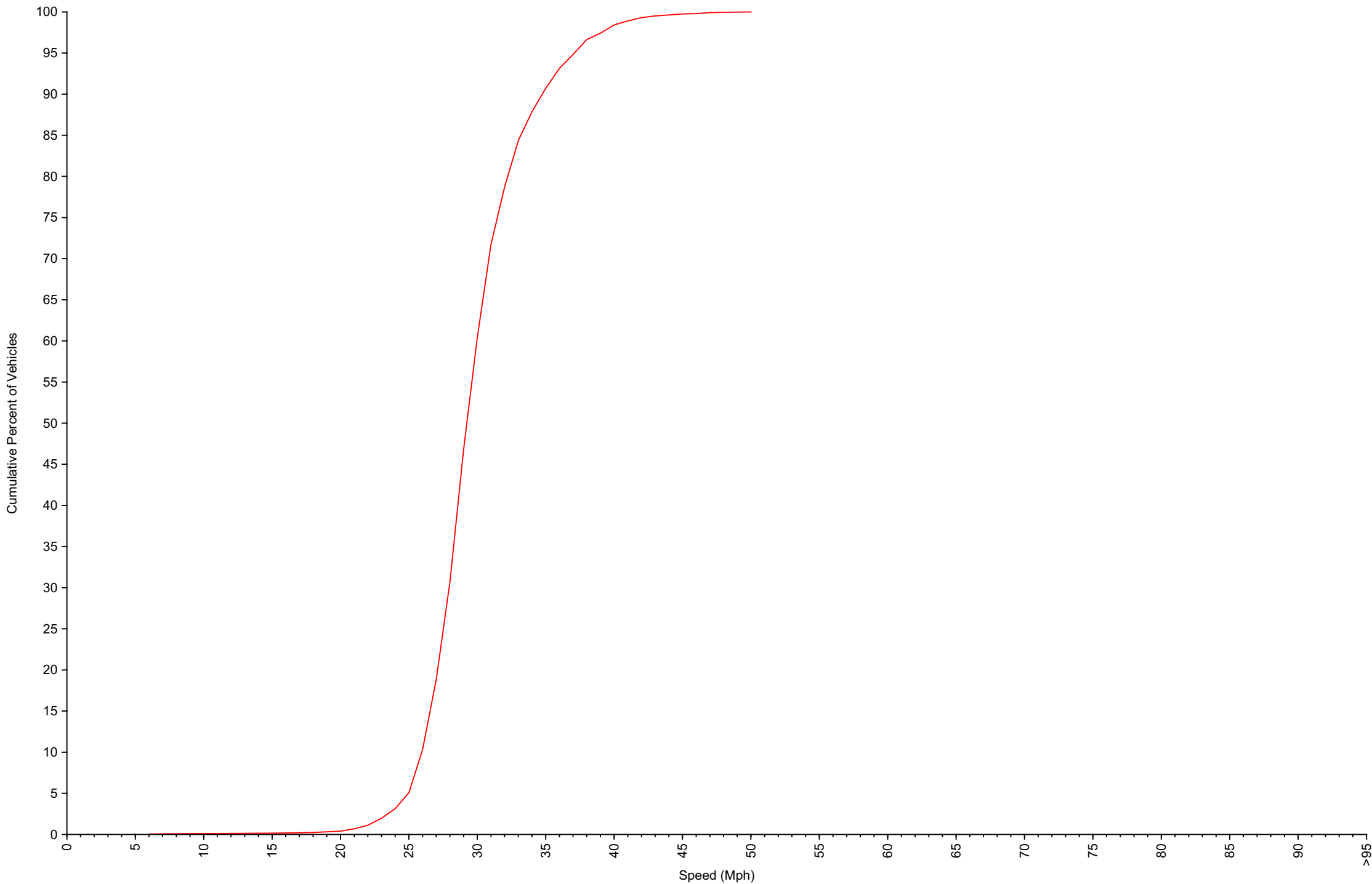
Cumulative Speed Distribution Curve Daily Overview for Tue Aug 19 2025
