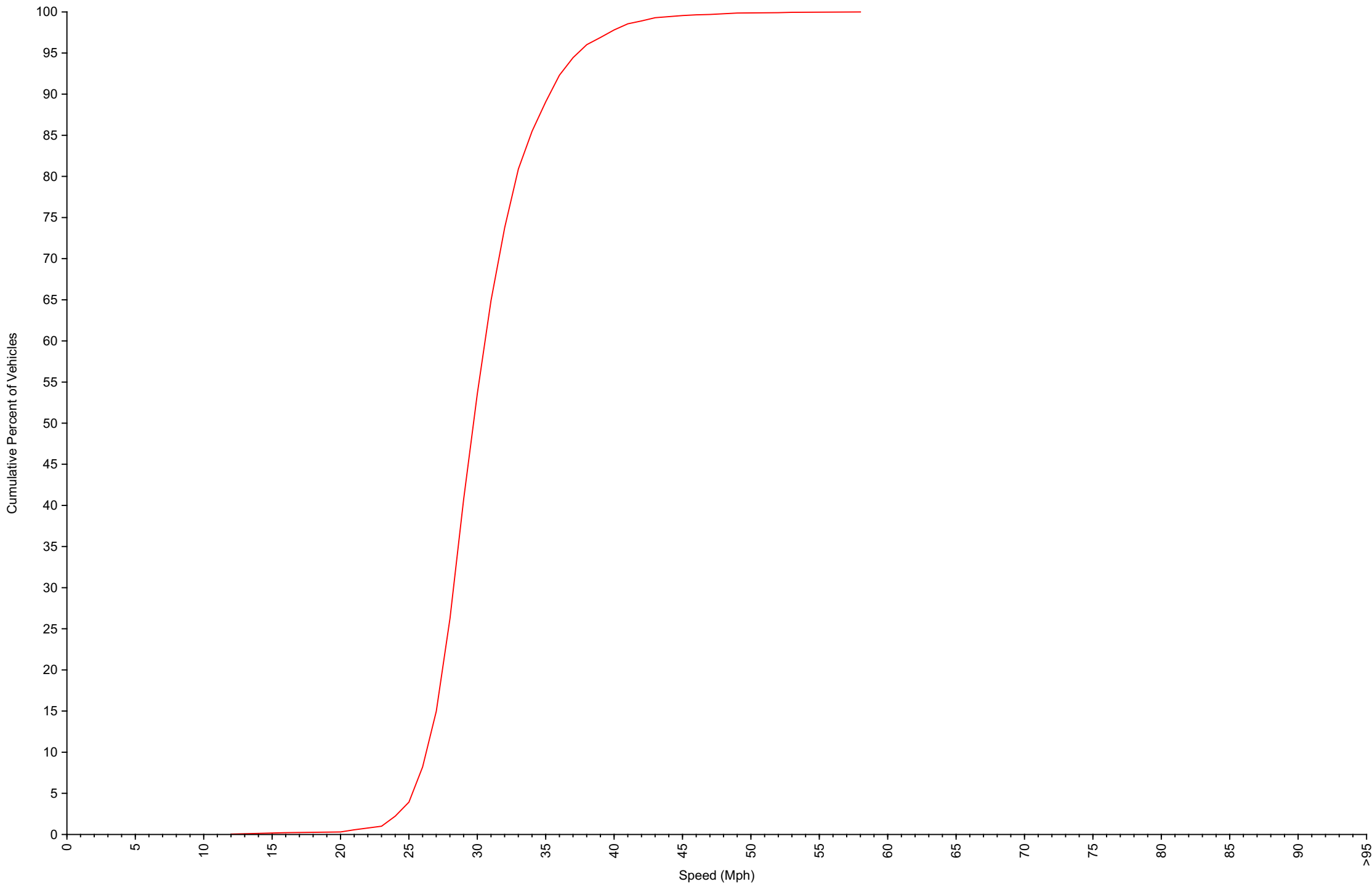
Cumulative Speed Distribution Curve Daily Overview for Mon Aug 11 2025
