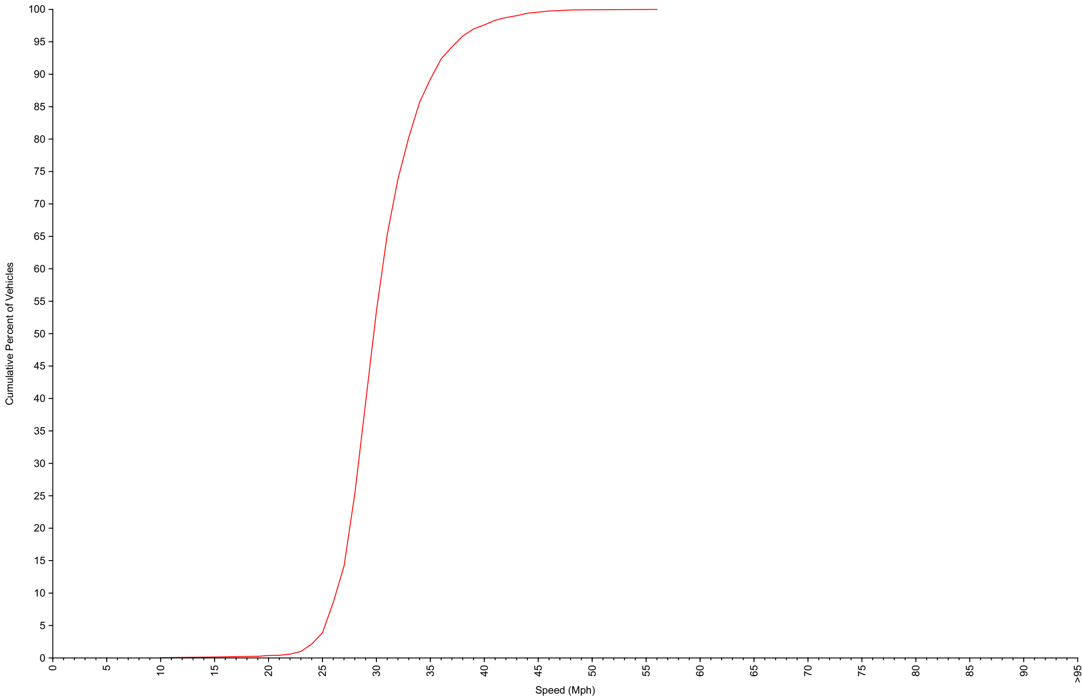
Cumulative Speed Distribution Curve Daily Overview for Wed Aug 6 2025
