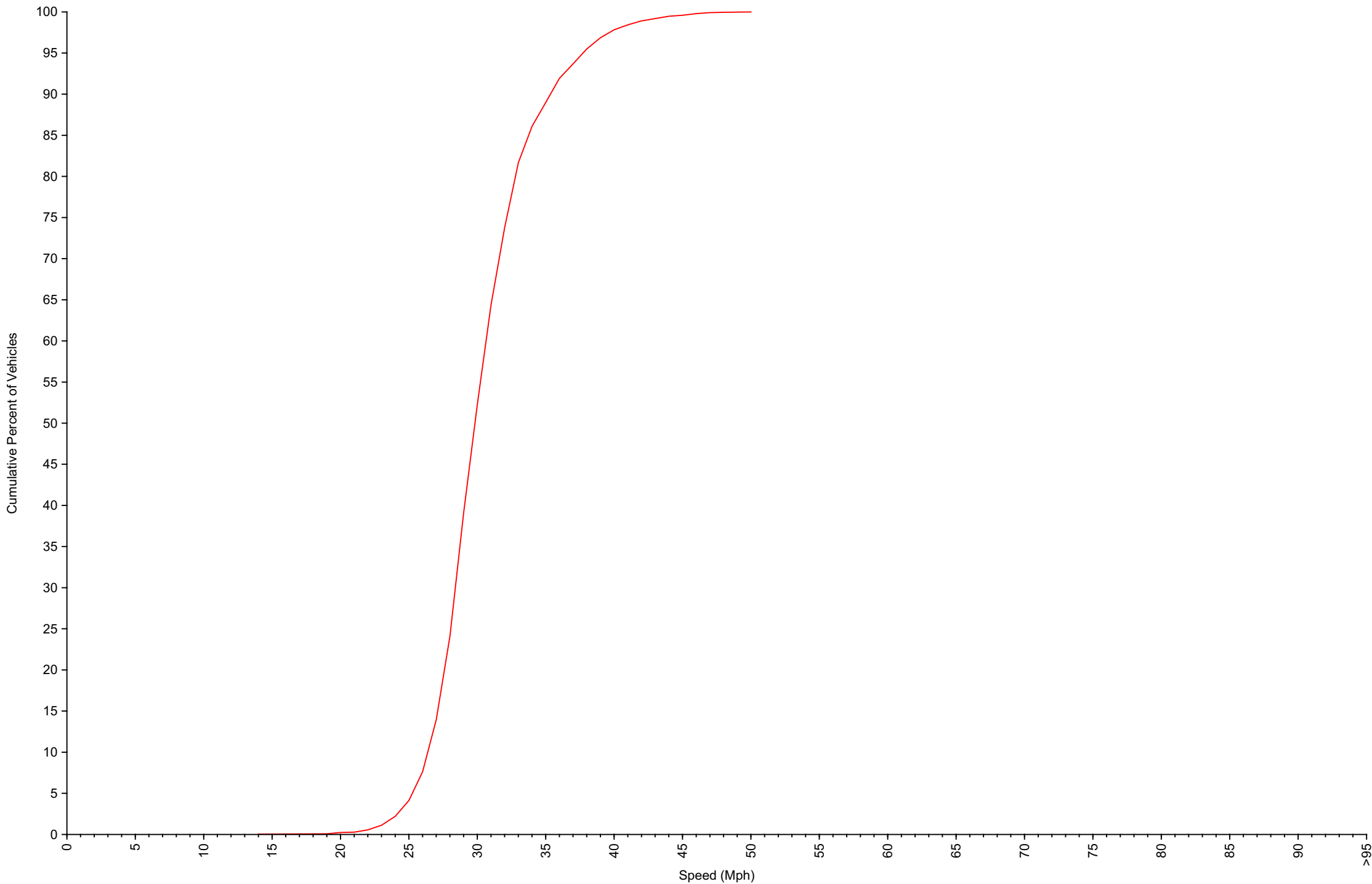
Cumulative Speed Distribution Curve Daily Overview for Fri Aug 29 2025
