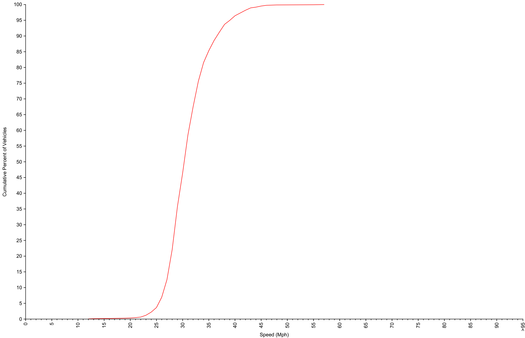
Cumulative Speed Distribution Curve Daily Overview for Sun Aug 3 2025
