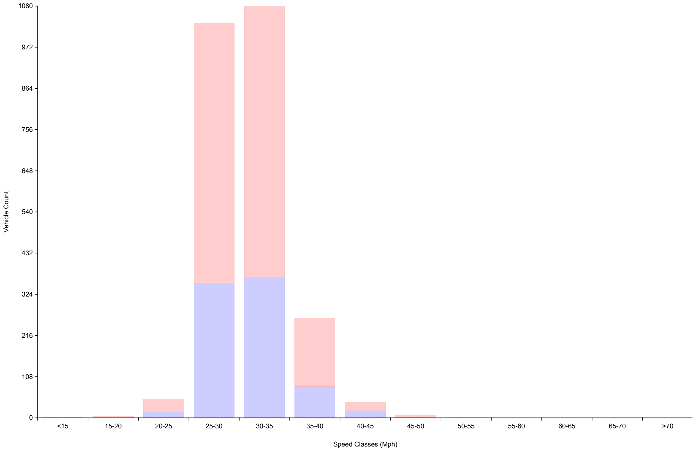
Vehicle Counts By Speed Class Daily Overview for Thu Aug 28 2025
