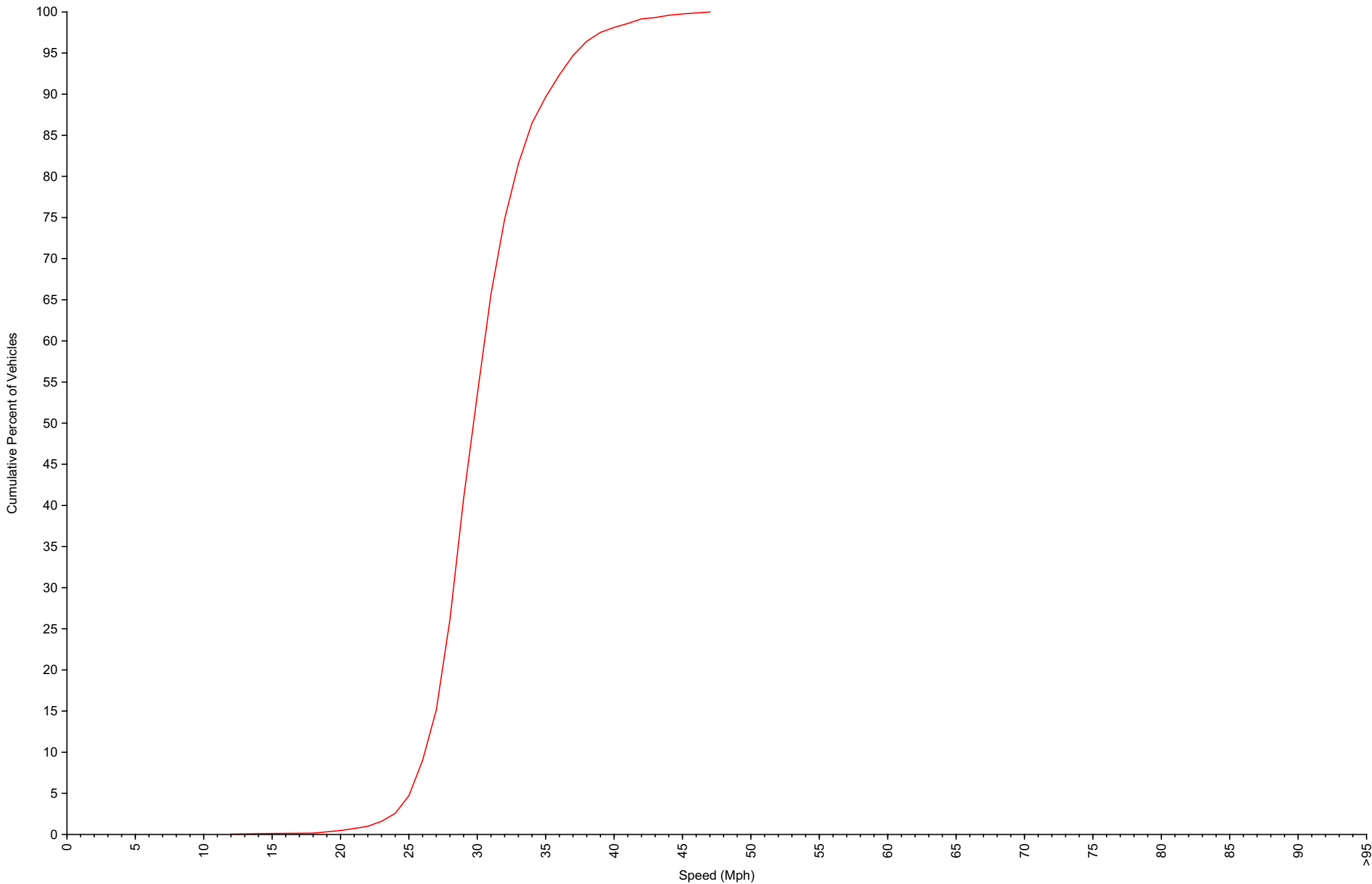
Cumulative Speed Distribution Curve Daily Overview for Thu Aug 14 2025
