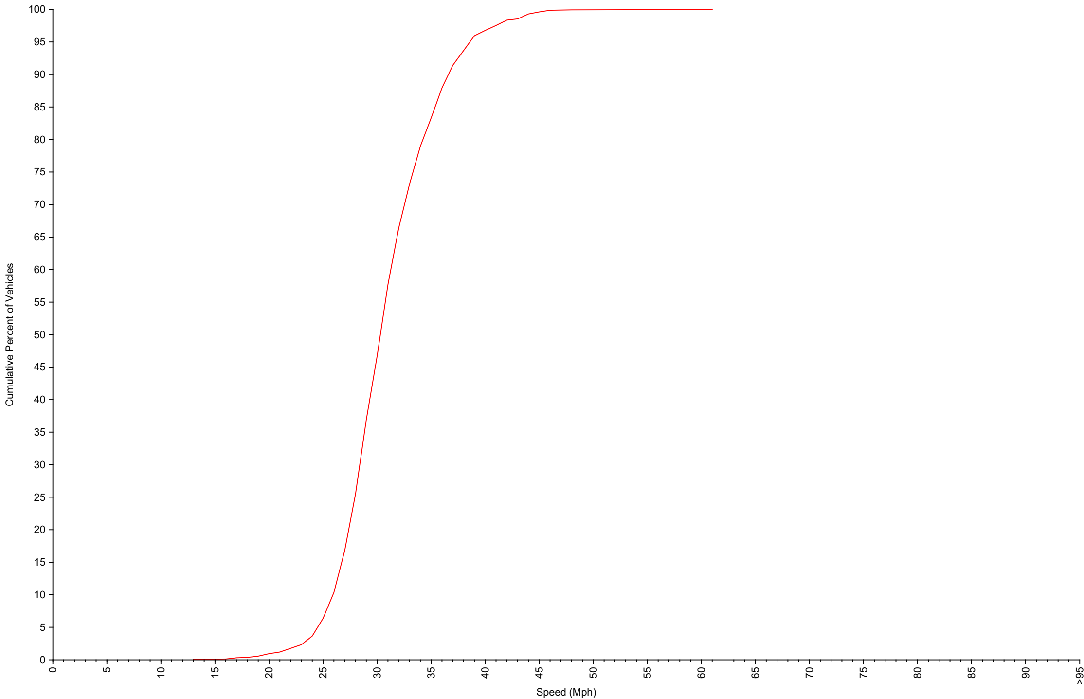
Cumulative Speed Distribution Curve Daily Overview for Wed Aug 13 2025
