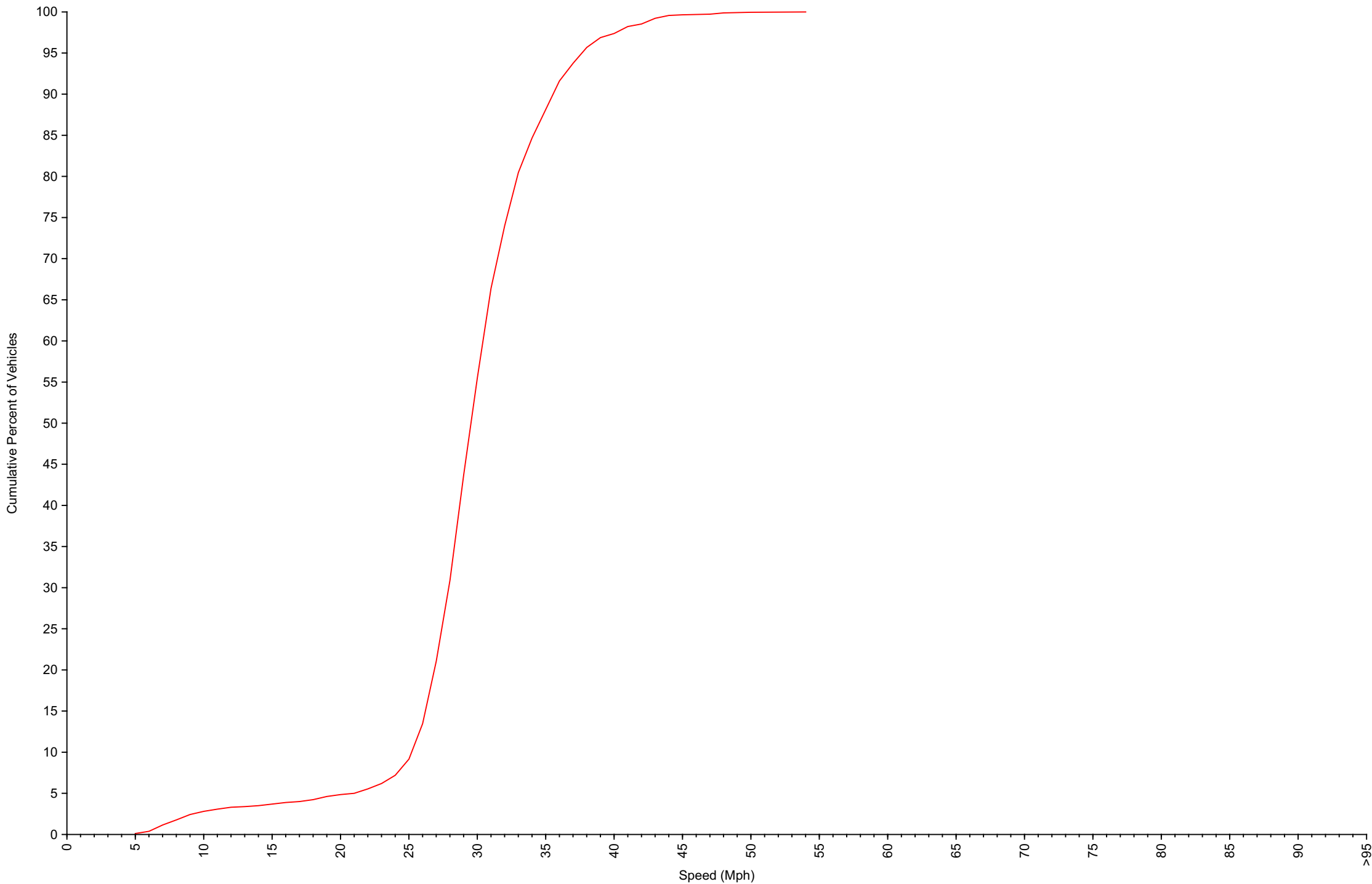
Cumulative Speed Distribution Curve Daily Overview for Tue Aug 12 2025
