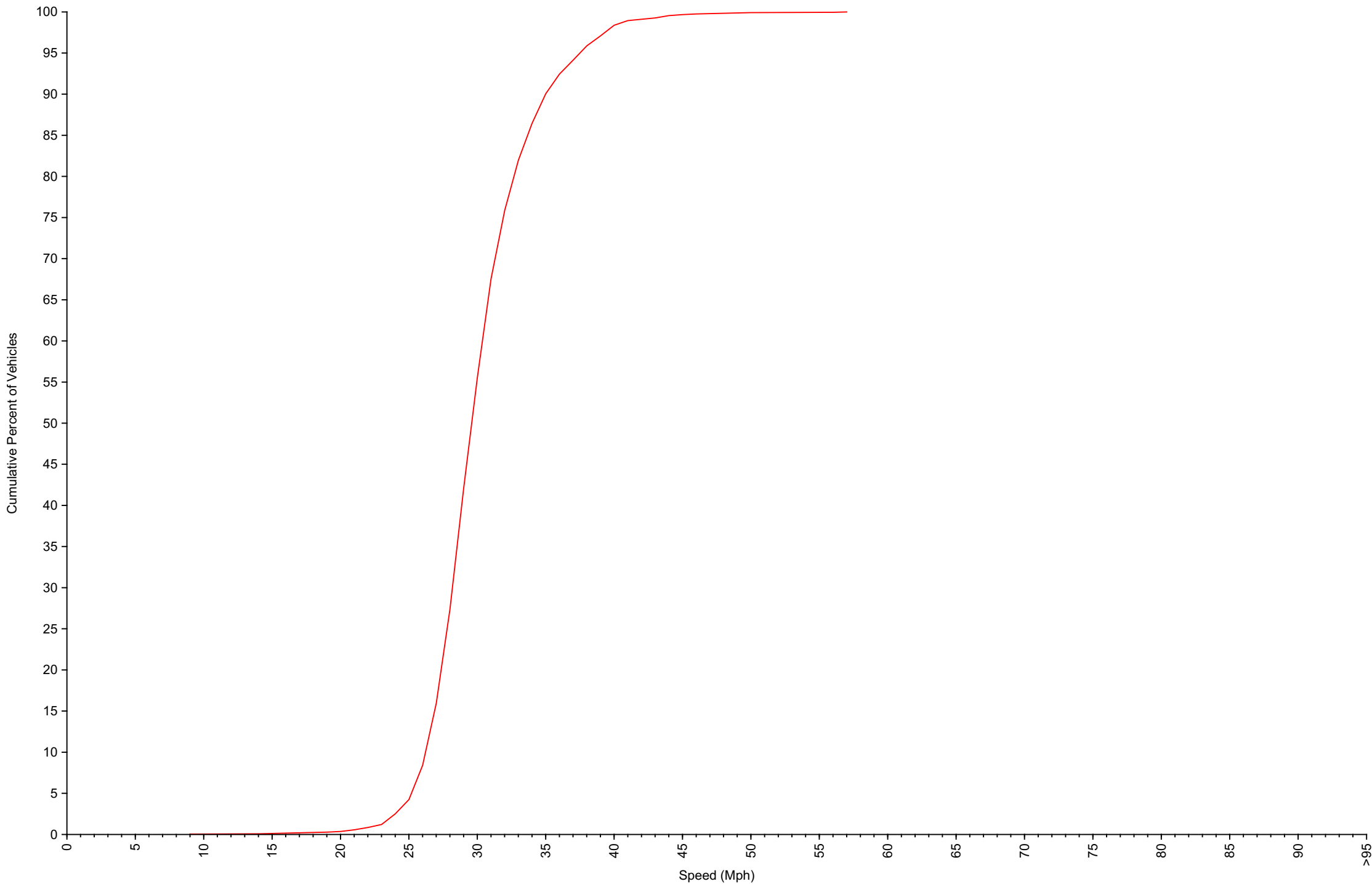
Cumulative Speed Distribution Curve Daily Overview for Thu Sep 4 2025
