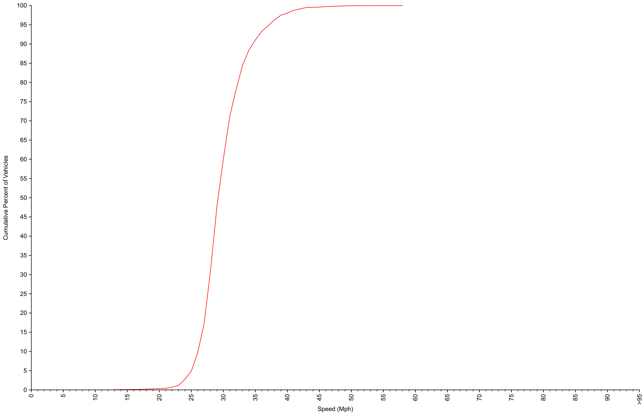
Cumulative Speed Distribution Curve Daily Overview for Mon Sep 15 2025
