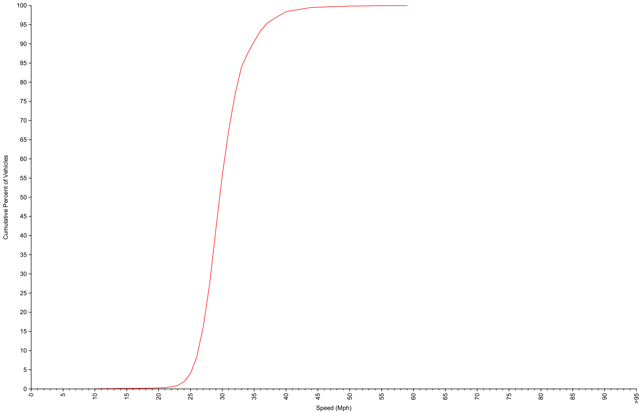
Cumulative Speed Distribution Curve Daily Overview for Tue Sep 23 2025
