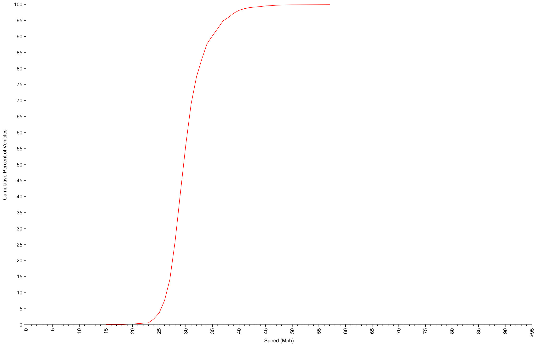
Cumulative Speed Distribution Curve Daily Overview for Mon Sep 8 2025
