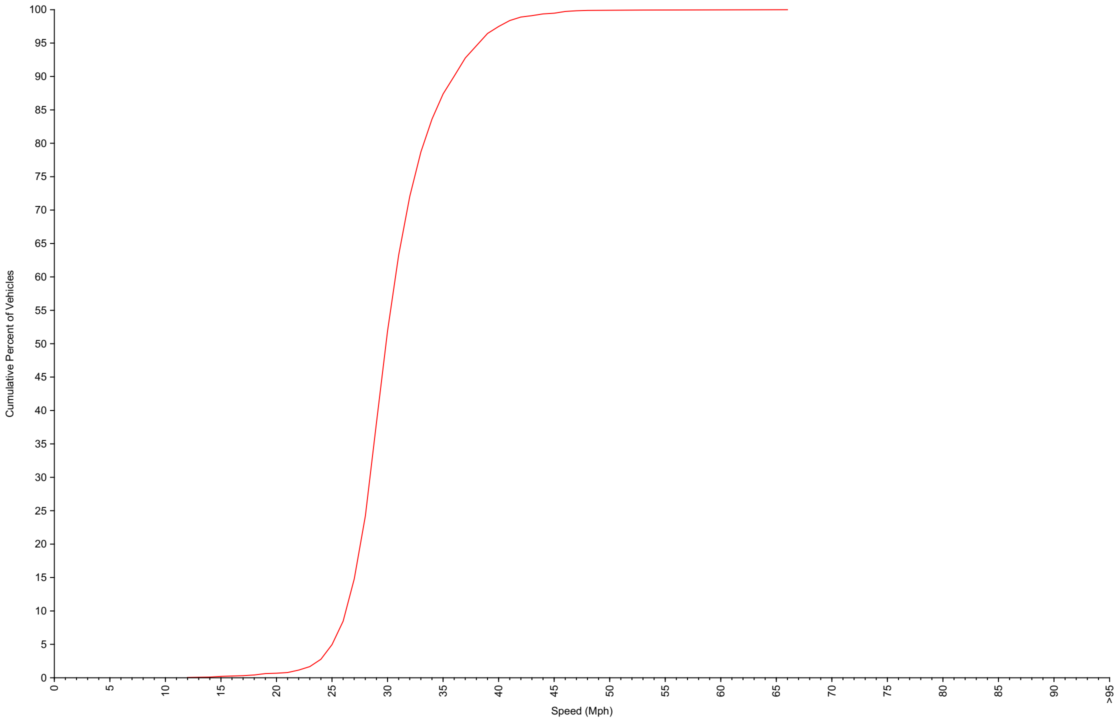
Cumulative Speed Distribution Curve Daily Overview for Sun Sep 28 2025
