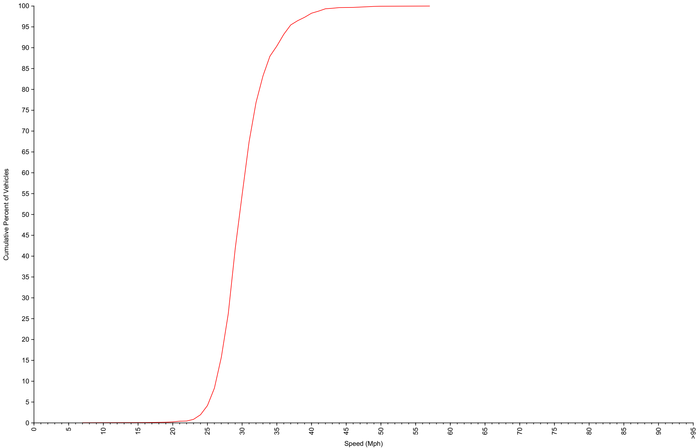
Cumulative Speed Distribution Curve Daily Overview for Mon Sep 1 2025
