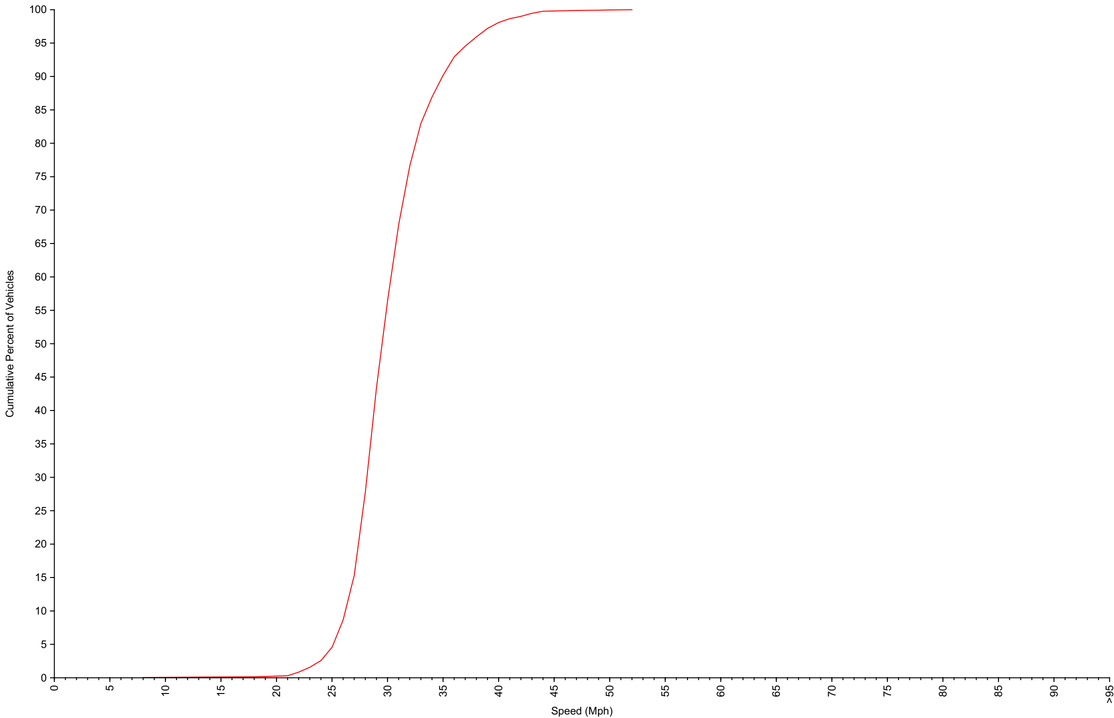
Cumulative Speed Distribution Curve Daily Overview for Fri Sep 26 2025
