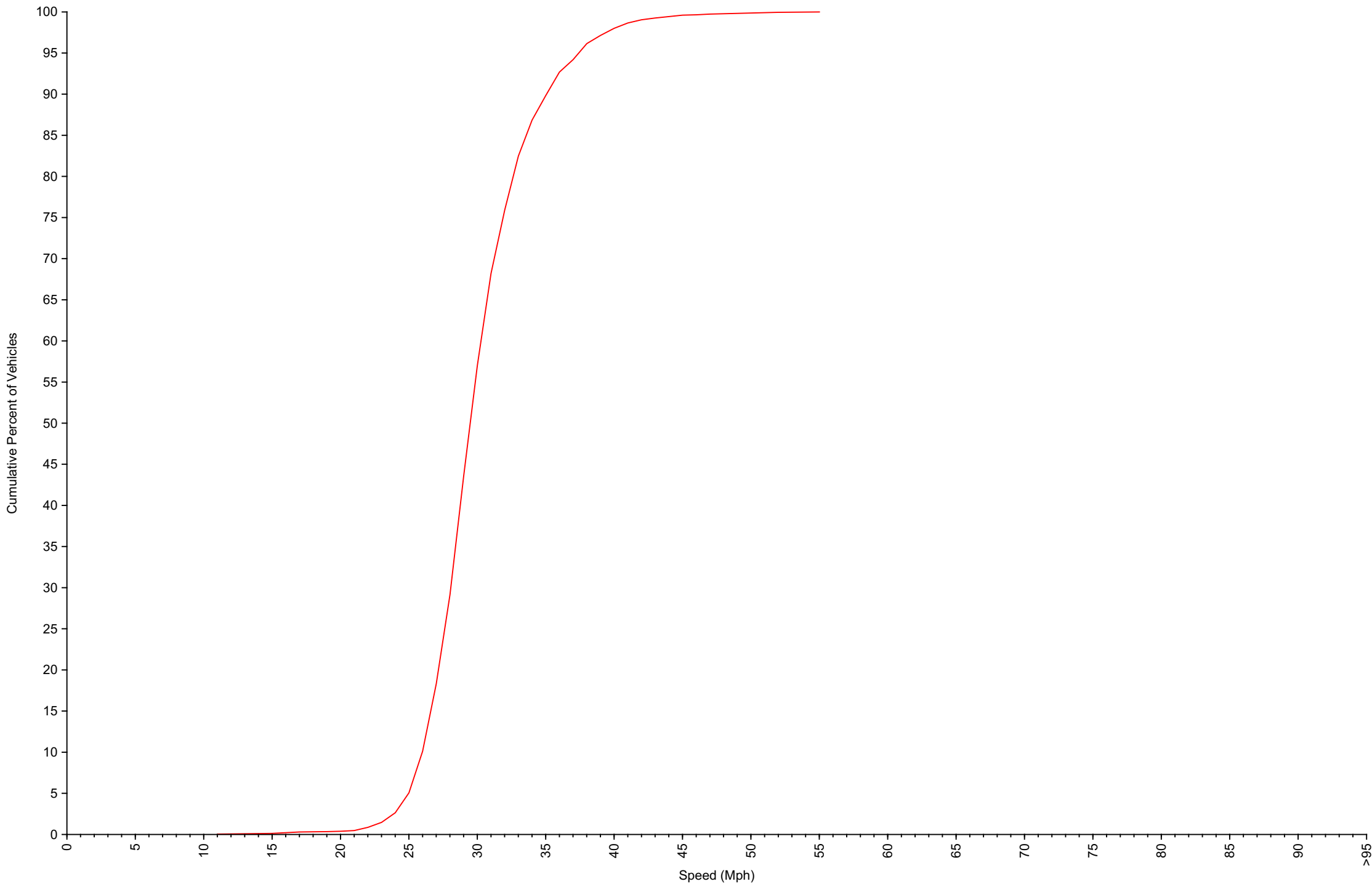
Cumulative Speed Distribution Curve Daily Overview for Mon Sep 22 2025
