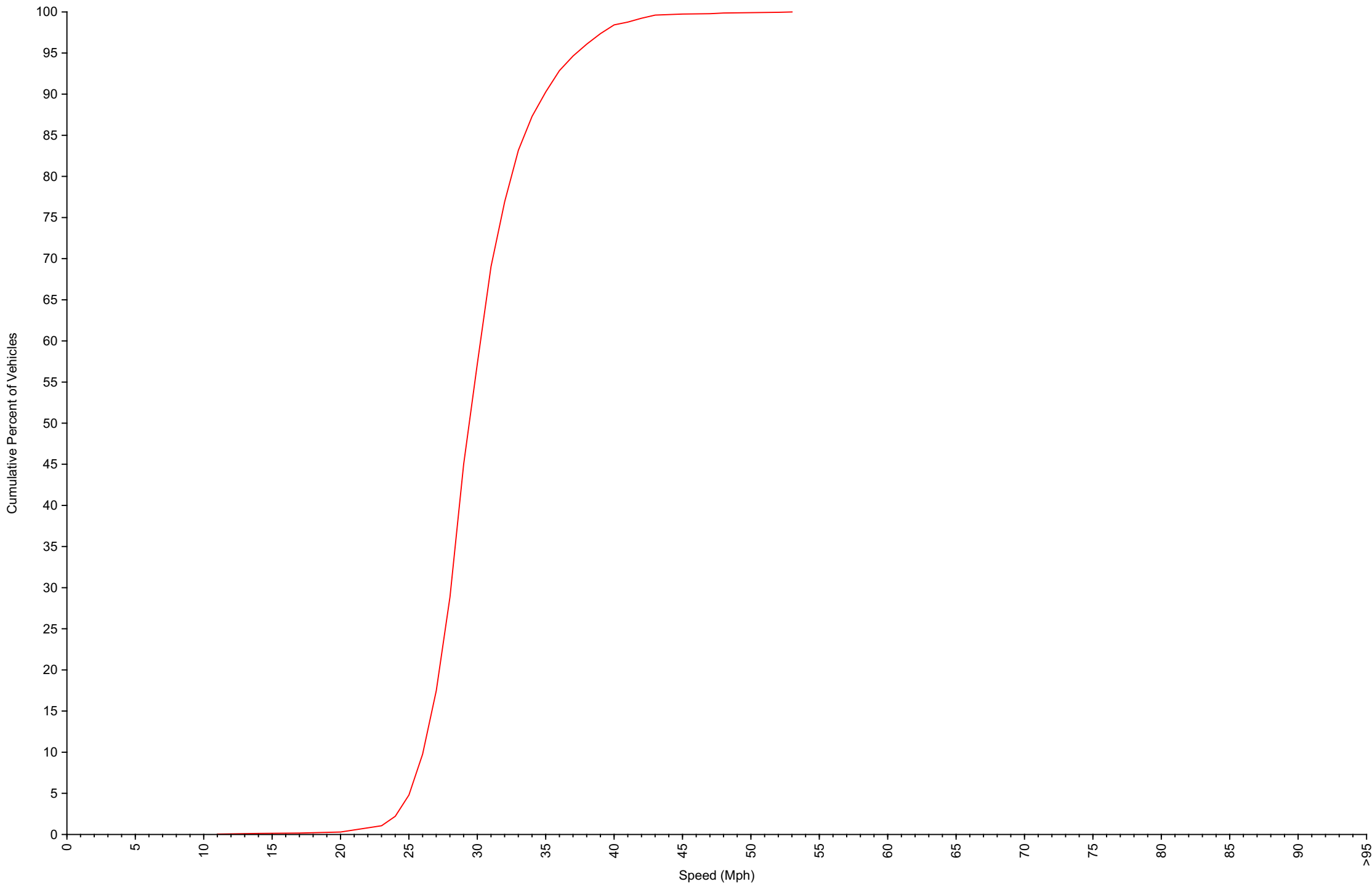
Cumulative Speed Distribution Curve Daily Overview for Mon Sep 29 2025
